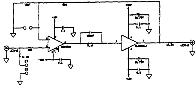
Fig. 2. Schematic diagram of a buffer/driver channel.
