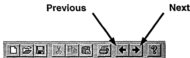
Figure 17: Toolbar
