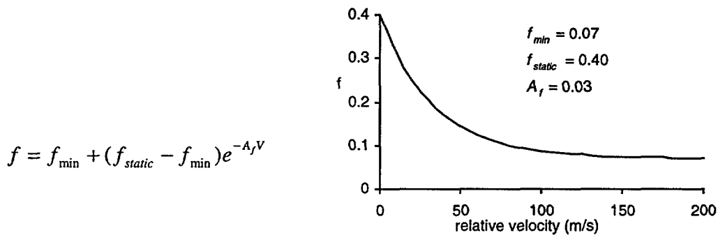
Figure 10: Friction Model
