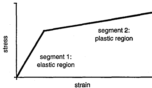
Figure 9: Material Model
