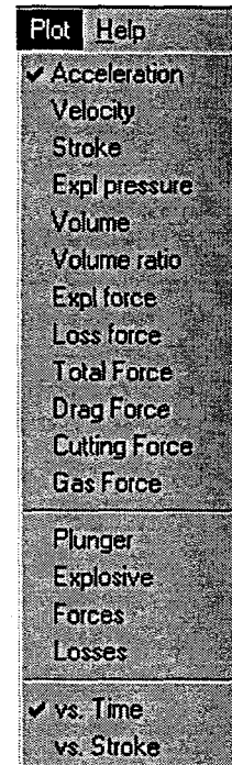
Figure 16: Plot Menu
