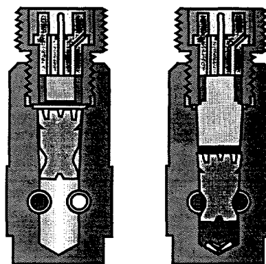
Figure 1: Valve Operation
