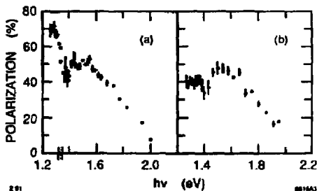
Figure 3. Electron spin-polarization as a function of excitation photon energy for the 0.1 μm-thick sample (a) and for the 1.14 μm-thick sample (b). The shaded region in Fig. 3a shows the expected light hole to conduction band energy difference compatible with the indium concentration uncertainty and the thin sample X-ray analysis.
