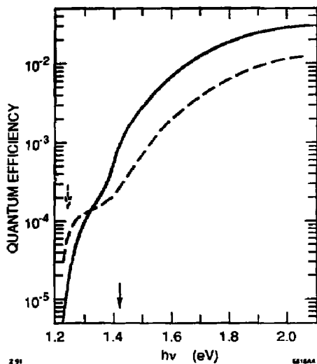
Figure 2. Cathode quantum efficiency as a function of excitation photon energy. The solid curve is for the 0.1 μm-thick sample, and the dashed curve is for the 1.14 μm-thick sample. The band gap energies of GaAs (solid arrow) and relaxed InGaAs (dashed arrow) are indicated.
