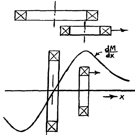
Fig. 1: The mutual inductance gradient as a function of drive coil position for planar and axial mass drivers; ref. 6.
