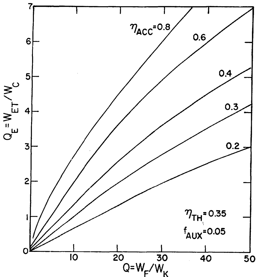
Fig. 2 Parametric systems design curves for an Impact Fusion Reactor (IFR).
