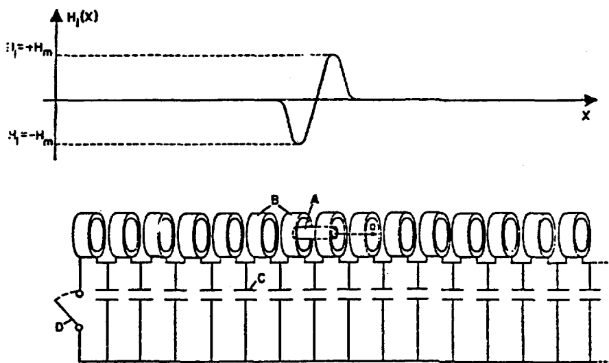
FIG. 5.—Transmission line accelerator. A: accelerated solenoid; B: field coils; C: capacitors; D: switch to be closed to start travelling magnetic wave. H_1(x) : magnetic field on transmission line relative to the frame of the solenoid. n(x) : windings per unit length in field coils (arbitrary units).
