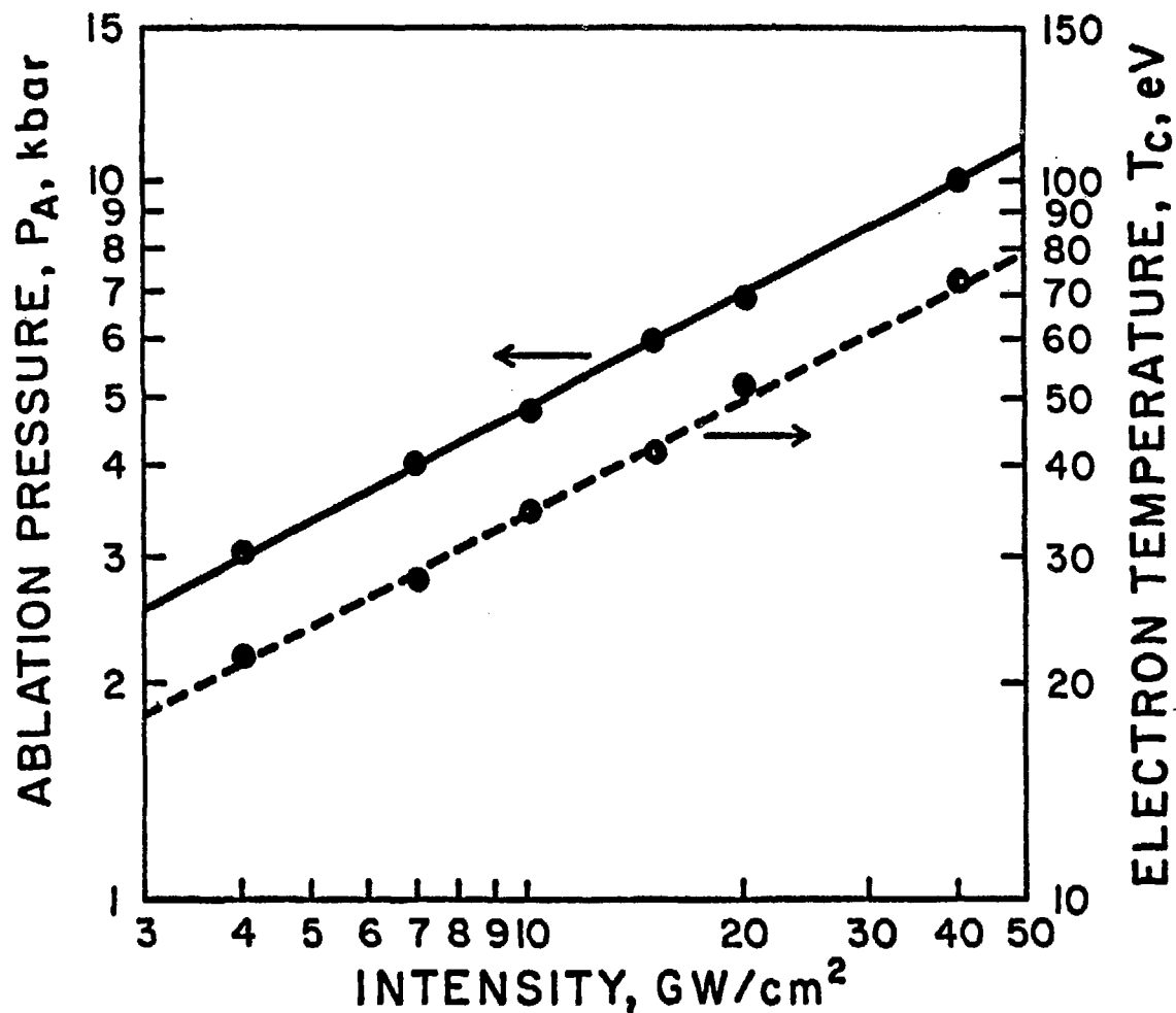
Fig 4 Ablation pressure and electron temperature at the absorption surface as a function of laser intensity. The laser wavelength, \lambda = 5\mu . The solid circles are time ( 0.5 \mu\text{sec} ) averaged results from the 1-D calculations.
