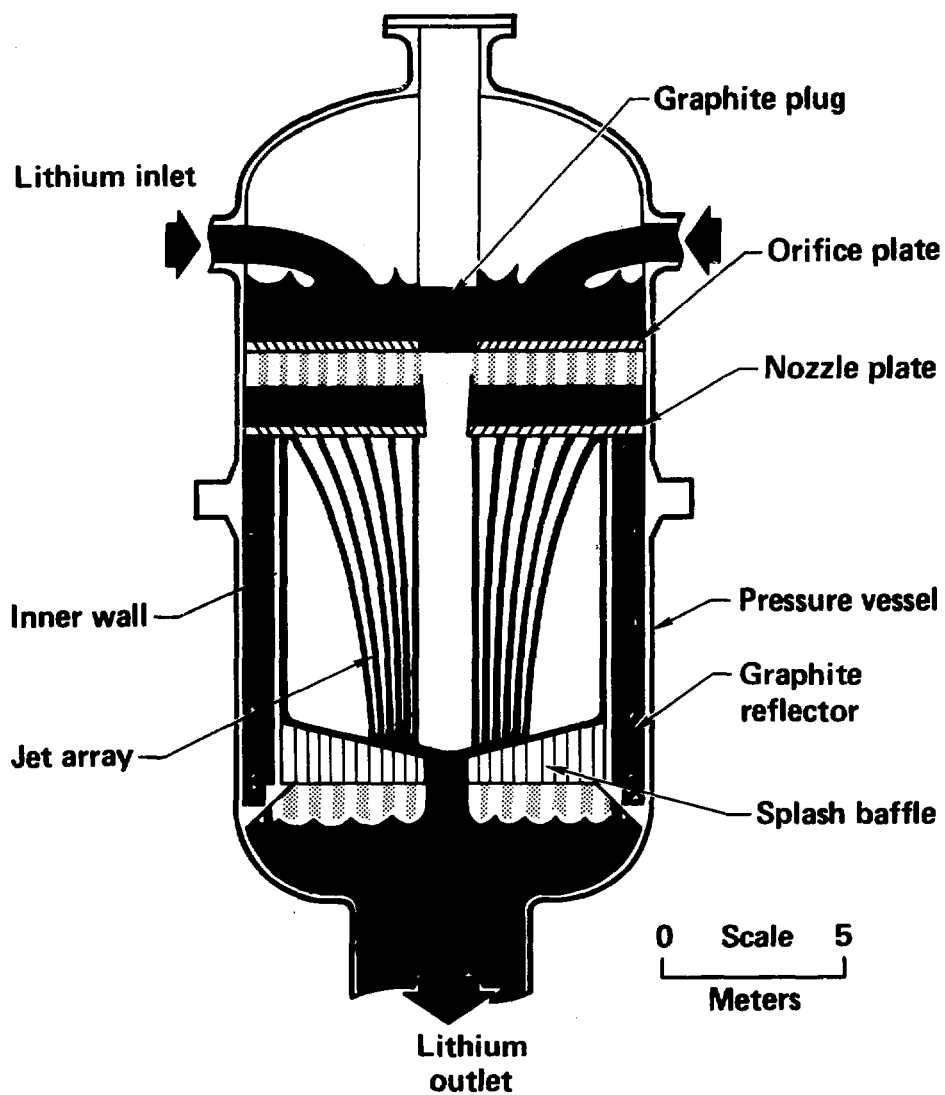
Fig.5 The HYLIFE Converter Concept.
