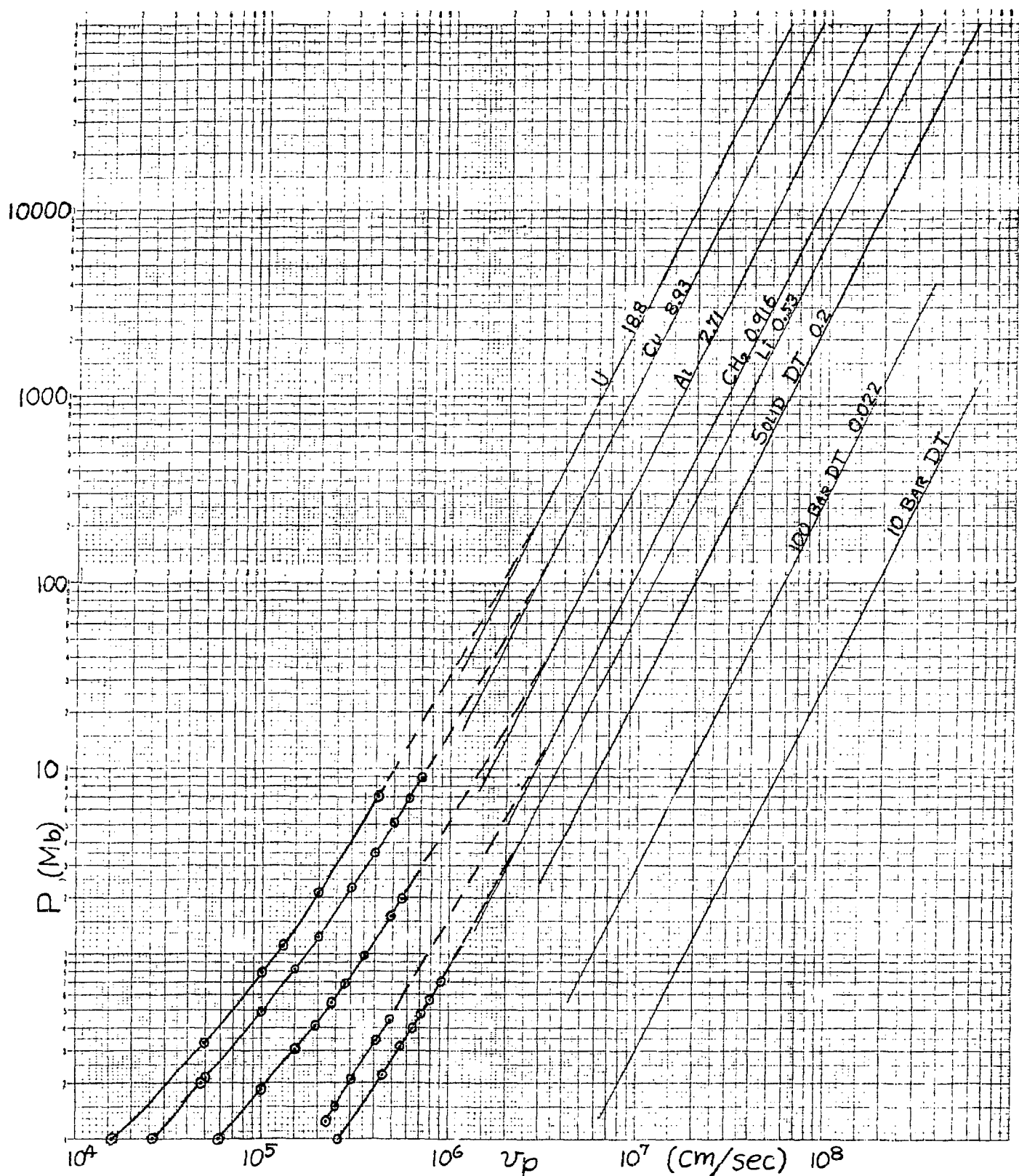
Fig. 1. Pressure vs. particle velocity Hugonicts for representative materials. Hugonicts are experimental below 10^6 cm/sec and 10 Mb. Straight lines at high velocity and pressure assume \gamma = 5/3 gas law behavior.
