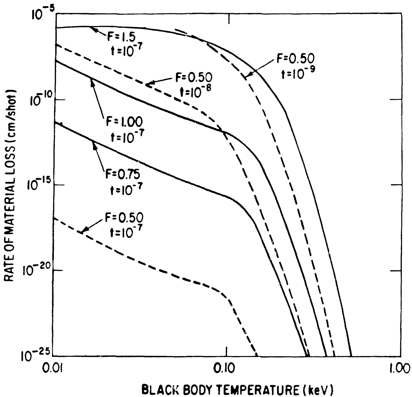
Fig. 1 Rate of material loss of carbon surface from x rays. F is fluence in \text{J}/\text{cm}^2 , t is pulse width in seconds.
