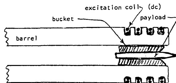
Fig. 5: The Momentum Transformer.
