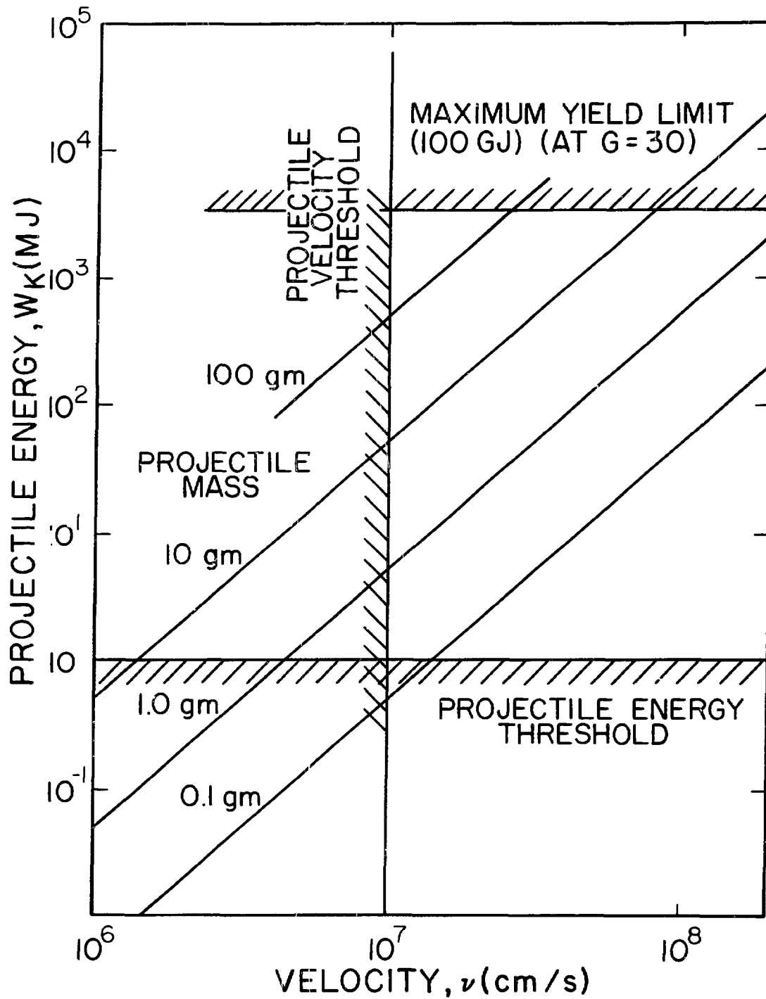
PROJECTILE ENERGY, MASS, VELOCITY RELATIONS Fig.4
