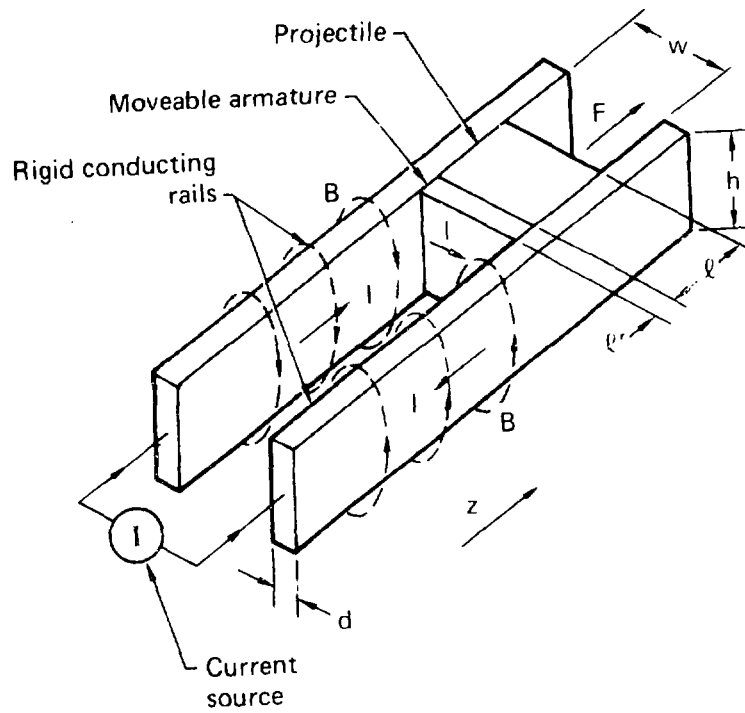
Fig. 1 Schematic diagram of a rail gun (11)
