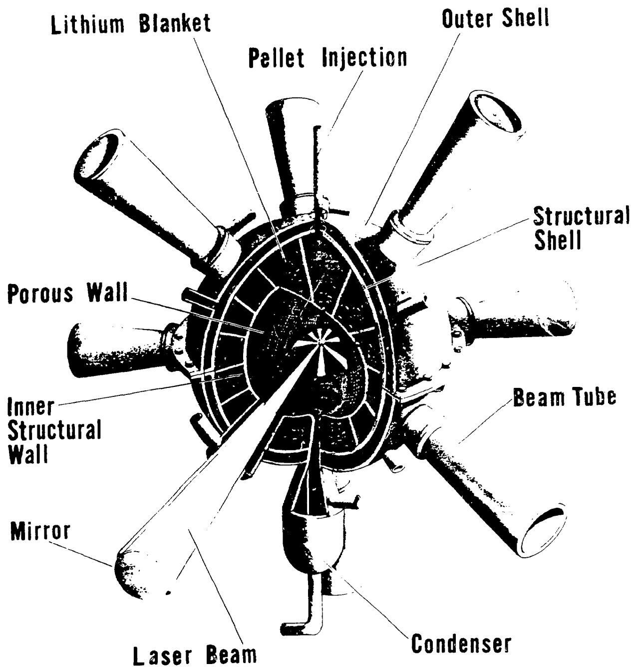
Fig. 3. The wetted-wall reactor concept
