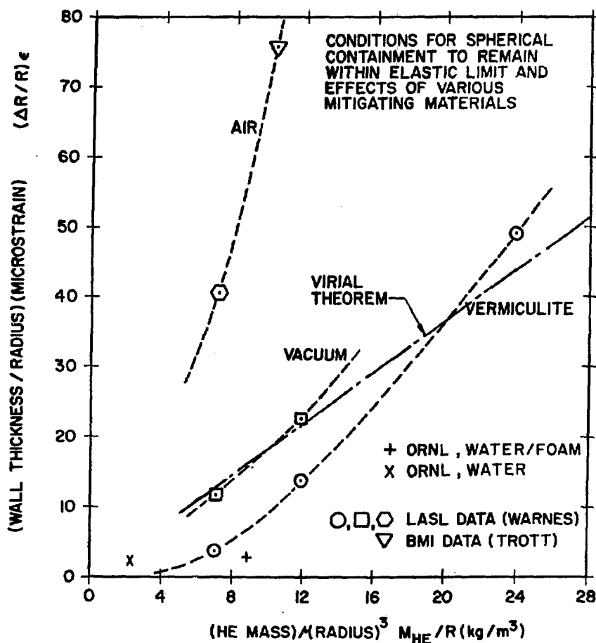
Fig. 1. Virial-theorem scaling of blast-confinement data using high-explosive detonations in spherical vessels. All data represent tests which measured only the onset of plastic deformation of the blast-containment vessel. ORNL (Ref.5), LASL (Ref.7), BMI (Ref.13).
