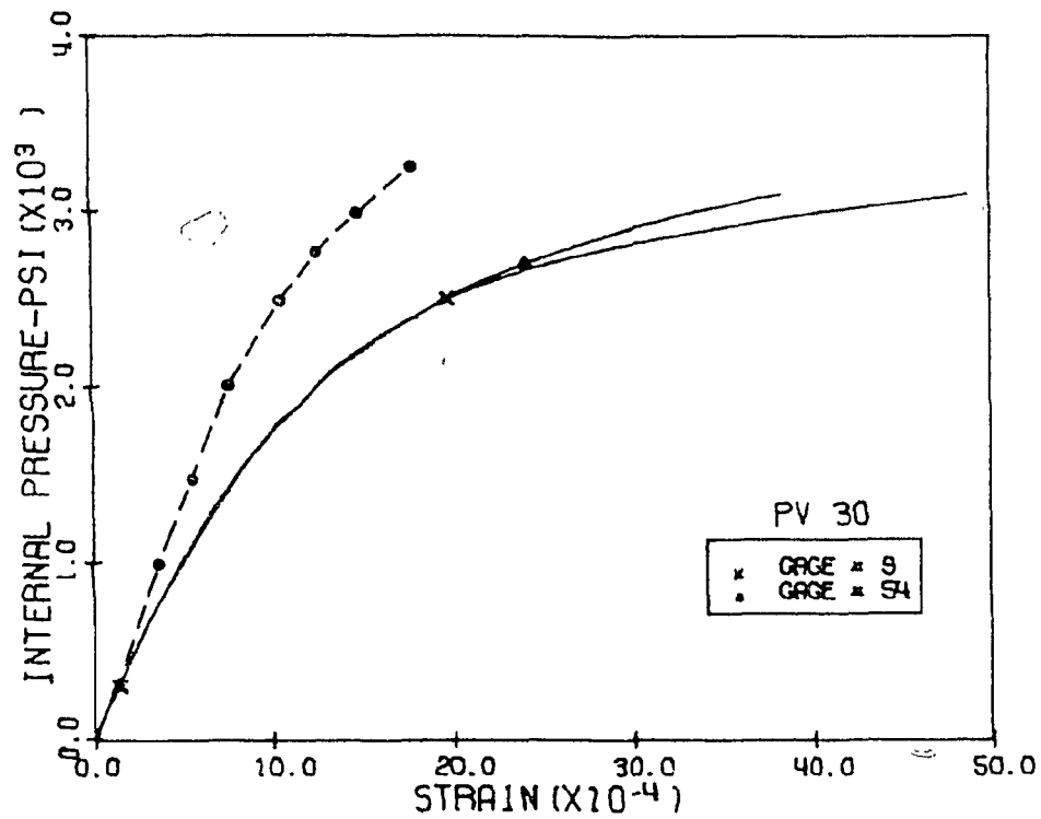
Fig. 5.15 Measured and Calculated Compression Diagonal Strains, Level 3 Penetrations 1 and 3, PV30
