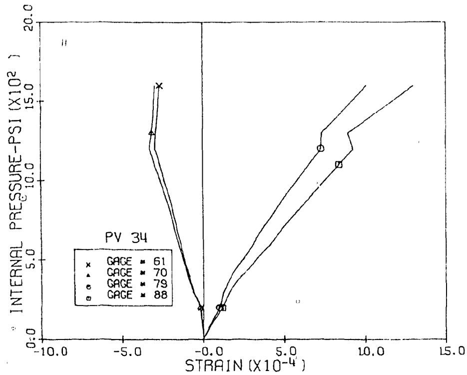
Fig. 3.92 Measured Vertical Strains, Level 3, Pen. 4 & 5, PV34
