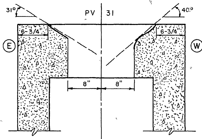
Fig. 3.8a End Slab after Test PV31
