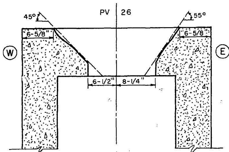
Fig. 3.3 End Slab after Test, PV26
