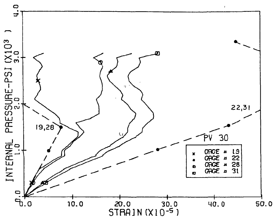
Fig. 5.17 Measured and Calculated Vertical Strains, Levels 1 and 2 Penetration 2, PV30
