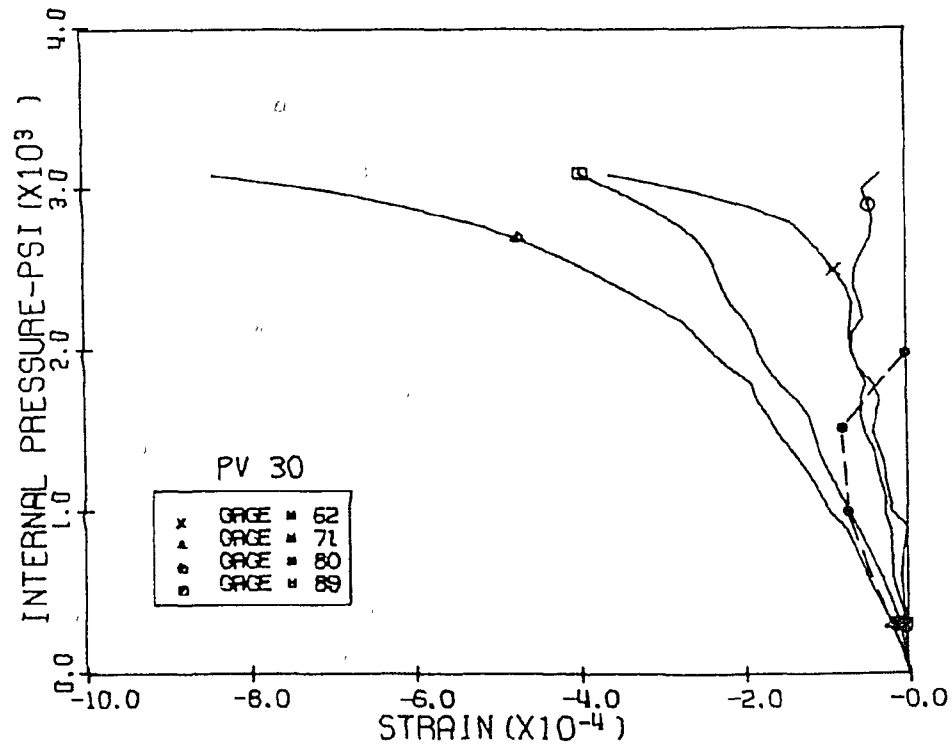
Fig. 5.31 Measured and Calculated Horizontal Strains, Level 3 Penetrations 4 and 5, PV30
