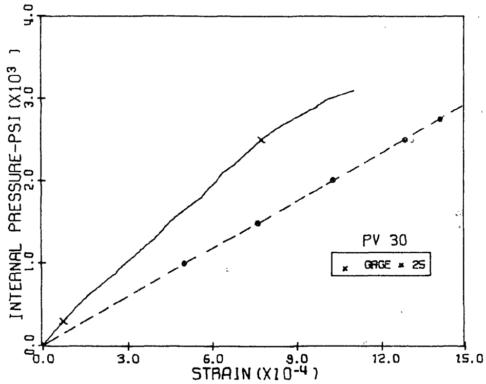
Fig. 5.20 Measured and Calculated Vertical Strain, Level 3 Penetration 2, PV30
