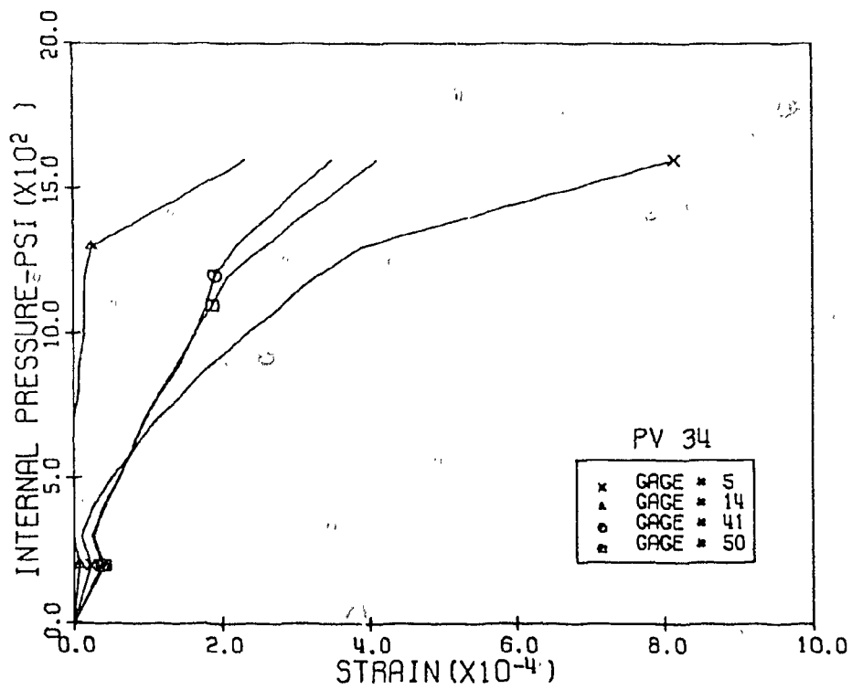
Fig. 3.72 Measured Horizontal Strains, Level 2, Pen. 1 & 3, PV34
