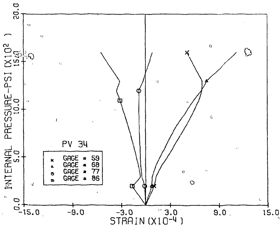
Fig. 3.89 Measured Horizontal Strains, Level 2, Pen. 4 & 5, PV34
