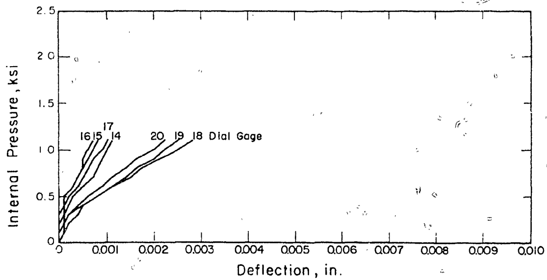
Fig. A.25 Measured Pressure-Deflection Curves, Test PV31.1
