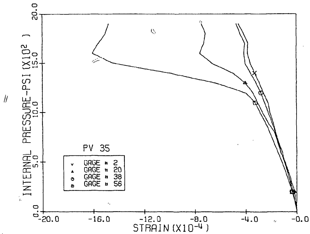
Fig. 3.96 Measured Horizontal Strains, Level 1, 12:00 & 6:00 Pos., PV35
