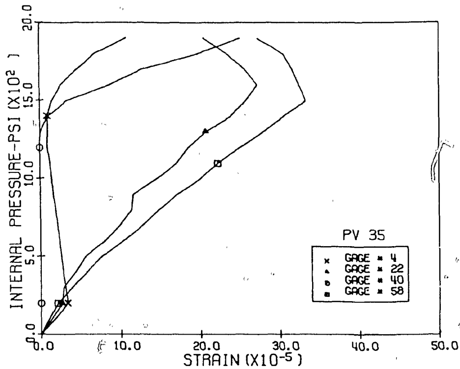
Fig. 3.105 Measured Vertical Strains, Level 2, 12:00 & 6:00 Pos., PV35
