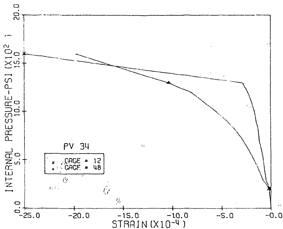
Fig. 3.69 Measured Comp. Diag. Strains, Level 1, Pen. 1 & 3, PV34
