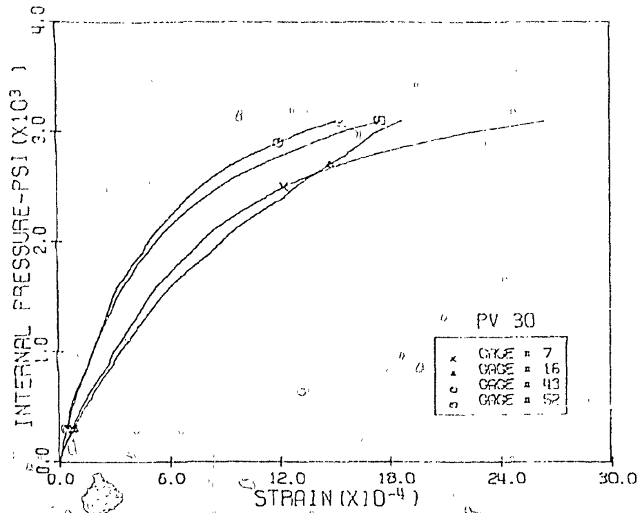
Fig. 3.25 Measured Vertical Strains, Level 3, Pen. 1 & 3, PV30
