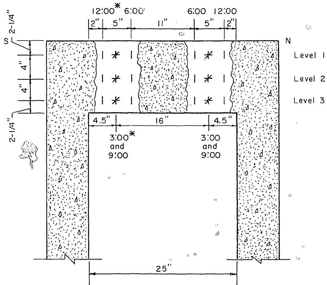
Fig. 3.16c Location of Strain Rosettes in the Vertical Plane (*Numerals designating location in plan. See Fig. 5.31a)
