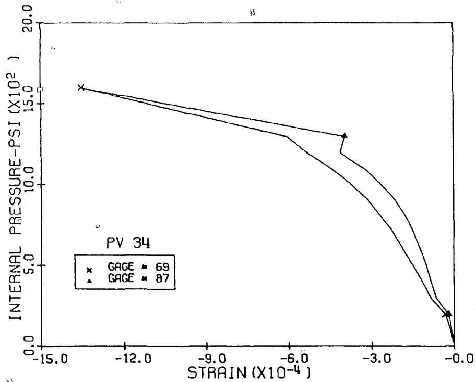
Fig. 3.91 Measured Tens. Diag. Strains, Level 2, Pen. 4 & 5, PV34
