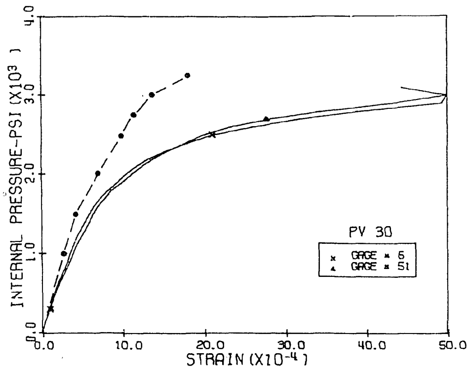
Fig. 5.11 Measured and Calculated Compression Diagonal Strains, Level 2 Penetrations 1 and 3, PV30
