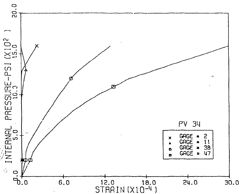
Fig. 3.68 Measured Horizontal Strains, Level 1, Pen. 1 & 3, PV34
