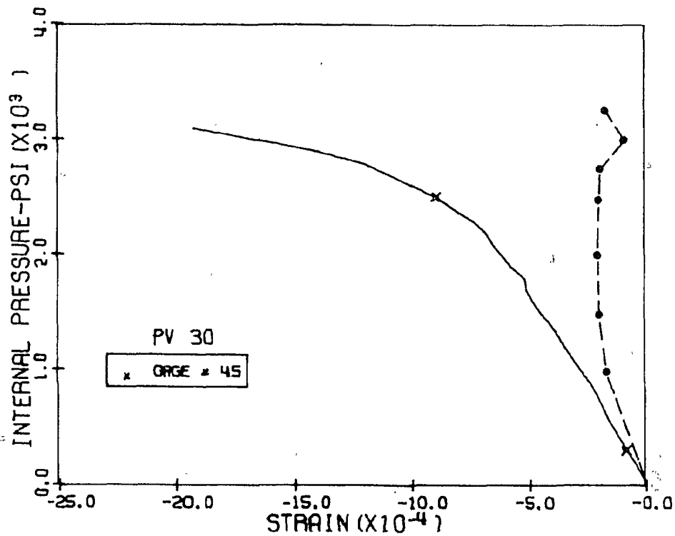
Fig. 5.16 Measured and Calculated Tension Diagonal Strains, Level 3 Penetrations 1 and 3, PV30
