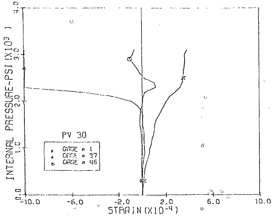
Fig. 3.17 Measured Vertical Strains, Level 1, Pen. 1 & 3, PV30
