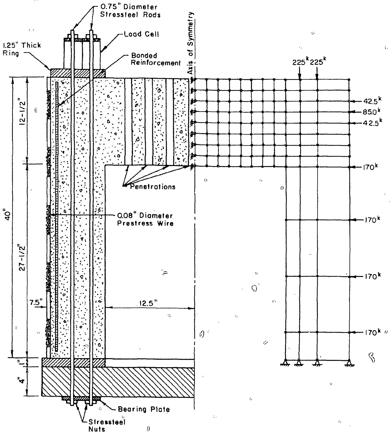
Fig. 5.1 Cross-section of PV30 and the Axisymmetric Finite Element Mesh Used in the Analysis
