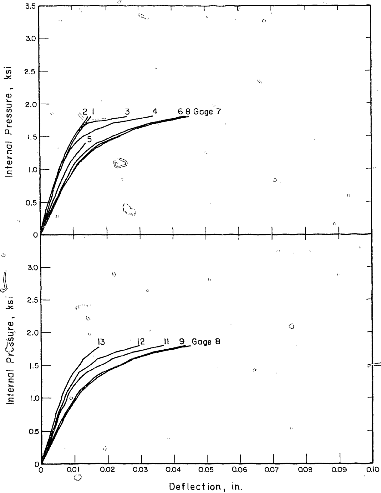
Fig. A.35 Measured Pressure-Deflection Curves, End Slab, PV35 (See Fig. A.28 for Gage Locations)
