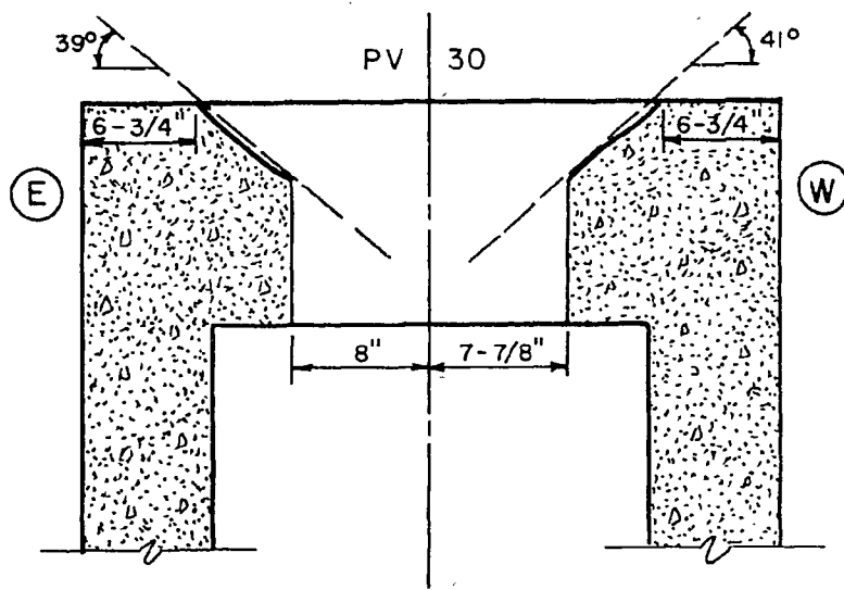
Fig. 3.7 End Slab after Test PV30
