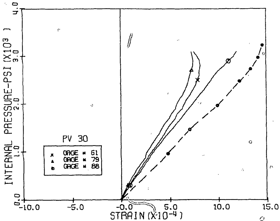
Fig. 5.30 Measured and Calculated Vertical Strains, Level 3 Penetrations 4 and 5, PV30
