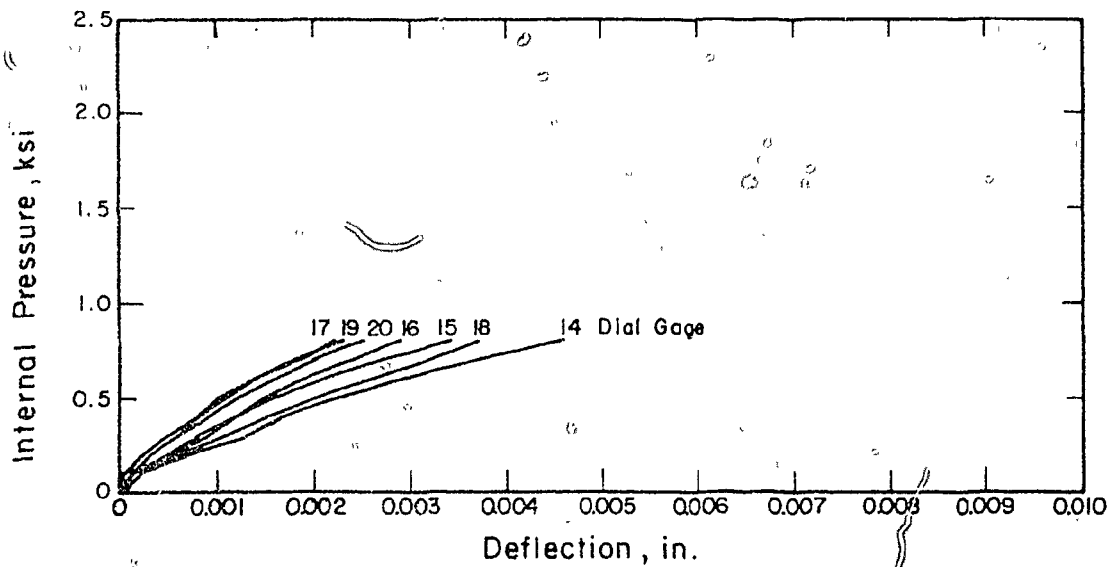
Fig. A.13 Measured Pressure-Deflection Curves, Test PV26.1
