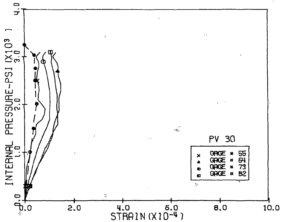
Fig. 5.22 Measured and Calculated Vertical Strains, Level 1 Penetrations 4 and 5, PV30
