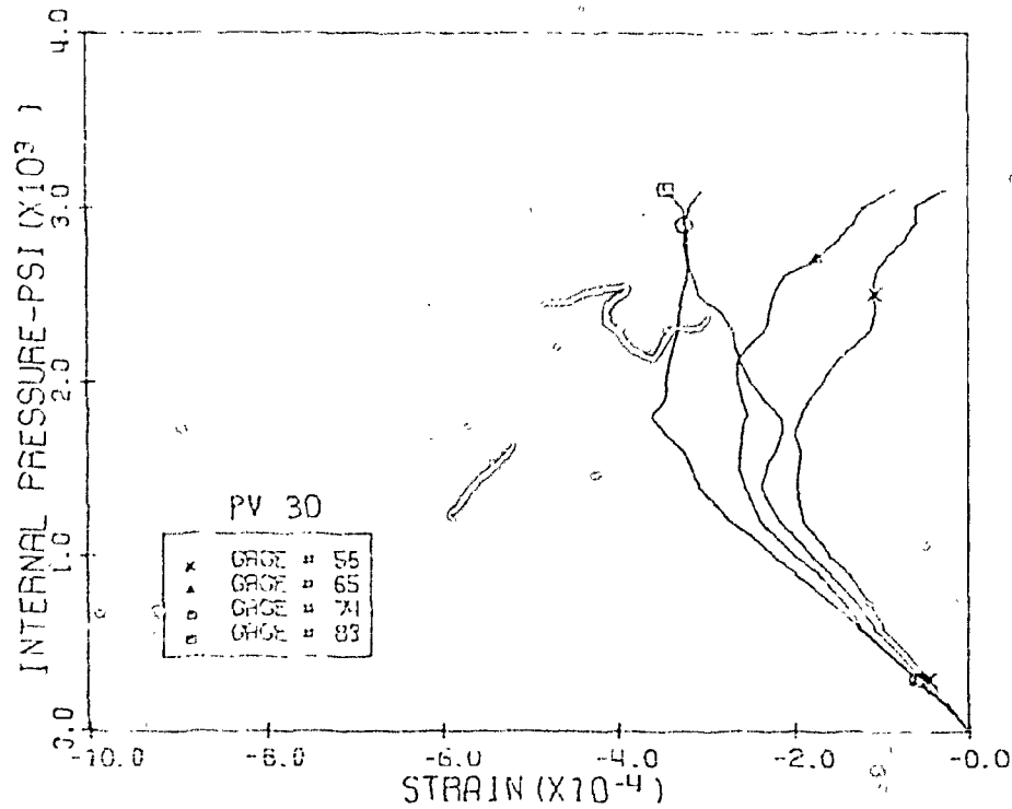
Fig. 3.35 Measured Horizontal Strains, Level 1, Pen. 4 & 5, PV30
