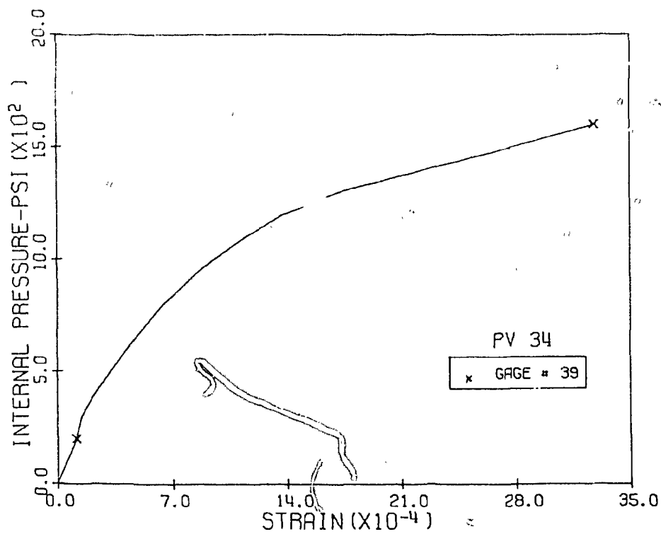
Fig. 3.70 Measured Tens. Diag. Strains, Level 1, Pen. 1 & 3, PV34
