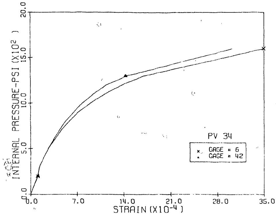
Fig. 3.73 Measured Comp. Diag. Strains, Level 2, Pen. 1 & 3 PV34
