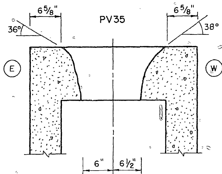
Fig. 3.11 End Slab After Test PV35
