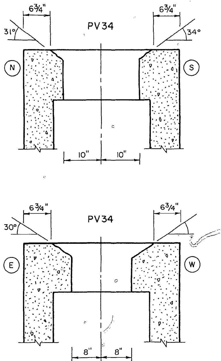
Fig. 3.8b End Slab After Test PV34
