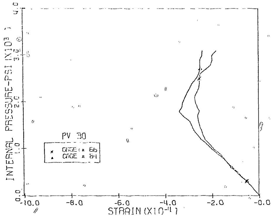
Fig. 3.37 Measured Tens. Diag. Strains, Level 1, Pen. 4 & 5, PV30
