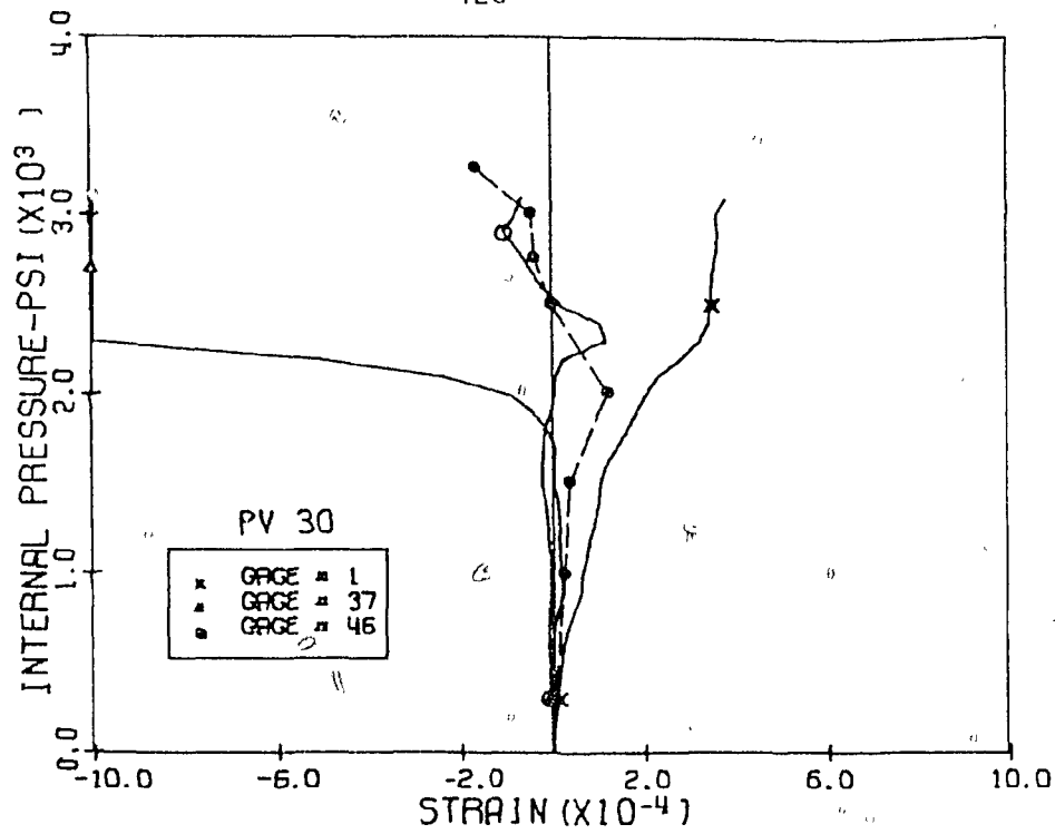
Fig. 5.5 Measured and Calculated Vertical Strains, Level 1 Penetrations 1 and 3, PV30
