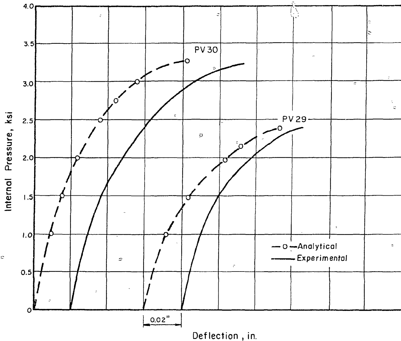
Fig. 5.35 Measured and Calculated Deflections at the Center of the End Slab for the Vessels with 2-in. Penetrations
