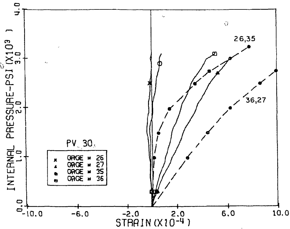
Fig. 5.21 Measured and Calculated Horizontal and Diagonal Strains Level 3 Penetration 2, PV30
