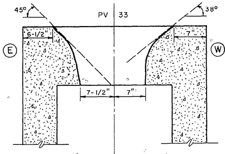
Fig. 3.10 End Slab after Test PV33
