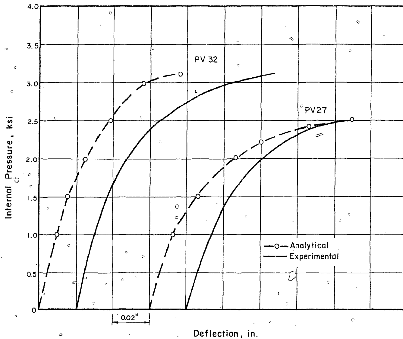
Fig. 5.34 Measured and Calculated Deflections at the Center of the End Slab for the Vessels with 5-in. Penetrations
