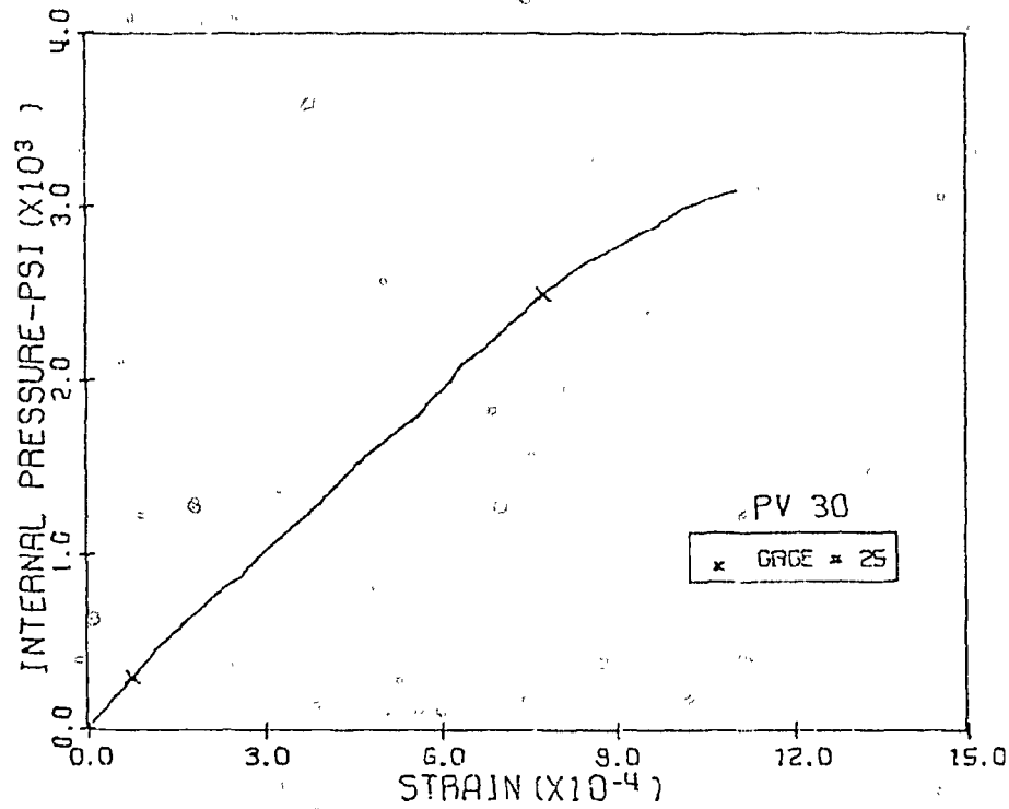
Fig. 3.32 Measured Vertical Strains, Level 3, Penetration 2, PV30
