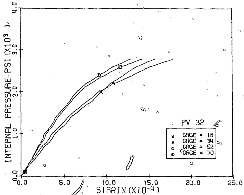
Fig. 3.61 Measured Vertical Strains, Level 3, 3:00 & 9:00 Pos., PV32
