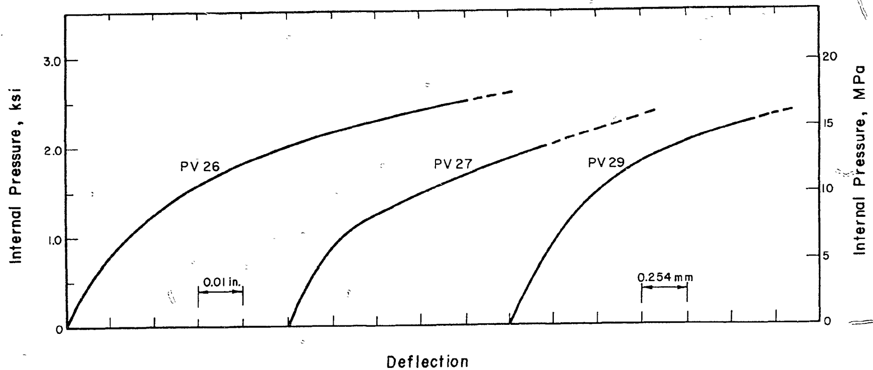
Fig. 3.1 Measured Relationships Between Internal Pressure and Total Deflection at Midspan of End Slab for Test Vessels with 10-in. End Slabs
