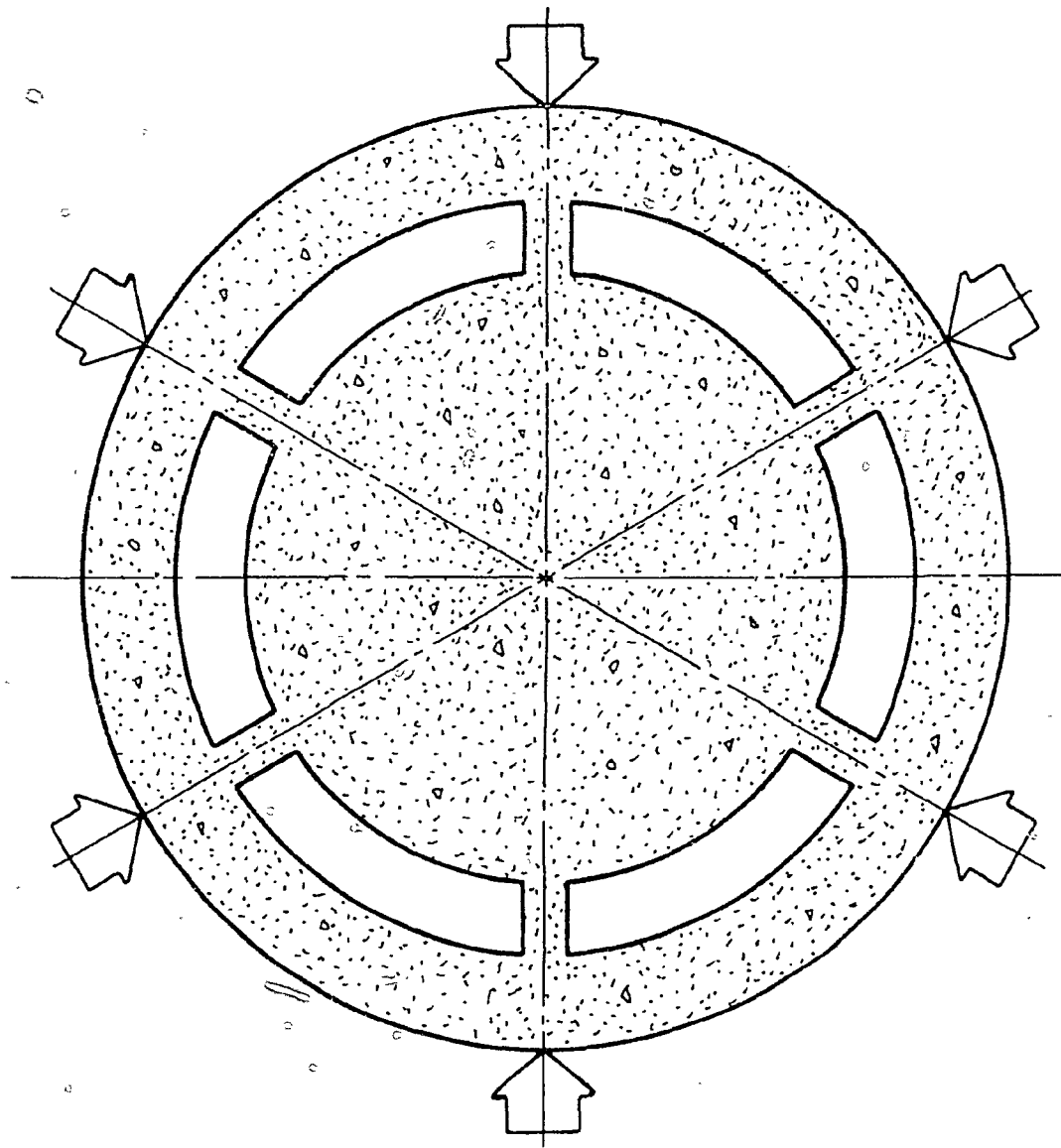
Fig. 3.14 Idealized Model for Perforated End Slabs
