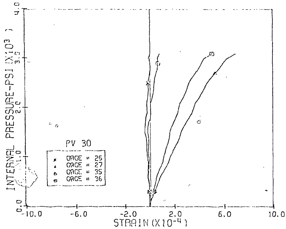
Fig. 3.33 Measured B6 Level 3, Penetration 2, PV30
