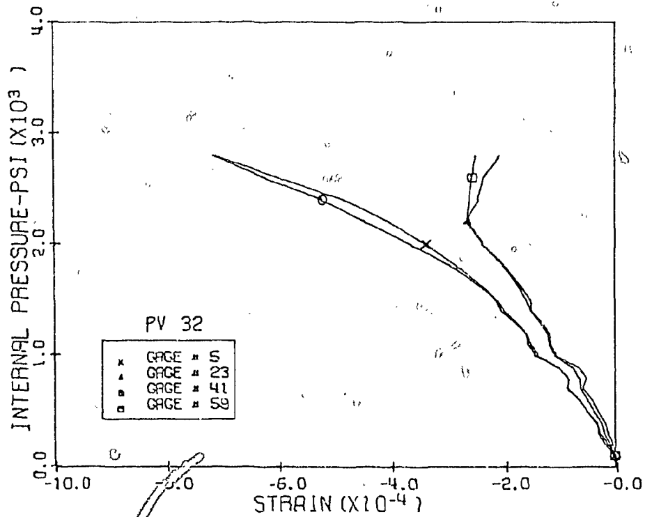
Fig. 3.55 Measured Horizontal Strains, Level 2, 12:00 & 6:00 Pos., PV32
