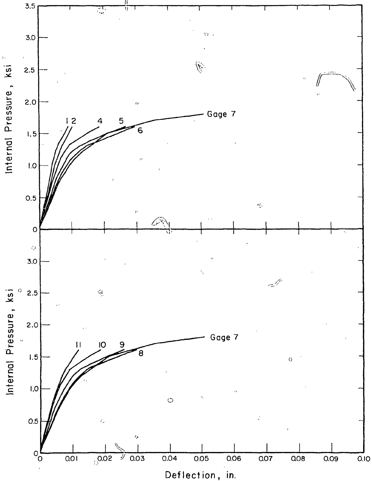
Fig. A.33 Measured Pressure-Deflection Curves, End Slab, PV34 (See Fig. A.26 for Gage Locations)
