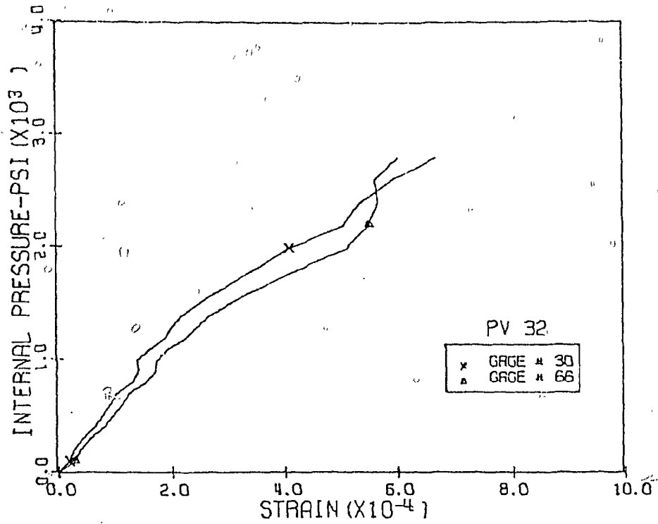
Fig. 3.52 Measured Comp. Diag. Strains, Level 1, 9:00 Pos., PV32
