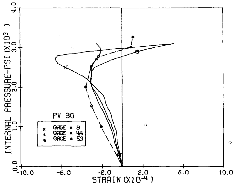
Fig. 5.14 Measured and Calculated Horizontal Strains, Level 3 Penetrations 1 and 3, PV30
