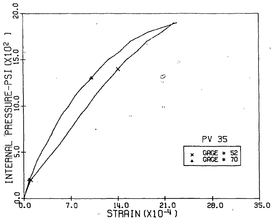
Fig. 3.113 Measured Vertical Strains, Level 3, 3:00 & 9:00 Pos., PV35
