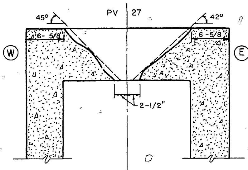
Fig. 3.4 End Slab after Test, PV27
