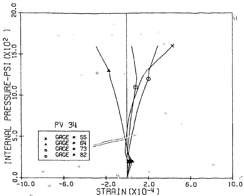
Fig. 3.84 Measured Vertical Strains, Level 1, Pen. 4 & 5, PV34
