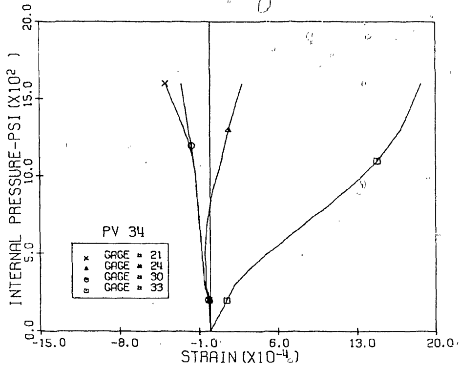
Fig. 3.81 Measured Diagonal Strains, Level 1 & 2, Penetration 2, PV34
