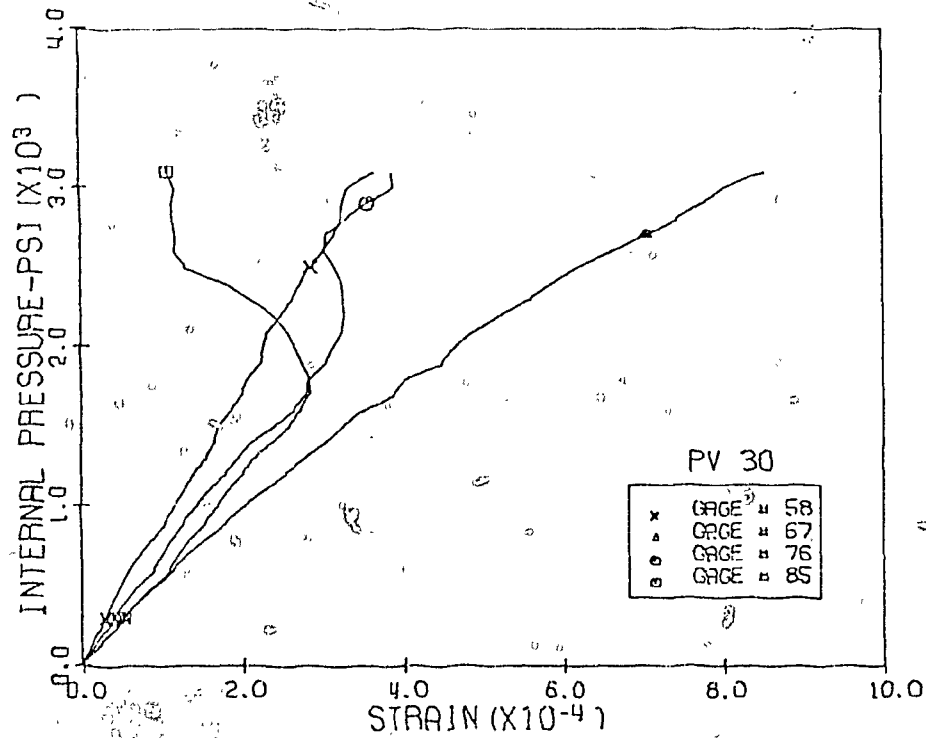
Fig. 3.38 Measured Vertical Strains, Level 2, Pen. 4 & 5, PV30
