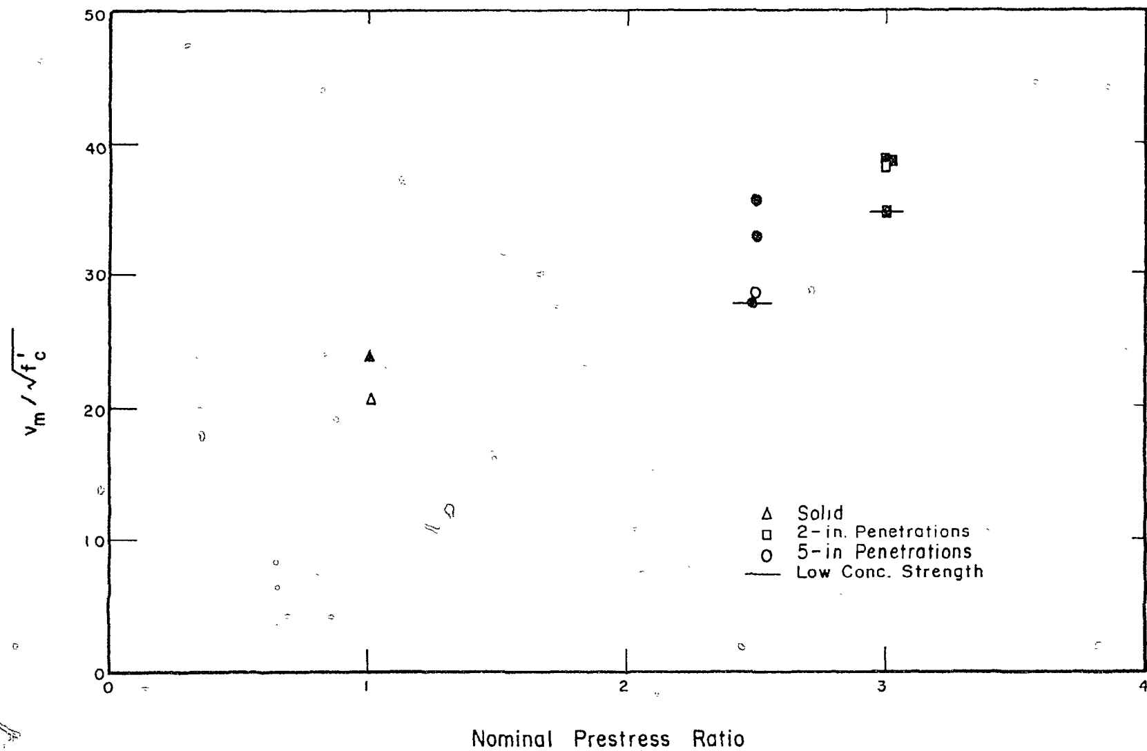
Fig. 3.13 Variation of Unit Nominal Shear Stress (Normalized) with a parameter Reflecting the Effect of Circumferential Prestress
