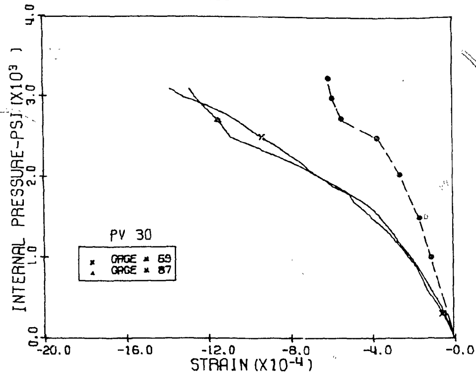
Fig. 5.29 Measured and Calculated Tension Diagonal Strains, Level 2 Penetrations 4 and 5, PV30
