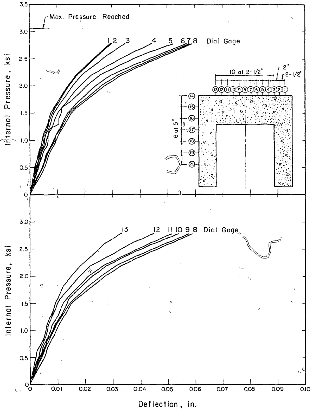
Fig. A.28 Measured Pressure-Deflection Curves End Slab, Test PV32
