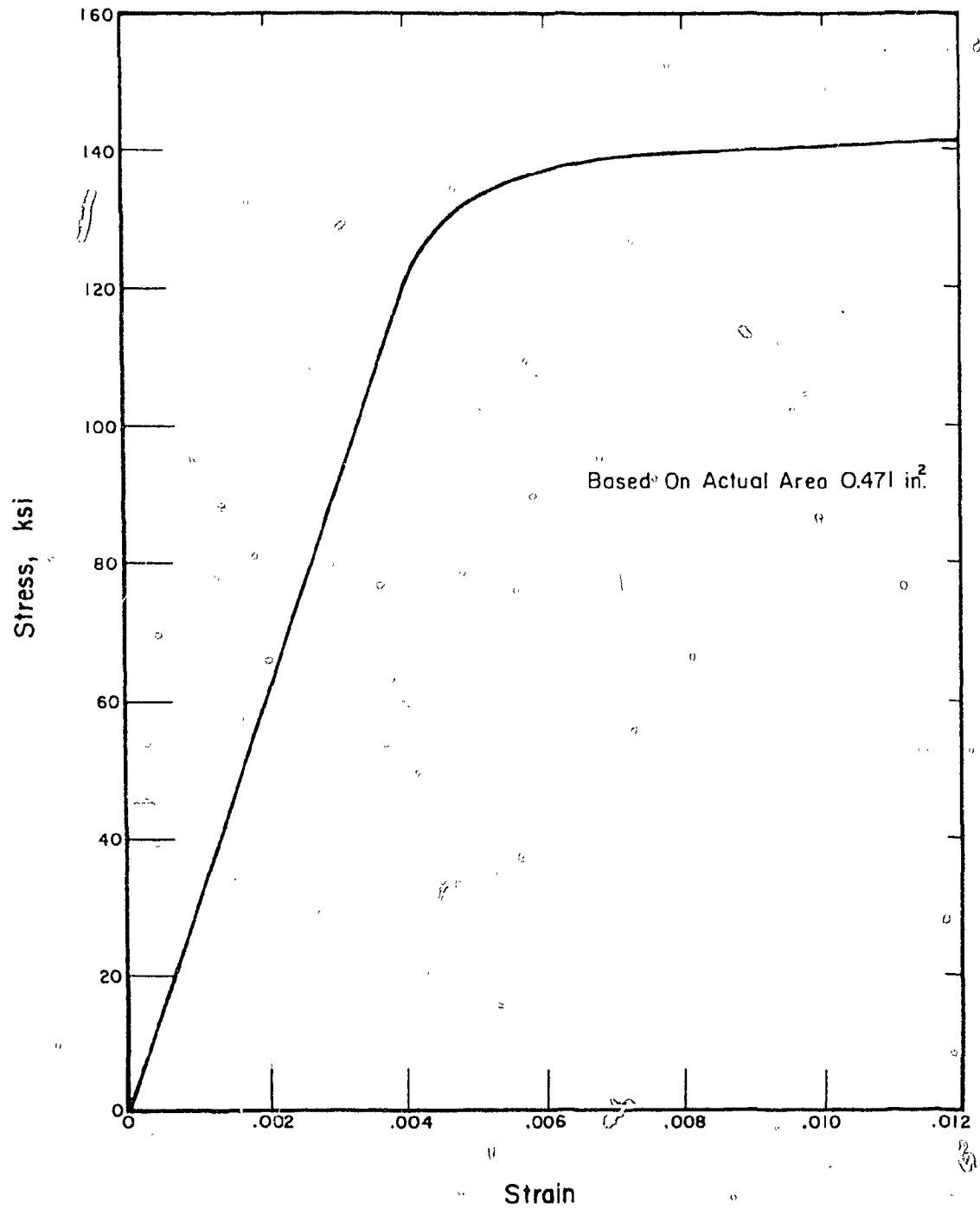
Fig. A.1 Stress-Strain Curve for Stressteel Rods
