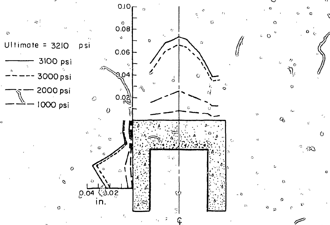
Fig. A.24 Measured Pressure-Deflection Curves Side Wall, Test PV30
