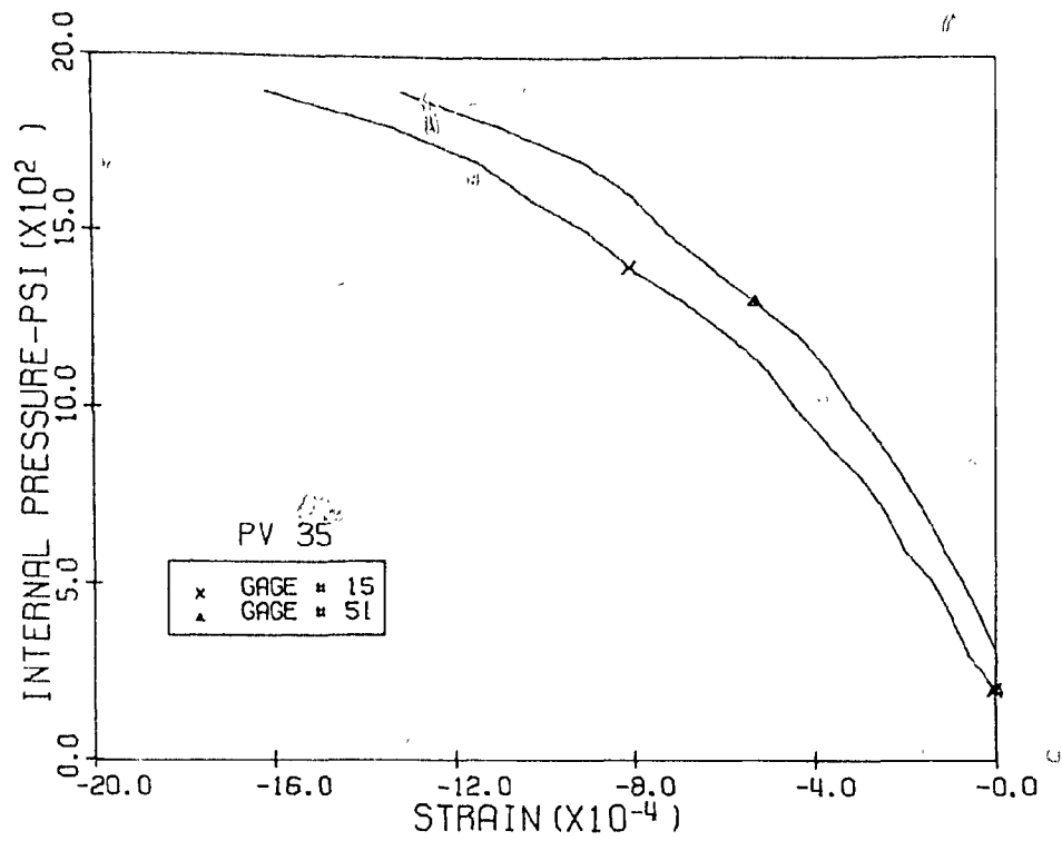
Fig. 3.108 Measured Tens. Diag. Strains, Level 2, 3:00 Pos., PV35
