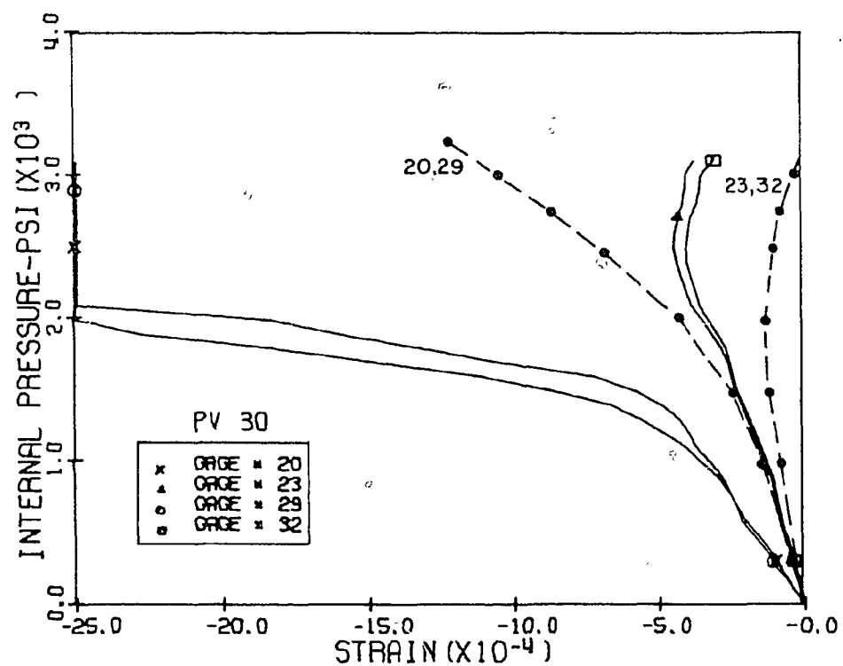
Fig. 5.18 Measured and Calculated Horizontal Strains, Levels 1 and 2 Penetration 2, PV30
