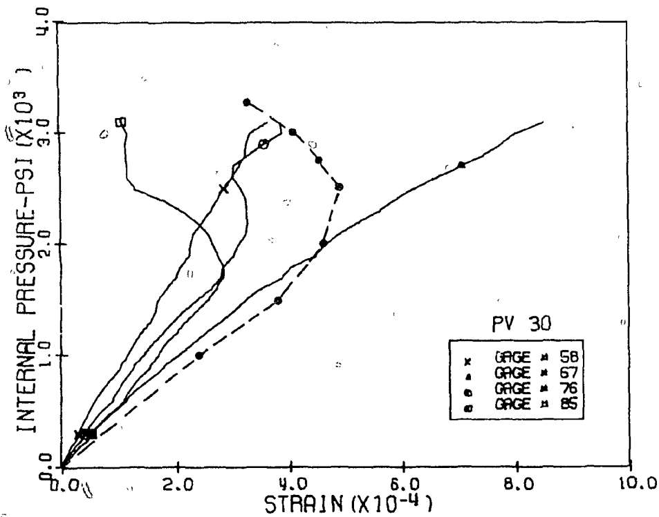
Fig. 5.26 Measured and Calculated Vertical Strains, Level 2 Penetrations 4 and 5, PV30
