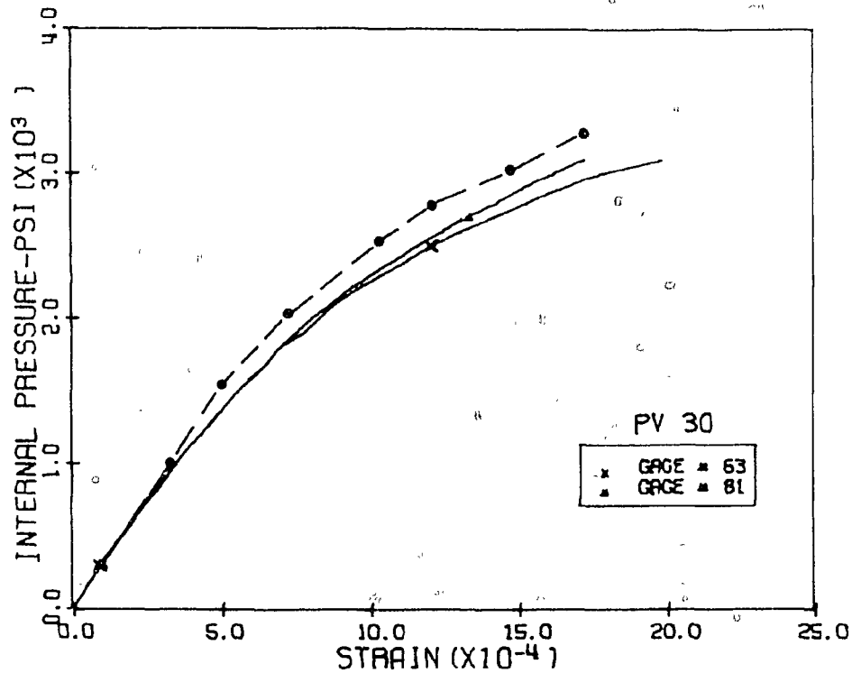
Fig. 5.32 Measured and Calculated Compression Diagonal Strains, Level 3 Penetrations 4 and 5, PV30
