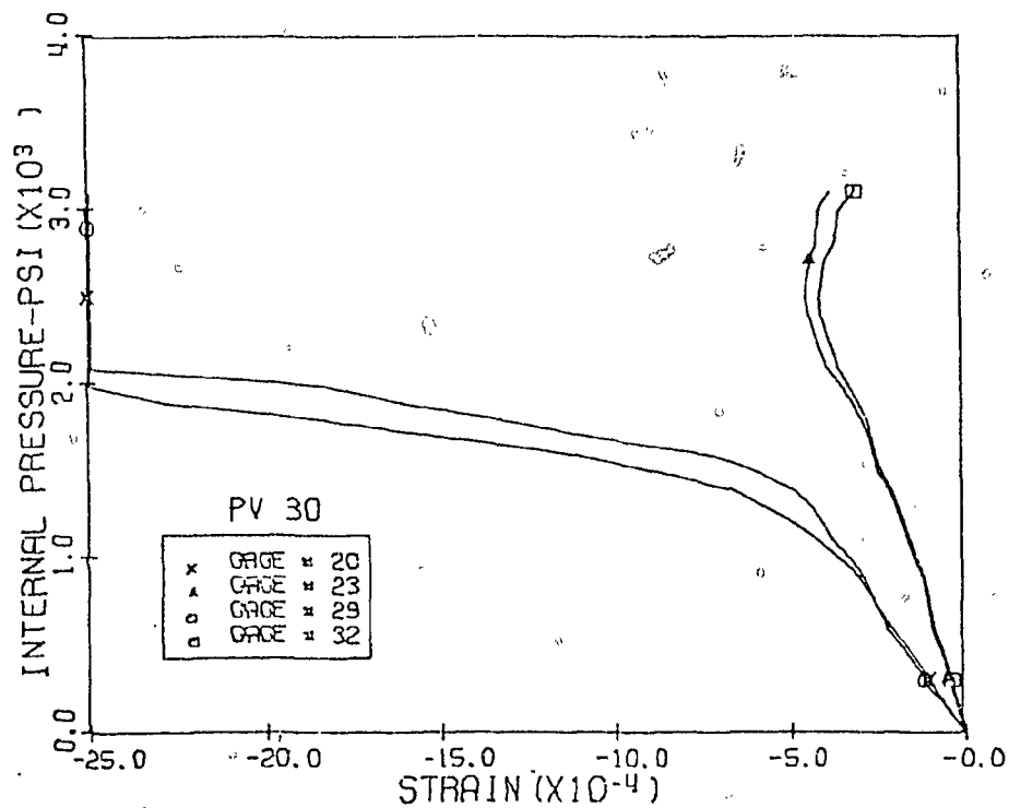
Fig. 3.30 Measured Horizontal Strains, Level 1 & 2, Penetration 2, PV30
