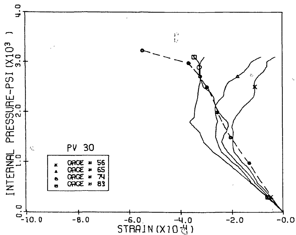
Fig. 5.23 Measured and Calculated Horizontal Strains, Level 1 Penetrations 4 and 5, PV30
