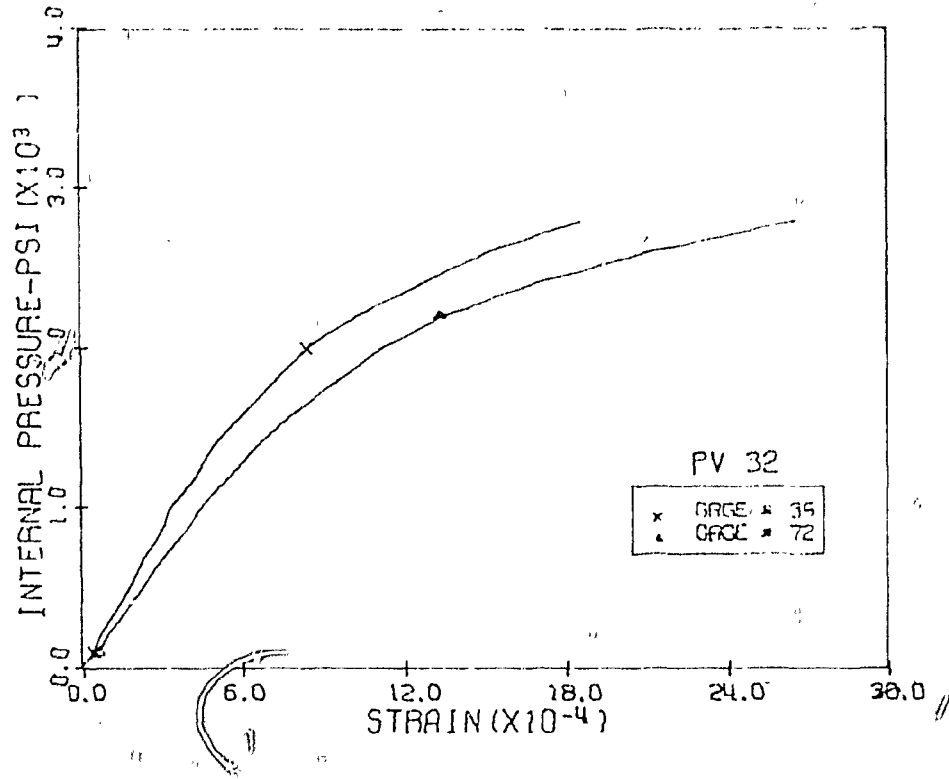
Fig. 3.66 Measured Comp. Diag. Strains, Level 3, 9:00 Pos., PV32
