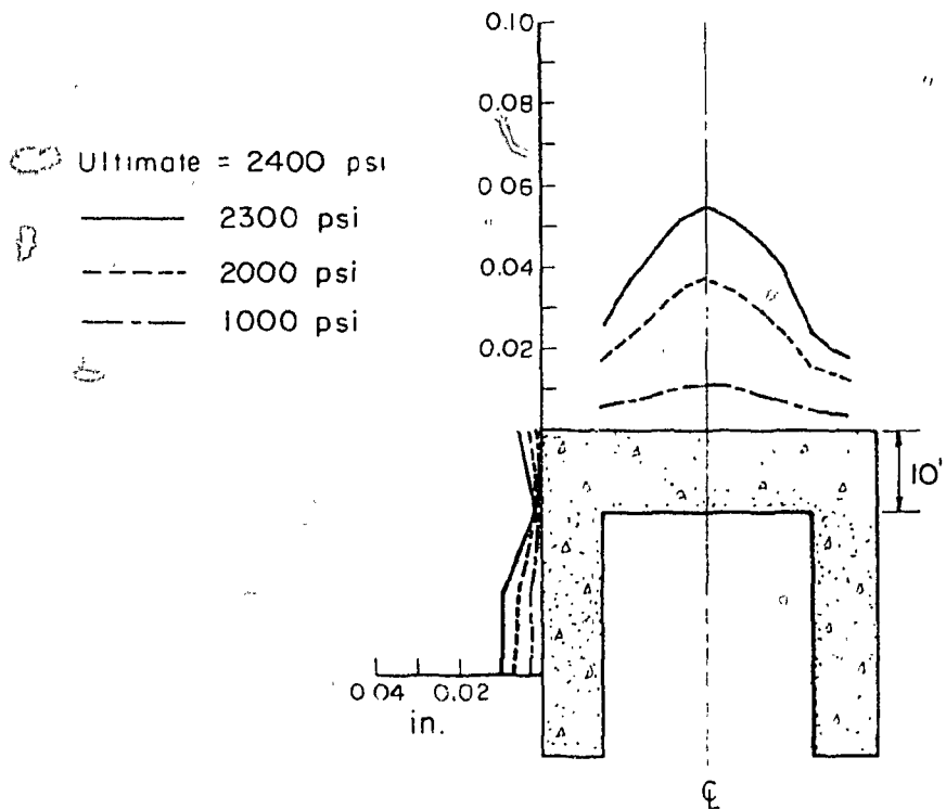
Fig. A.19 Measured Pressure-Deflection Curves Side Wall, Test PV29
