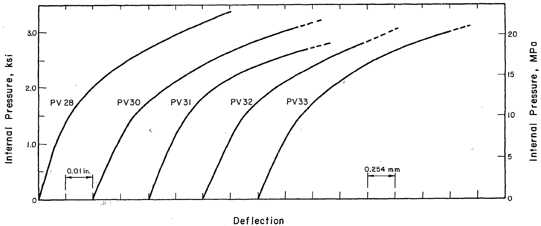
Fig. 3.2 Measured Relationships Between Internal Pressure and Total Deflection at Midspan of End Slab for Test Vessels with 12.5 in. End Slabs
