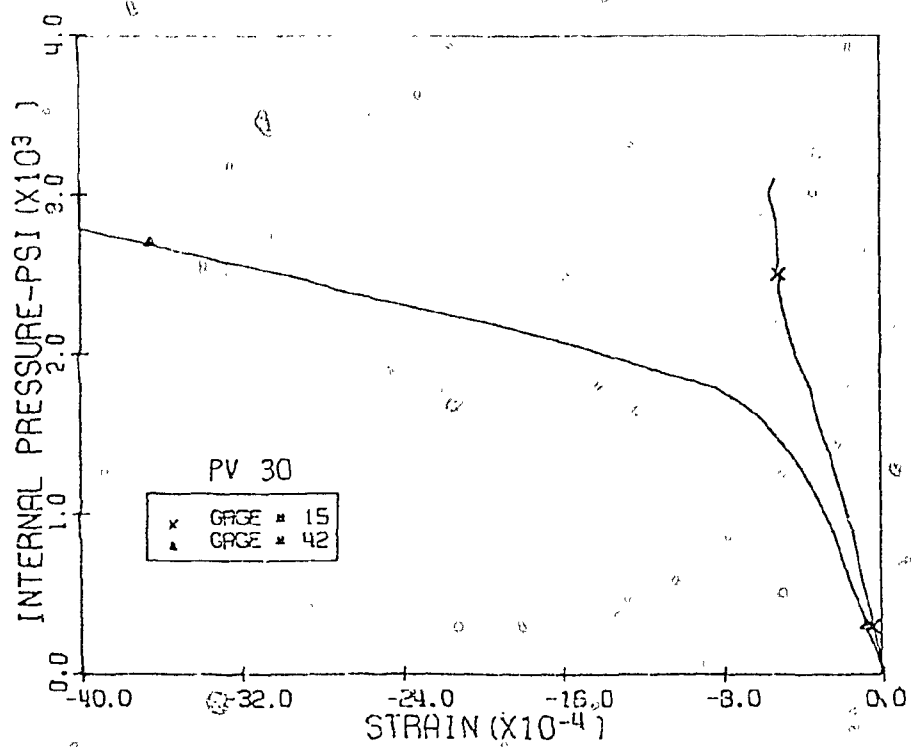
Fig. 3.24 Measured Tens. Diag. Strains, Level 2, Pen. 1 & 3, PV30
