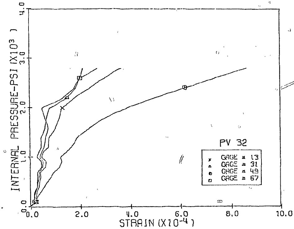
Fig. 3.54 Measured Vertical Strains, Level 2, 3:00 & 9:00 Pos., PV32
