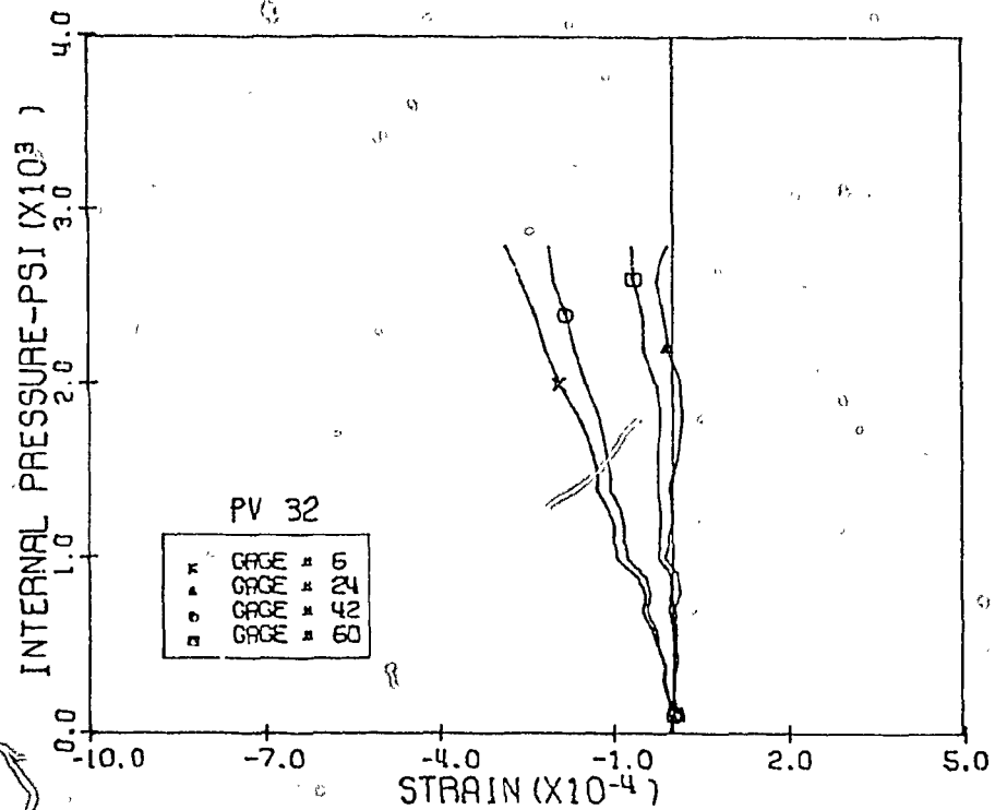
Fig. 3.57 Measured Diagonal Strains, Level 2, 12:00 & 6:00 P.m., PV32
