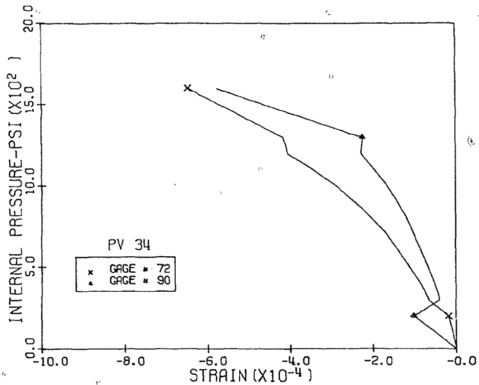
Fig. 3.95 Measured Tens. Diag. Strains, Level 3, Pen. 4 & 5, PV34
