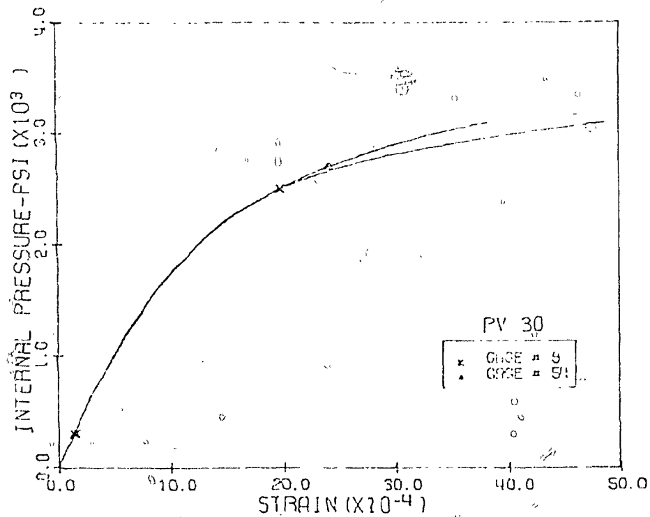
Fig. 3.27 Measured Comp. Diag. Strains, Level 3, Pen. 1 & 3, PV30
