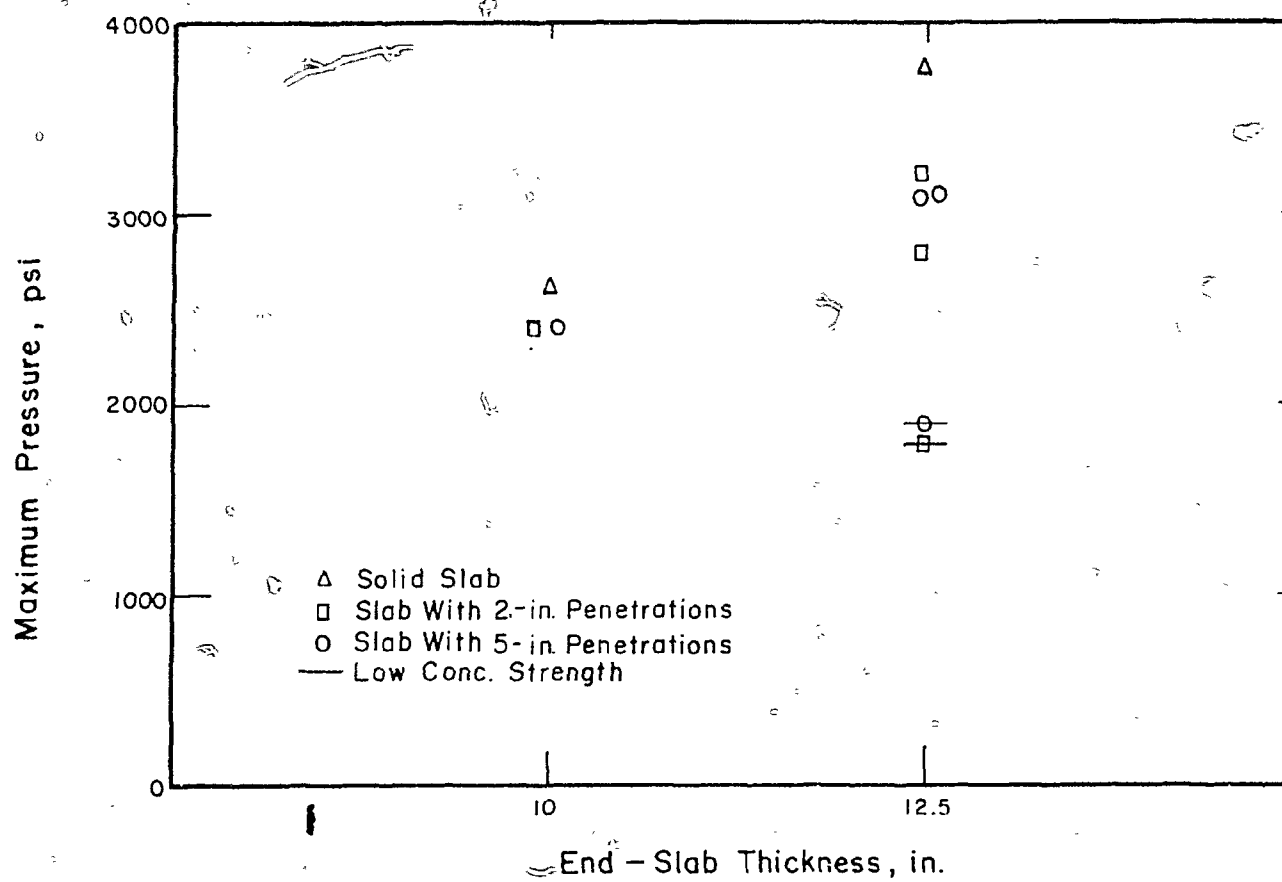
Fig. 3.12 Measured Maximum Internal Pressures
