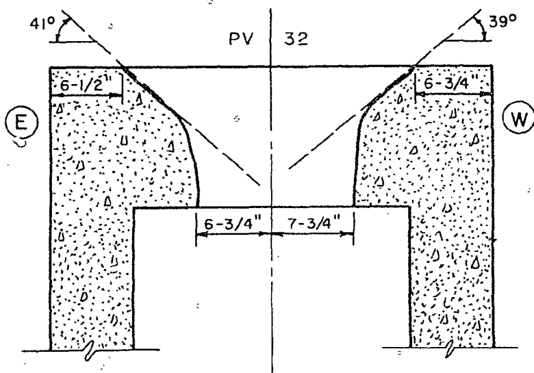
Fig. 3.9 End Slab after Test PV32
