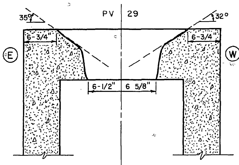
Fig. 3.5 End Slab after Test PV29
