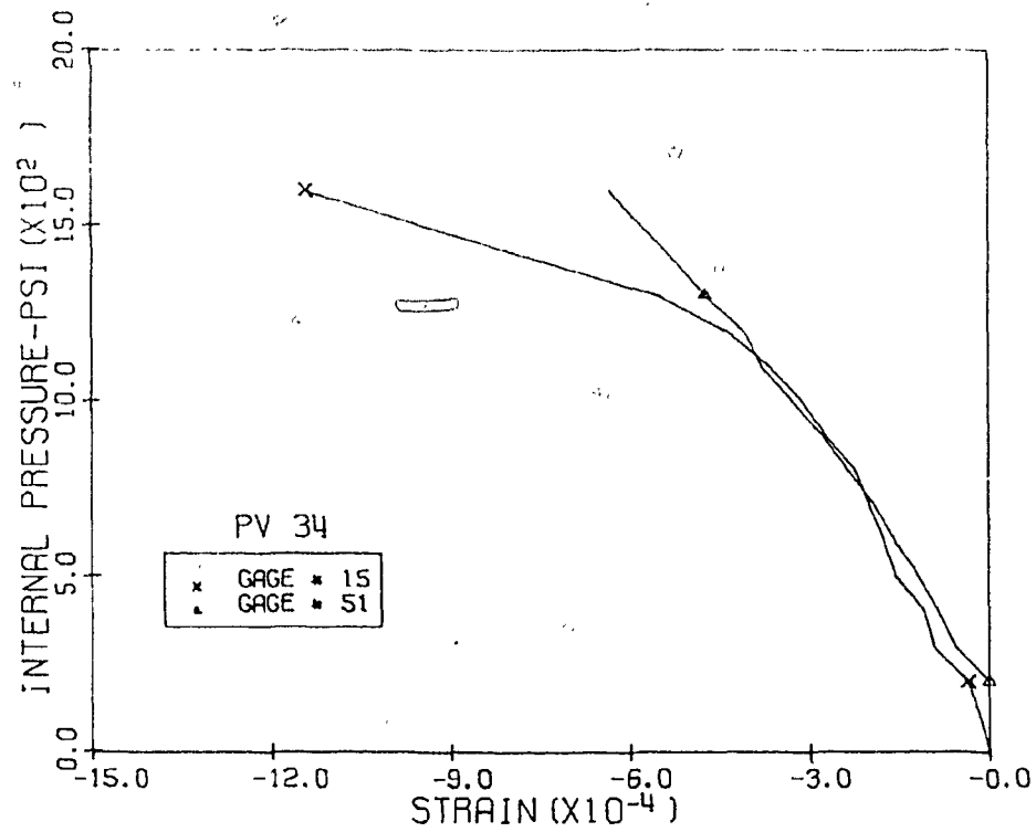
Fig. 3.74 Measured Tens. Diag. Strains, Level 2, Pen. 1 & 3, PV34
