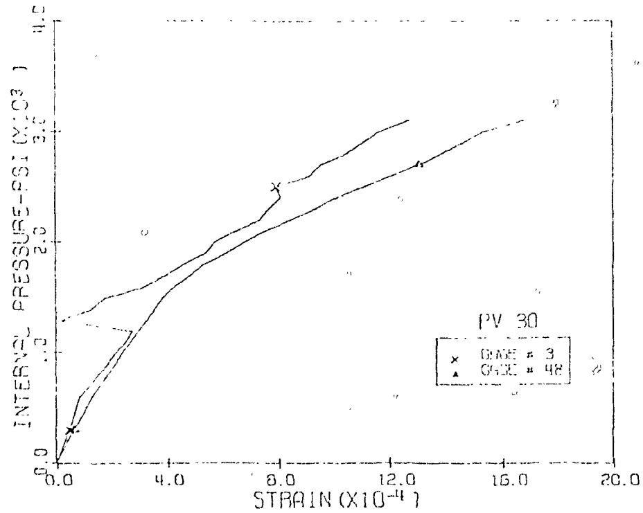
Fig. 3.19 Measured Comp. Diag. Strains, Level 1, Pen. 1 & 3, PV30
