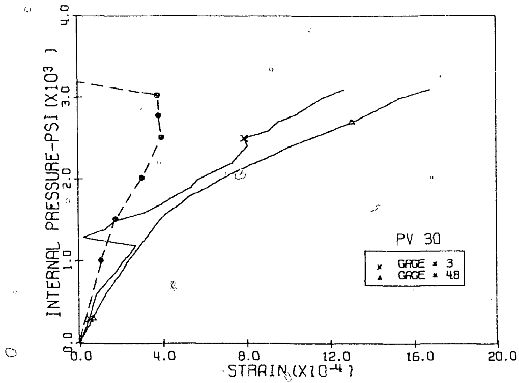
Fig. 5.7 Measured and Calculated Compression Diagonal Strains, Level 1 Penetrations 1 and 3, PV30
