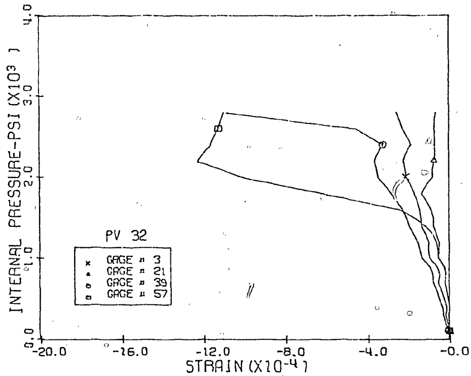
Fig. 3.50 Measured Diagonal Strains, Level 1, 12:00 & 6:00 Pos., PV32
