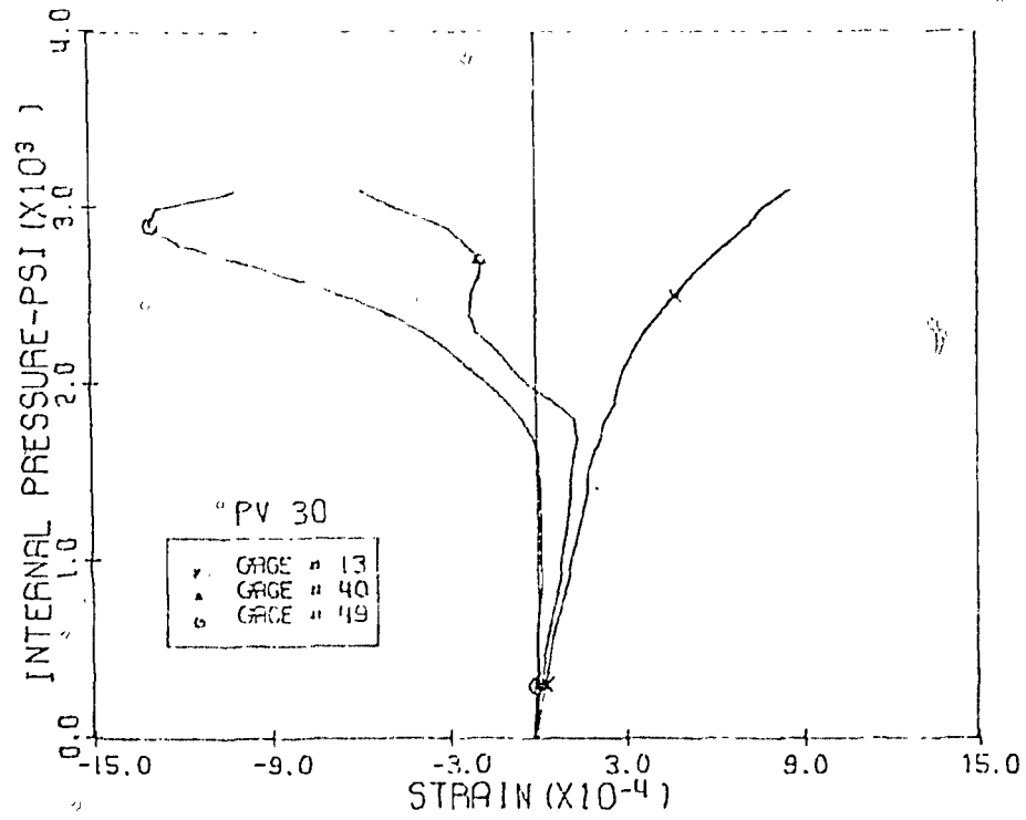
Fig. 3.21 Measured Vertical Strains, Level 2, Pen. 1 & 3, PV30
