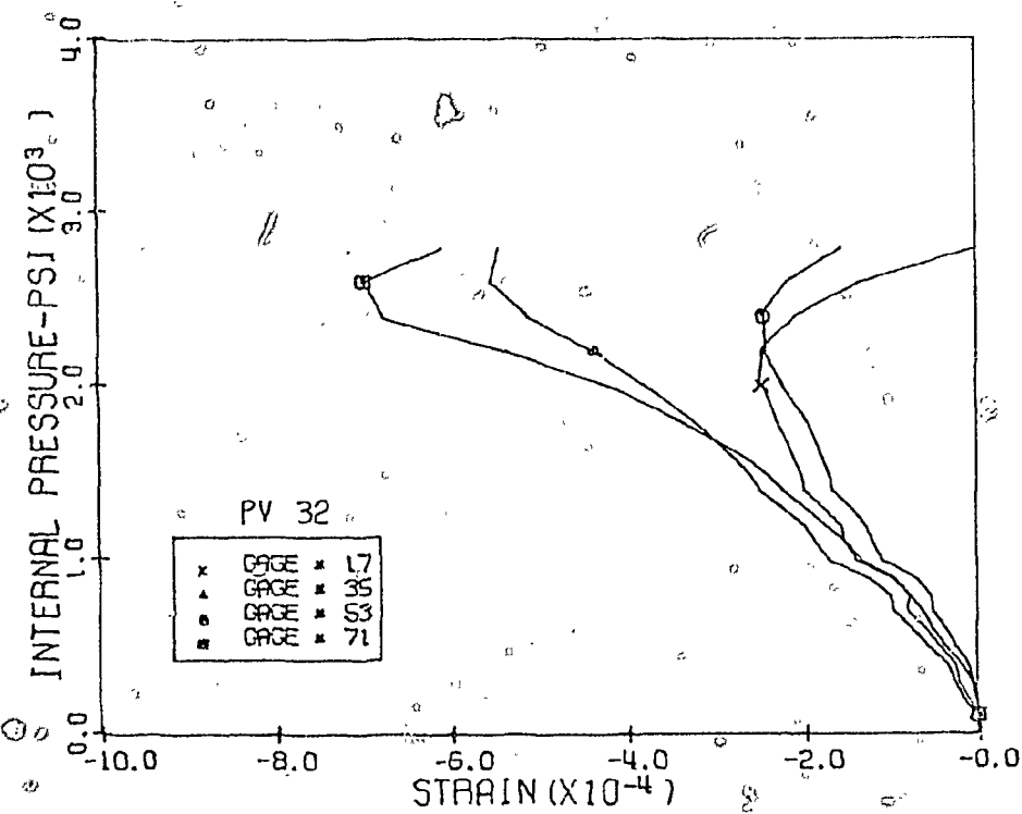
Fig. 3.63 Measured Horizontal Strains, Level 3, 3:00 & 9:00 Pos., PV32
