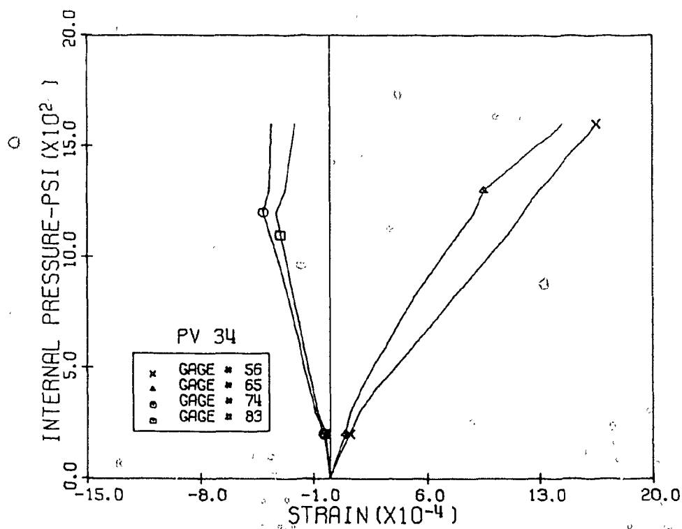
Fig. 3.85 Measured Horizontal Strains, Level 1, Pen. 4 & 5, PV34
