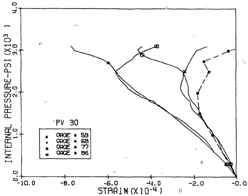
Fig. 5.27 Measured and Calculated Horizontal Strains, Level 2 Penetrations 4 and 5, PV30
