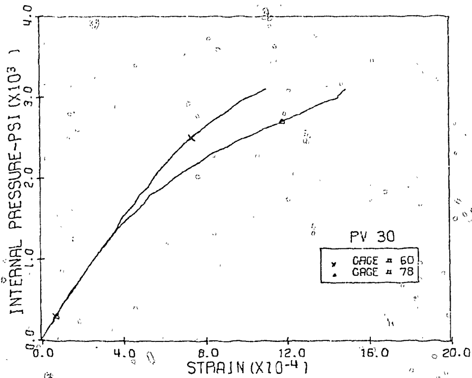
Fig. 3.40 Measured Comp. Diag. Strains, Level 2, Pen. 4 & 5, PV30
