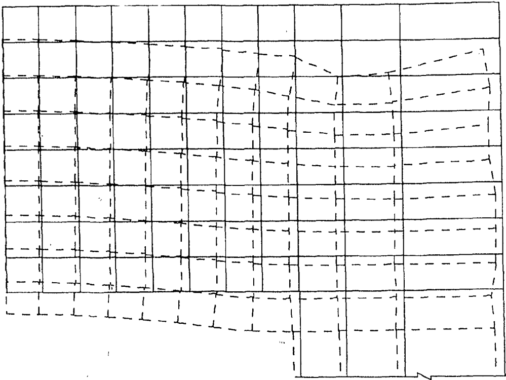
Fig. 5.2c Deflected Shape of End Slab at 1500 psi Internal Pressure
