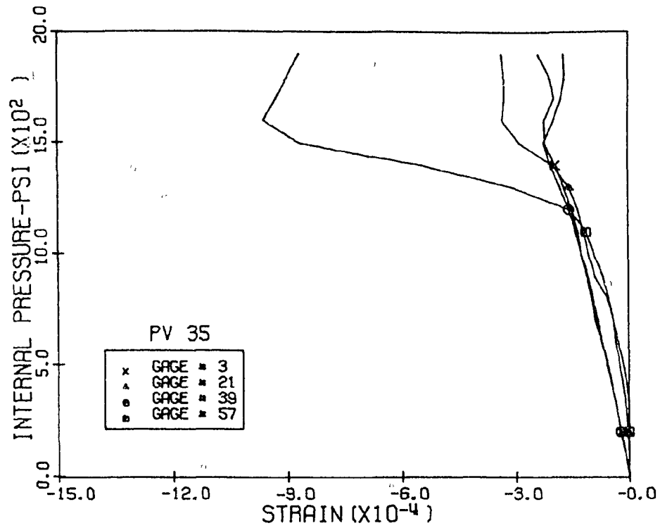
Fig. 3.100 Measured Tens. Diag. Strains, Level 1, 12:00 & 6:00 Pos., PV35
