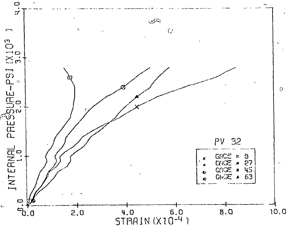
Fig. 3.64 Measured Diagonal Strains, Level 3, 12:00 & 6:00 Pos., PV32
