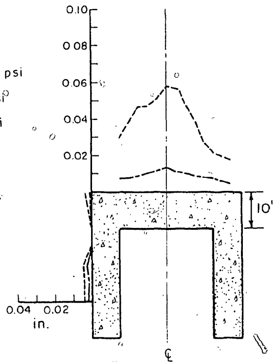
Fig. A.17 Measured Pressure-Deflection Curves Side Wall, Test PV27
