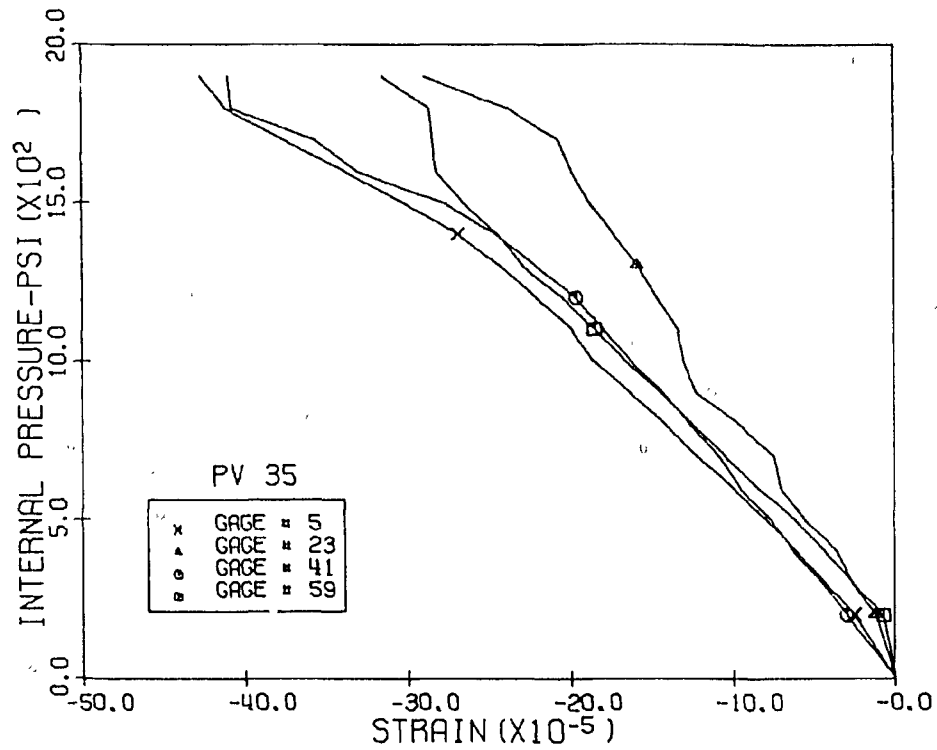
Fig. 3.103 Measured Horizontal Strains, Level 2, 12:00 & 6:00 Pos., PV35
