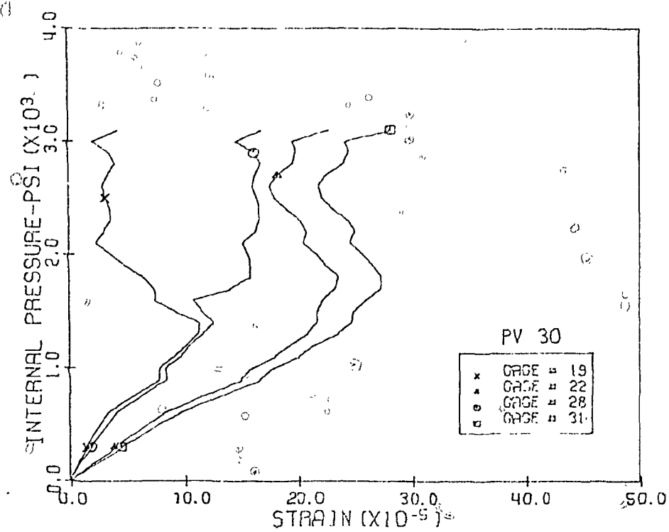
Fig. 3.29 Measured Vertical Strains, Level 1 & 2, Penetration 2, PV30
