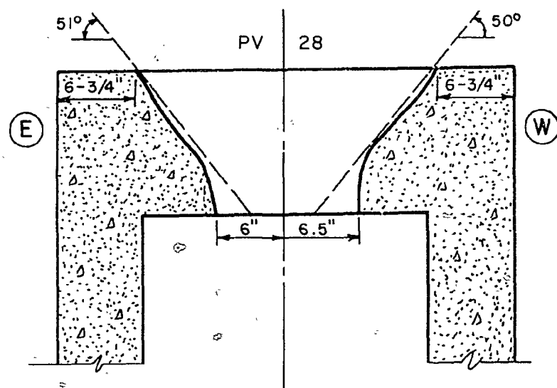
Fig. 3.6 End Slab after Test PV28
