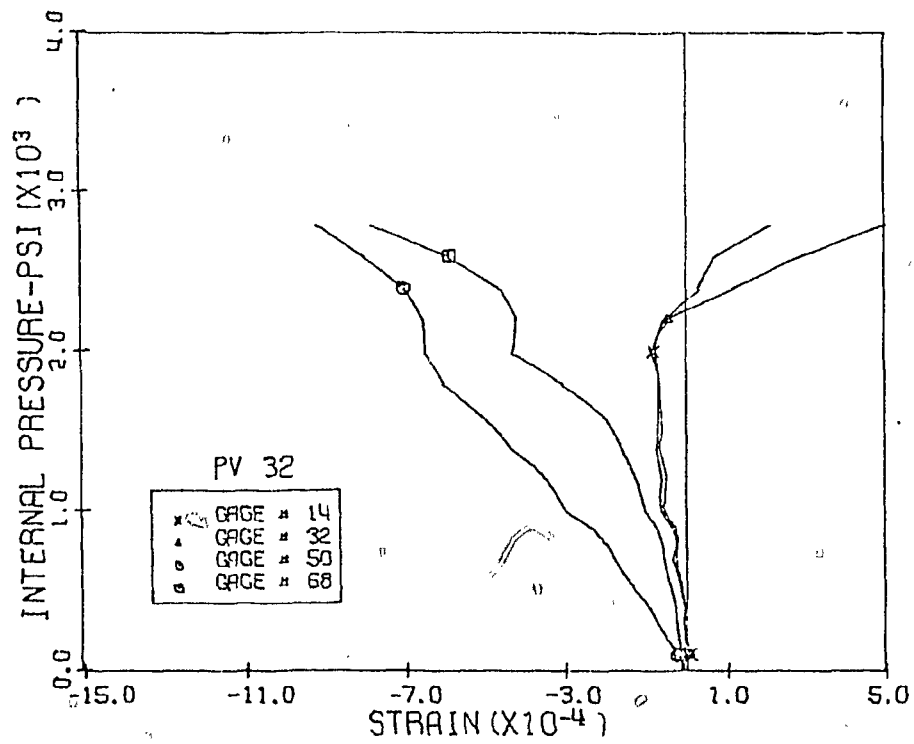
Fig. 3.56 Measured Horizontal Strains, Level 2, 3:00 & 9:00 P.m., PV32
