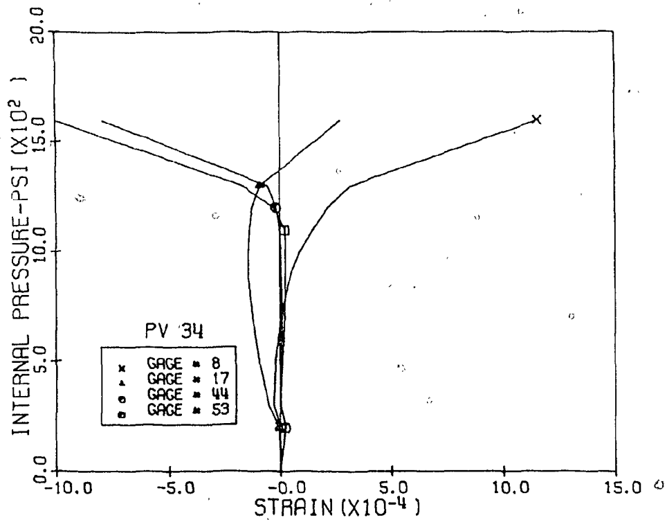
Fig. 3.76 Measured Horizontal Strains, Level 3, Pen. 1 & 3, PV34
