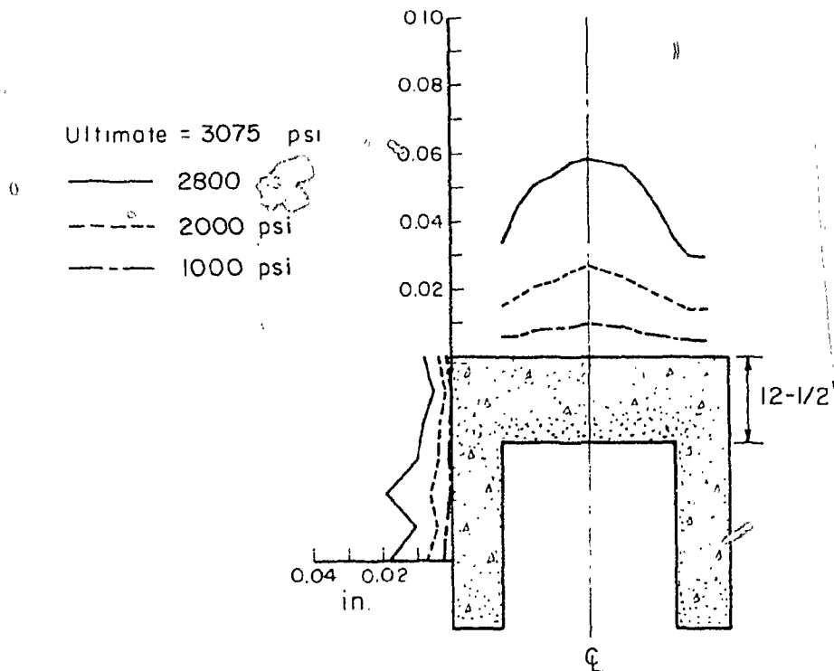
Fig. A.29 Measured Pressure-Deflection Curves Side Wall, Test PV32
