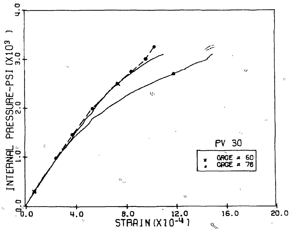
Fig. 5.28 Measured and Calculated Compression Diagonal Strains, Level 2 Penetrations 4 and 5, PV30
