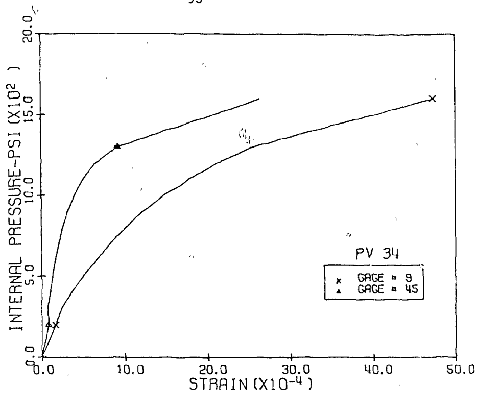
Fig. 3.77 Measured Comp. Diag. Strains, Level 3, Pen. 1 & 3, PV34
