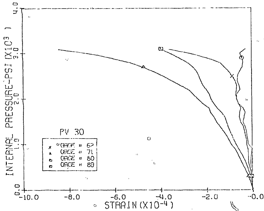
Fig. 3.43 Measured Horizontal Strains, Level 3, Pen. 4 & 5, PV30
