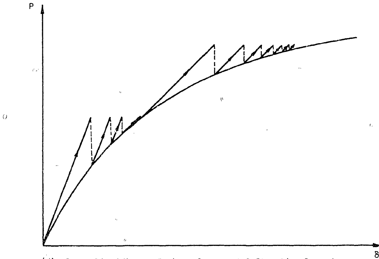
(a) Generalized Newton-Raphson Incremental-Iterative Procedure
