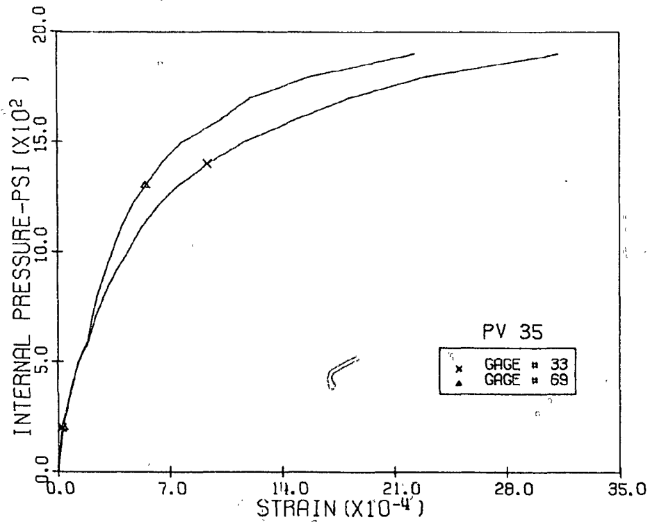
Fig. 3.109 Measured Comp. Diag. Strains, Level 2, 9:00 Pos., PV35
