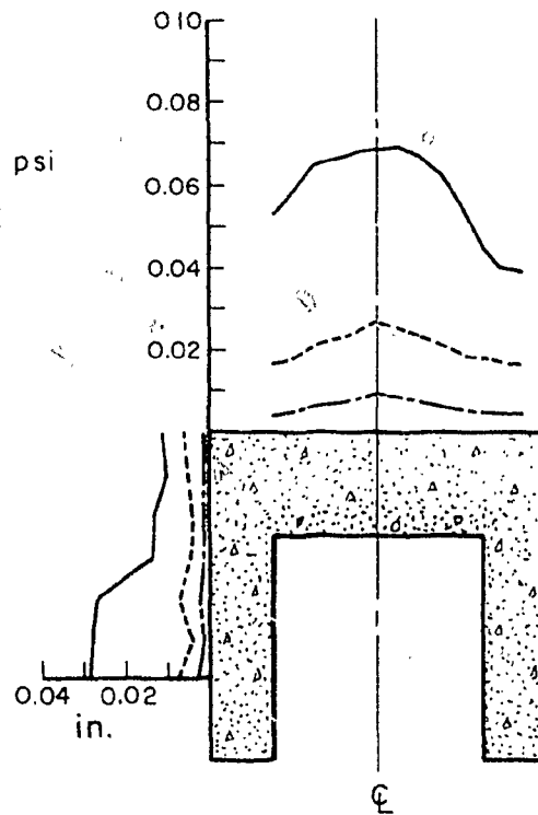
Fig. A.32 Measured Pressure-Deflection Curves Side Wall, Test PV33.2
