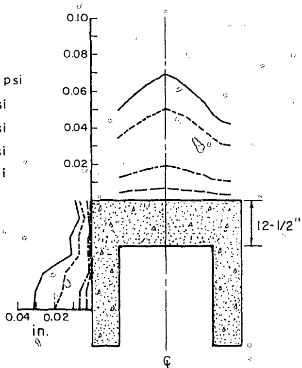
Fig. A.22 Measured Pressure-Deflection Curves Side Wall, Test PV28.2
