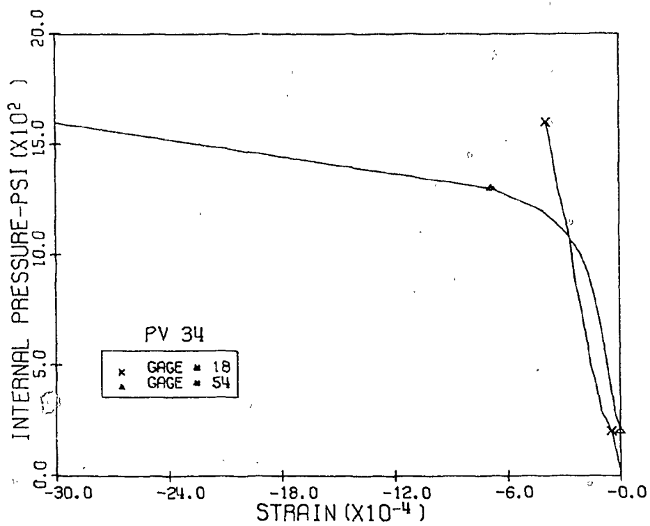
Fig. 3.78 Measured Tens. Diag. Strains, Level 3, Pen. 1 & 3, PV34
