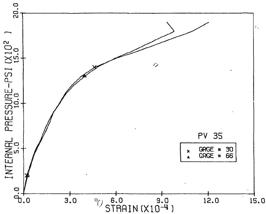
Fig. 3.102 Measured Tens. Diag. Strains, Level 1, 9:00 Pos., PV35
