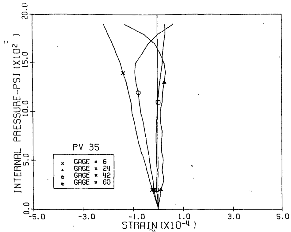
Fig. 3.107 Measured Diagonal Strains, Level 2, 12:00 & 6:00 Pos., PV35
