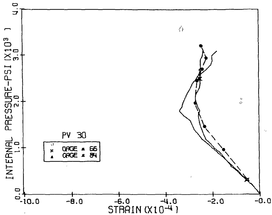
Fig. 5.25 Measured and Calculated Tension Diagonal Strains, Level 1 Penetrations 4 and 5, PV30
