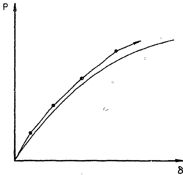
(b) Incremental Solution Procedure
