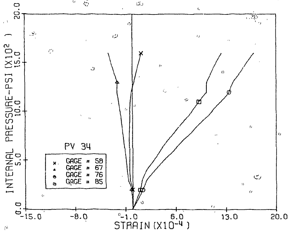
Fig. 3.88 Measured Vertical Strains, Level 2, Pen. 4 & 5, PV34
