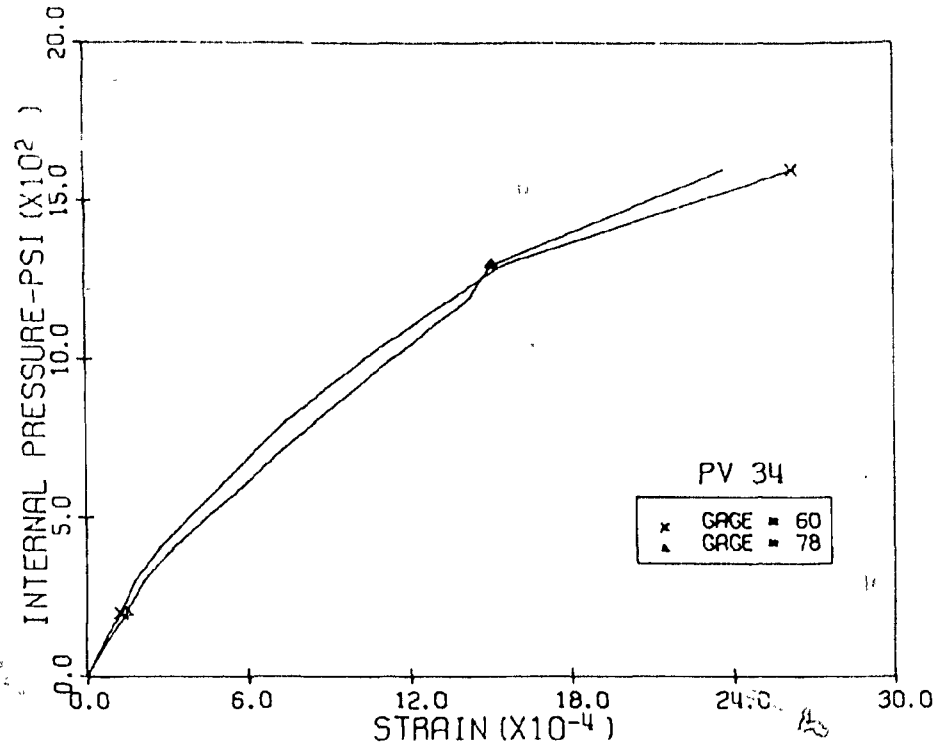
Fig. 3.90 Measured Comp. Diag. Strains, Level 2, Pen. 4 & 5, PV34
