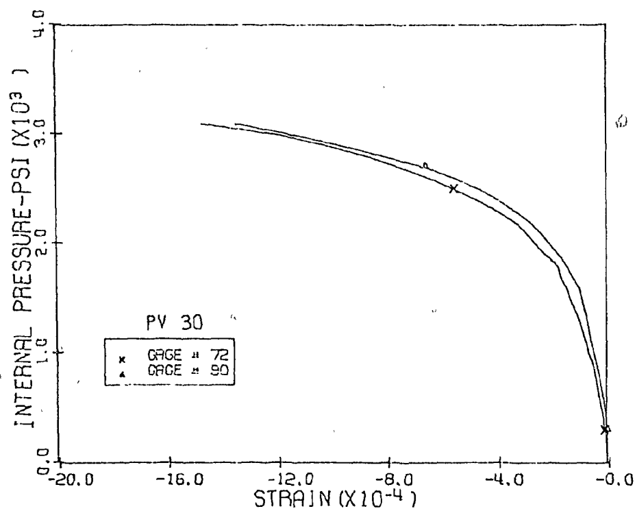
Fig. 3.45 Measured Tens. Diag. Strains, Level 3, Pen. 4 & 5, PV30
