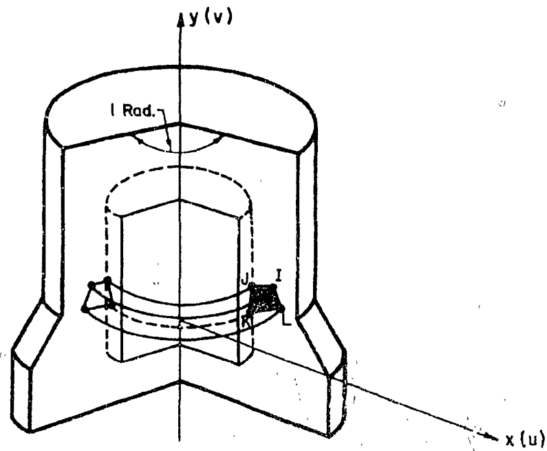
(a) Element of an Axisymmetric Solid
