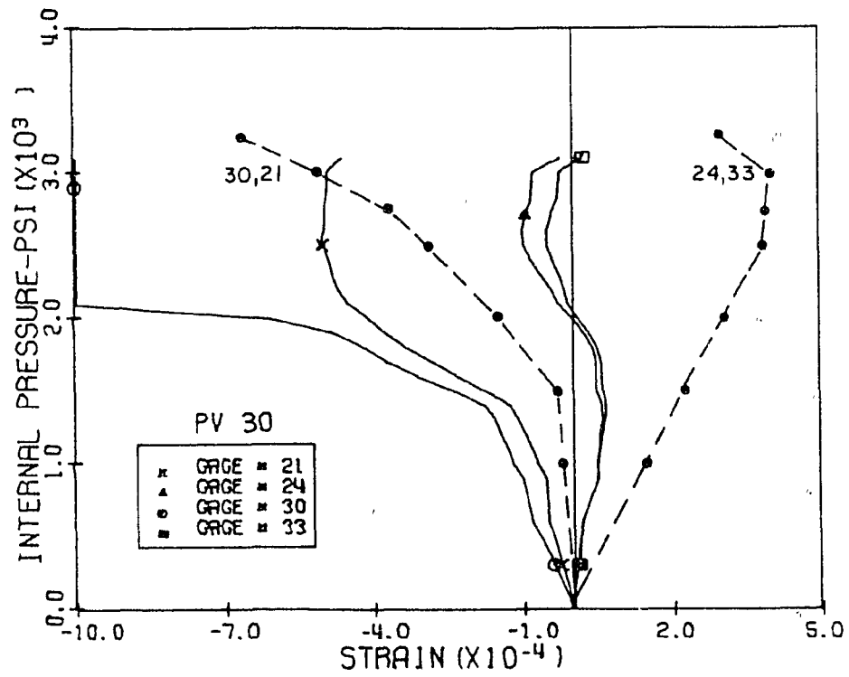
Fig. 5.19 Measured and Calculated Diagonal Strains, Levels 1 and 2 Penetration 2, PV30
