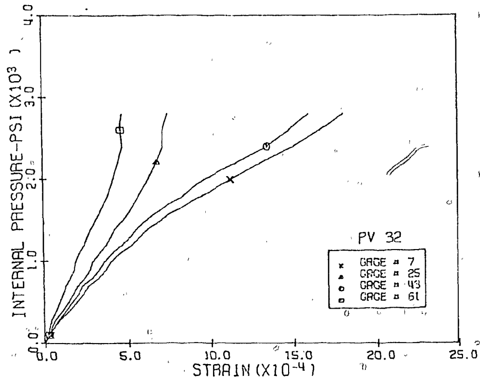
Fig. 3.60 Measured Vertical Strains, Level 3, 12:00 & 6:00 Pos., PV32
