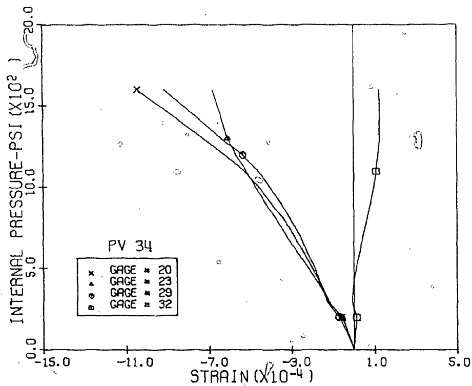
Fig. 3.80 Measured Horizontal Strains, Level 1 & 2, Penetration 2, PV34
