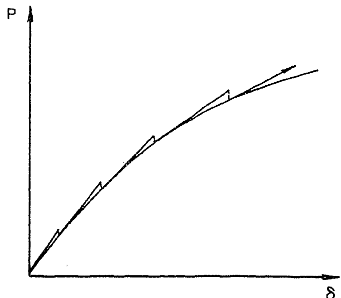
(c) Incremental Solution Procedure with Residual Load Corrections
