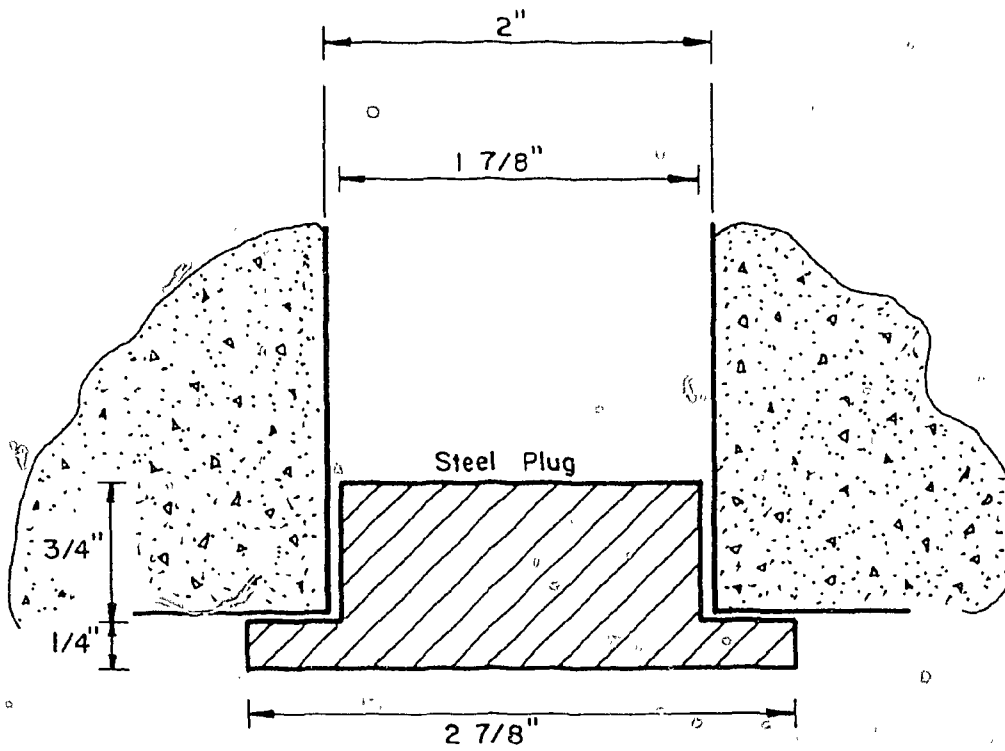
Fig. A.7 Steel Closure Plates
