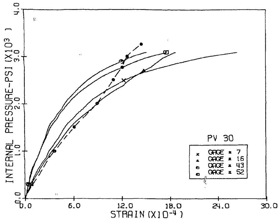
Fig. 5.13 Measured and Calculated Vertical Strains, Level 3 Penetrations 1 and 3, PV30
