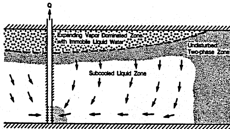
Figure 2. Schematic model of flow patterns and depletion mechanisms for a well with a deep feed zone (from Bodvarsson and Cox, 1986). XBL 866-10863
