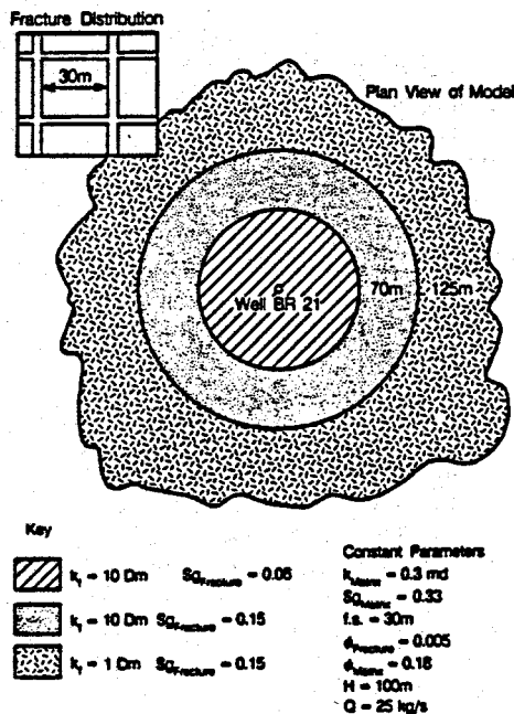
Fig. 1. Diagram of best fit model for the reservoir region near well BR-21, Ohaaki, New Zealand (from Gaulke and Bodvarsson, 1987). XBL 8612-12791
