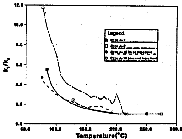
Fig. 10. Permeability enhancement plotted as a function of the sandface injection temperature for the four Los Azufres injection tests (from Benson et al., 1987).
