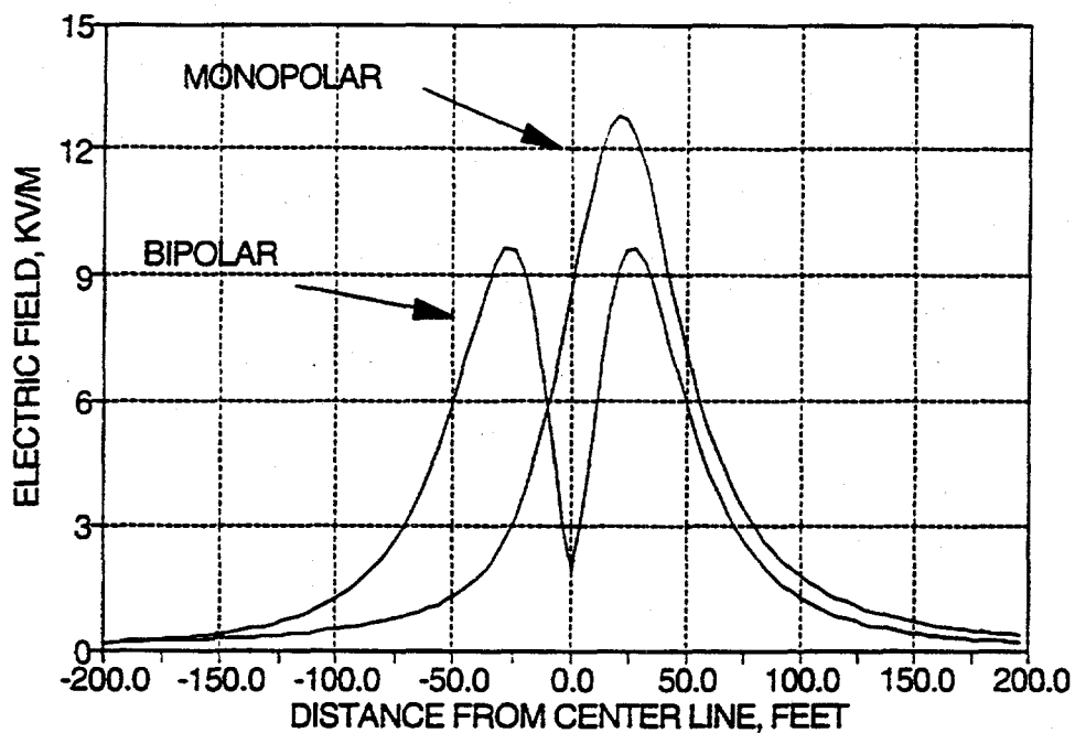
Figure 10.8 EF DC Line Monopolar and Bipolar Operation
