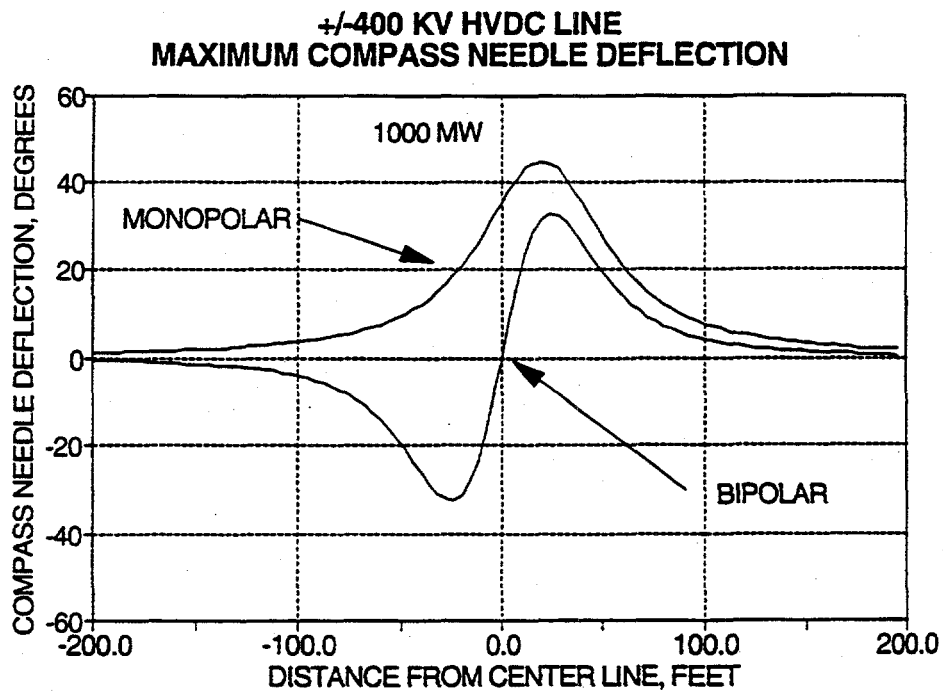
Figure 10.13 Compass Needle Deflection Monopolar and Bipolar Operation
