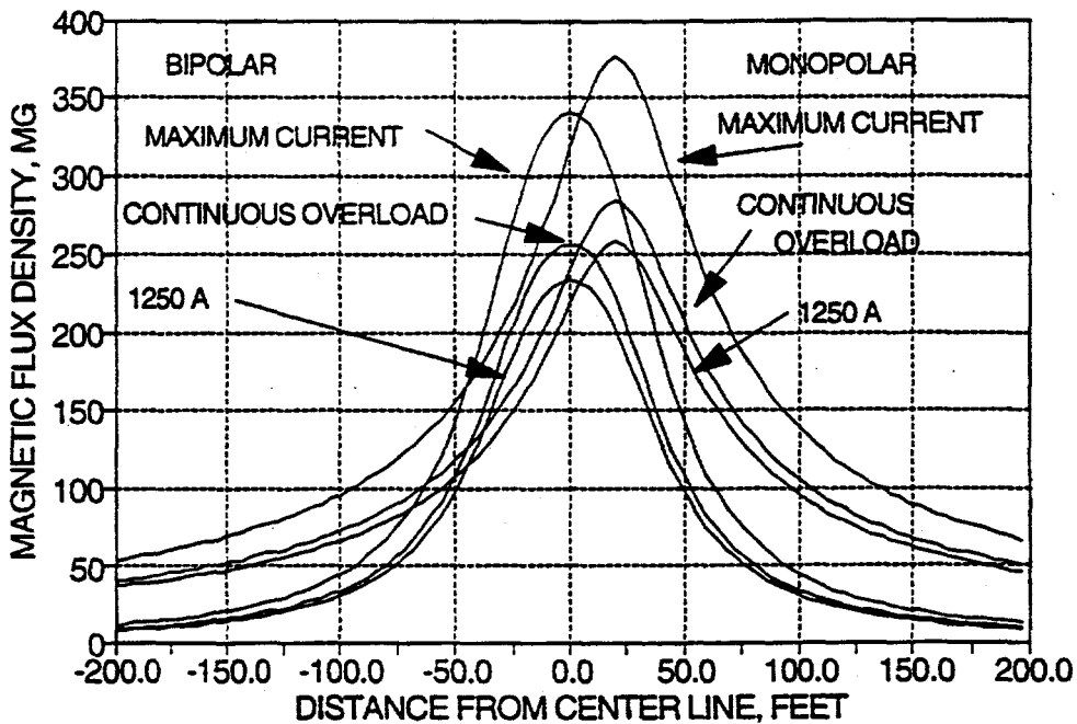
Figure 10.10 MF DC Line Monopolar and Bipolar Operation
