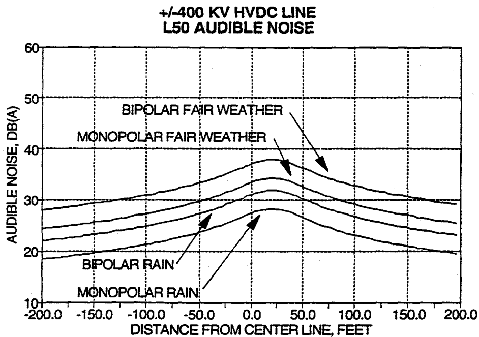
Figure 10.6 AN DC Line Monopolar and Bipolar Operation
