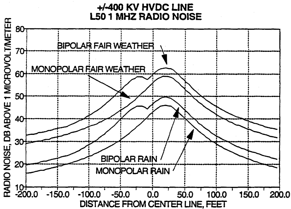
Figure 10.2 RN DC Line Monopolar and Bipolar Operation
