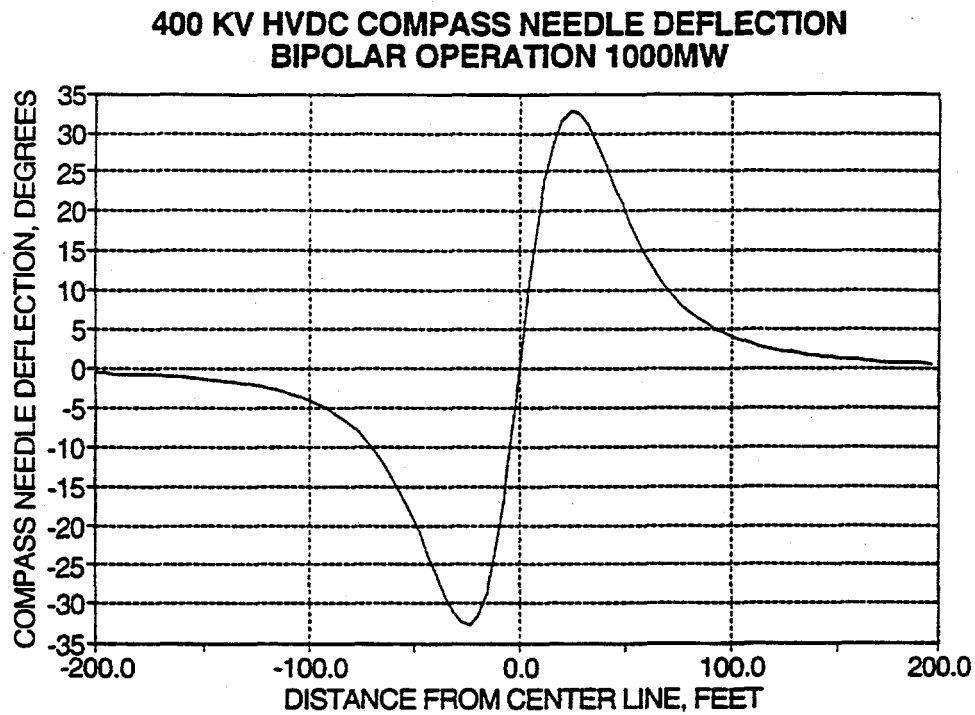
Figure 10.12 Bipolar Operation Compass Needle Deflection
