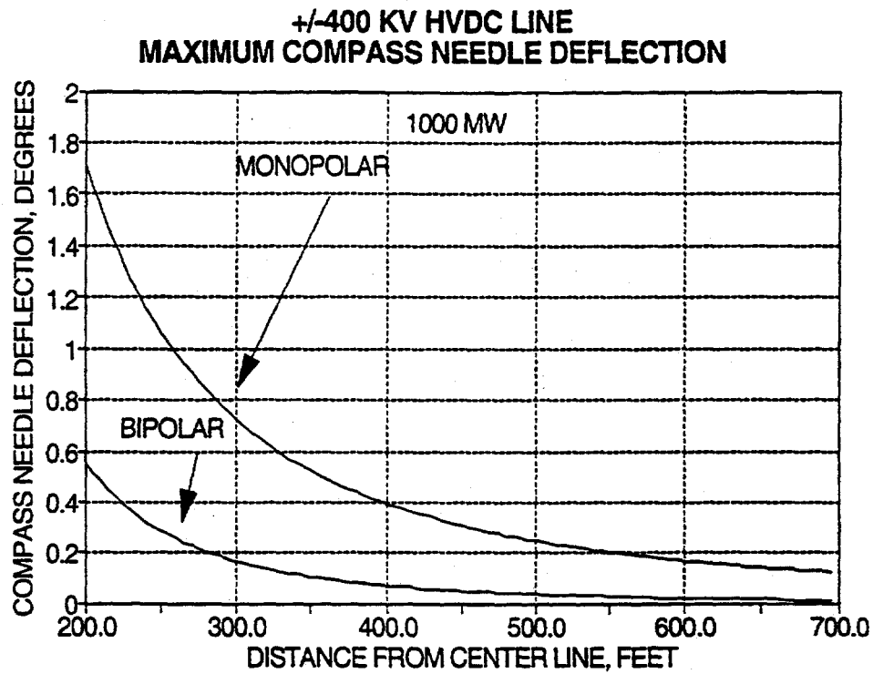
Figure 10.14 Compass Needle Deflection Far From DC Line
