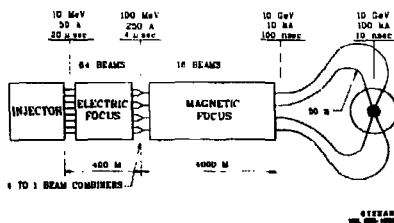
Fig. 3. Schematic of a driver with parameters near the cost optimum.
