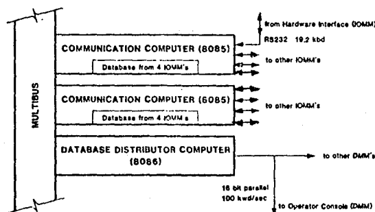
Fig. 4: Multiplexer Microcomputer Module. Database information is exchanged between eight IOMM's and one of the display microcomputer modules through this unit, using both serial and parallel transmission. Shared access to any of the IOMM databases is essential.
