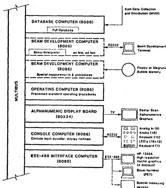
Fig. 5: Display Microcomputer Module. Up to three independent computers (boxes 2 to 4 from top) are planned to perform the operating tasks. They have access to the accelerator by writing into or reading from the database. They control the console devices by exchanging messages with the console computer over the Multibus.
