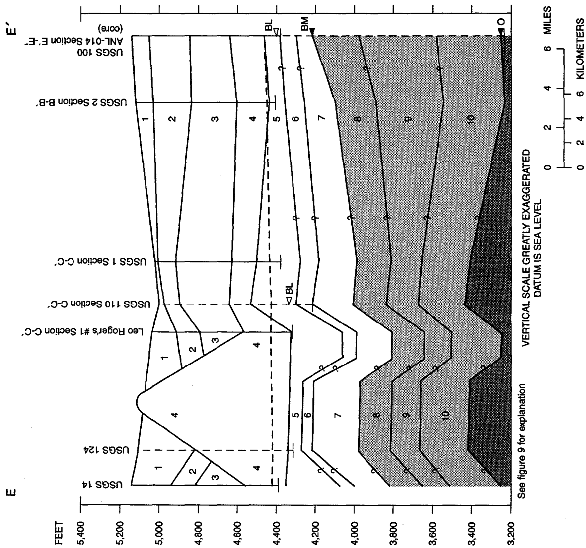
Figure 14. Geologic section E-E' at the Idaho National Engineering Laboratory.
