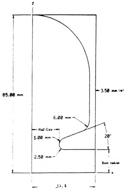
Fig.2 Cross section of a typical accelerating cavity.
