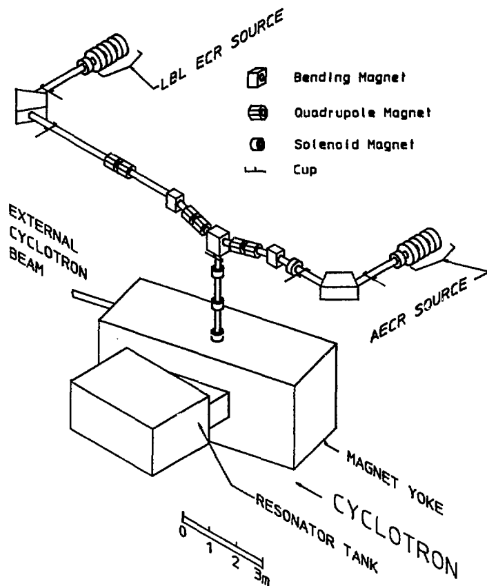
Fig. 1. Schematic view of the injection beam transport lines for the 88-Inch Cyclotron, from the LBL ECR and the AE CR sources. Either of these two ion sources can inject beams into the cyclotron. XBL 915-1071.
