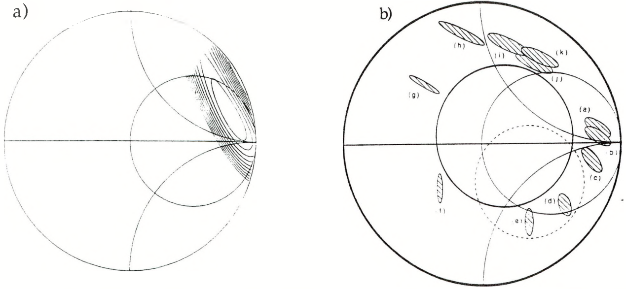
Fig. 3 a) Typical contour map of the fitting parameter \epsilon as a function of embedding admittance plotted on an admittance Smith chart. Fit quality is best inside the innermost oblong contour. Within this contour calculated pumped I-V curves are visually indistinguishable from those measured experimentally. The contour spacing is 0.0005 \text{ mV}^2 . The chart is normalized to 0.02 \Omega^{-1} . b) Range of admittances available at 93 GHz. The ranges of imbedding admittance deduced from a set of I-V curves pumped at 93 GHz, each with the backshort position stepped 0.0165 \text{ mm} farther away from the mixer, are represented by the shaded regions. Region (a) is for the backshort approximately 1.15 \text{ mm} away from the junction, with this distance increasing to region (k). The dashed circle is the range of imbedding admittances measured from the scaled model at the scaled frequency corresponding to 93 GHz. The solid circle is the same range, except that the susceptance due to the estimated capacitance of 160 \text{ fF} has been added in parallel.
