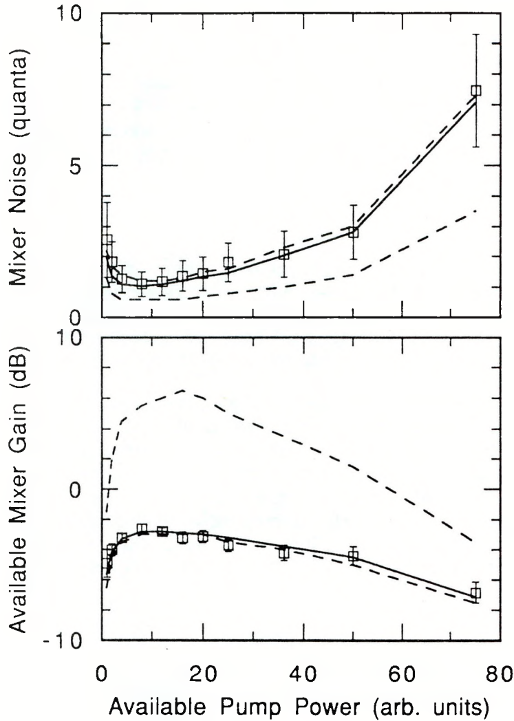
Fig. 4 Added mixer noise and available gain as a function of local oscillator power with f_{LO} = 95.0 GHz, V_{DC} = 1.956 mV. The dashed lines are the limits of the performance that are consistent with I-V curve shape. The solid line is the best fit to measured performance, with Y_{USB} = 0.14 + 0.08i \Omega^{-1} and Y_{LSB} = 0.04 + 0.18i \Omega^{-1} . All measurements were performed with no applied magnetic field.
