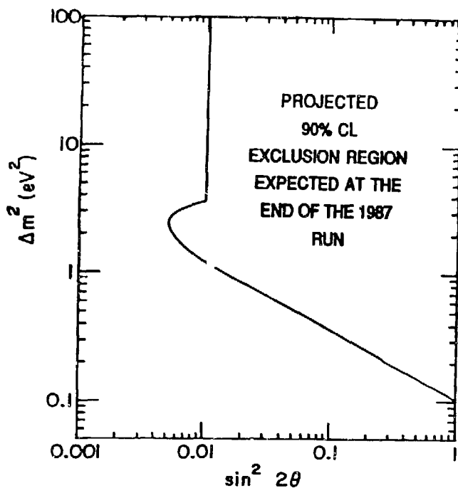
Fig. 4b Projected limits (90% cl) from the present E645 \bar{\nu}_\mu + \bar{\nu}_e appearance search. The limits indicate the expected sensitivity if no evidence for neutron oscillations is seen in the rest of 1987 run
