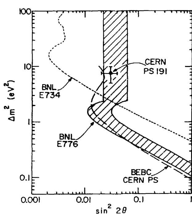
Fig. 4a Exclusion limits (90% cl) and possible positive indications ( 1\sigma ) from \nu_\mu + \nu_e searches. (See References in the text, especially Refs. 7 and 8)
