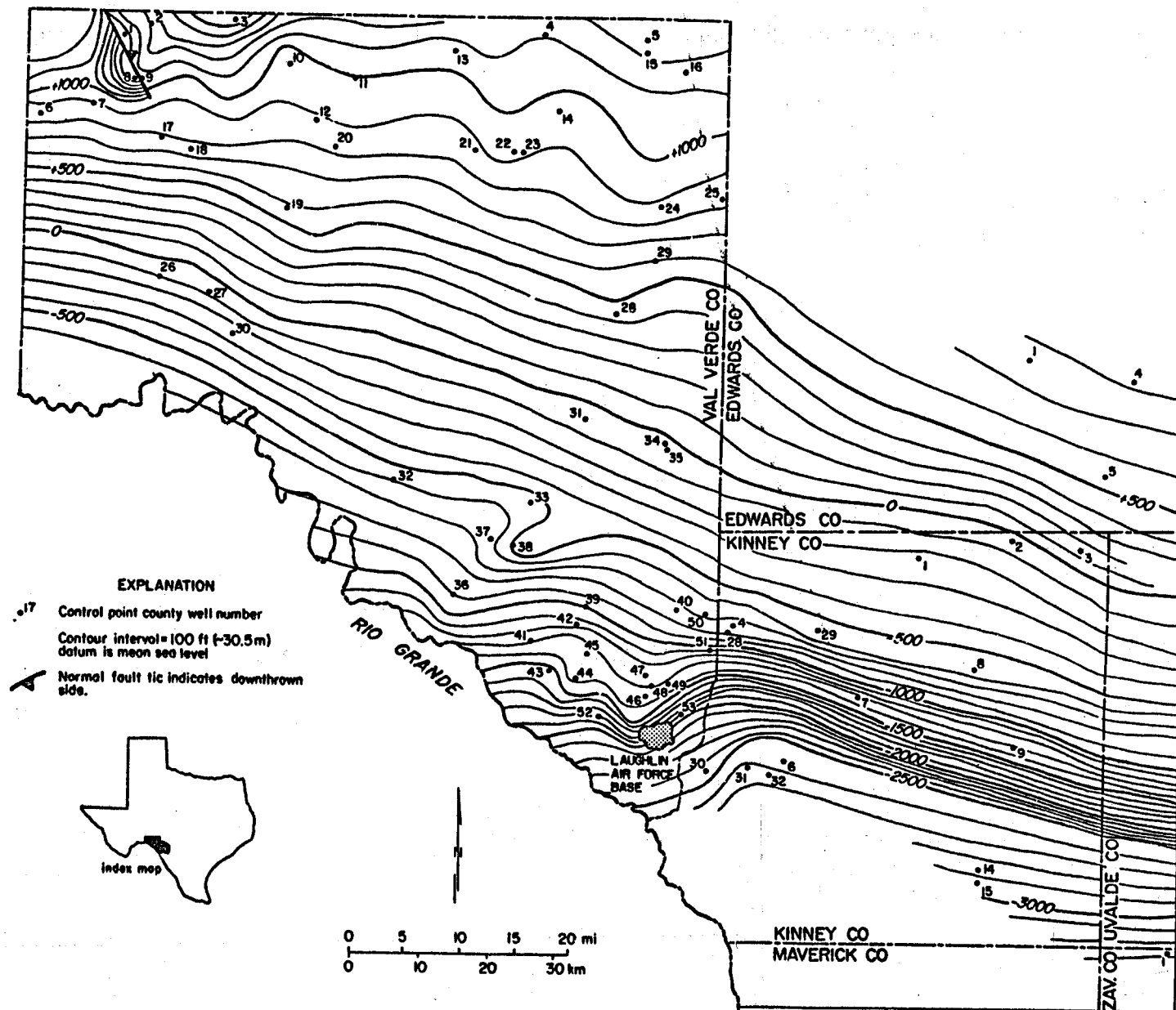
Figure H-16. Structure Contour Map on the Top of the Paleozoic Complex, Val Verde and Kinney Counties.
