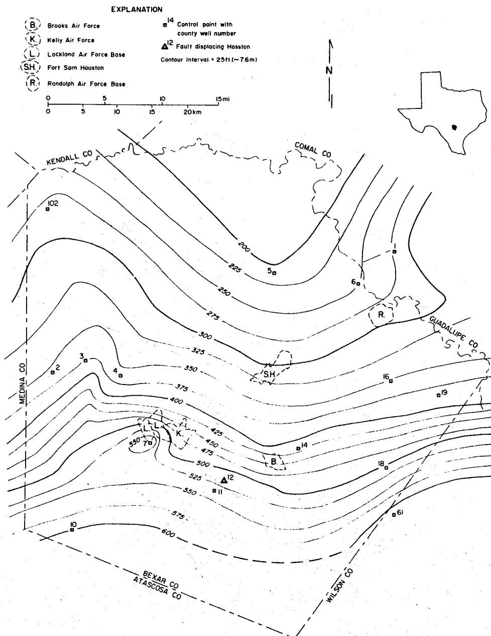
Figure H-10. Total formation thickness of the Hosston Sand, Bexar County.
