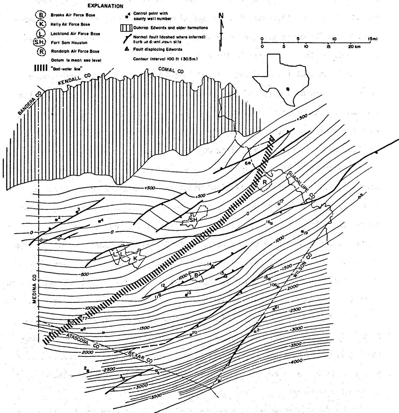
Figure H-4. "Bad-water line" of Edwards aquifer depicted on structural contours on top of the Edwards.
