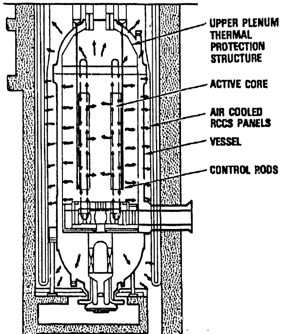
Figure 6 MHTGR Pressurized-Conduction Cooldown Heat Flow Path
