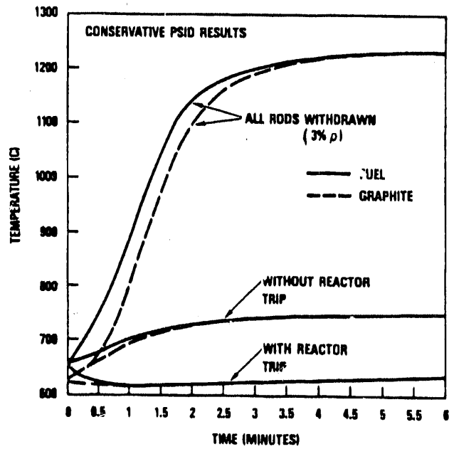
Figure 11 Control Of MHTGR Fuel Temperature By Negative Temperature Coefficient During Loss Of Forced Cooling.
