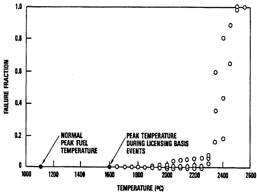
Figure 9 Integrity Of MHTGR Coated Fuel Particles During Temperature Ramp Tests In Which Fuel Was Heated From 1100 To 2500 °C In Times Ranging From 8 to 80 hours.
