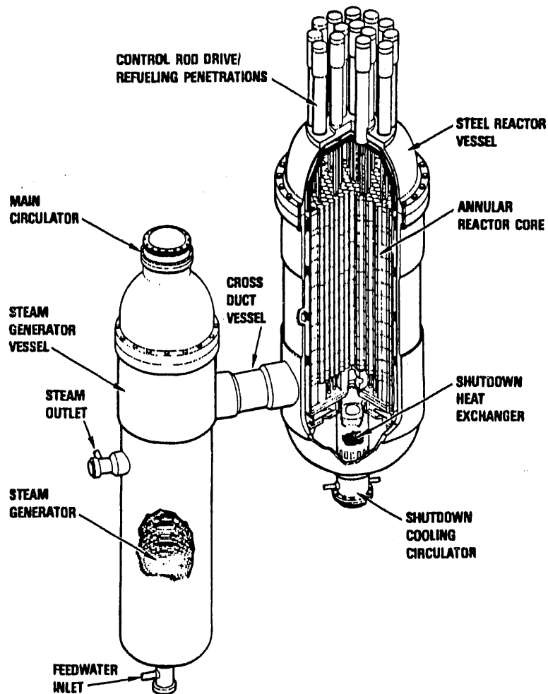
Figure 2 MHTGR Single Module Reactor Arrangement
