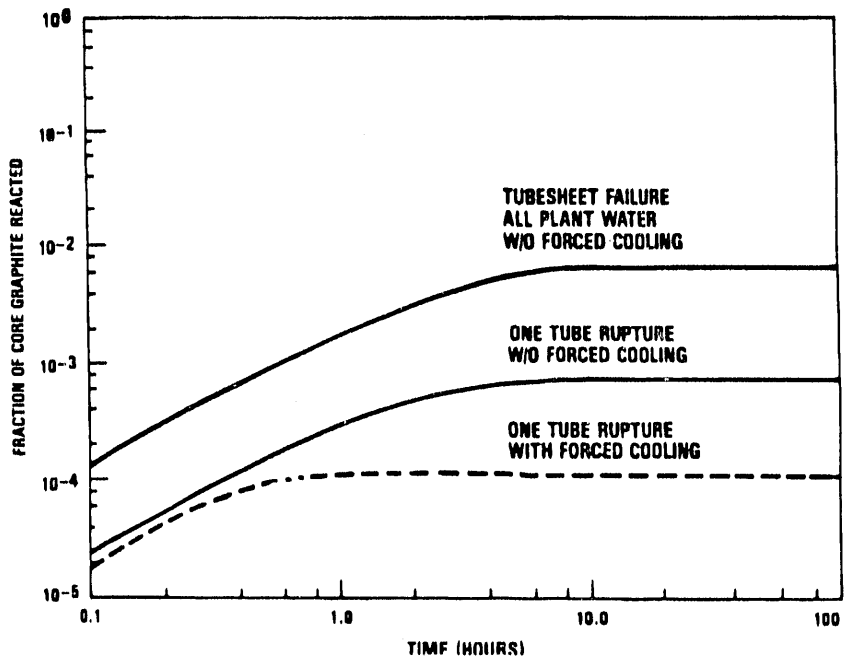
Figure 12 Integrity Assurance Of MHTGR Coated Fuel Particles During Water Ingress.
