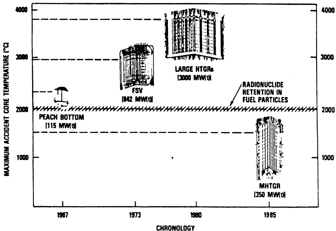
Figure 10 The MHTGR Represents A Fundamental Change In Reactor Safety Philosophy - Sized To Tolerate Even A Severe Accident
