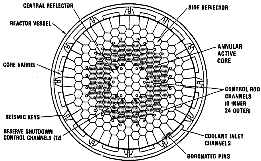
Figure 3 Reactor Core Cross Section
