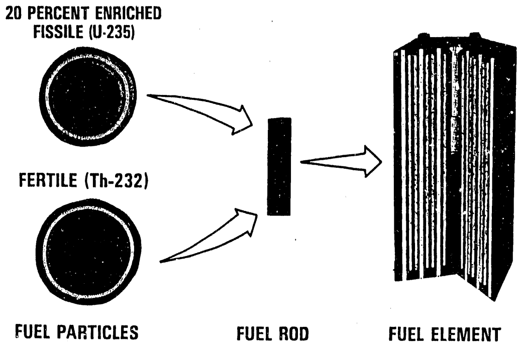
Figure 4 MHTGR Fuel Components
