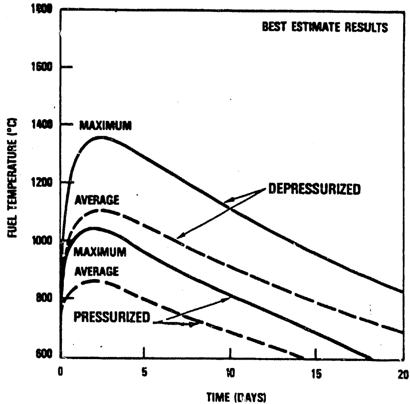
Figure 8 MHTGR Fuel Temperatures With Passive Heat Removal During Loss Of Forced Cooling.
