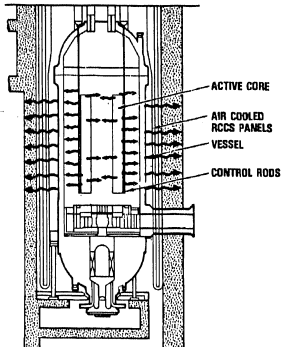
Figure 7 Depressurized-Conduction Cooldown Heat Flow Paths
