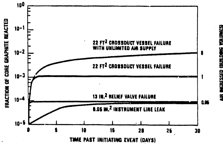
Figure 13 Insignificant Oxidation Of MHTGR Graphite Limited By Air Mass Transfer And Core Temperatures.
