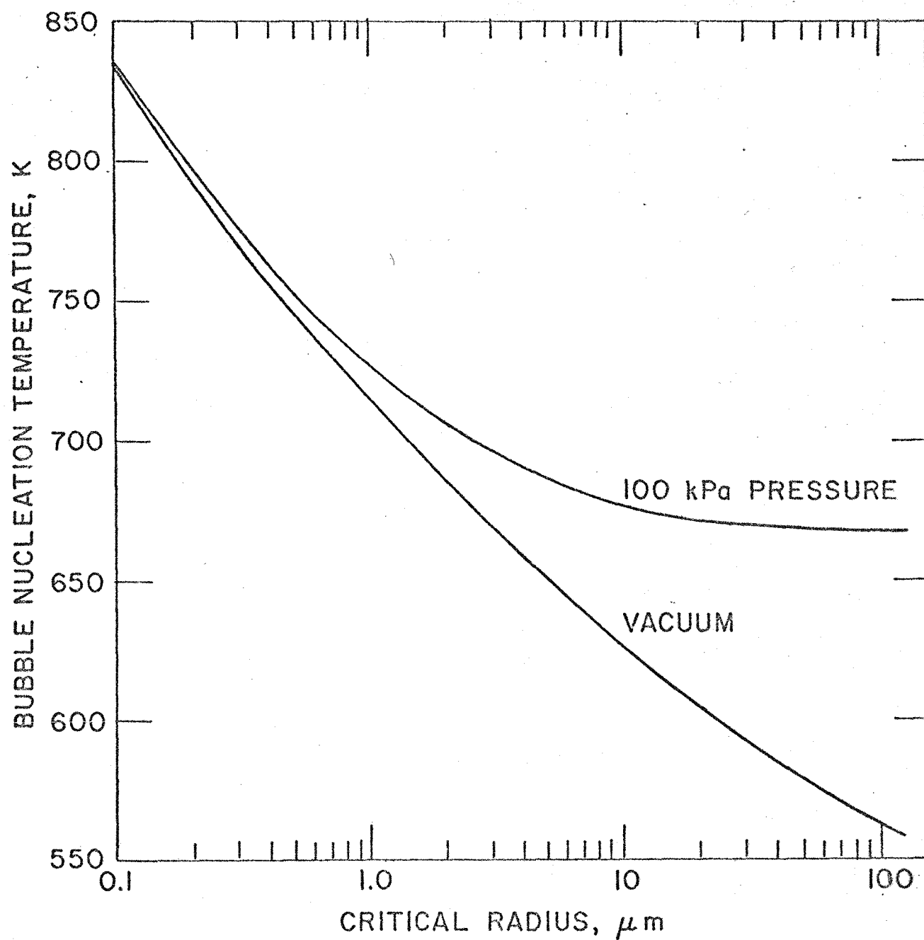
Figure 1. Temperature required to nucleate bubbles of various sizes under vacuum and atmospheric pressure.
