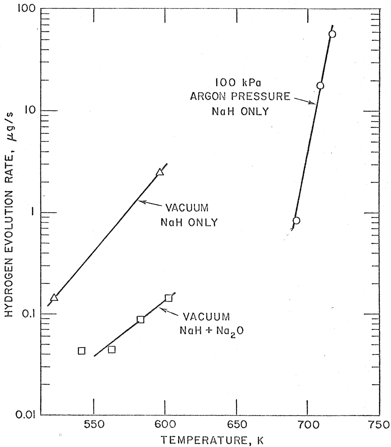
Figure 6. Hydrogen evolution rates observed in all tests.
