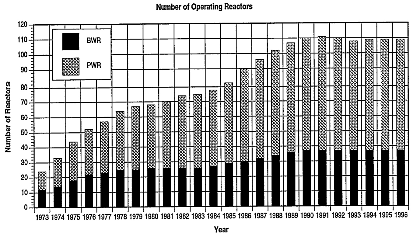
Figure 4.2 Number of Operating Reactors and Gross Electricity Generated 1973 – 1996
