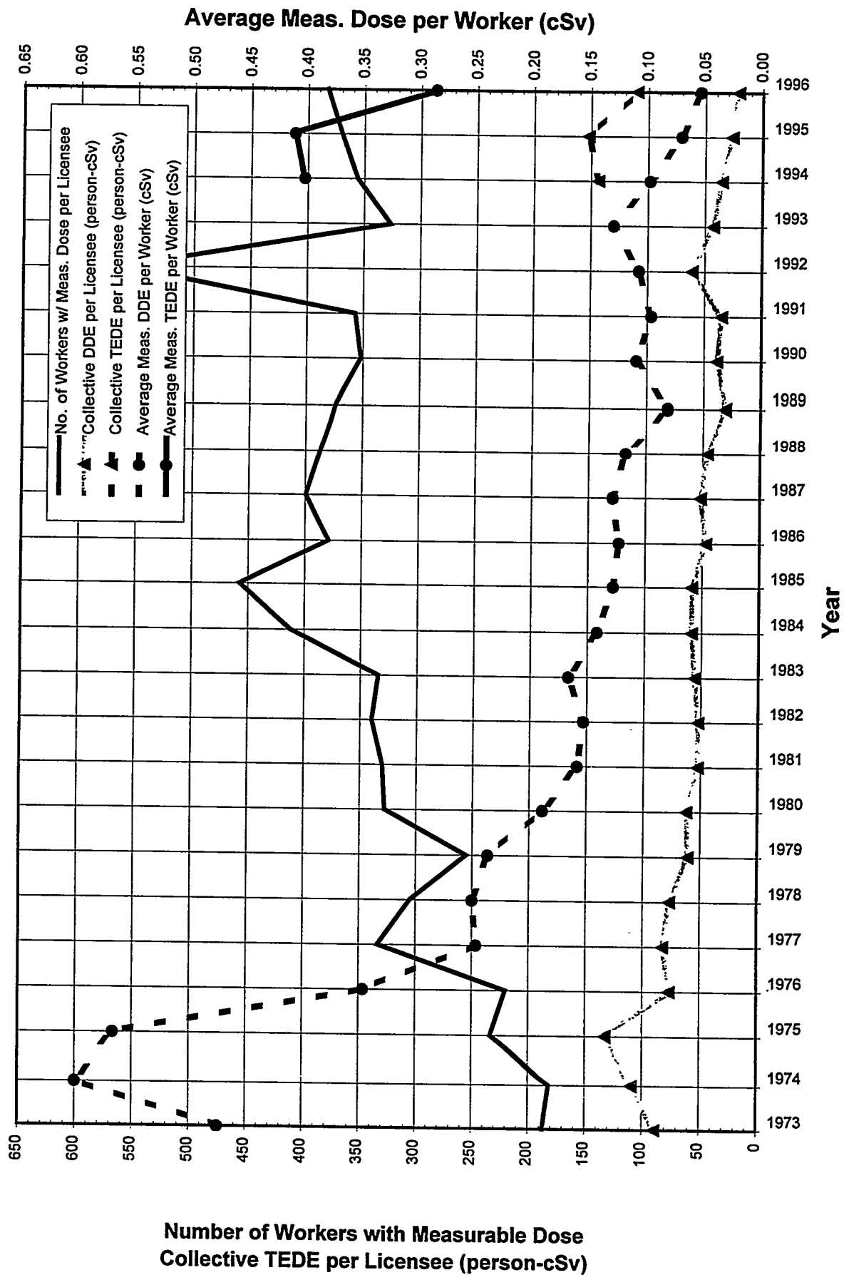
FIGURE 3.5 Average Annual Values at Fuel Fabrication and Processing Facilities 1973 - 1996
