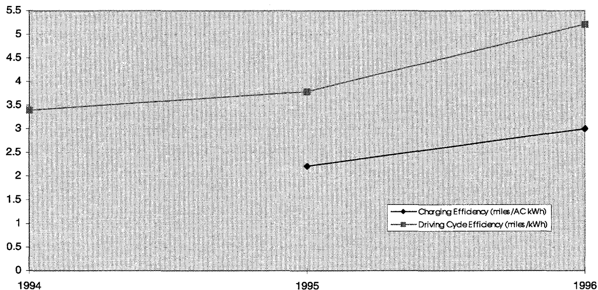
Figure EVA-2. EV America energy efficiency results for the charging efficiency test and the SAE J1634 driving cycle test. The plotted results are the average test results for all vehicles tested during each respective year. The charging efficiency test was not performed on the 1994 tested vehicles.
