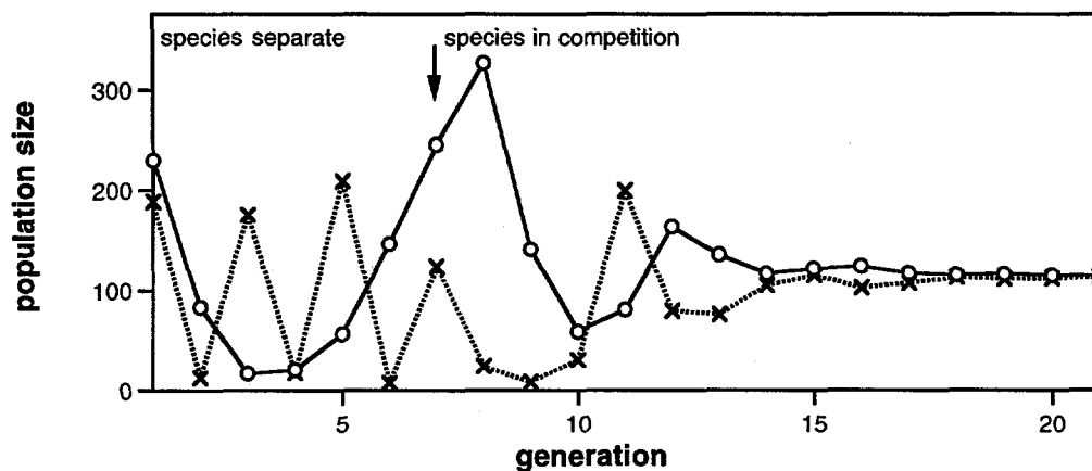
Figure 8. Demonstration of the effects of the introduction of a competitor on population dynamics. A) differences only in r ( r_A = 2.2, g_A = 0.0, \alpha_A = 0.75, r_B = 3.0, g_B = 0.0, \alpha_B = 0.75 ); B) differences in r and a ( r_A = 2.2, g_A = 0.0, \alpha_A = 0.5, r_B = 3.0, g_B = 0.0, a_B = 0.75 ); C) differences in r and g ( r_A = 1.2, g_A = 1.0, \alpha_A = 0.75, r_B = 3.0, g_B = 0.0, \alpha_B = 0.75 ). See text for further discussion.
