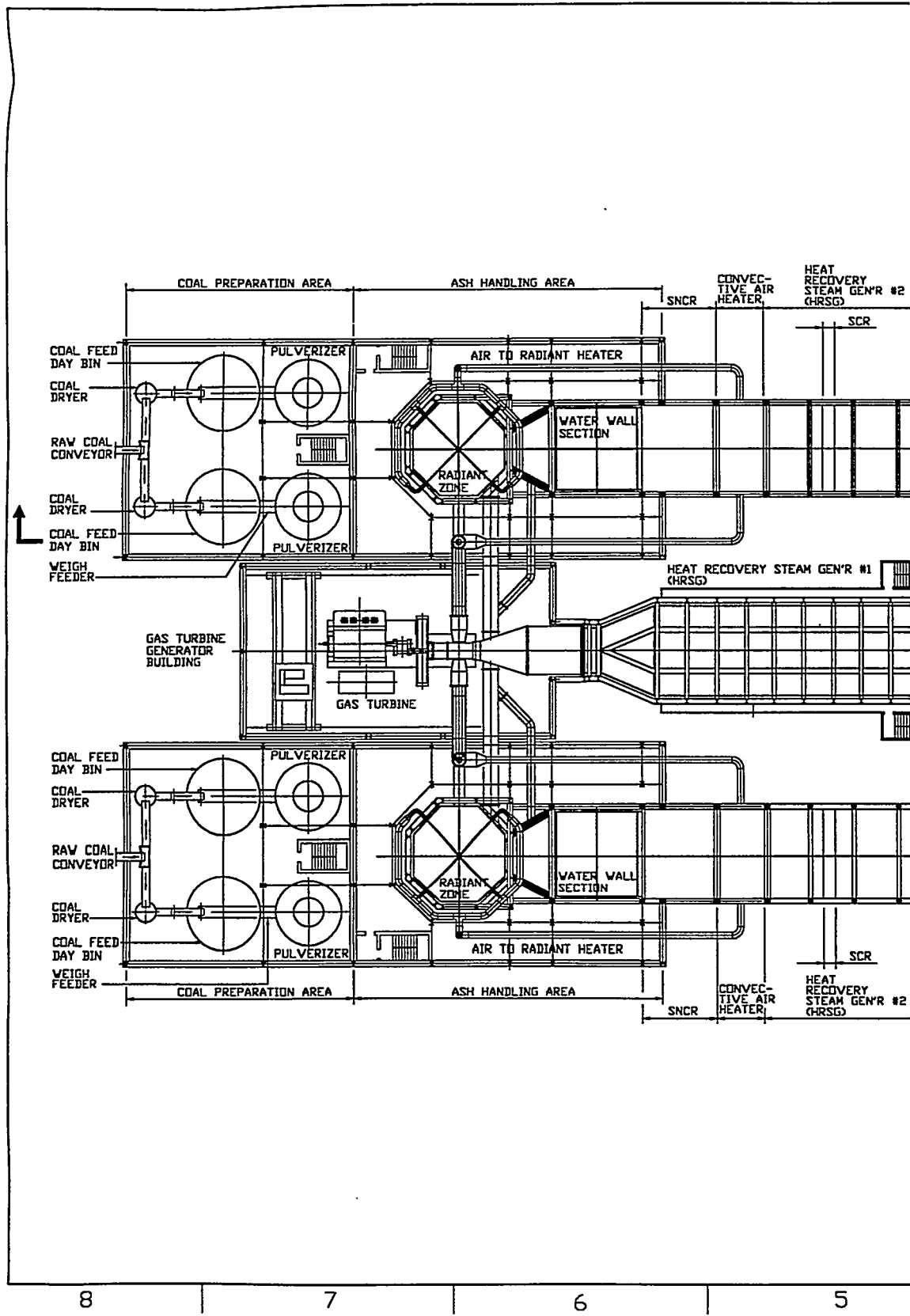
Figure 3.3-3 HIPPS I
