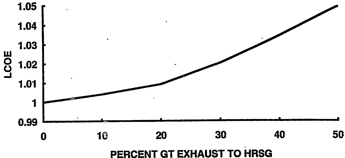
Figure 3.15-2 LCOE for FT4000 with Feed Water Heating.
