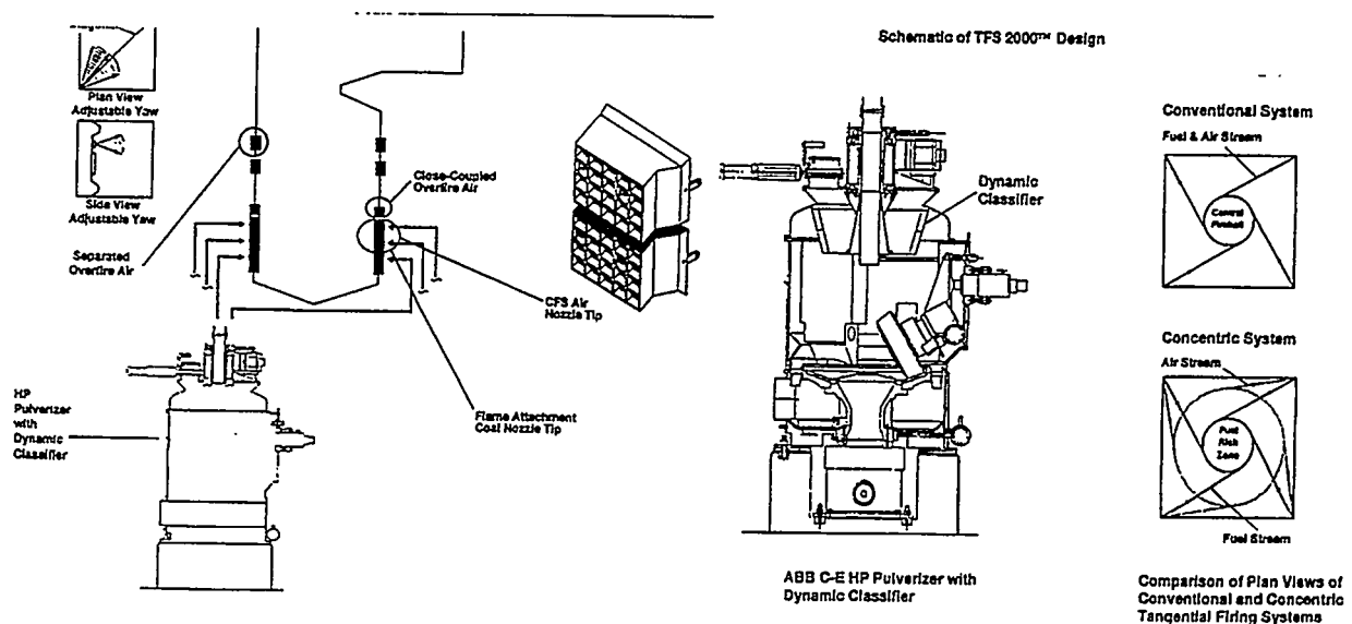
Figure 5.7-6 Schematic of ABB C-E's TFS-2000 Low- NO_x firing system, HP Pulverizer with Dynamic Classifier, and Plan View of Conventional and Concentric Tangential Firing System.
