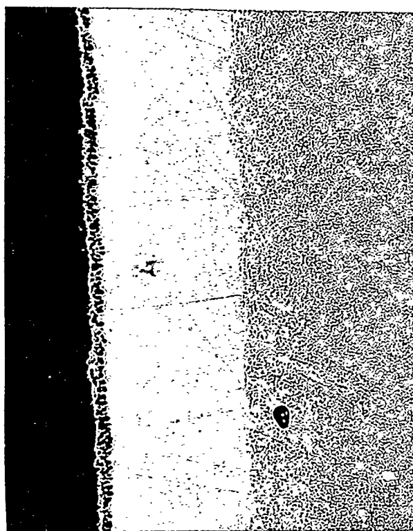
Figure 4.2-14c Compatability Studies - B-1900/Fusion Cast Chromia-Alumina. 500X
