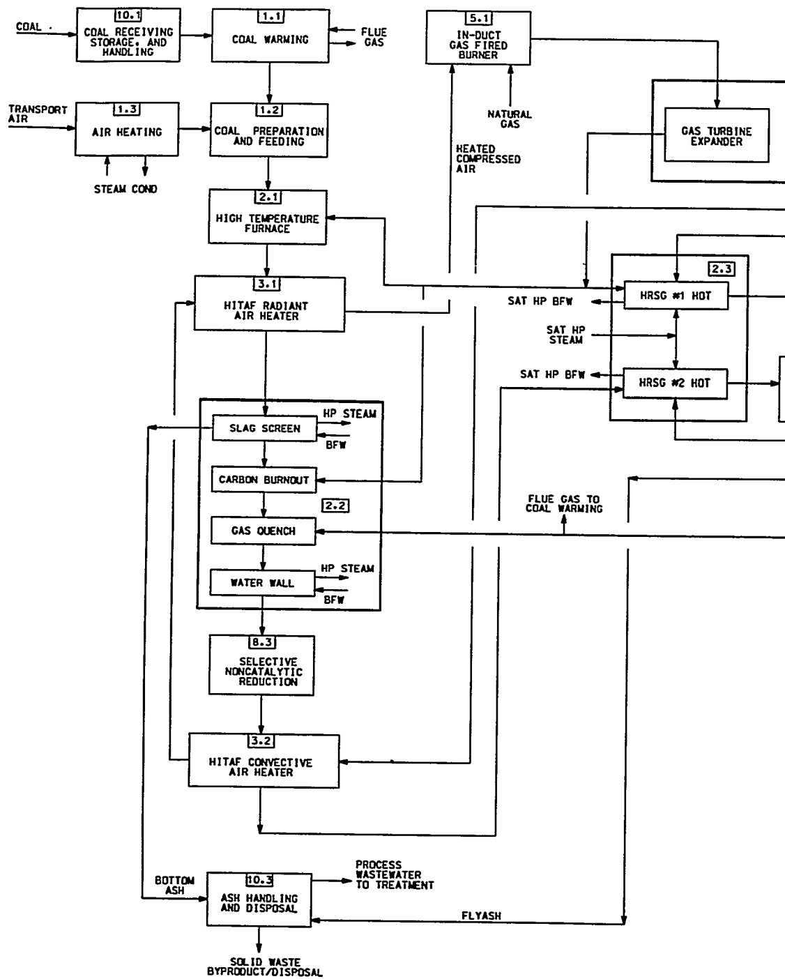
HIPPS Overall Block Flow Diagram
