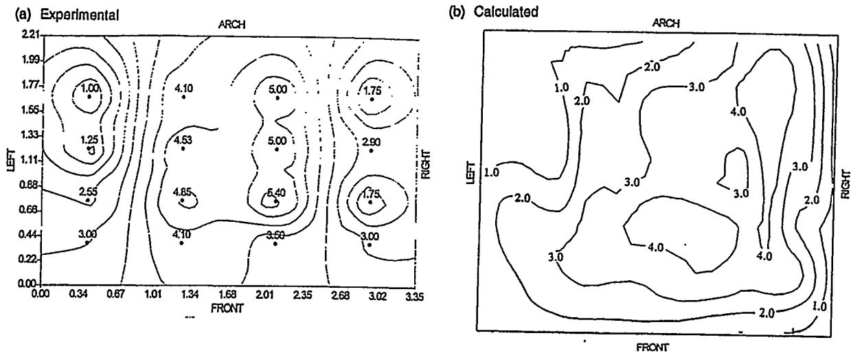
Figure 5.7-2 Comparison of Predicted and Measured Oxygen Mole Fraction Contours at the BSF Arch (HFOP) Elevation, (a) Experimental and (b) Calculated
