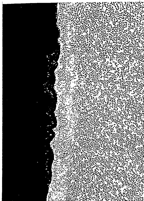
Figure 4.2-14d Compatability Stuies – B1900/Bonded Fused Grain AZS. 500X
