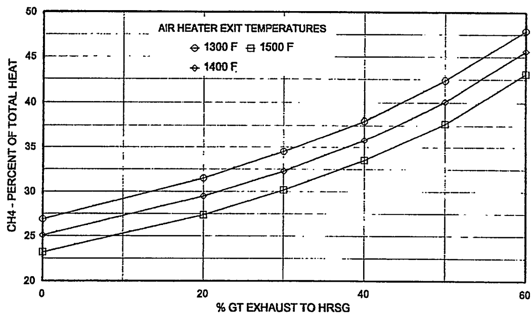
Figure 3.13-9 Methane Requirements.
