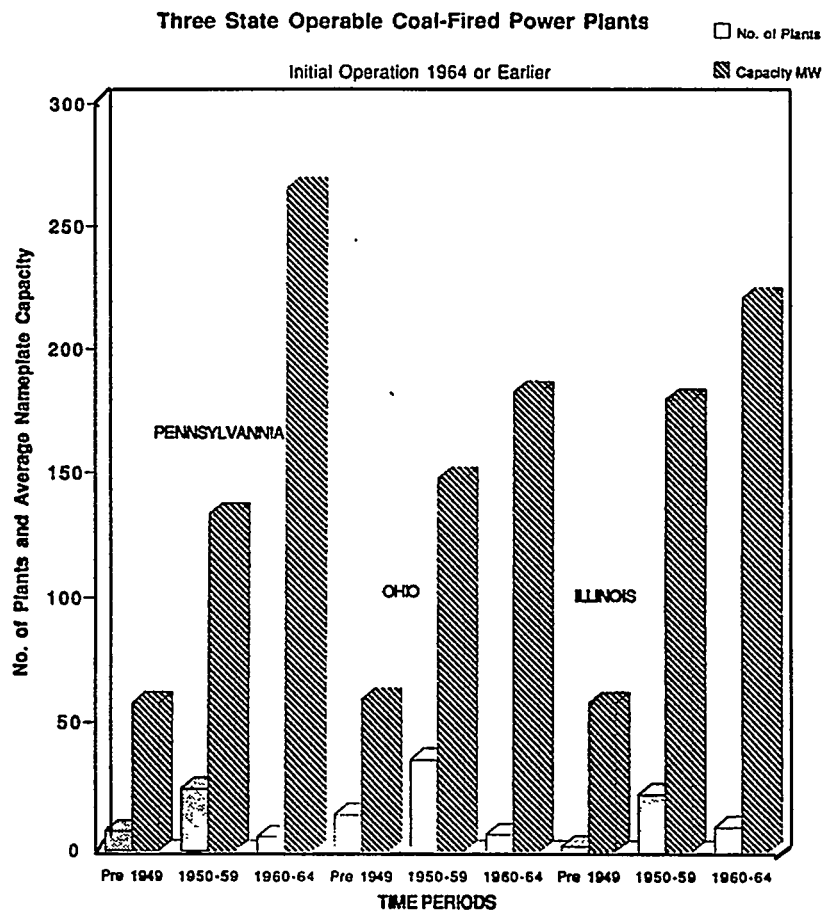
Figure 3.9-1 Installed Capacity.
