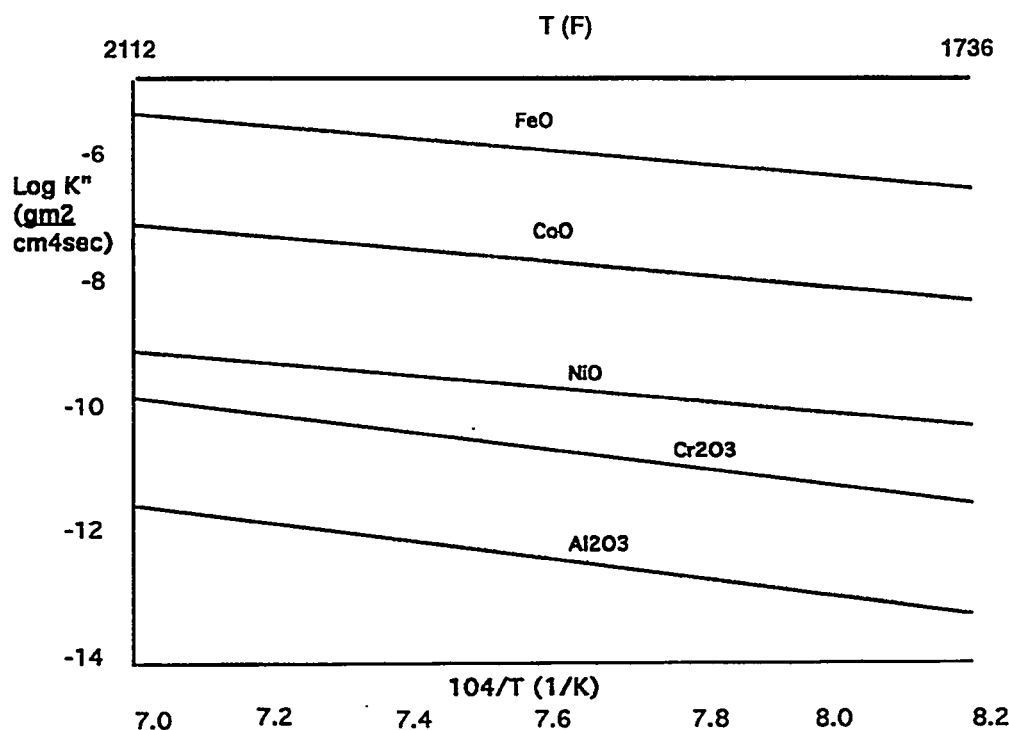
Figure 4.2-5 Oxidation Temperature Dependency.
