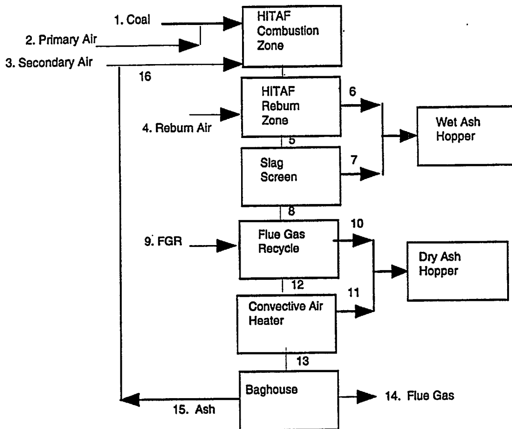
Figure 4.3-27 Ash Mass Balance in HITAF.
