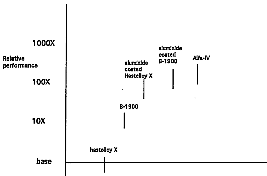
Figure 4.2-6 Relative Oxidation Resistance at 1950°F.
