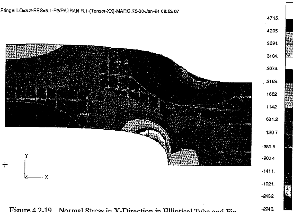
Figure 4.2-19 Normal Stress in X-Direction in Elliptical Tube and Fin.
