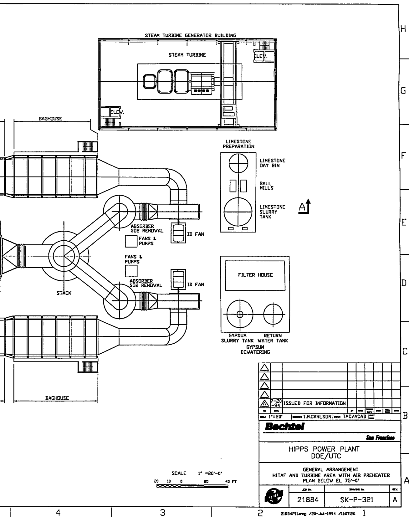
Equipment Plan View.
