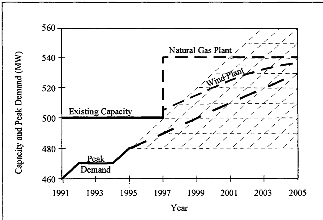
Figure 5-8. Municipal utility capacity with gas and wind plants.
