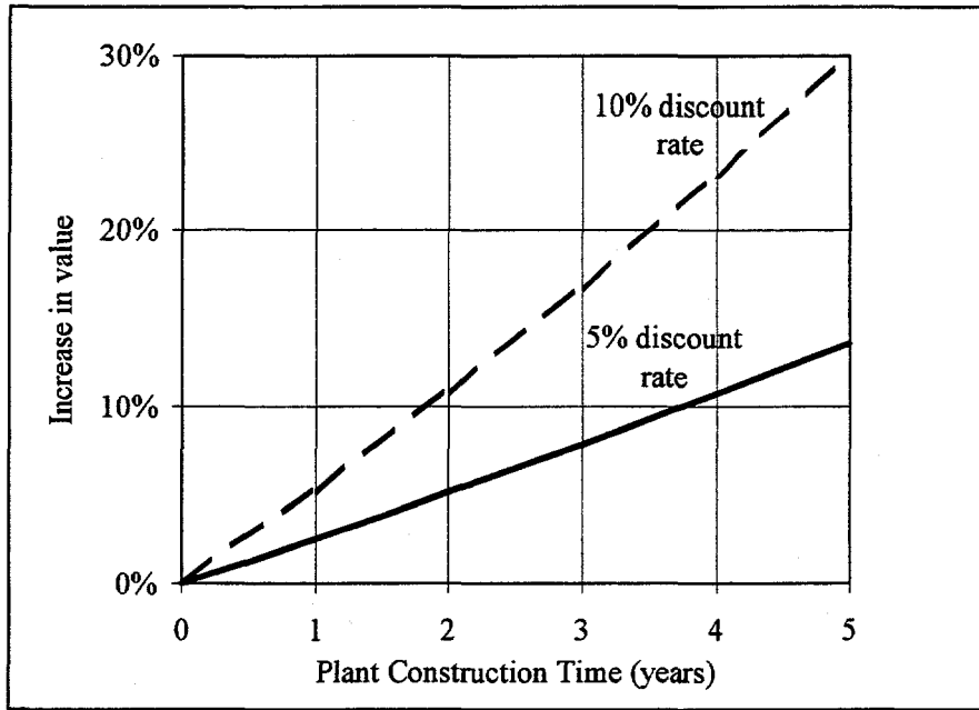
Figure 5-11. Value of early availability increases with construction time.
