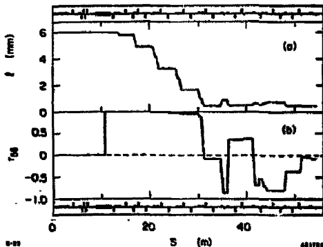
Fig. 5. (a) Bunch length vs. s (m) for V_{RF} = 33 MeV; \text{Bunl} rms length is 0.5 mm. (b) r_{02}(l - \delta) correlation vs. s (m).
