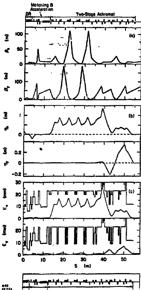
Fig. 4. (a) Beta vs. s (m); (b) Eta vs. s (m); (c) Envelope vs. s (m); where E = \sqrt{\epsilon_x^2 + \epsilon_y^2} , for \epsilon_x = \epsilon_y = 0.01 mm-mrad and \delta = 3\% .
