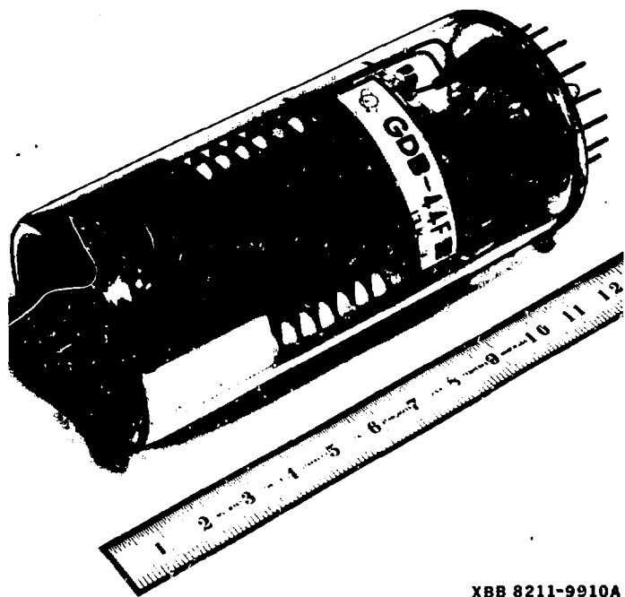
Fig. 1. The GDB-44F photomultiplier tube.
