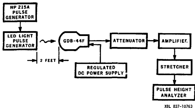
Fig. 13. Block diagram of the system for pulse-height resolution measurements.
