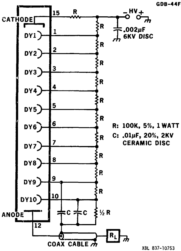
Fig. 2. Schematic diagram of high gain divider.
