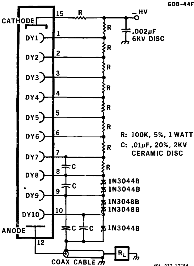
Fig. 3. Schematic diagram of high current divider.
