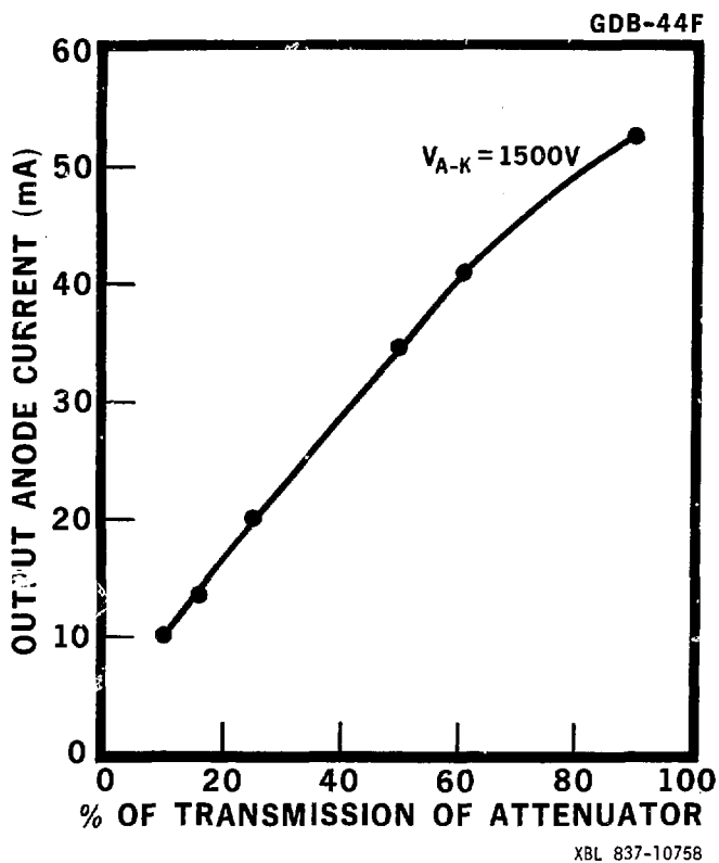
Fig. 7. Anode output pulse current as a function of light transmission of the optical attenuator.
