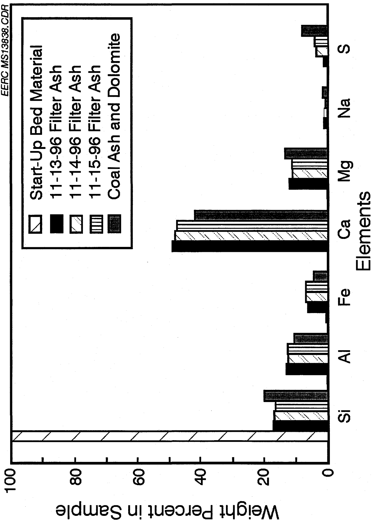
Figure 16. Chemical composition of filter ash for test P050.
