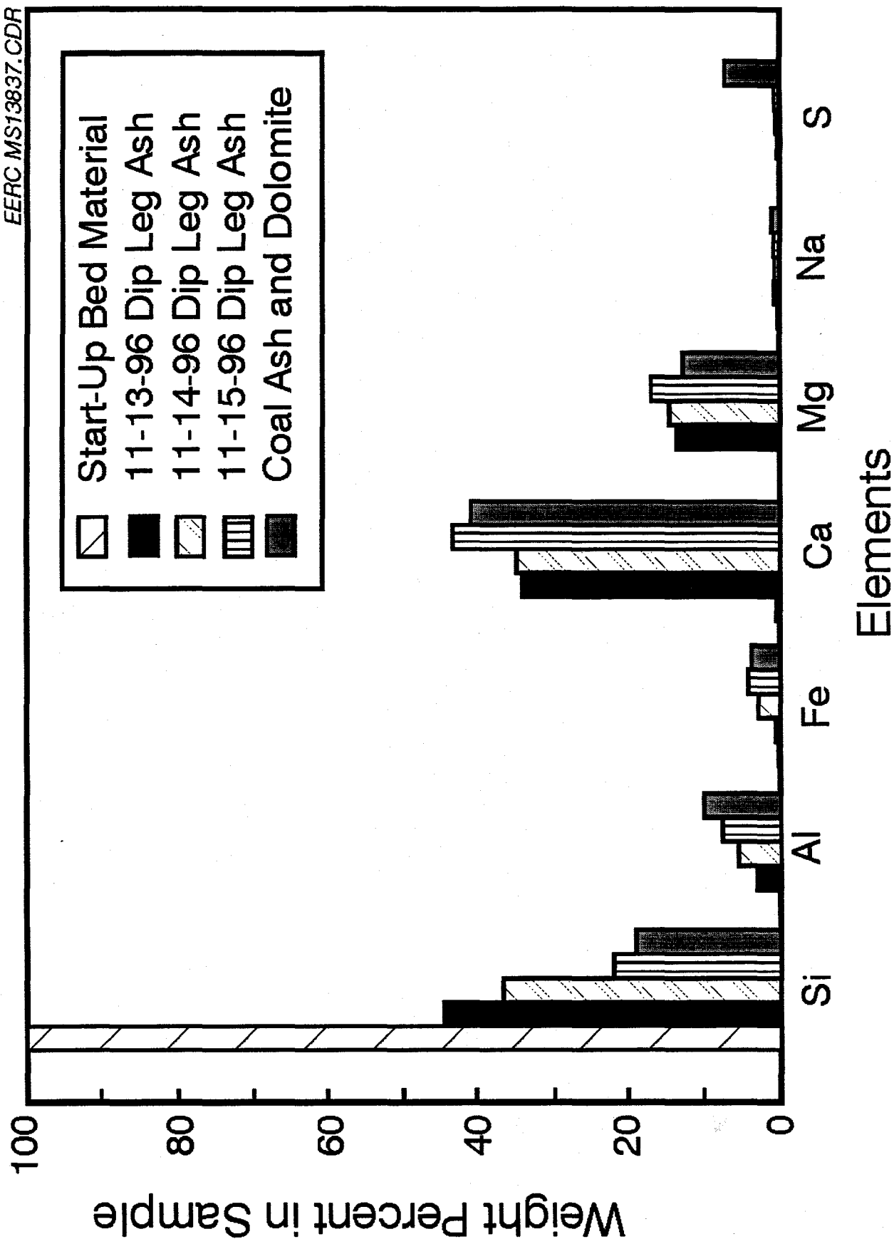
Figure 6. Chemical composition of primary cyclone ash during Test P050.
