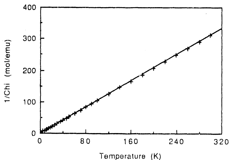
Figure 1. Plot of 1/\chi_M vs. T for (\text{Me}_5\text{C}_5)_2\text{VF}
