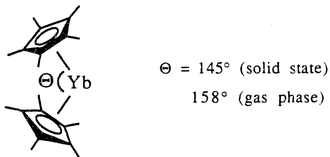
Figure 1. Structure of (\text{Me}_5\text{C}_5)_2\text{Yb} .
