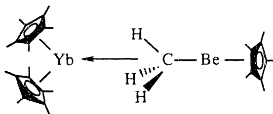
Figure 3. Structure of (\text{Me}_5\text{C}_5)_2\text{Yb}(\mu\text{-Me})\text{Be}(\text{Me}_5\text{C}_5) .
