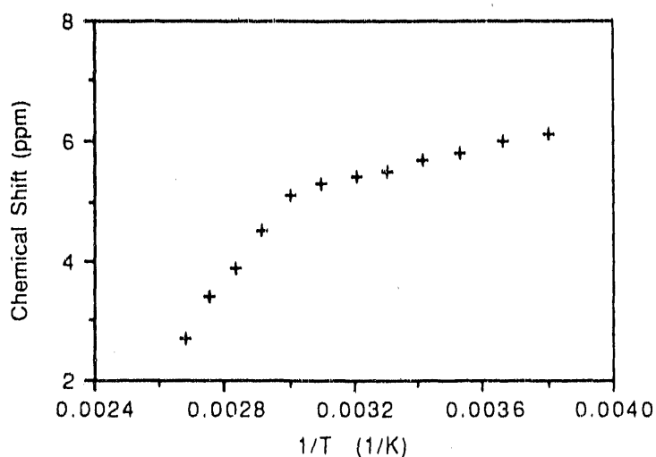
Figure 7. Plot of \delta vs. 1/T for [(\text{Me}_5\text{C}_5)_2\text{Yb}]_2(\mu\text{-Me})
