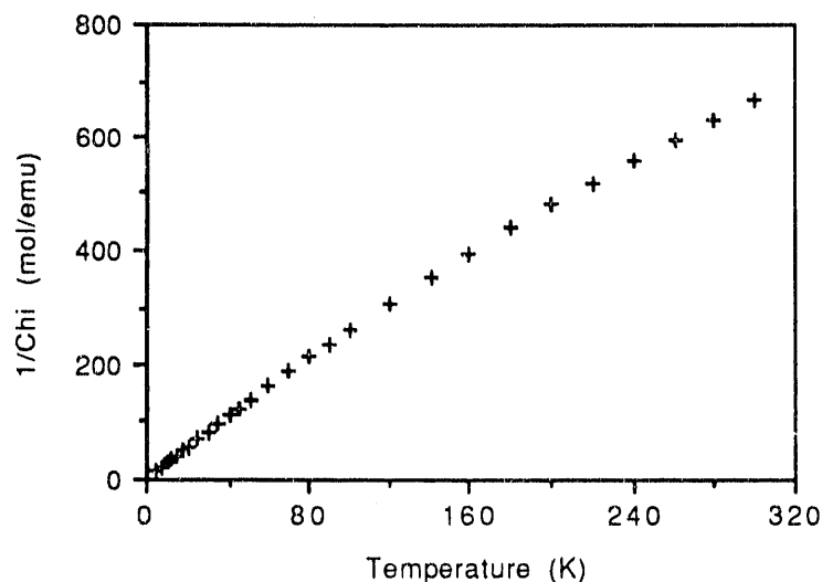
Figure 1. Plot of 1/\chi_M vs. T for (\text{Me}_5\text{C}_5)_2\text{TiH} .
