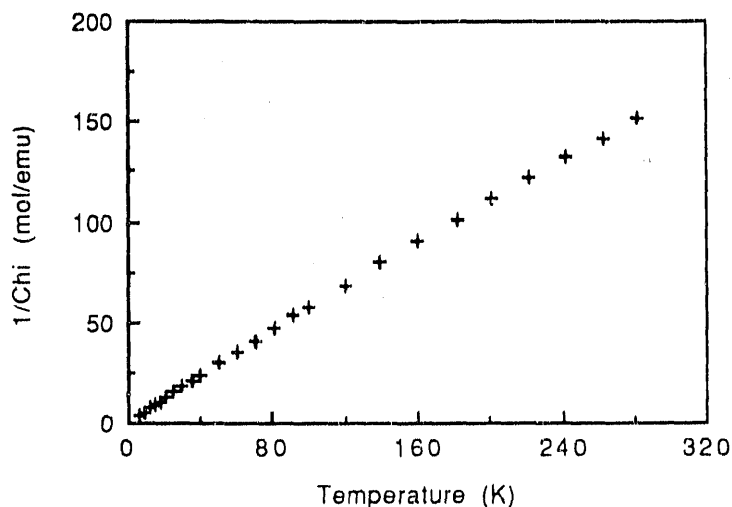
Figure 2. Plot of 1/\chi_M vs. T for (\text{Me}_5\text{C}_5)_2\text{YbMe}
