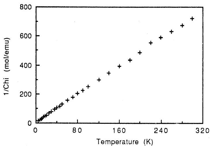
Figure 4. Plot of 1/\chi_M vs. T for (\text{Me}_5\text{C}_5)_2\text{Yb}(\mu\text{-Cl})\text{Ti}(\text{Me}_5\text{C}_5)_2 .
