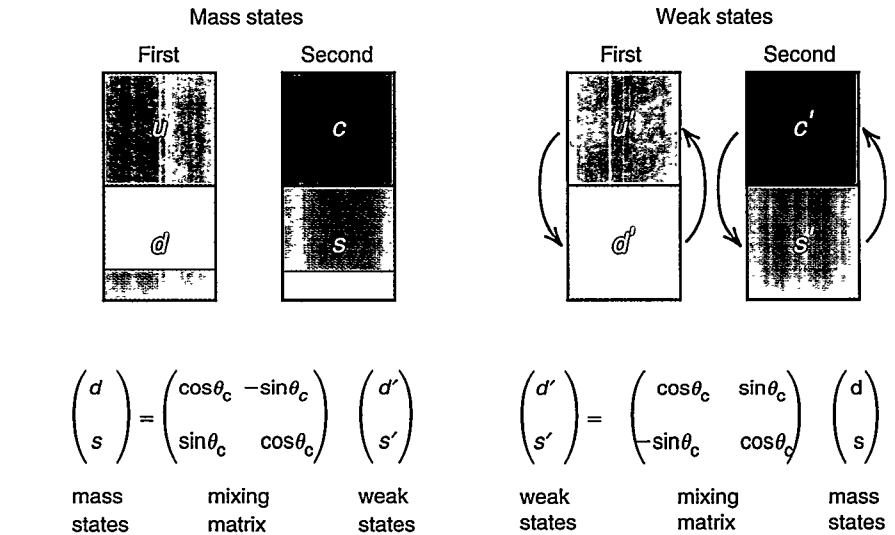
Figure 8. Two-Family Mixing among the Quarks
