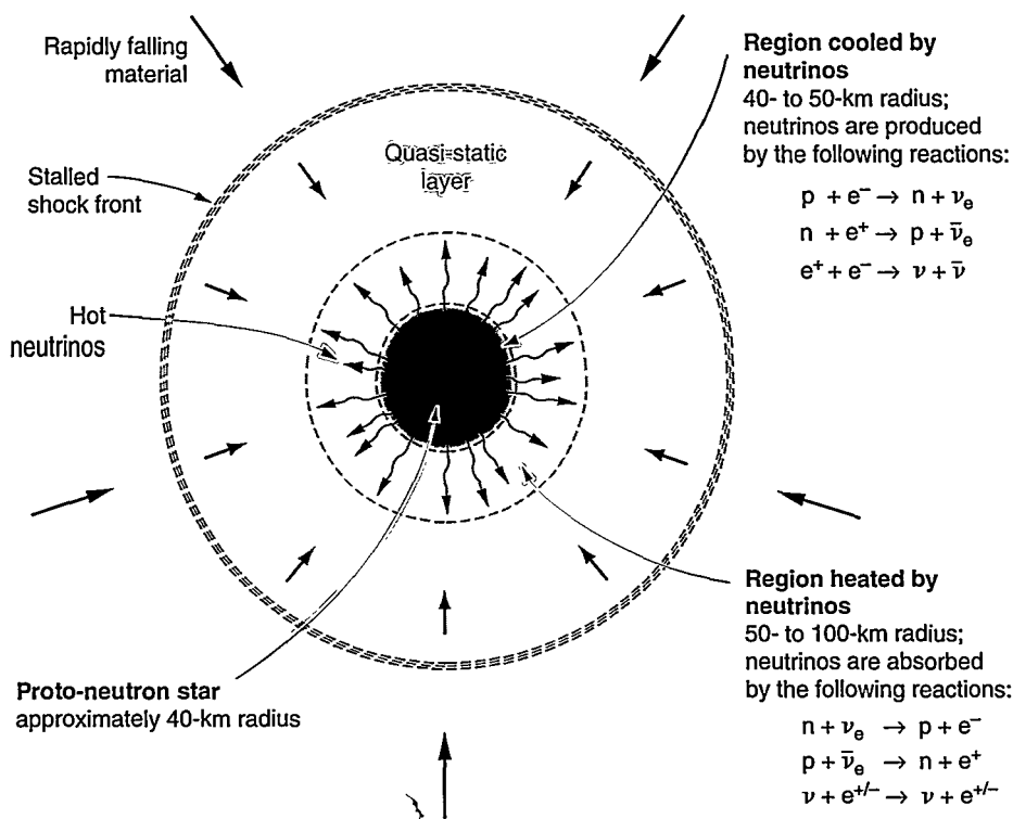
Figure 4. Behind the Front: Heating Matter with Neutrinos
