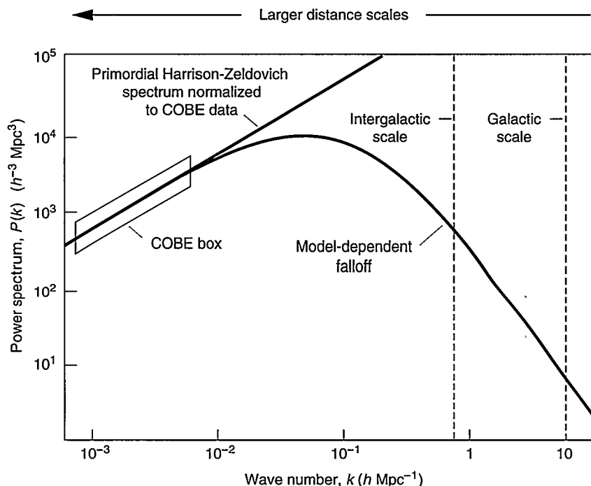
Figure 4. The Harrison-Zeldovich Spectrum and a Processed Spectrum
