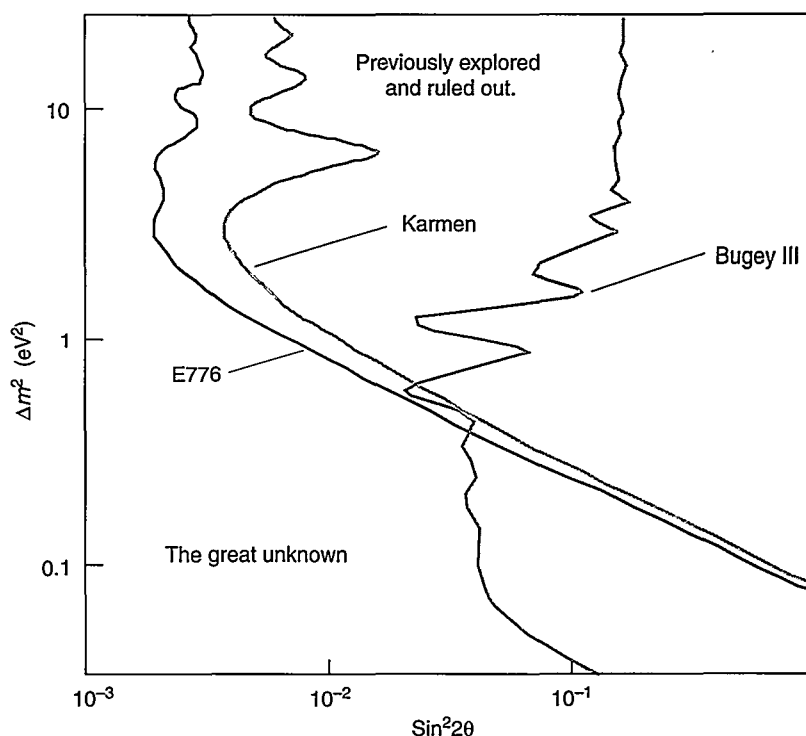
Figure 4. Values of \Delta m^2 and \sin^2 2\theta Explored Before LSND
