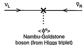
Figure 20. Neutrino Mass Terms
