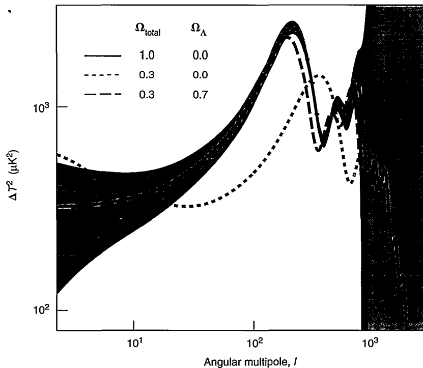
Figure 6. MAP and the Future
