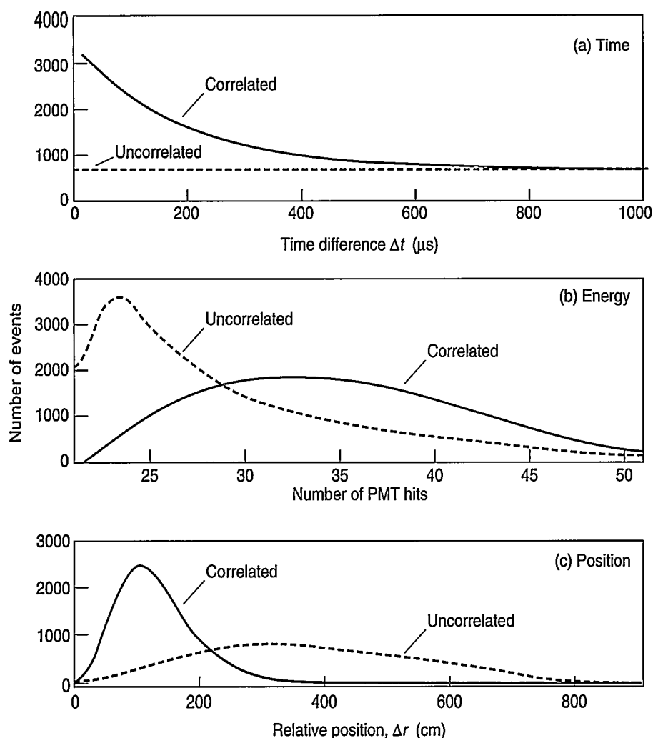
Figure 9. Identifying the Photon from Neutron Capture
