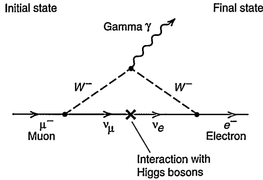
Figure 16. Example of Lepton-Family Mixing
