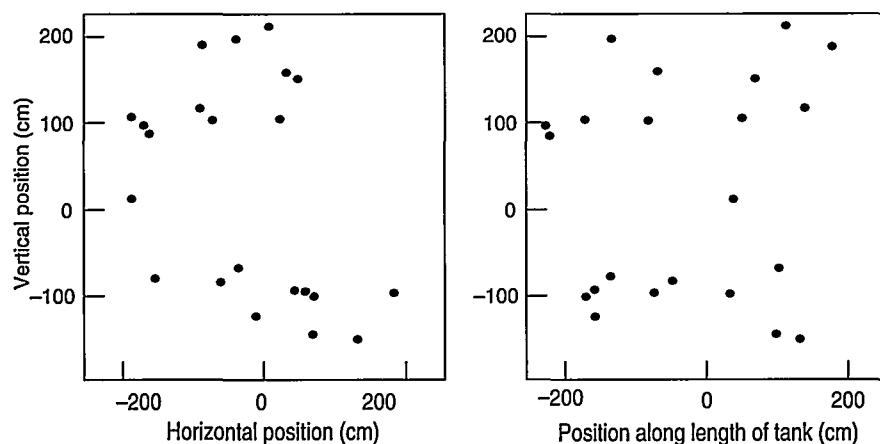
Figure 10. Evidence for Oscillations The likelihood function R was used to sift through the 1995 LSND data to determine if a photon was likely to have come from neutron capture and was correlated with a positron event. In all, there were 22 events when the beam was on that had R values >30 (that is, that had a high level of correlation). Only 4.6 \pm 0.6 events were expected from background processes. The 22 events appeared scattered across both tank cross sections.
