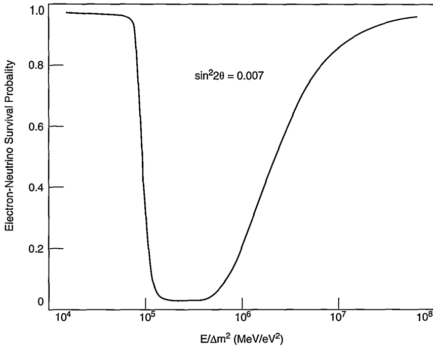
Figure 2. The MSW Survival-Probability Curve for the Sun
