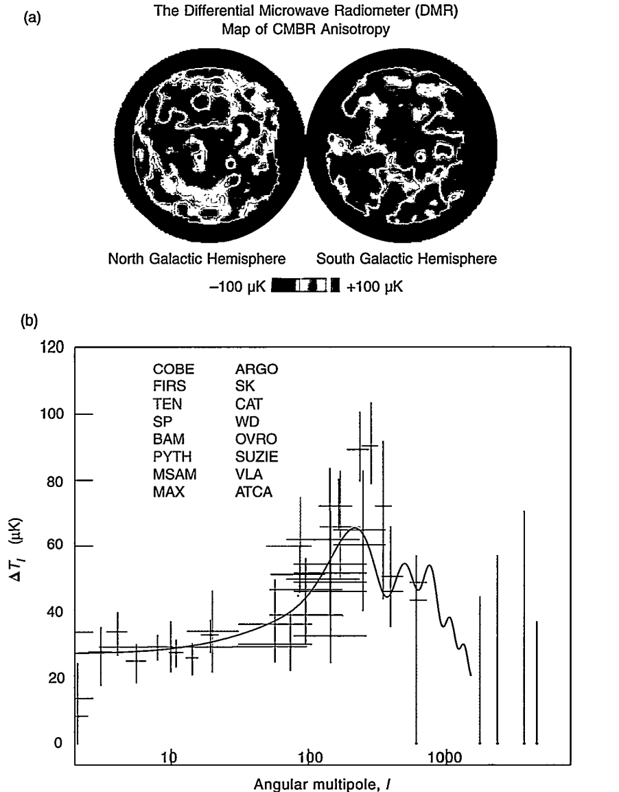
Figure 3. Temperature Fluctuations across the Microwave Sky
