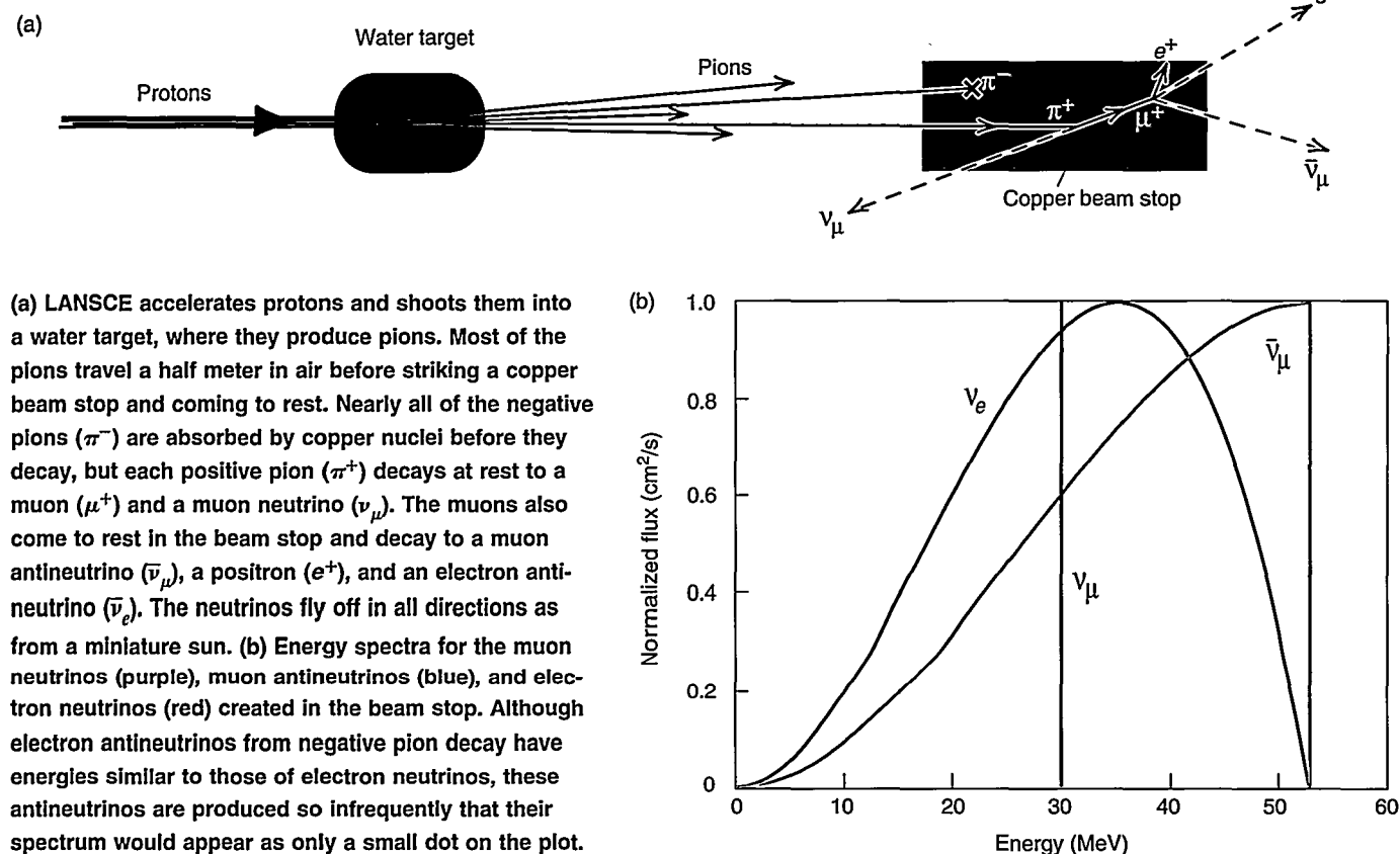
Figure 5. LANSCE Production of Decay-at-Rest (DAR) Neutrinos and Their Energy Spectra
