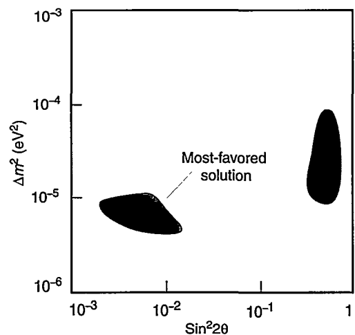
Figure 1. MSW Solutions to the Solar-Neutrino Problem
