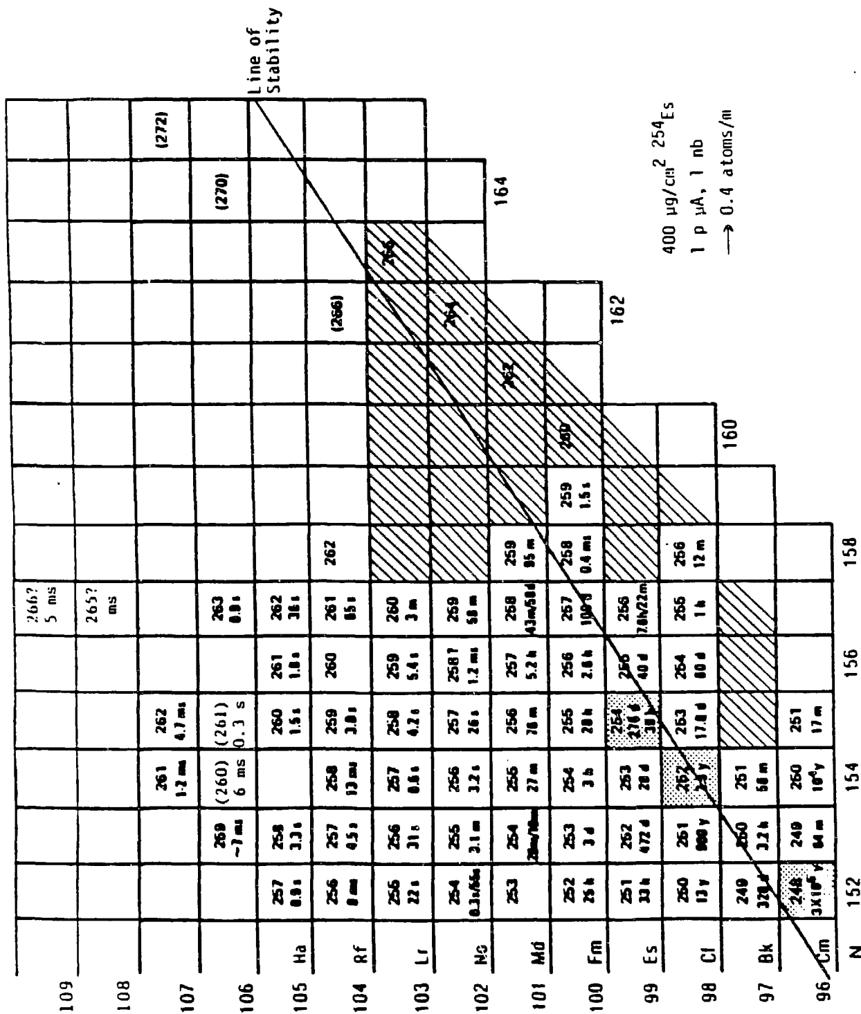
Fig. 1. Portion of table of isotopes showing neutron-rich trans-Actinoid isotopes. Hatched regions indicate new actinide isotopes postulated to be produced with >1-nb cross sections from transfer reactions to a 400 μg/cm 2 254 Es target with a projectile beam of 1 μA. Compound nuclei for reactions of 180 with 246 Cm, 252 Cf, and 254 Es are shown in parentheses.
