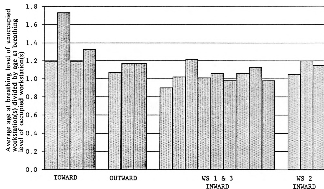
Figure 5. Average age of air at breathing level of unoccupied workstations divided by air at breathing level of occupied workstation(s). Only occupied workstations have an operating TAM. Tests with mixing fans in the CEC are not included. Tests are divided into groups depending on direction of air exiting TAM (toward occupant, outward, inward and upward). With air directed inward and upward, we separate tests with TAM operation in WS2 which was associated with short circuiting of supply air to the return grill.
