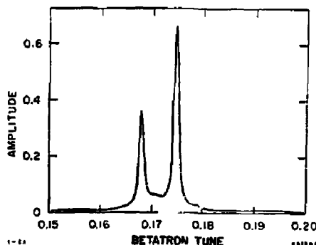
Fig. 4. Spectrum of the two-particle motion near the threshold.
