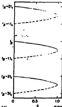
Fig. 5. The frequency spectra of the two fast-head-tail modes in the two-particle model. The solid curves are the spectra for one mode and the dashed curves are for the other mode. The frequencies of the two modes become degenerate at the instability threshold g = K/K_{\text{threshold}} = 1 .
