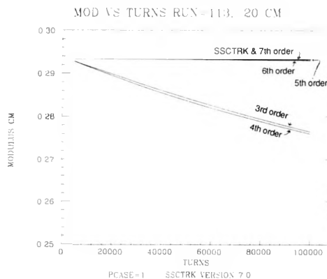
Figure 1: Comparison of the combined horizontal-vertical invariant for the truncated Taylor maps of order three through seven with that of the original SSCTRK kick-drift code for initial 2 mm amplitude over 100,000 turns.
