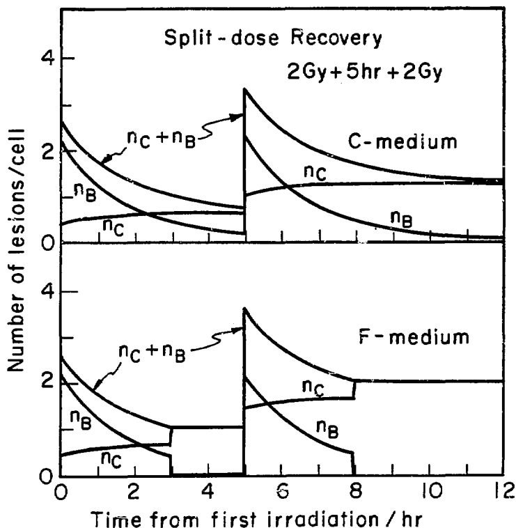
Figure 9. Time course of the mean number of lethal ( n_C ) and potentially lethal ( n_B ) lesions for a split dose recovery experiment in "conditioned" medium (top) and in fresh medium (bottom). The experiment assumes an absorbed dose of 2 Gy is followed by a repair period of 5 hours followed by another absorbed dose of 2 Gy. (XBL 836-3802)
