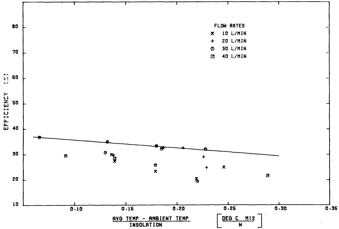
FIGURE 8 SCIENTIFIC ATLANTA FFNC EFFICIENCY VS DELTA TEMPERATURE / INSOLATION (RAW DATA)
