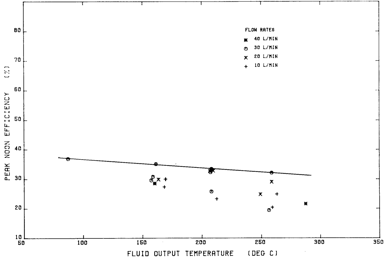
FIGURE 7 SCIENTIFIC ATLANTA FPMC EFFICIENCY (RAW DATA)
