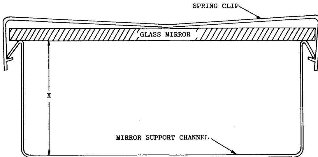
Figure 12. Sketch of Mirror Position.
