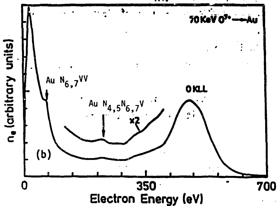
Fig. 16. Measured electron energy distribution for 70 keV O^{7+} incident on a clean Au surface at 5°.
