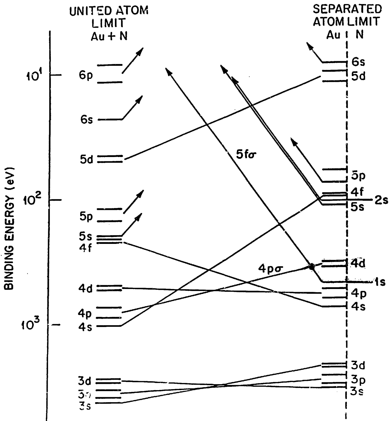
Fig. 17. N-Au correlation diagram, showing the pathway for vacancy transfer from the 1s shell of N to the 4d shell of Au.
