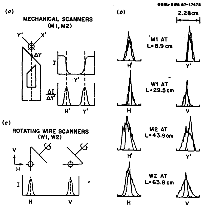
Fig. 8. Sample beam overlap scans along merge path.
