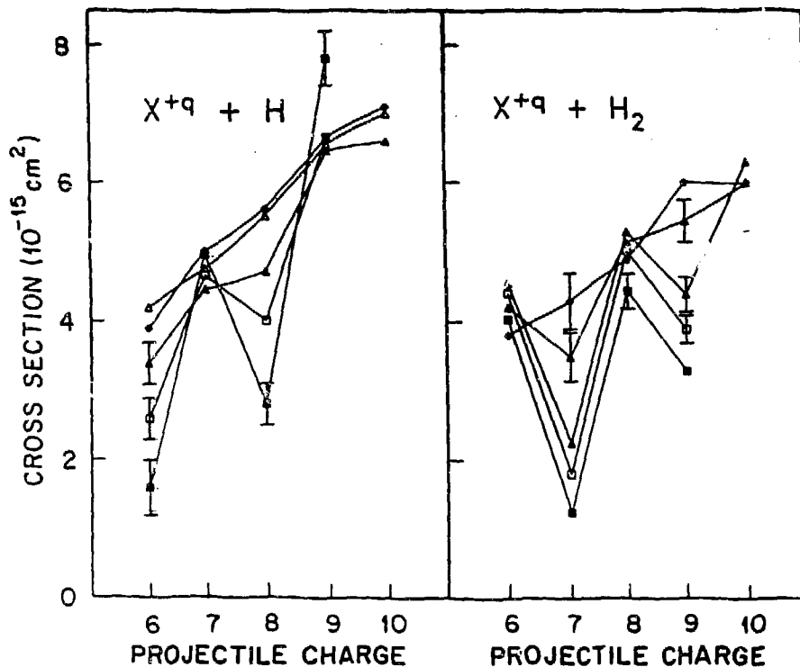
Charge dependence of experimental total electron capture cross sections for fully stripped projectiles ( 6 \leq Z \leq 10 ) incident on H and H_2 . ■ - 0.3 keV/amu; □ - 0.6 keV/amu; ▲ - 1.0 keV/amu; △ - 3.0 keV/amu; ◆ - 8.0 keV/amu. A few representative error bars are indicated.
