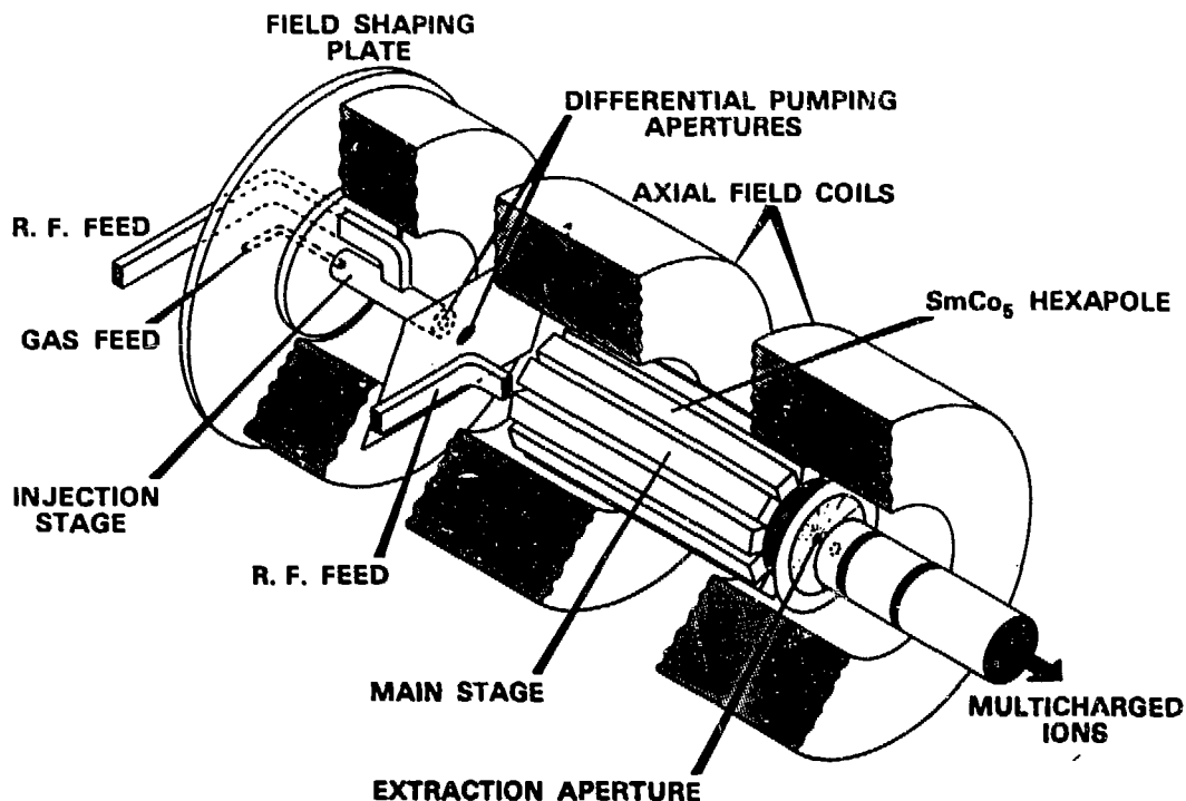
Fig. 1. Cutaway drawing of the ORNL ECR source.
