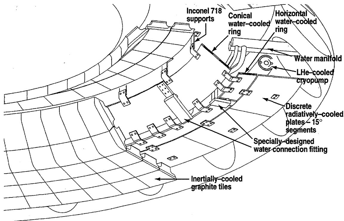
Fig. 1. Primary components of the Phase 1A Radiative Divertor.
