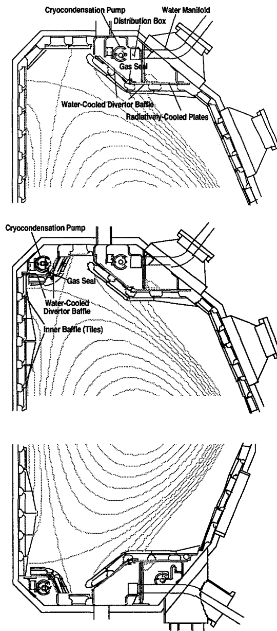
Fig. 4. Phased approach to the RDP installation. (a) Phase 1A installed 1997, (b) Phase 1B adds private flux baffle, and (c) Phase 1C adds inner and outer lower baffle structures.
