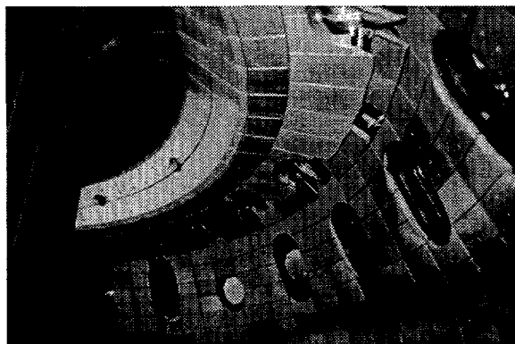
Fig. 2. Completed installation of Phase 1A RDP in upper outer corner of DIII-D.
