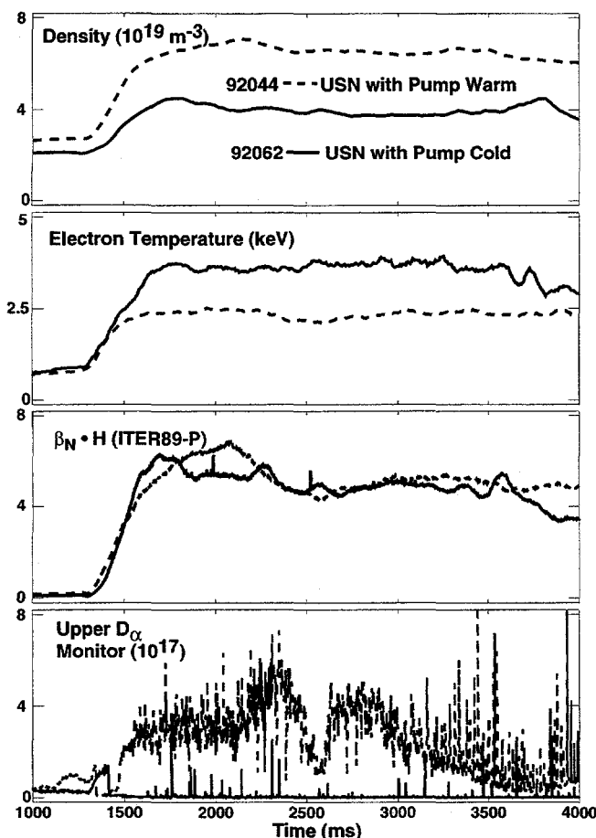
Fig. 3. Initial results showing density control and recycling reduction with no change in normalized confinement with the upper divertor pump (solid-pump cold, dashed-warm).
