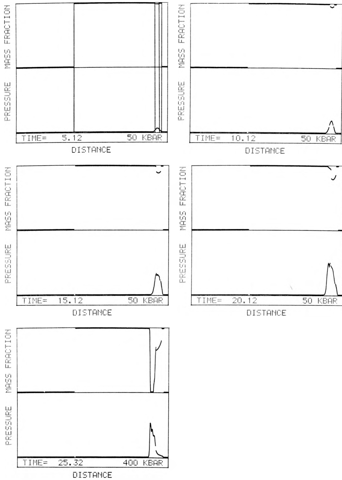
Fig. 4c One-dimensional cylindrically symmetric calculation with a 2.6-cm-thick porous bed and with (S/V)_0 = 120/\text{cm} .
