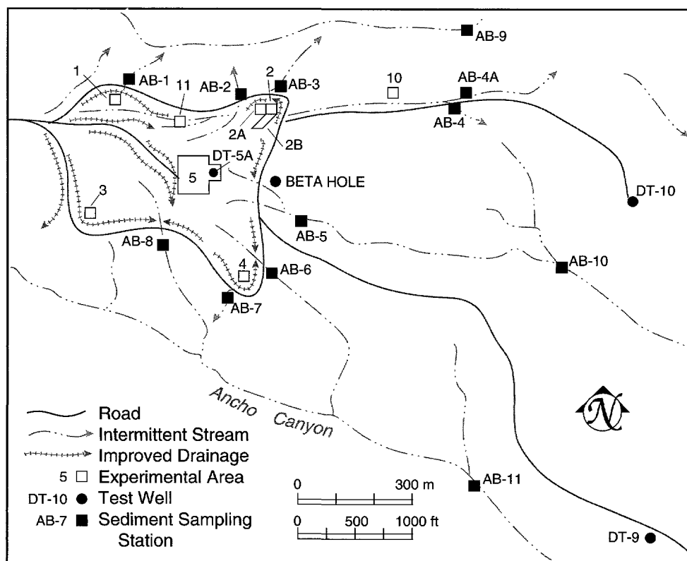
Figure 5-5. Sediment sampling stations at solid waste management areas.
