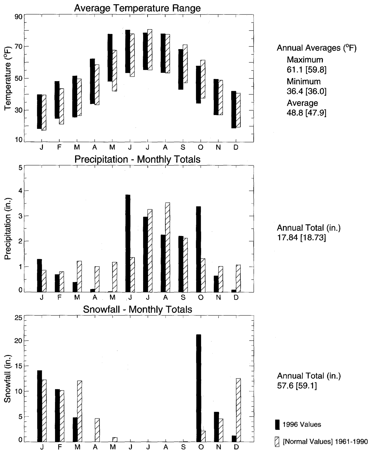
Figure 4-15. 1996 weather summary for Los Alamos (TA-6 station, elevation 7,424 ft.).
