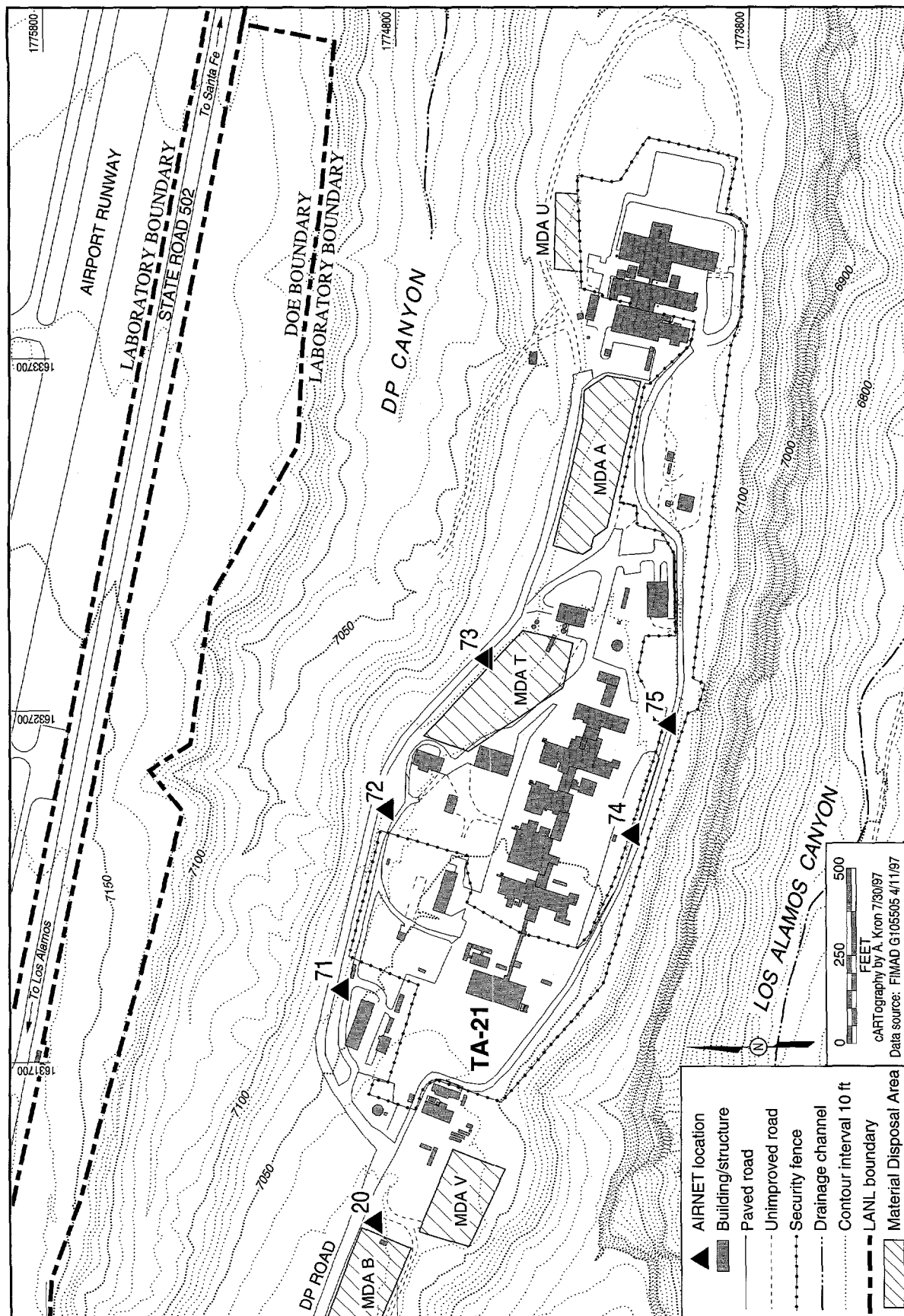
Figure 4-3. Technical Area 21 map of AIRNET locations.
