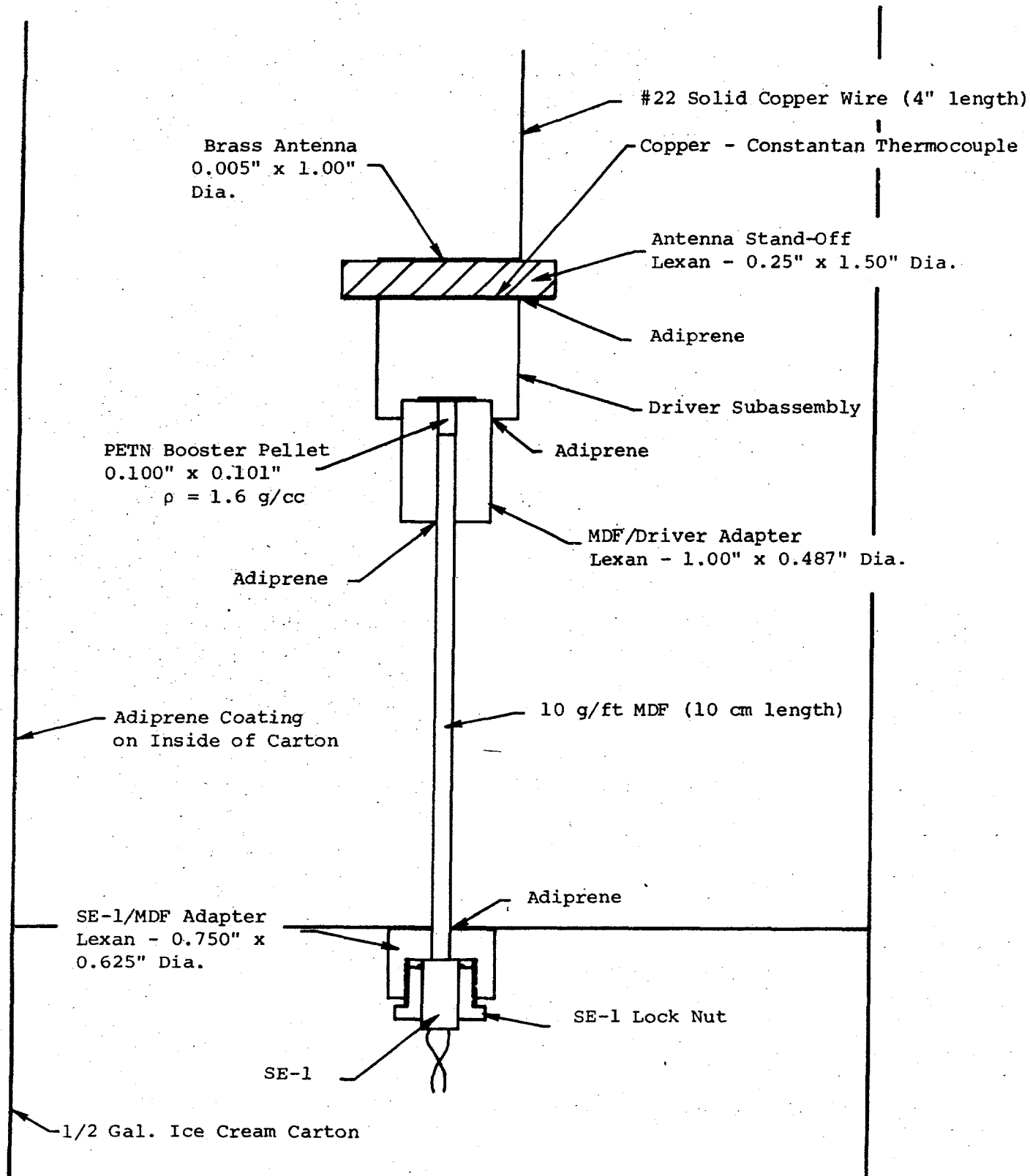
Fig. 2. Test Fire Assembly
