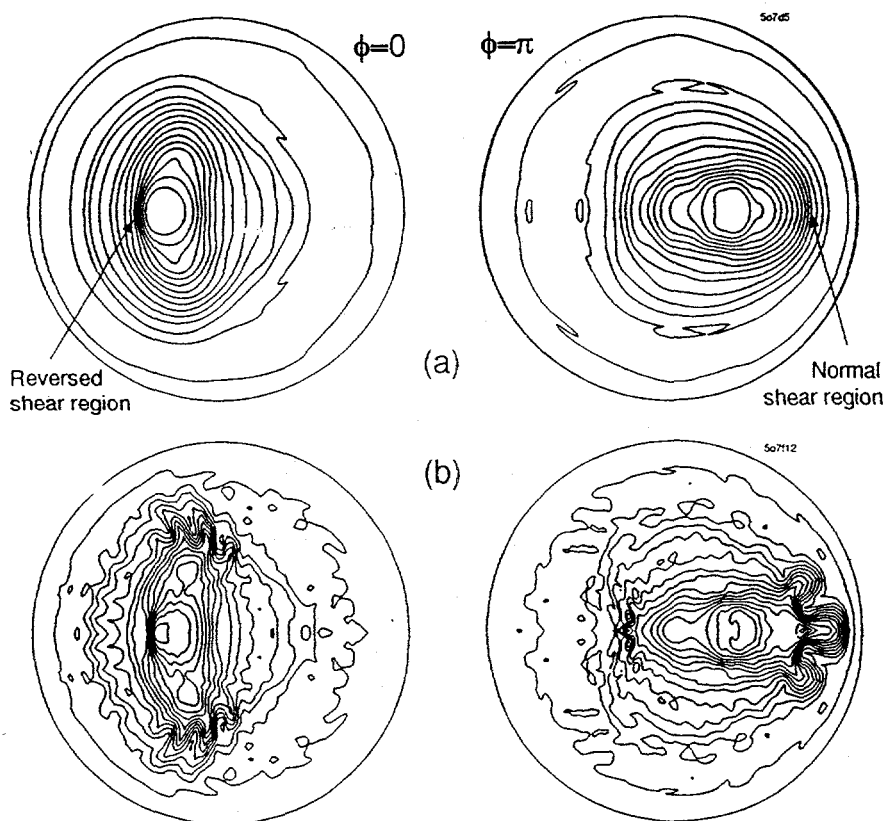
Figure 1: (a) Pressure contours of the 3D equilibrium. Two local pressure steepenings occur; the stronger one inside the reversed shear core region at \phi = 0 , and the other in the normal shear region at \phi = \pi . (b) The later nonlinear development of the pressure. The localized high- n ballooning mode develops only from the pressure steepening in the normal shear region.
