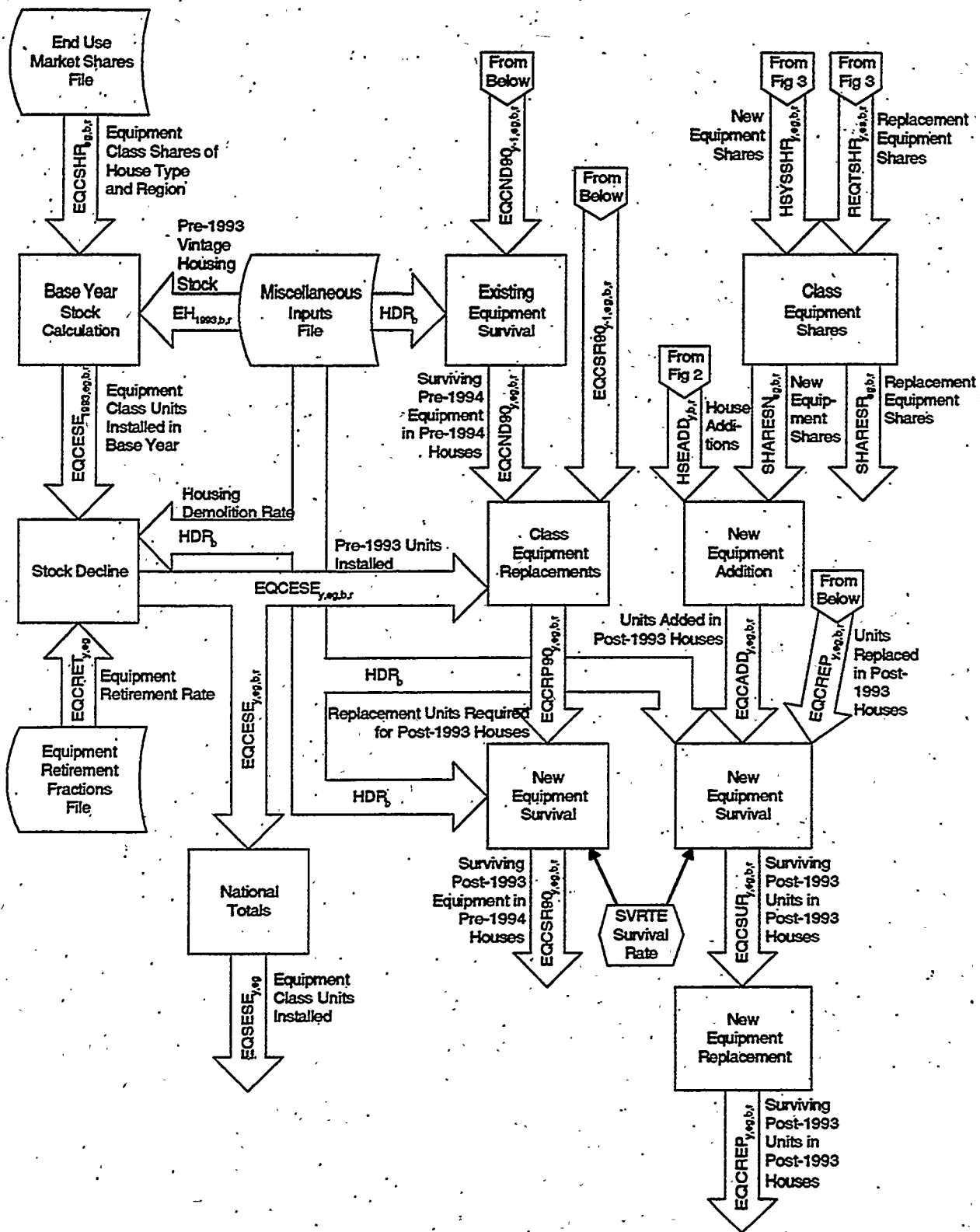
Figure 4. Appliance Stock Component Flow.
