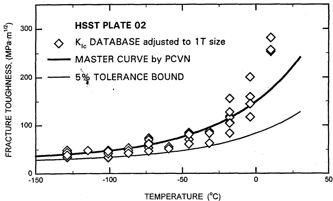
FIG. 1--Comparison of the HSST Plate 02 linear-elastic K_{Ic} database relative to the master curve with 5 % margin-adjusted tolerance bound curve derived by testing of several PCVN specimens.
