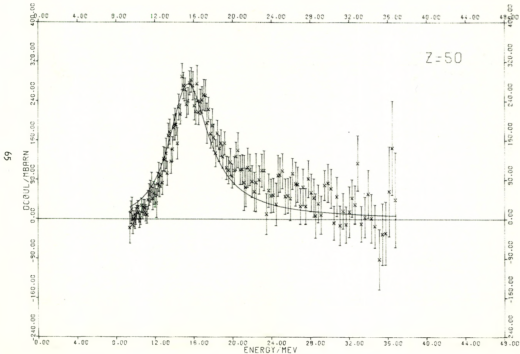
Figure 26 Total nuclear photoabsorption cross section, \sigma_{\text{nuc1}}(k) for tin in the giant resonance region. The curve gives the (\gamma, n) cross section [29]. The error bars indicate one standard deviation of the statistical error.
