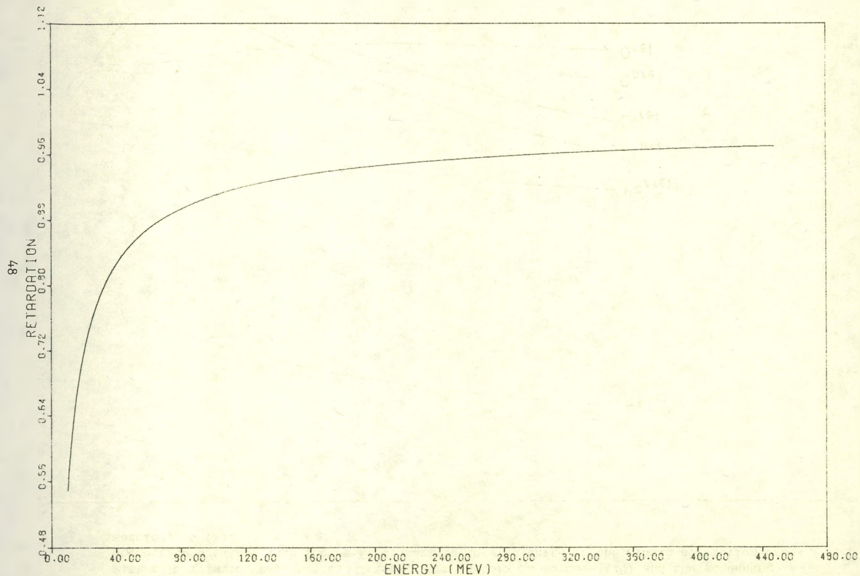
Figure 9 Retardation factor, f_{\text{ret}} , for triplet production derived from formula (40).
