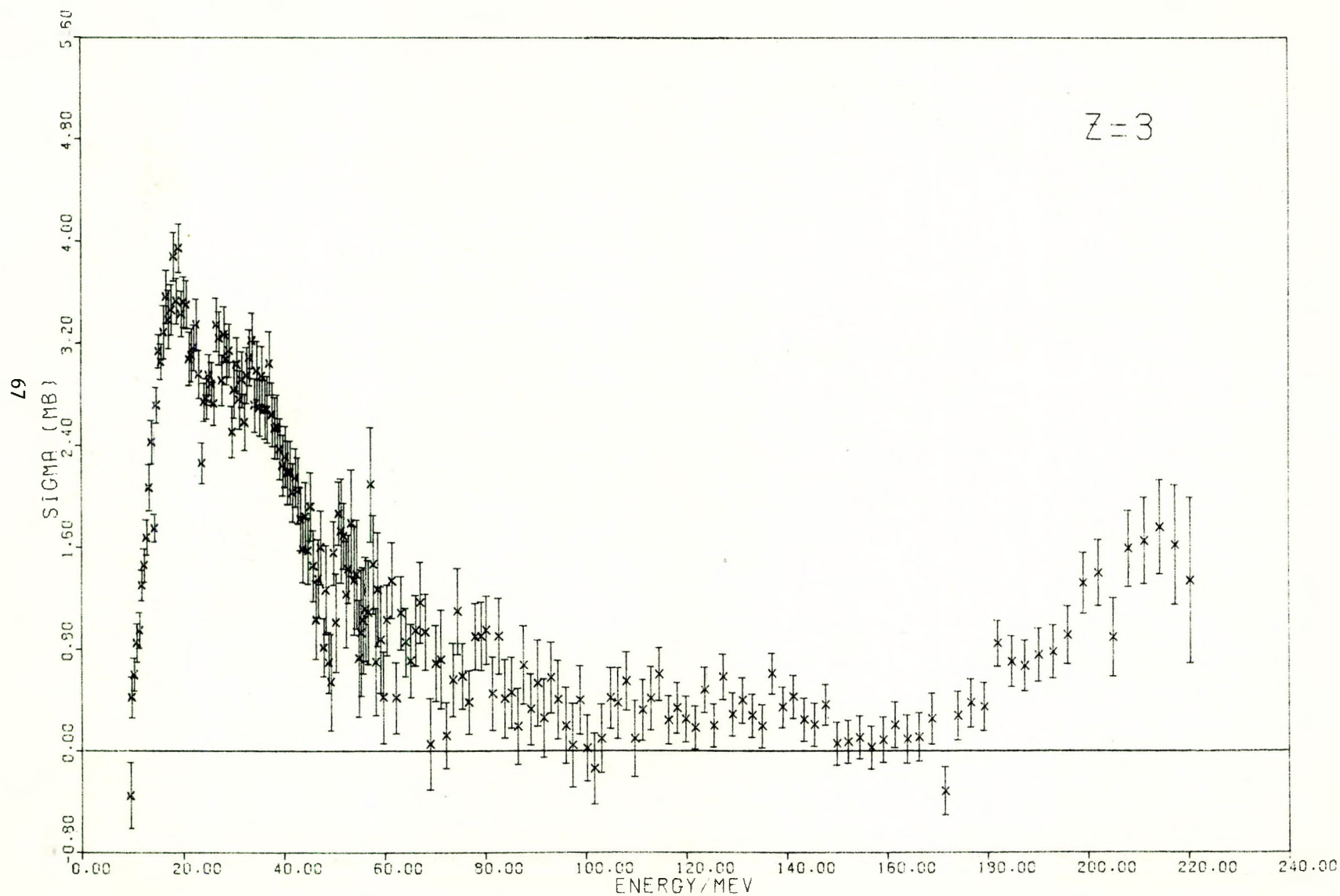
Figure 28 Total nuclear photoabsorption cross section, \sigma_{\text{nucl}}(k) for lithium (obtained from equation (1)). The error flags indicate the statistical errors of the experimental points.
