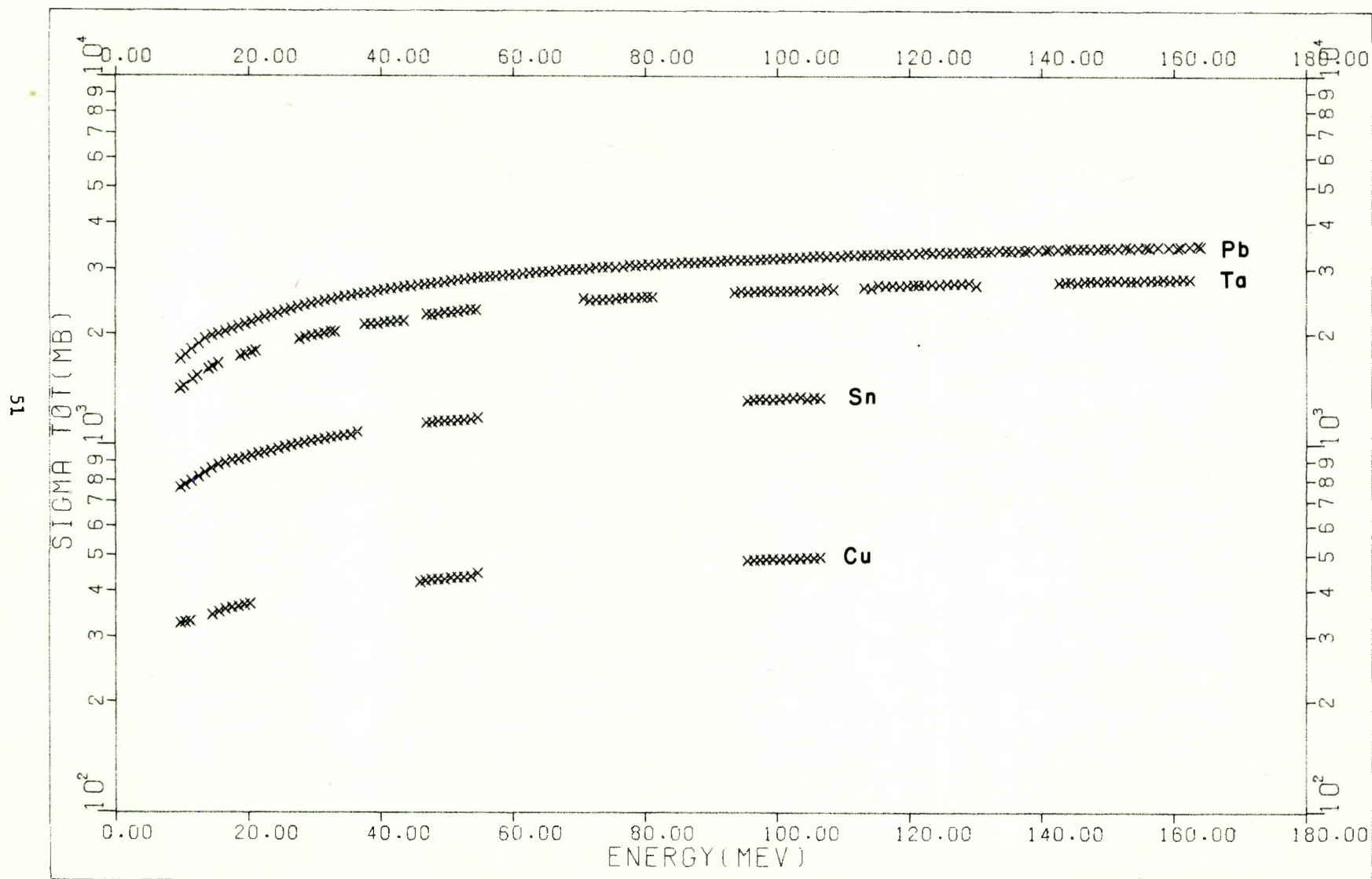
Figure 12 Measured total absorption cross sections, \sigma_{\text{tot}}(k) , for Cu, Sn, Ta and Pb. The statistical errors are smaller than the displayed points.
