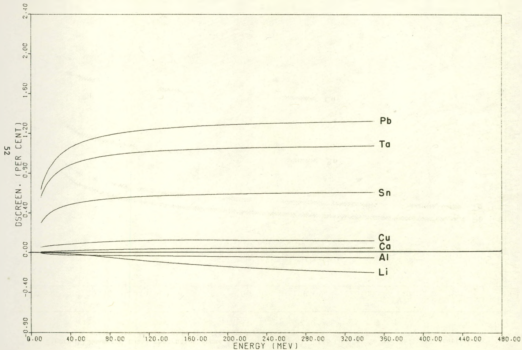
Figure 13 Difference of the screening correction for pair production in the nuclear Coulomb field obtained with relativistic form factors in equation (20) and the screening correction obtained with nonrelativistic form factors in units of the atomic cross section, \sigma_a(k) .
