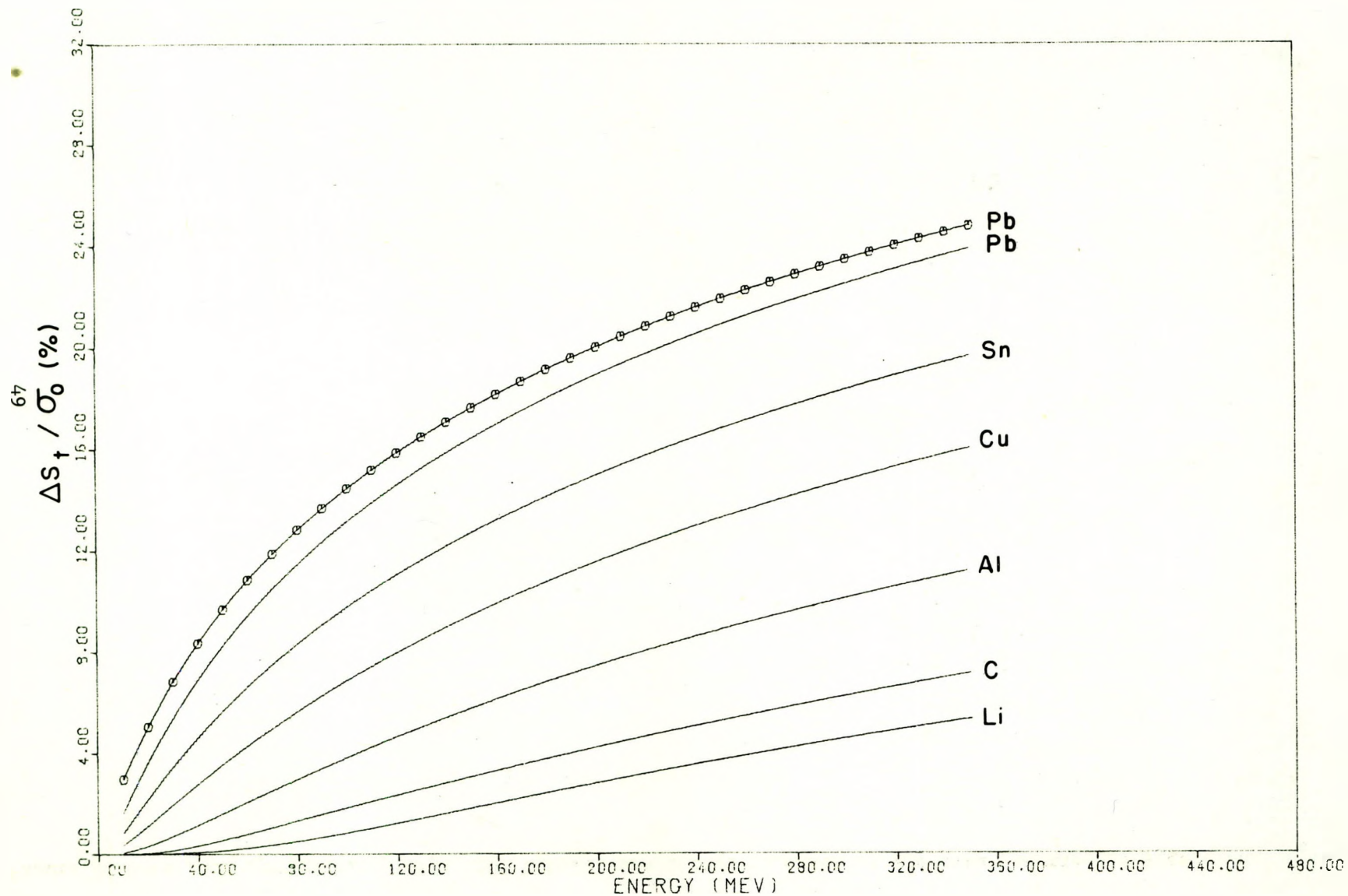
Figure 10 Screening correction, \Delta S_t , for triplet production in units of the unscreened triplet cross section, \sigma_0(k) . The circles indicate the screening correction for lead if retardation is neglected.
