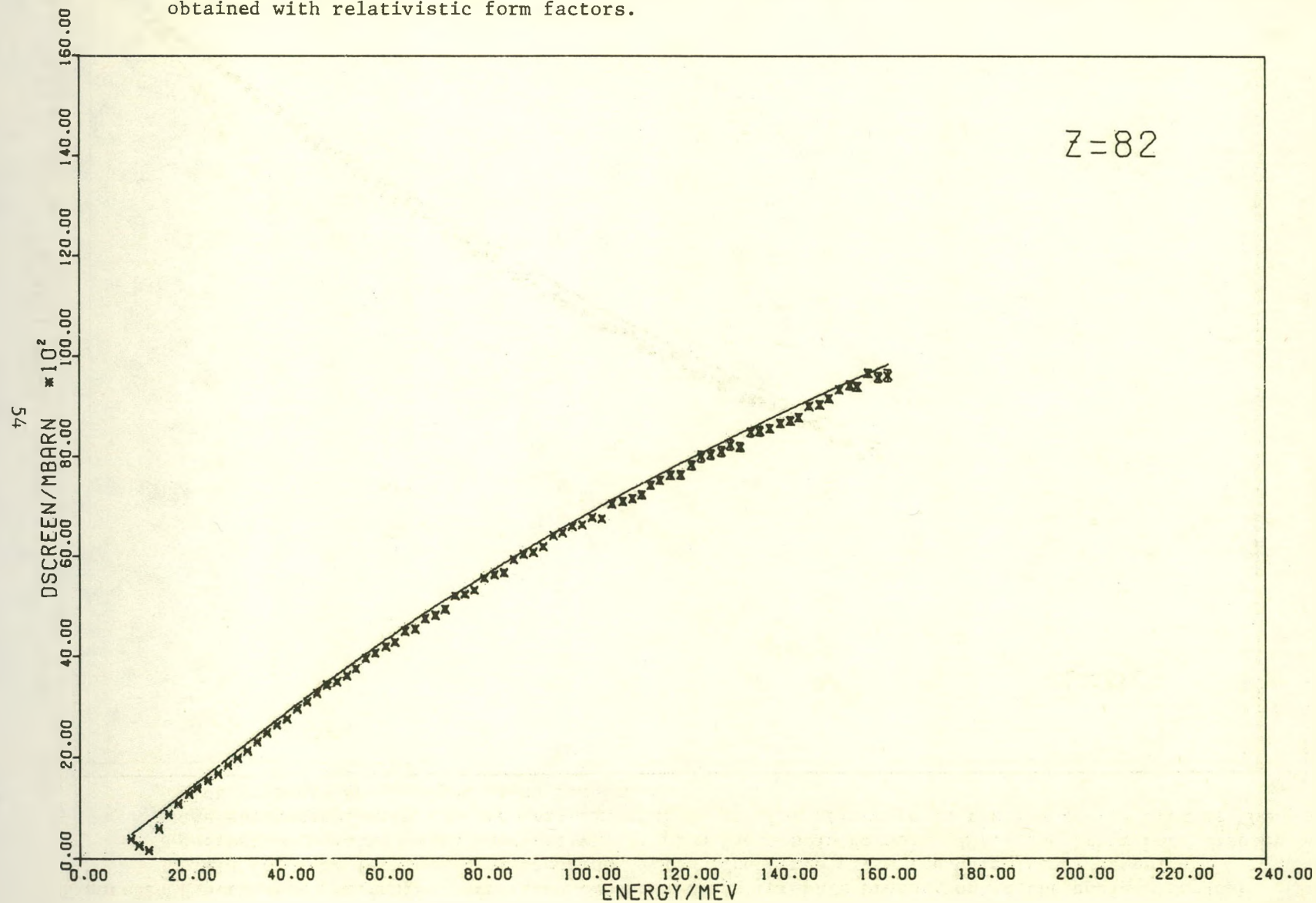
Figure 15 Experimental screening correction cross sections for pair production in the nuclear Coulomb field for lead (derived from equation (42)). The curve gives the calculated screening correction obtained with relativistic form factors.
