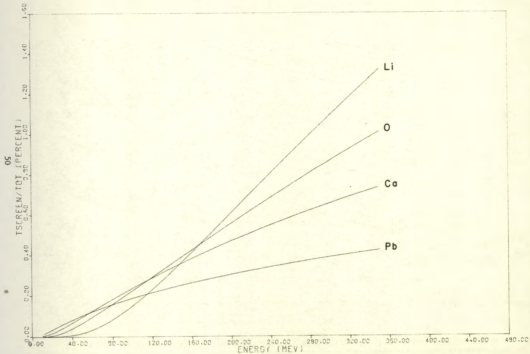
Figure 11 Screening correction, \Delta S_t , for triplet production in units of the total atomic cross section, \sigma_a(k) .
