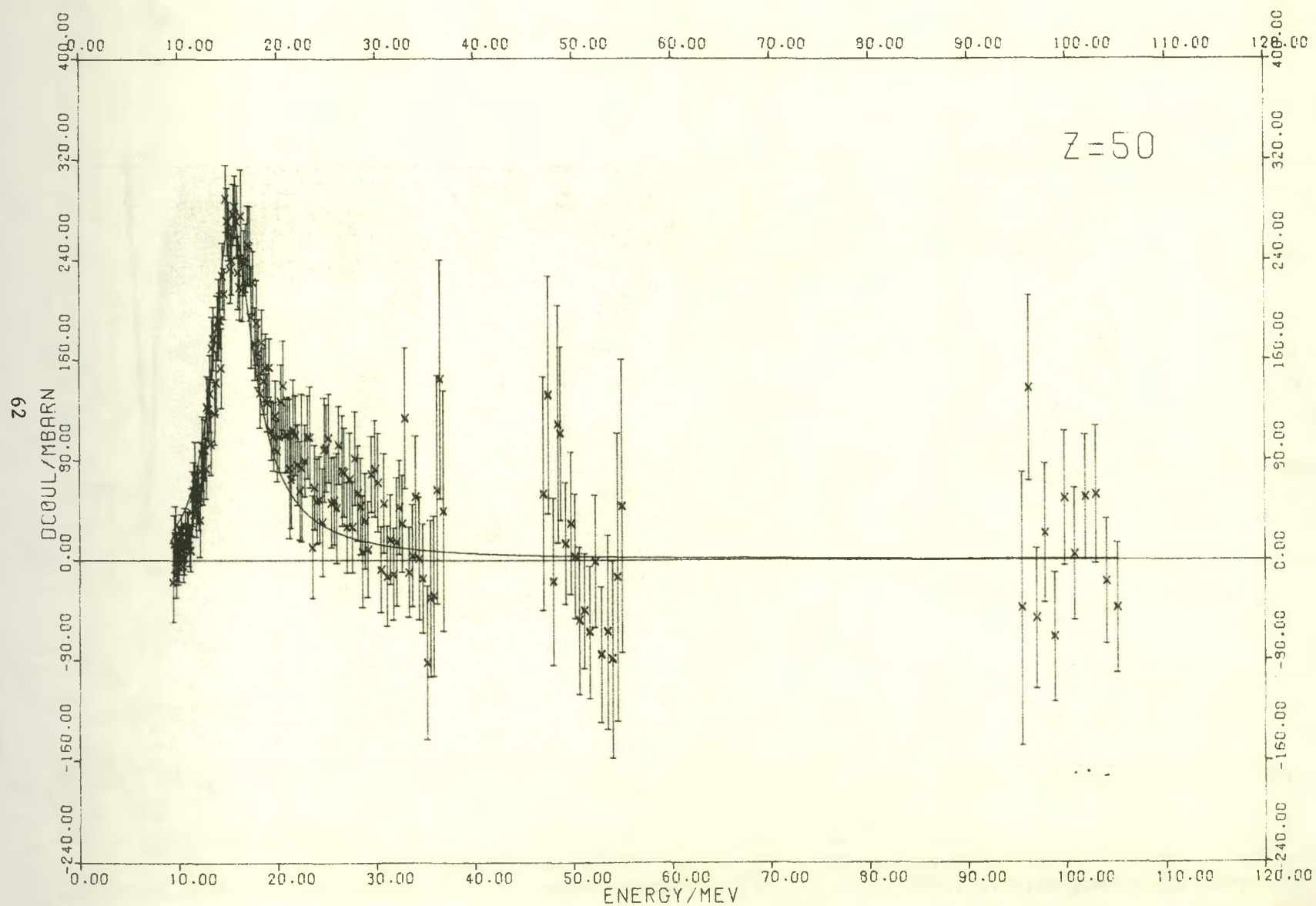
Figure 23 Total nuclear photoabsorption cross section, \sigma_{\text{nucl}}(k) , for tin (obtained from equation (1)). The error flags indicate the statistical errors of the experimental points.
