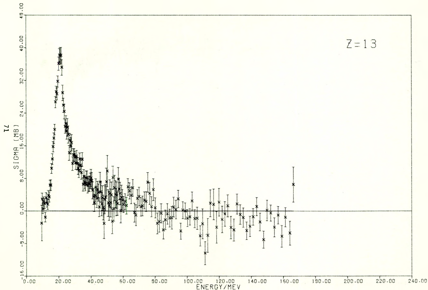
Figure 32 Total nuclear photoabsorption cross section, \sigma_{\text{nucl}}(k) for aluminum (obtained from equation (1)). The error flags indicate the statistical errors of the experimental points.
