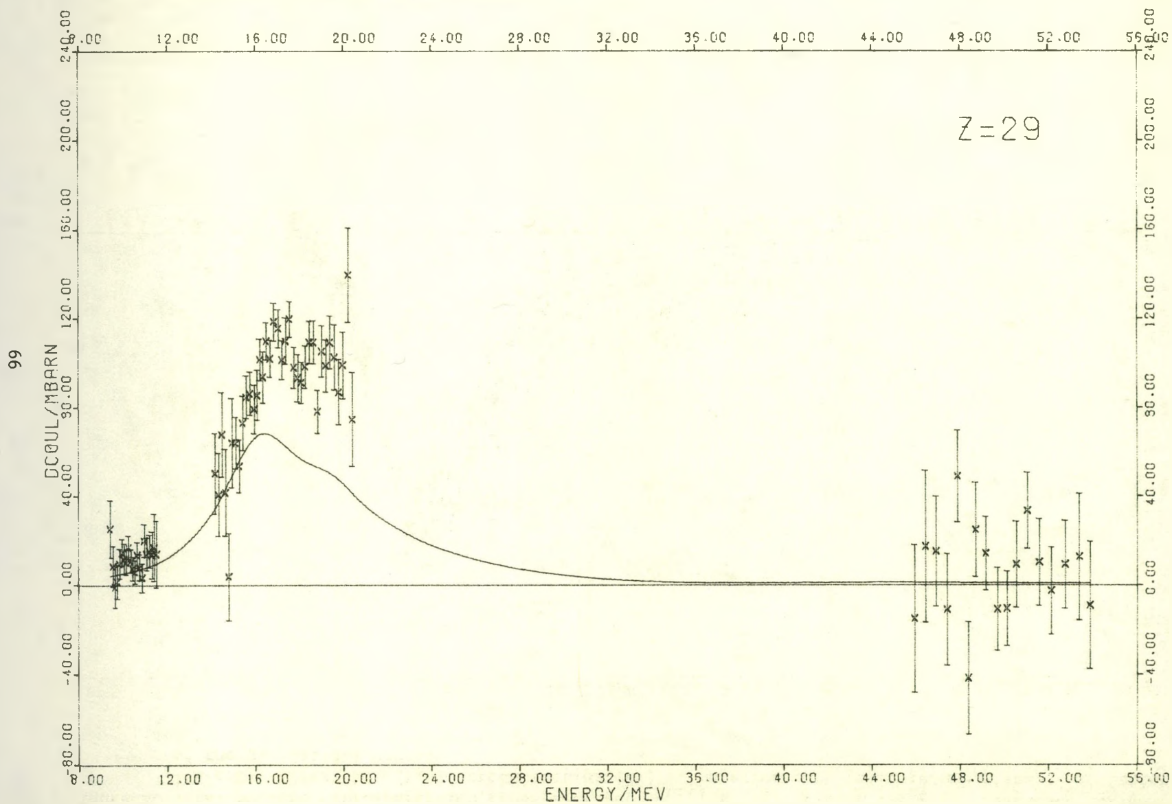
Figure 27 Total nuclear photoabsorption cross section, \sigma_{\text{nuc1}}(k) for copper in the giant resonance region. The curve gives the (\gamma, n) cross section [29]. The error bars indicate one standard deviation of the statistical error.
