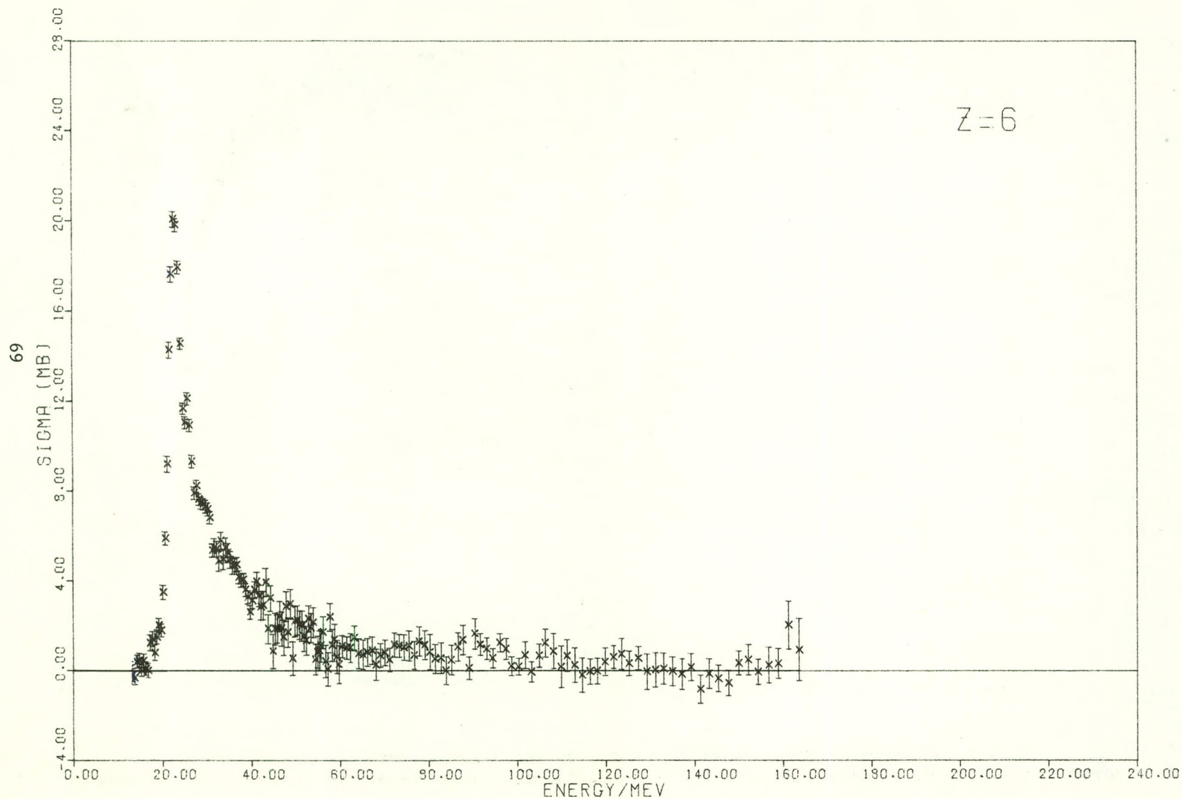
Figure 30 Total nuclear photoabsorption cross section, \sigma_{\text{nucl}}(k) for carbon (obtained from equation (1)). The error flags indicate the statistical errors of the experimental points.
