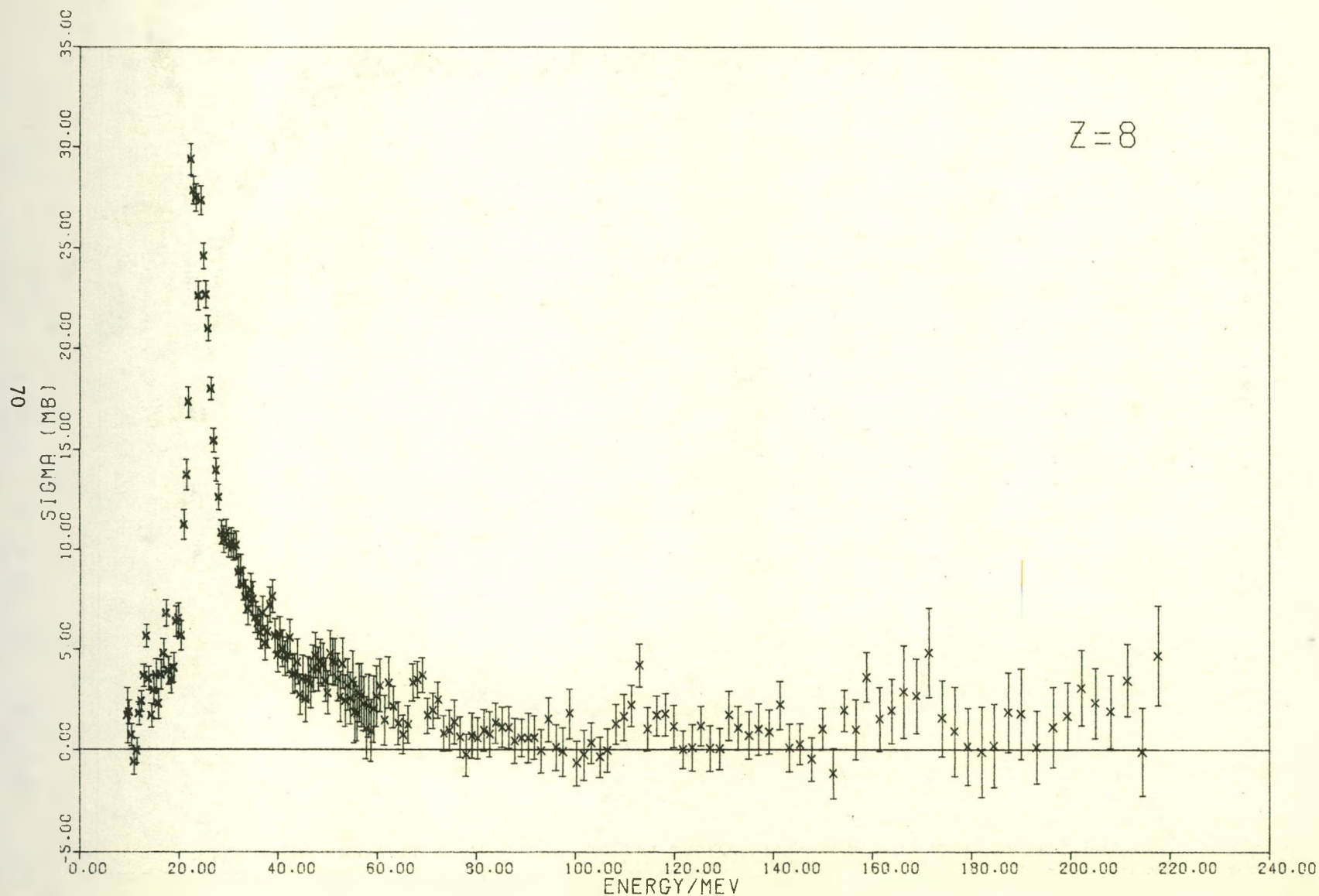
Figure 31 Total nuclear photoabsorption cross section, \sigma_{\text{nuc1}}(k) for oxygen (obtained from equation (1)). The error flags indicate the statistical errors of the experimental points.
