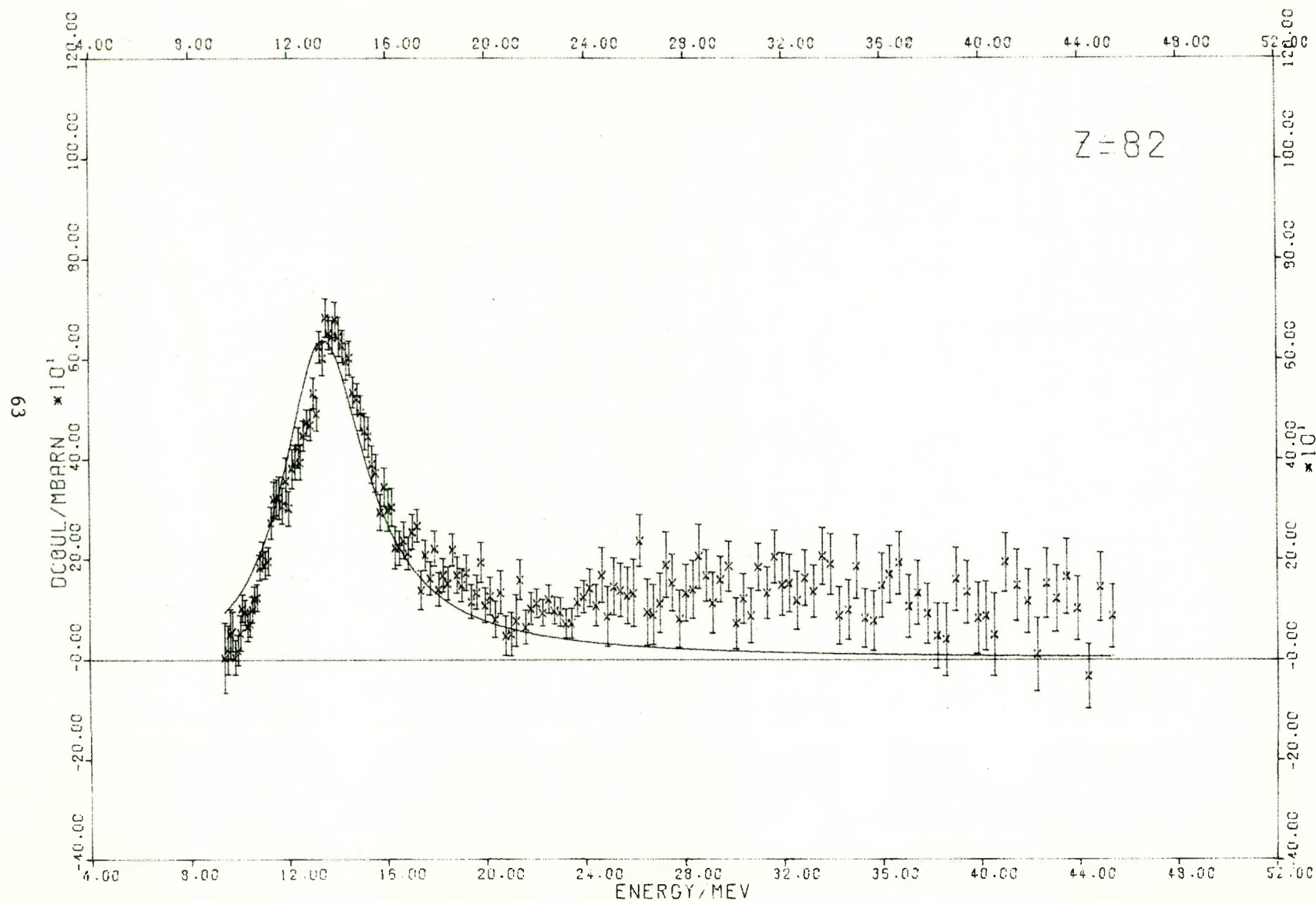
Figure 24 Total nuclear photoabsorption cross section, \sigma_{\text{nuc1}}(k) for lead in the giant resonance region. The curve gives the (\gamma, n) cross section [29]. The error bars indicate one standard deviation of the statistical error.
