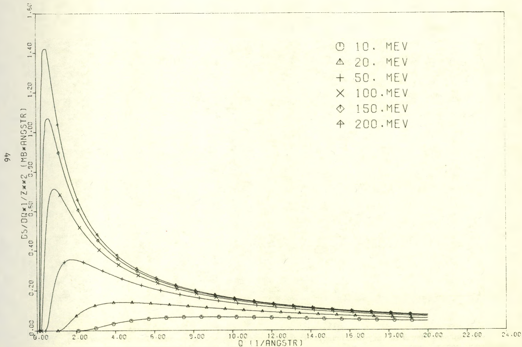
Figure 7 Recoil distribution, \frac{d\sigma}{dq}(k,q)/Z^2 , for pair production in the nuclear Coulomb field [14] (formula (21)).
