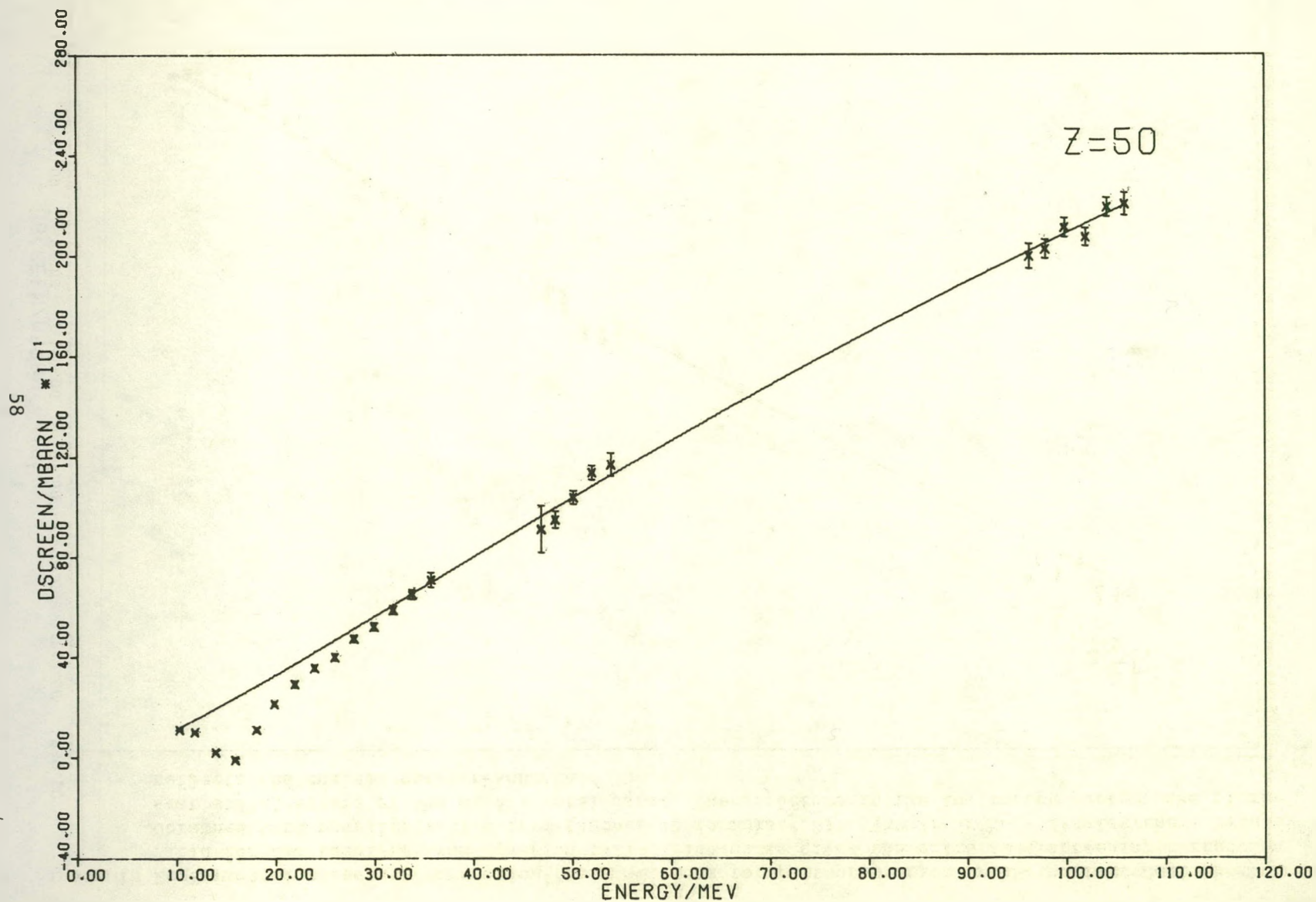
Figure 19 Experimental screening correction cross sections for pair production in the nuclear Coulomb field for tin (derived from equation (42)). The curve gives the calculated screening correction obtained with relativistic form factors.
