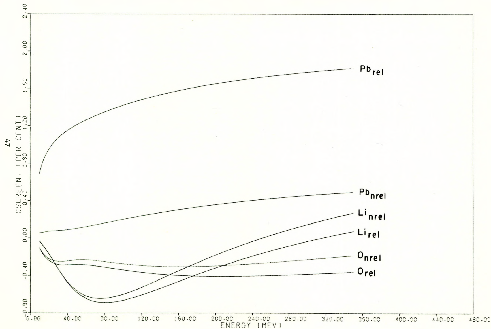
Figure 8 Difference between the screening correction for pair production in the nuclear field obtained with relativistic resp. nonrelativistic form factors in formula (20) and the screening correction obtained with Thomas-Fermi form factors in units of the atomic absorption cross section, \sigma_a(k) .
