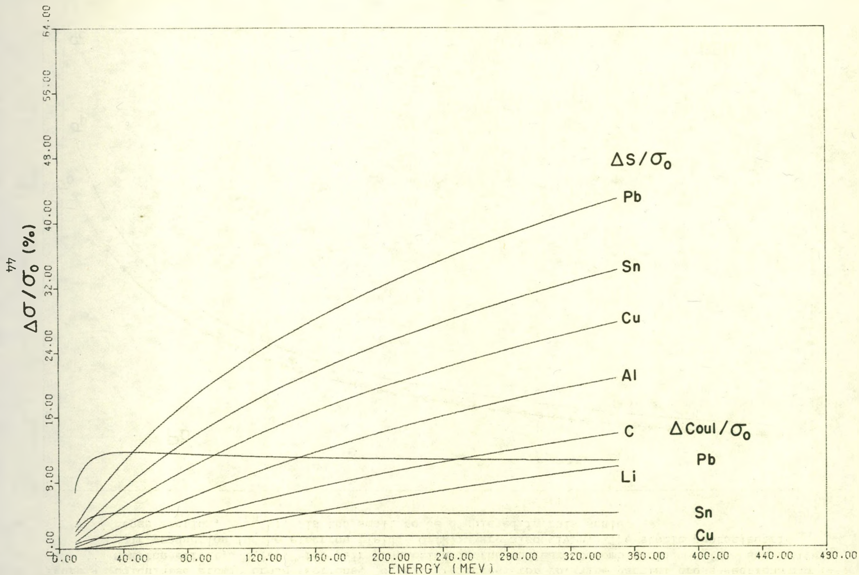
Figure 5 Screening corrections, \Delta S , and Coulomb corrections, \Delta \text{Coul} , for pair production in the nuclear Coulomb field in units of the atomic absorption cross section, \sigma_a(k) , for different elements.
