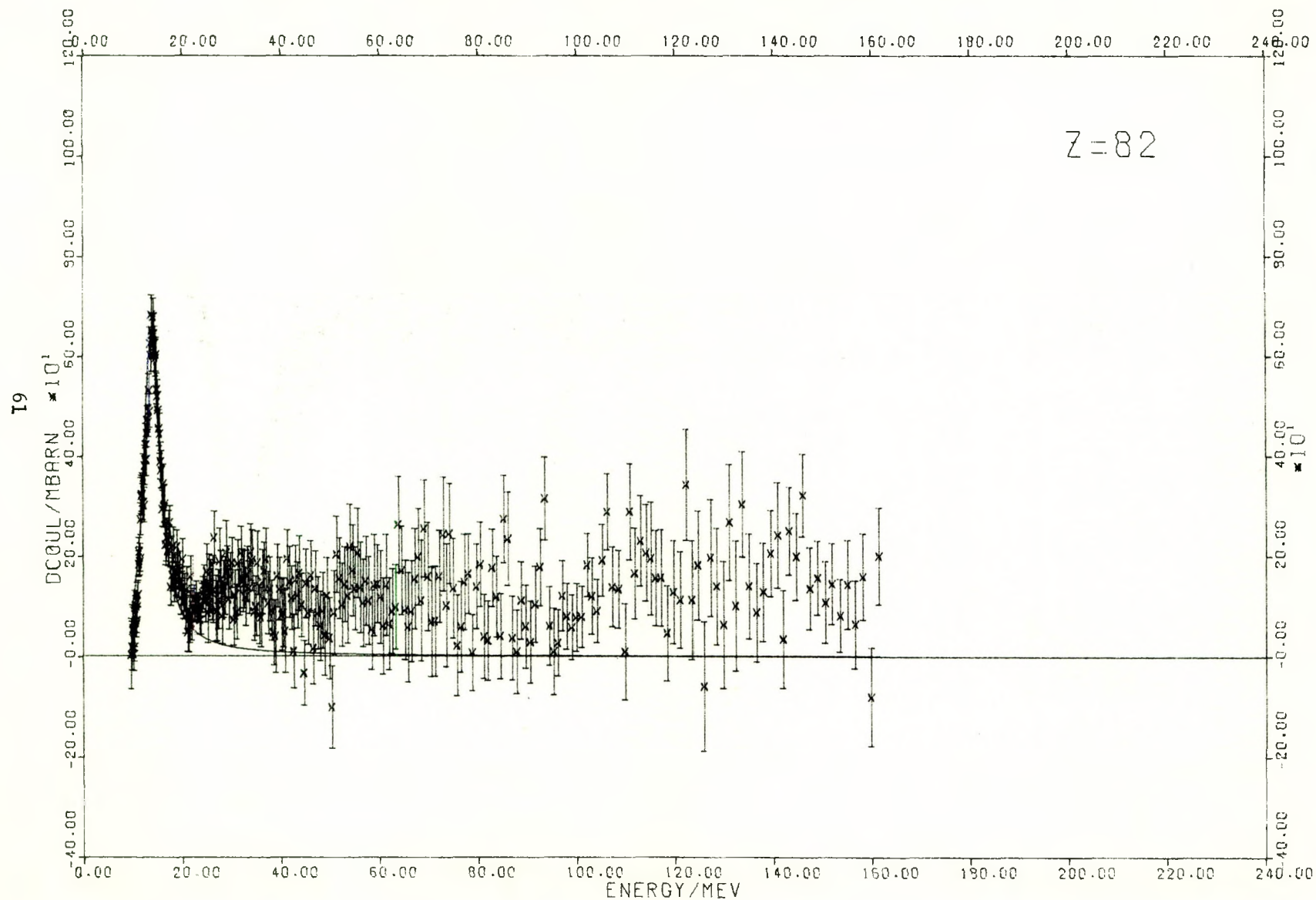
Figure 22 Total nuclear photoabsorption cross section, \sigma_{\text{nuc1}}(k) , for lead (obtained from equation (1)). The error flags indicate the statistical errors of the experimental points.
