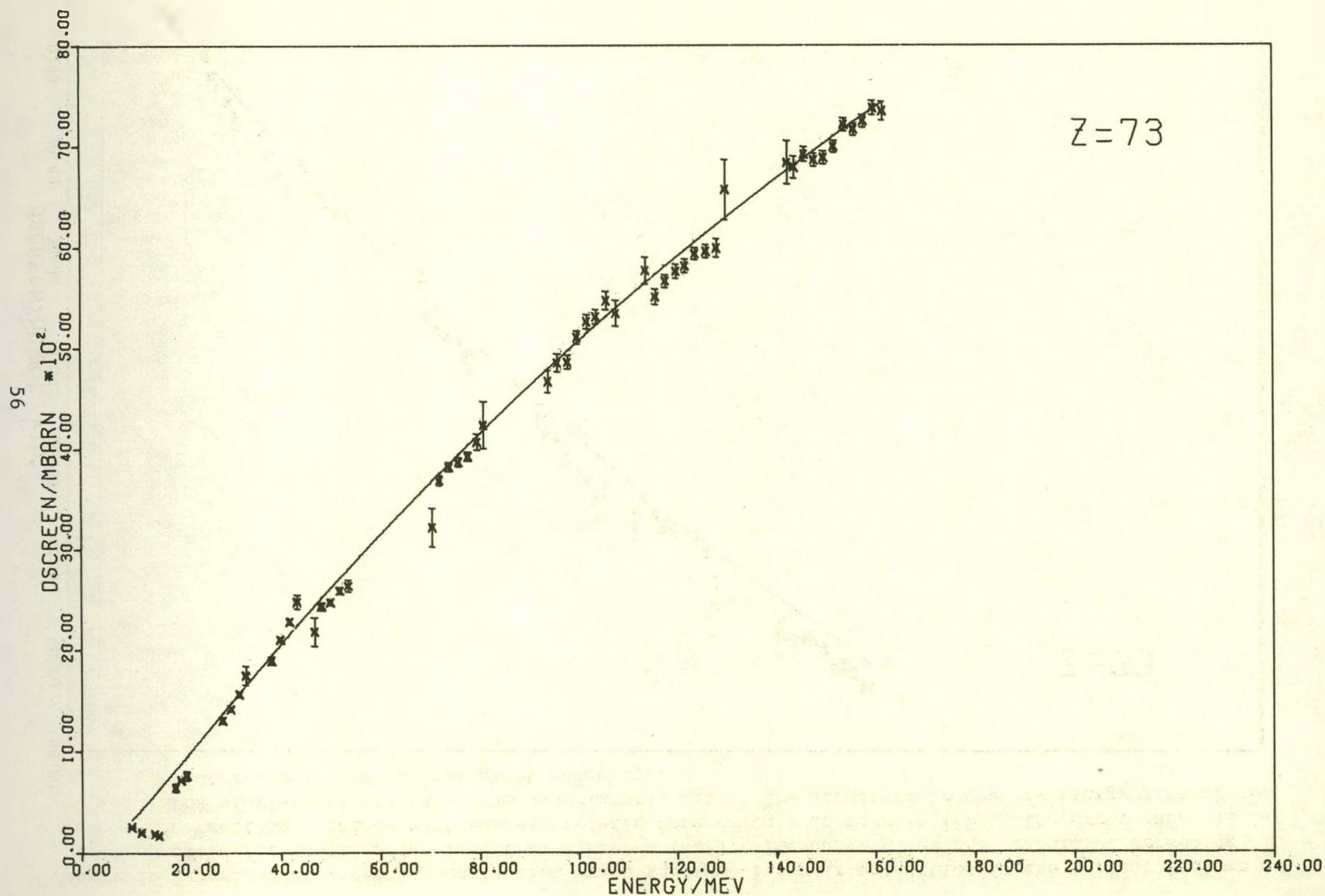
Figure 17 Experimental screening correction cross sections for pair production in the nuclear Coulomb field for tantalum (derived from equation (42)). The curve gives the calculated screening correction obtained with relativistic form factors.
