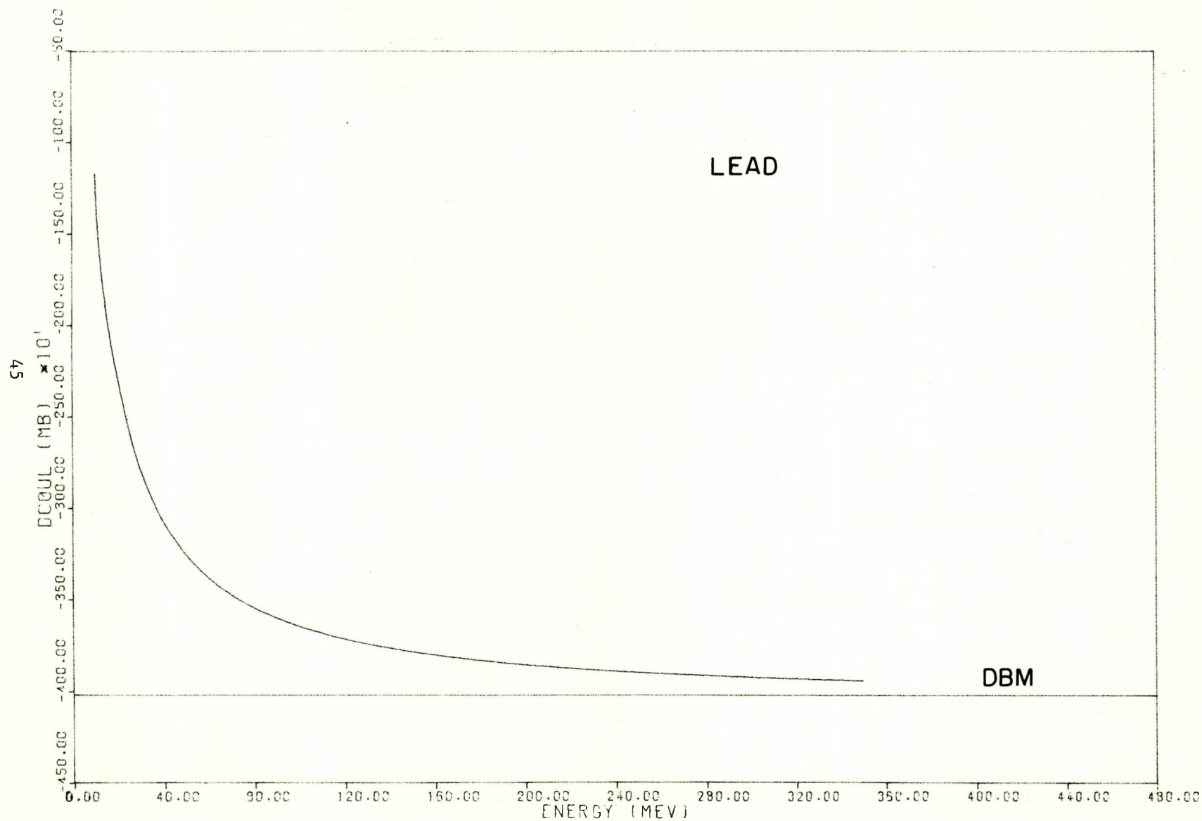
Figure 6 Coulomb correction cross section, \Delta_{\text{Coul}} , for pair production in the nuclear Coulomb field [12] for lead. The straight line (DBM) shows the energy independent value calculated by Davies, Bethe and Maximon [7].
