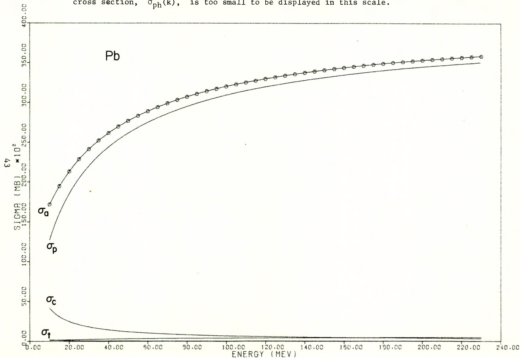
Figure 4 Calculated atomic cross sections, \sigma_a(k) , (circles) for Pb. The partial cross sections for Compton effect, \sigma_c(k) , for pair production in the nuclear Coulomb field, \sigma_p(k) and for pair production in the electron field, \sigma_t(k) , are also given. The atomic photoelectric cross section, \sigma_{ph}(k) , is too small to be displayed in this scale.
