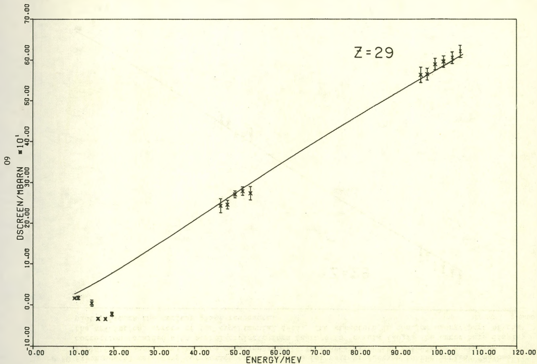
Figure 21 Experimental screening correction cross sections for pair production in the nuclear Coulomb field for copper (derived from equation (42)). The curve gives the calculated screening correction obtained with relativistic form factors.
