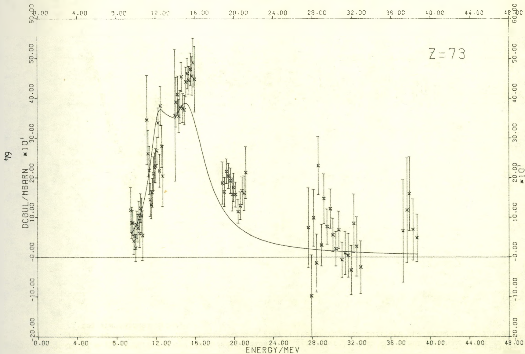
Figure 25 Total nuclear photoabsorption cross section, \sigma_{\text{nuc1}}(k) for tantalum in the giant resonance region. The curve gives the (\gamma, n) cross section [29]. The error bars indicate one standard deviation of the statistical error.
