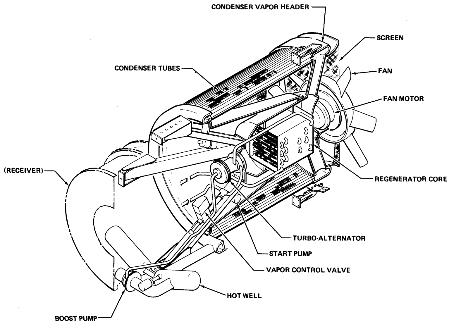
Figure 3-3. Power-Conversion Subsystem
