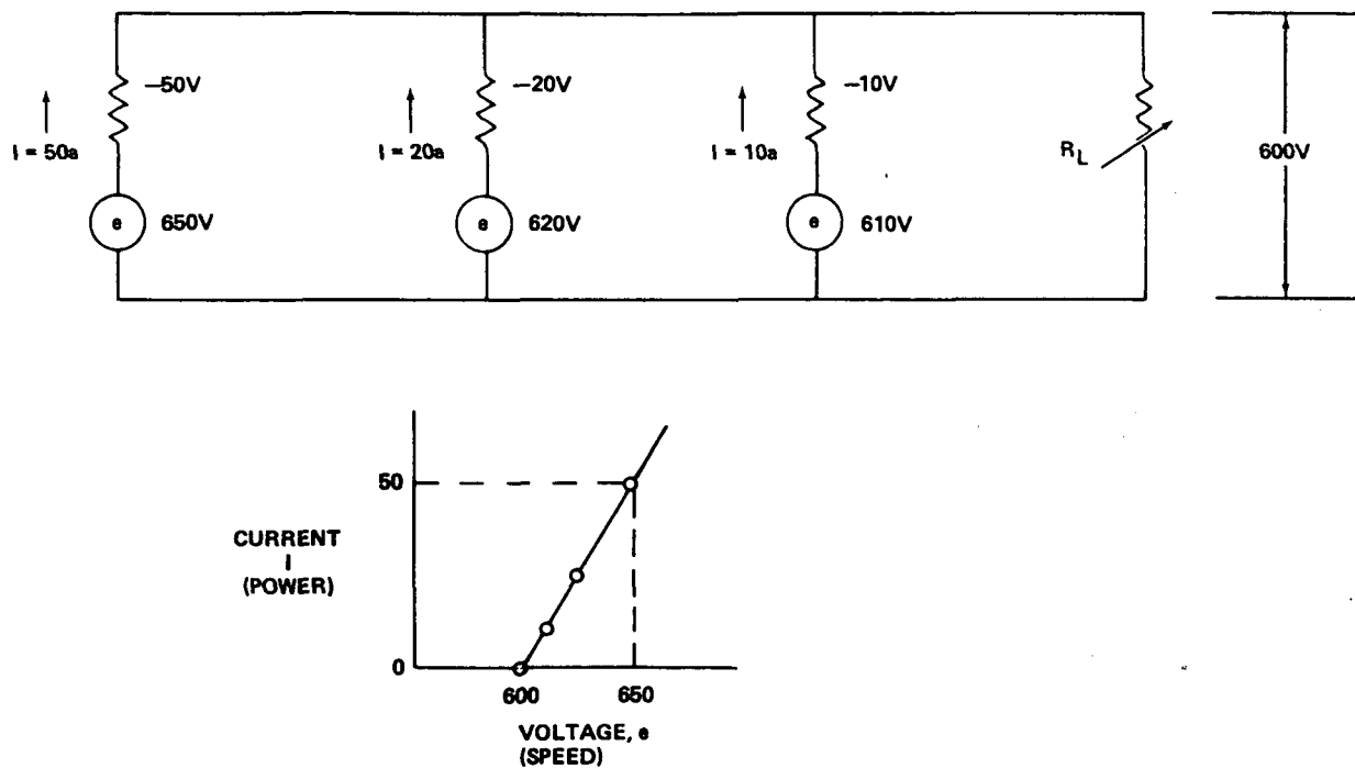
Figure 3-9. Effect of Variations in Current (or Power) Output for Alternators with Predetermined Internal Impedance Feeding a Variable Load that Maintains a Constant (600-V) Voltage Across Its Input.
