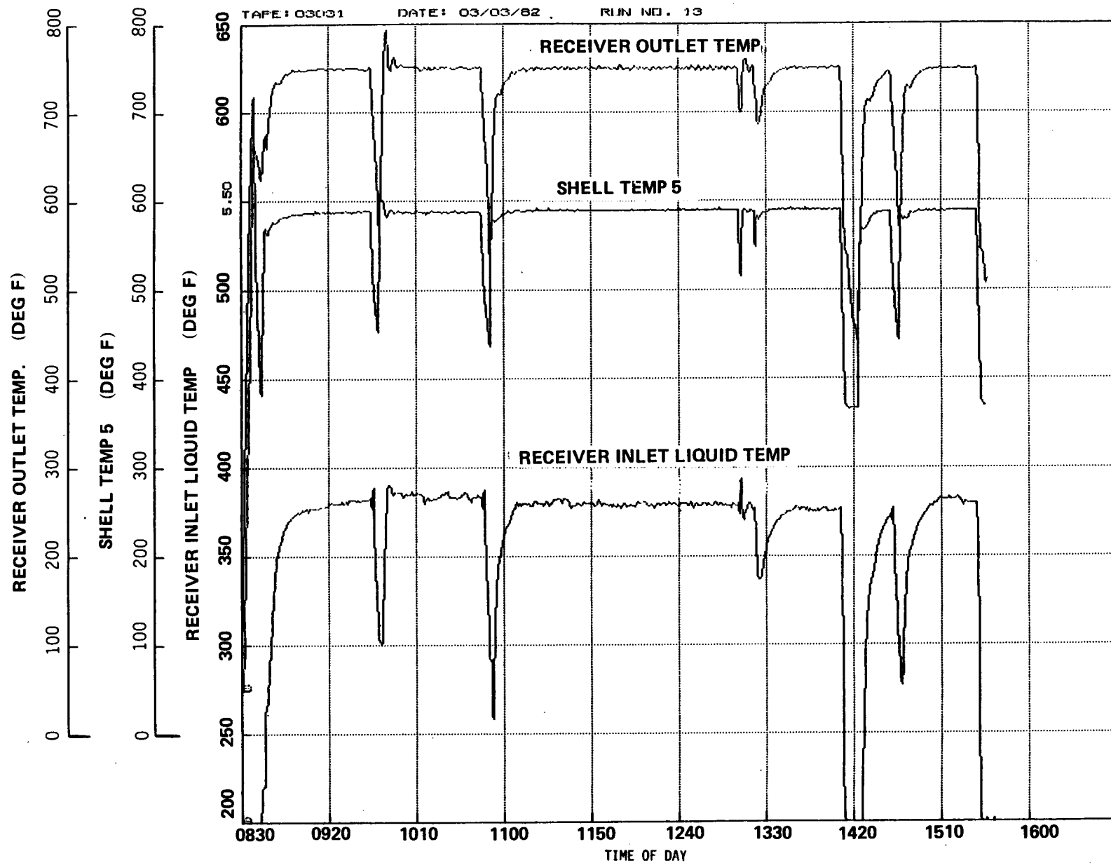
Figure 4-8. Receiver Temperatures for Run 13 (Test No. 8)
