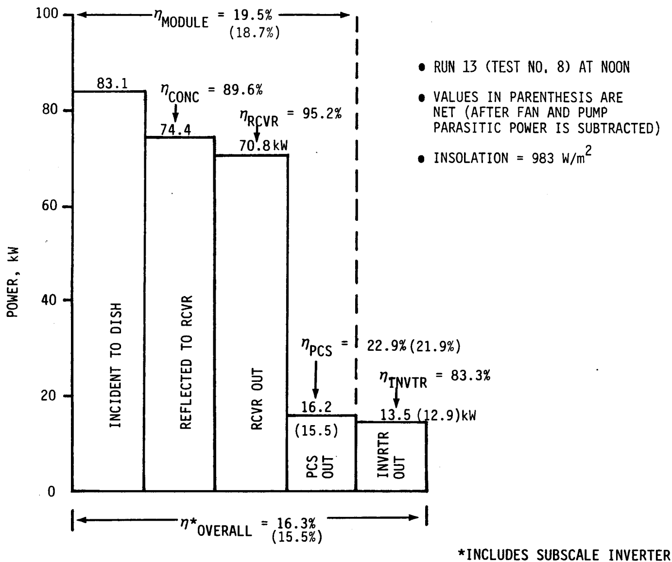
Figure 4-12. Measured Component, Module, and System Performance for a Typical Run
