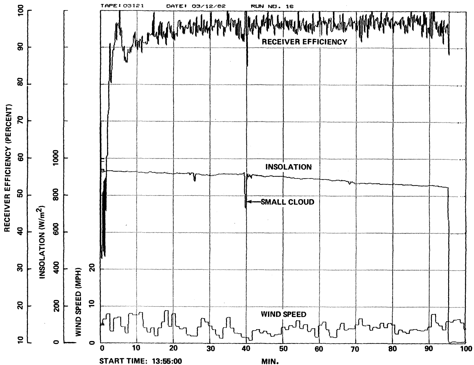
Figure 4-6. Typical Receiver Efficiency Plot (Run 16, Test No. 11)
