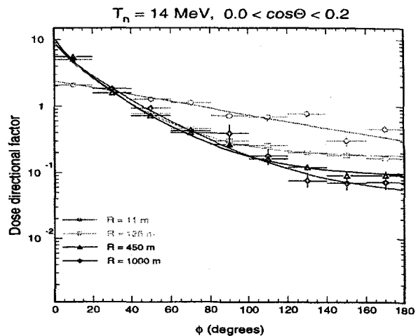
FIG. 9. Same as Fig. 8, but for the \cos(\Theta) = 0.1 interval.
