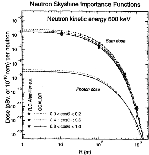
FIG. 3. Same as Fig. 2, but for the neutron kinetic energy interval 498 \text{ keV} < T_n < 743 \text{ keV} .
