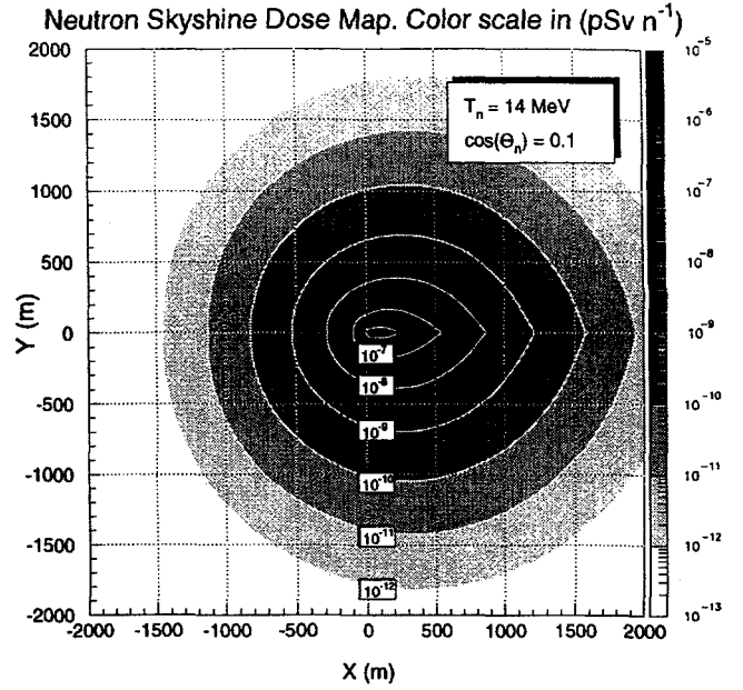
FIG. 12. Skyshine dose map calculated for the neutrons with fixed kinetic energy T_n = 14 MeV and \cos(\Theta) = 0.1 using the parameterization function SKYD. Neutron skyshine dose rate distribution around the source point is shown as a color (density) plot with lines of equal dose rate plotted as white contours. The logarithmic color scale for the dose rate is shown as the right scale in the figure; one step in color and the distance between neighboring lines of equal dose rate correspond to a factor of 10 in dose rate. The dose rate in pSv/n is indicated on the labels attached to the white contours.
