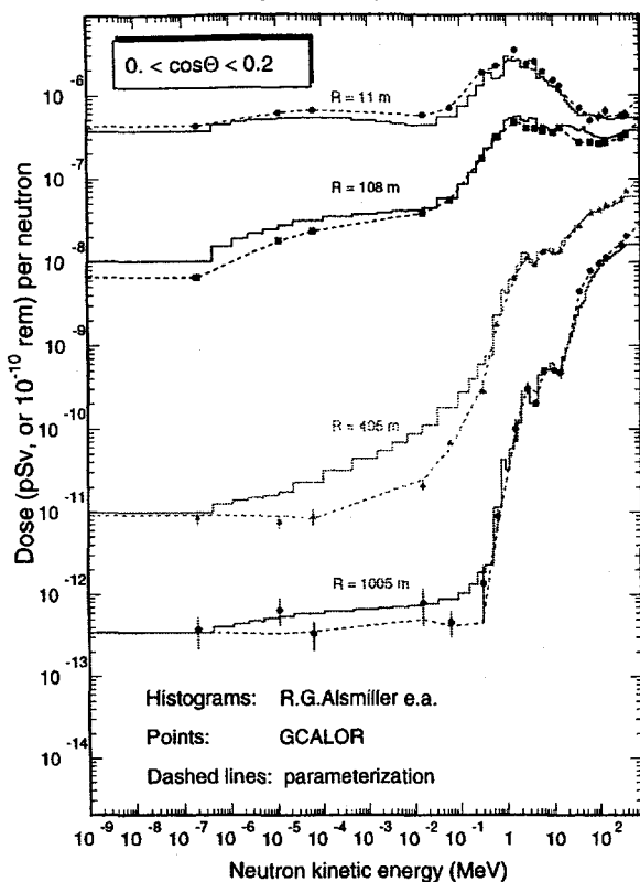
FIG. 7. Same as Fig. 6, but for the angular interval 78^\circ \lesssim \Theta < 90^\circ .
