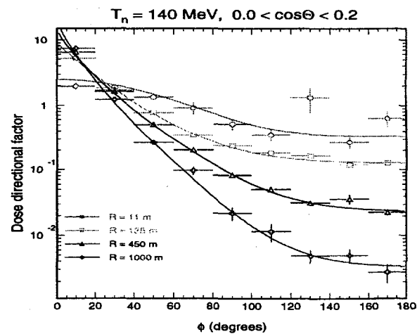
FIG. 11. Same as Fig. 10, but for the \cos(\Theta) = 0.1 interval.
