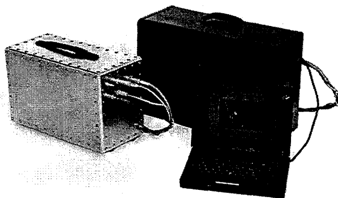
Figure 8. Photograph of portable system. Hermetically-sealed aluminum container, at left, houses detector vessel; detector window is at opposite end to cable connections. Contents of each container are shown in fig.2.
