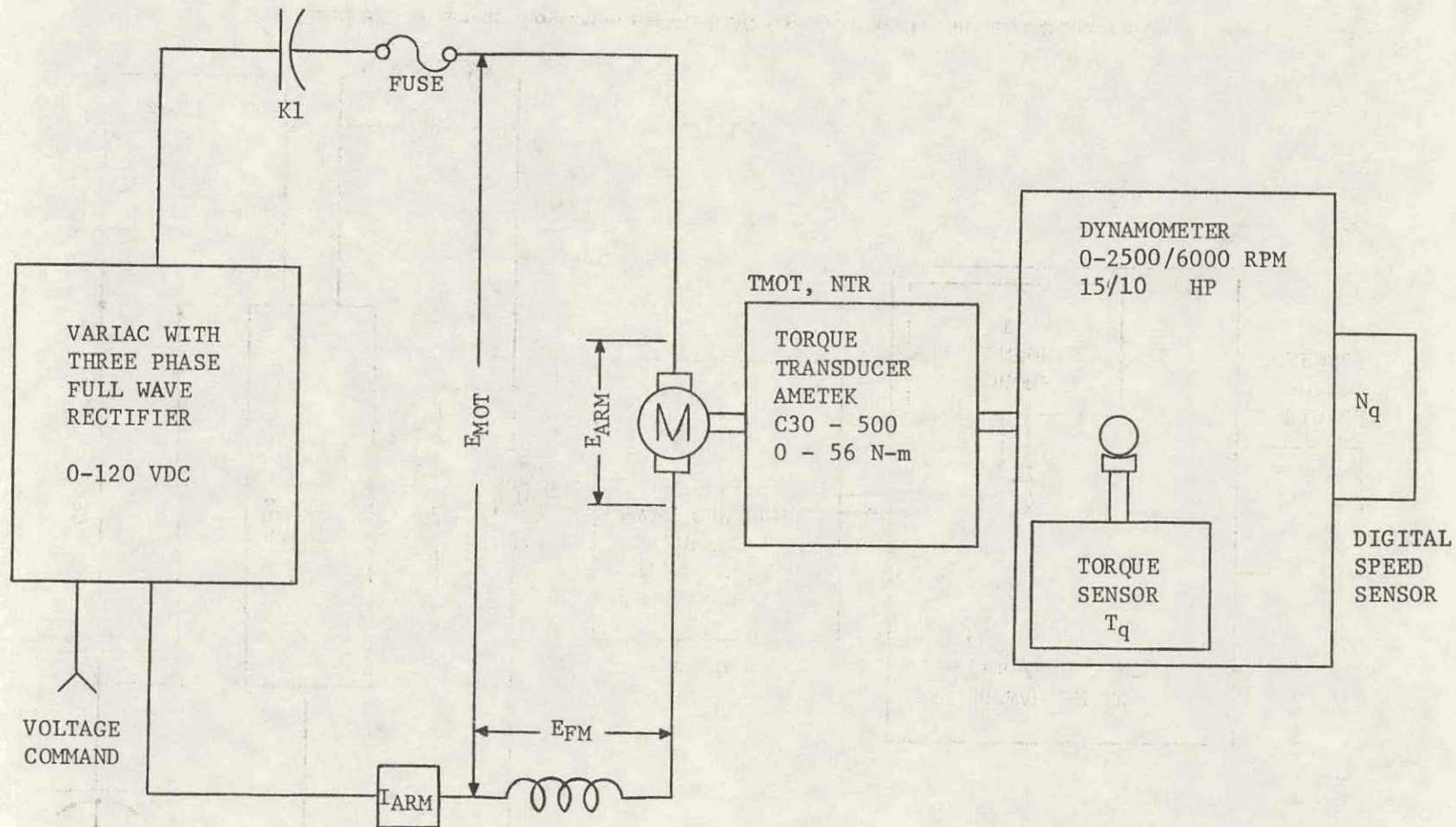
Figure 9.5. Schematic for dynamometer No. 3 DC motor test facility, continuous DC power mode.
