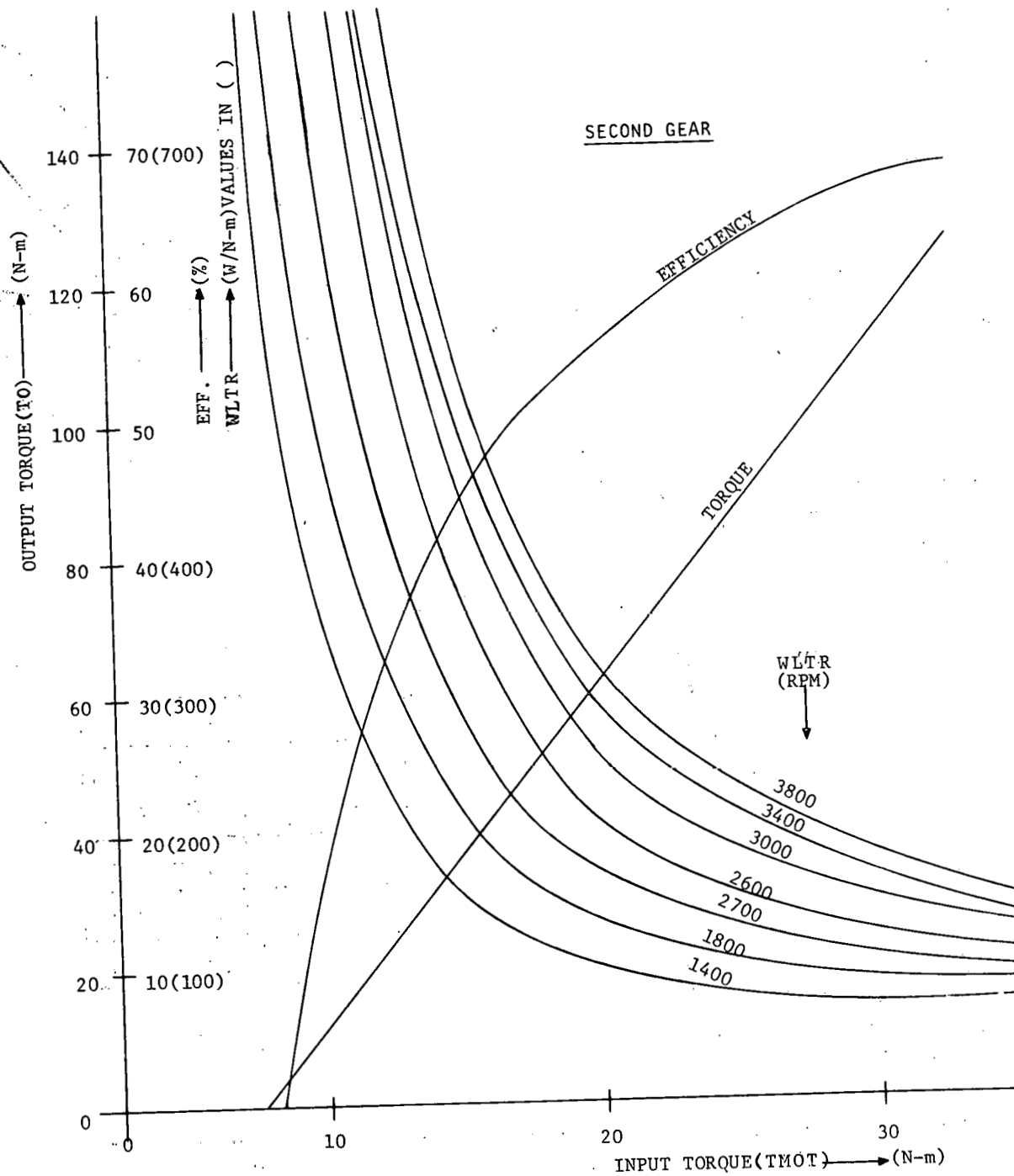
FIGURE 11.4: TRANSMISSION PERFORMANCE TEST IN SECOND GEAR (GR2)
