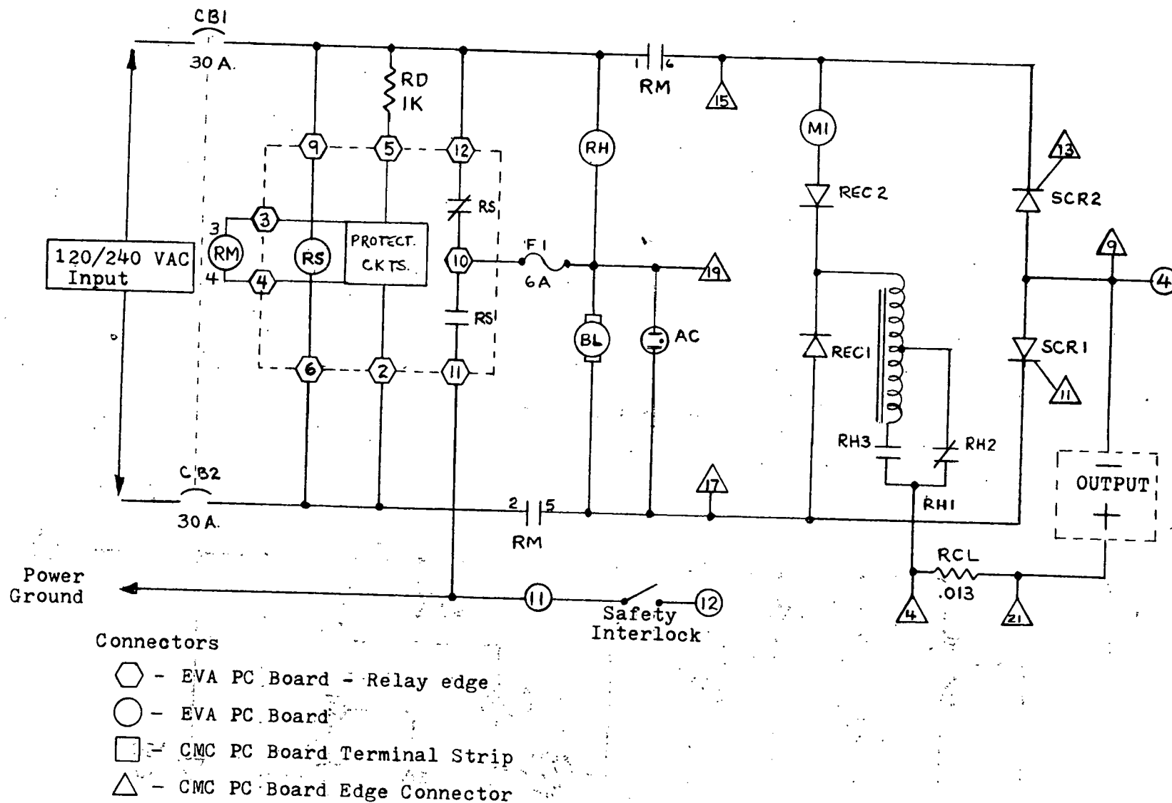
Figure E1. Main Input-Output Circuit (Components on PC Boards).
