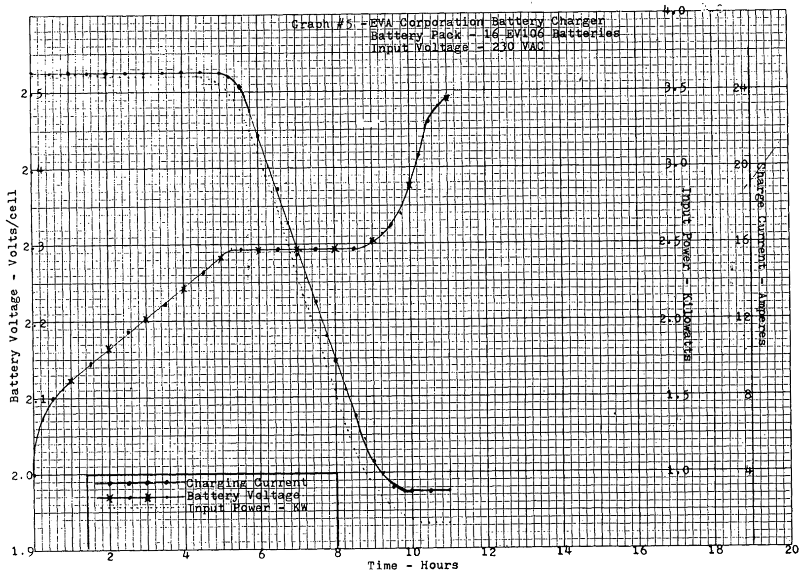
Figure E11. Battery Charger Power Consumption, 240 V RMS.
