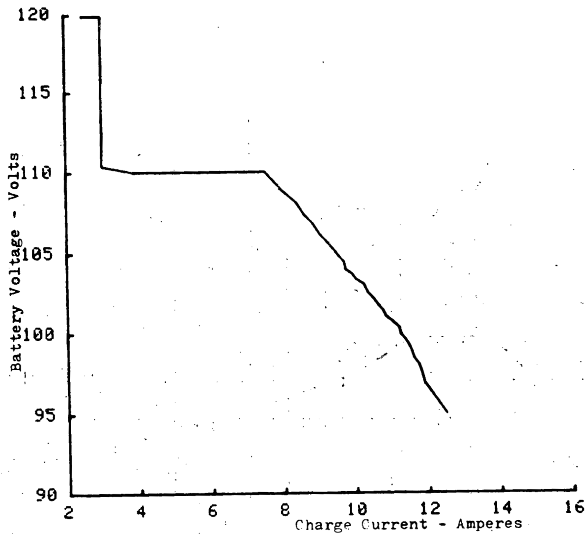
Figure E8. Battery Charger Voltage/Current Slope, Graph 2.
