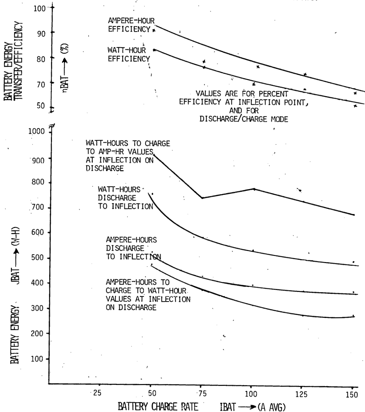
Figure 15.3. Battery discharge/charge efficiency.
