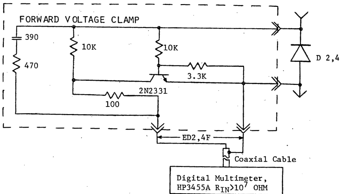
Figure 9.13. Adaptor circuit for measurement of diode forward voltage drop.
