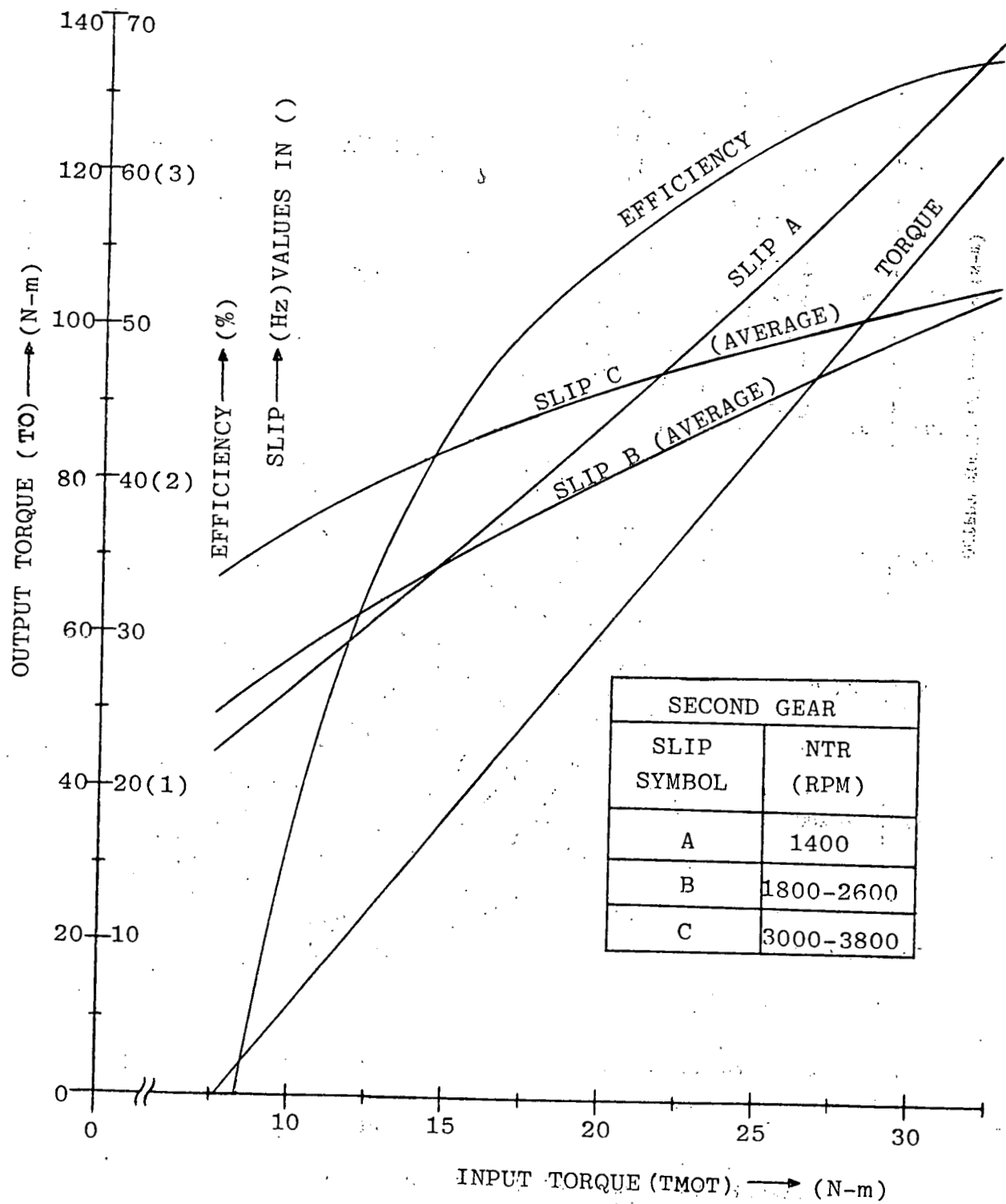
Figure 11.3. Transmission test performance in second gear (GR2).
