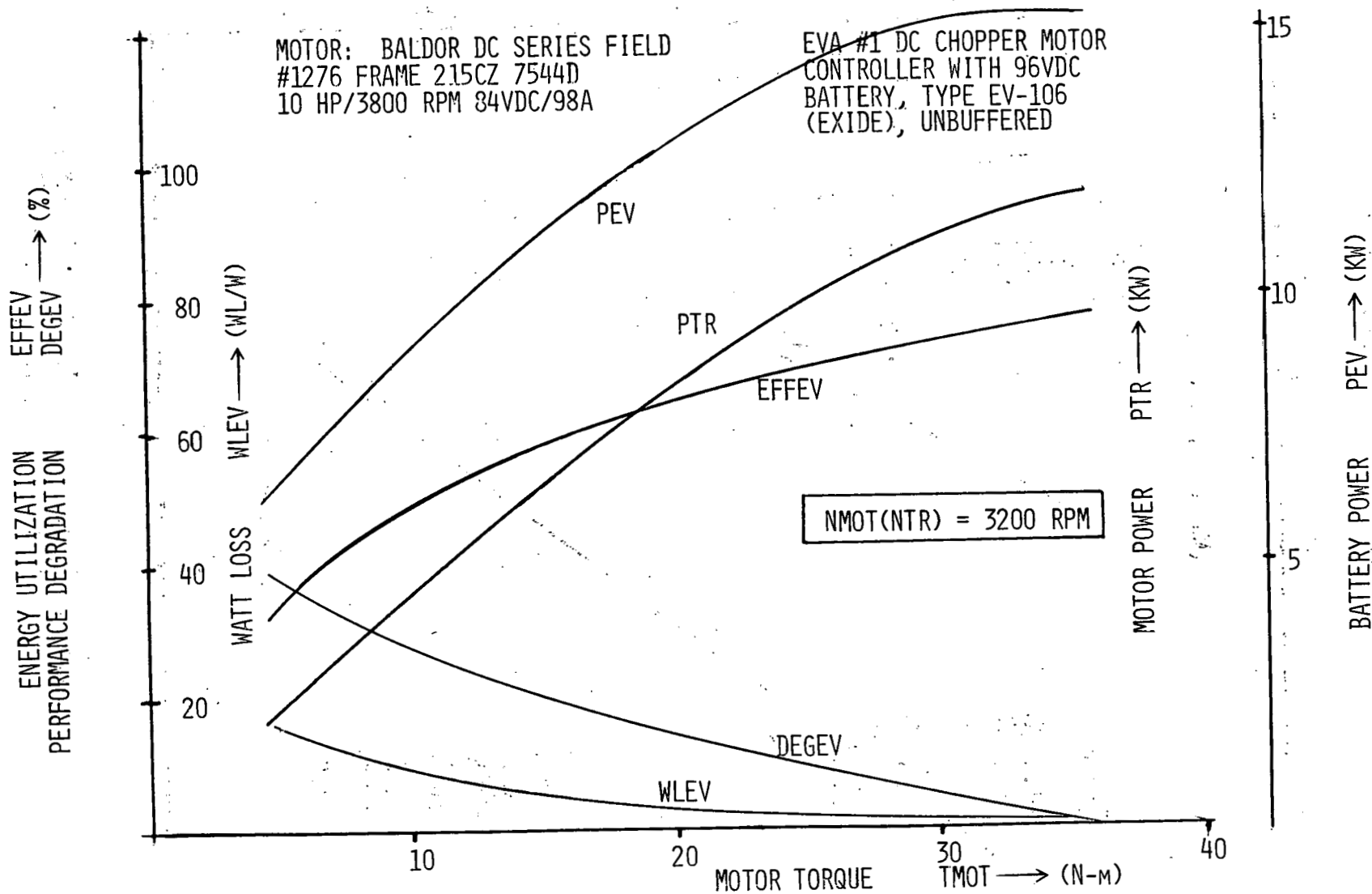
Figure 13.8K. System propulsion profile @ 3200 RPM, pulsed DC power.
