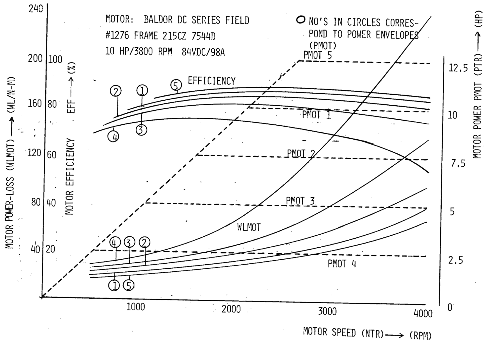
Figure 12.12. Parametric test data, motor efficiency and power loss per unit torque.
