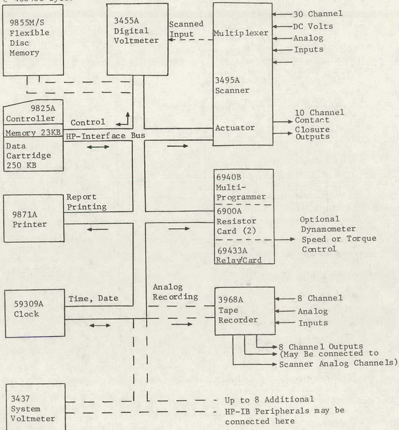
Figure 8.2. Schematic of HP 3052A data acquisition system.
