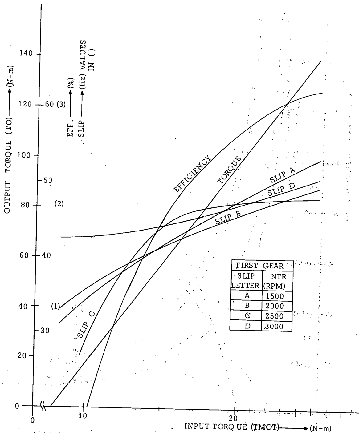
FIGURE 11.1: TRANSMISSION PERFORMANCE TEST IN FIRST GEAR (GR1)
