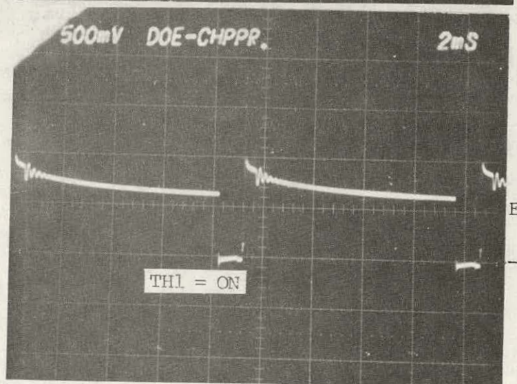
FIG. 14.5C: Forward conduction voltage (ED2F) of inverse by-pass diode (D2).
