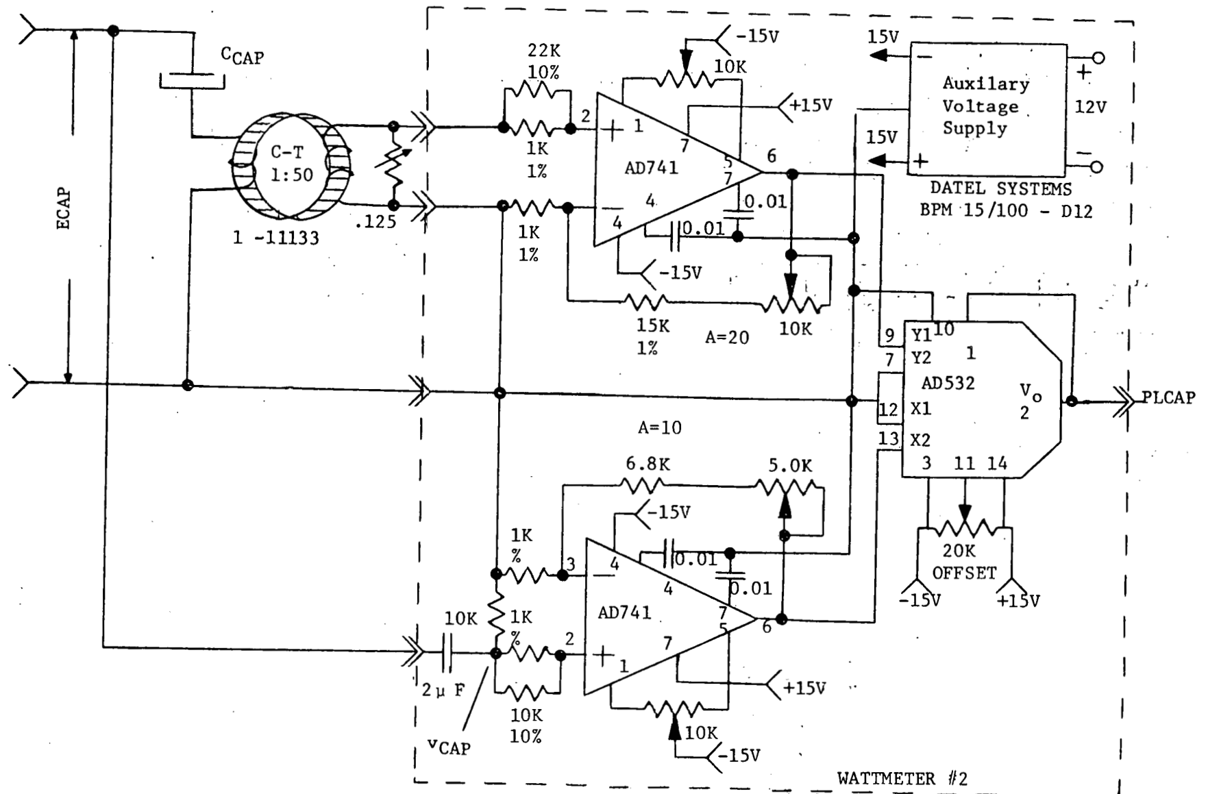
Figure 9.15. Measurement of power loss in capacitor (C4).
