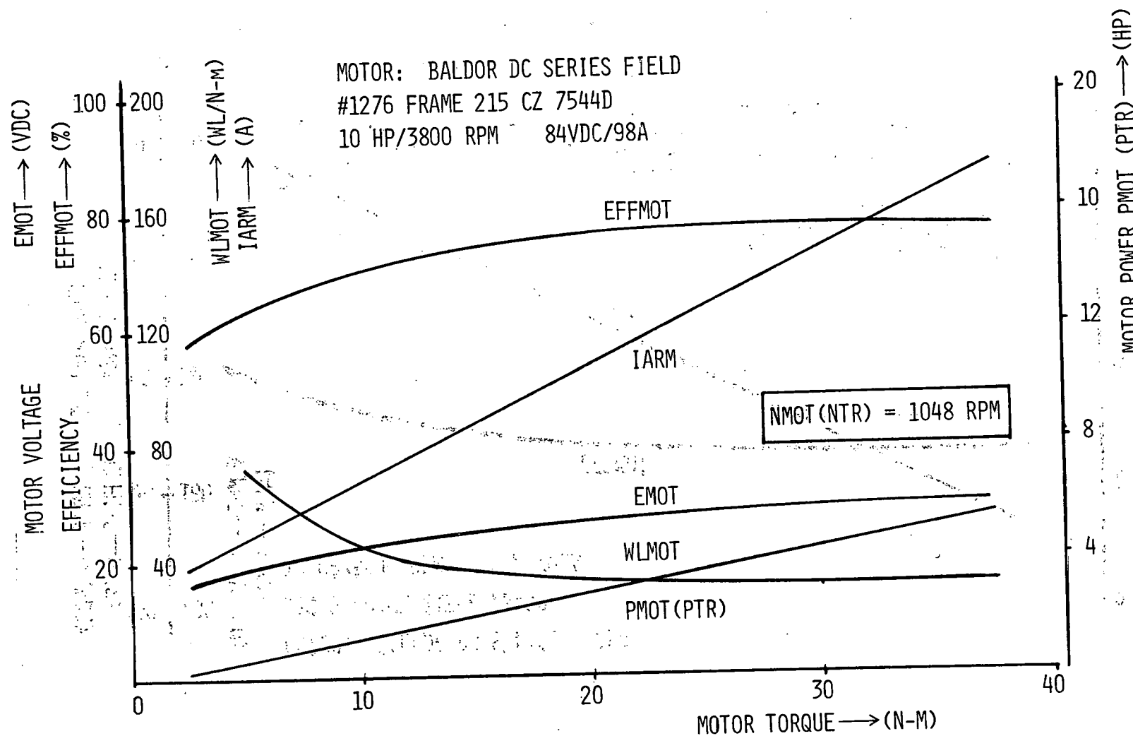
Figure 12.13C. Parametric test data @ N_{MOT} = 1048 \text{ RPM} .
