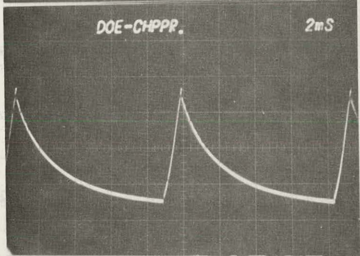
FIG. 14.6B: Motor current ( I_{ARM} = I_{TH1} + I_{D2F} ). The relative low chopper frequency results in high ripple amplitude.
