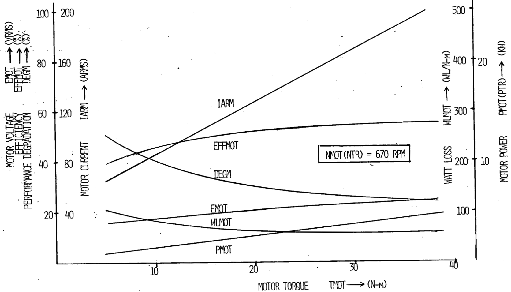
Figure 13.5C. Motor performance @ 670 RPM pulsed DC power.
