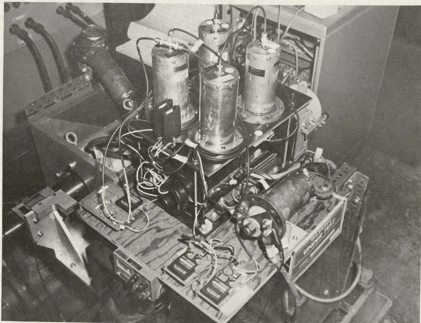
Figure 9.8. Mounting plate for coaxial current shunts on top of DC controller panel.
