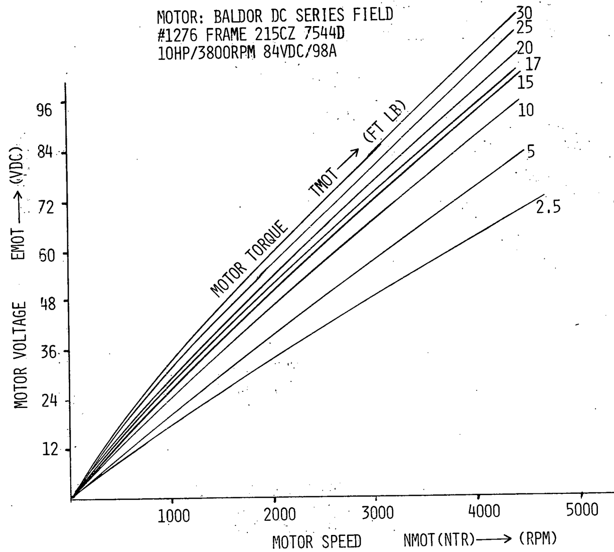
Figure 12.6. Motor voltage vs. motor speed.
