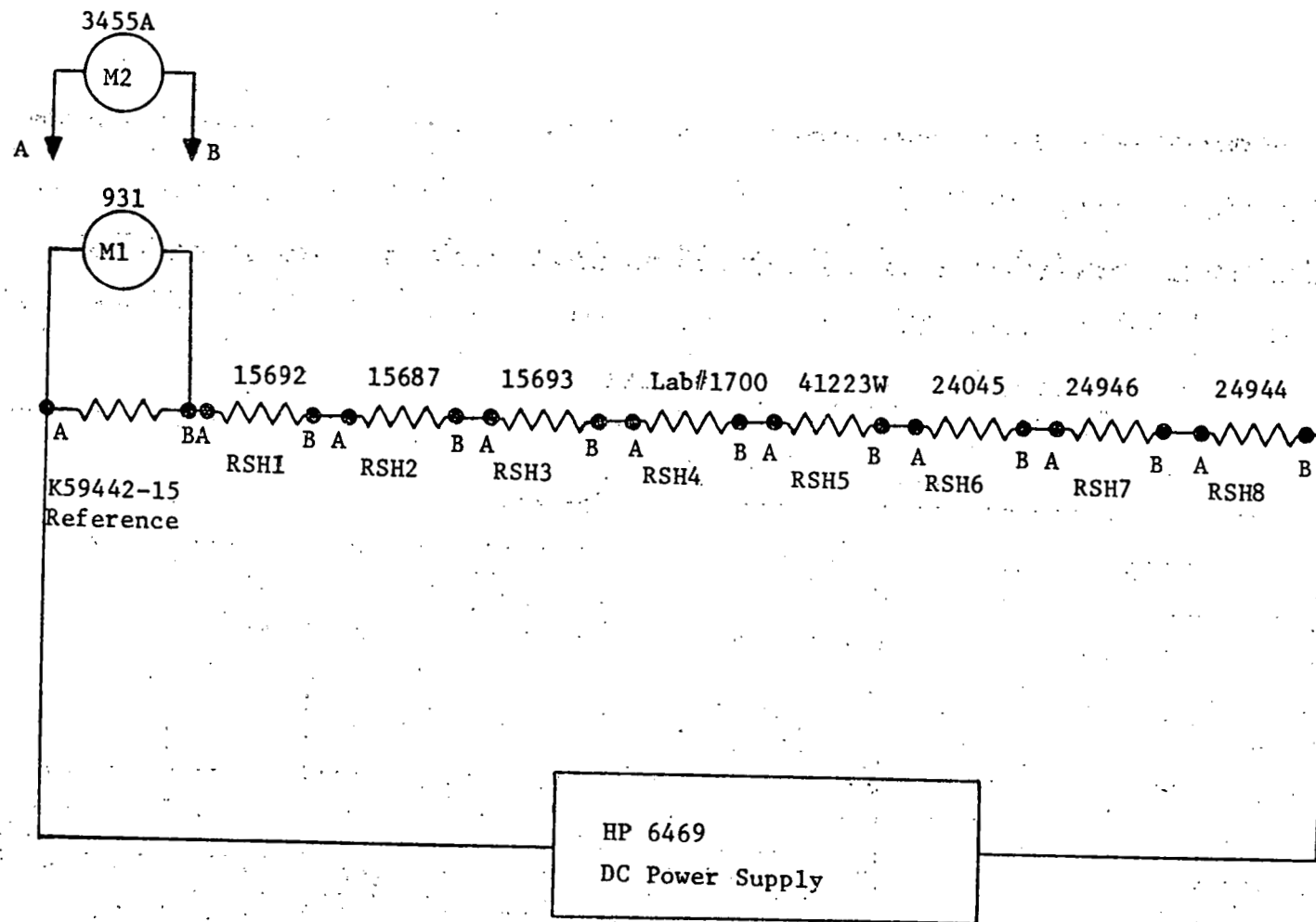
Figure 9.11. Calibration circuit for coaxial current shunts.
