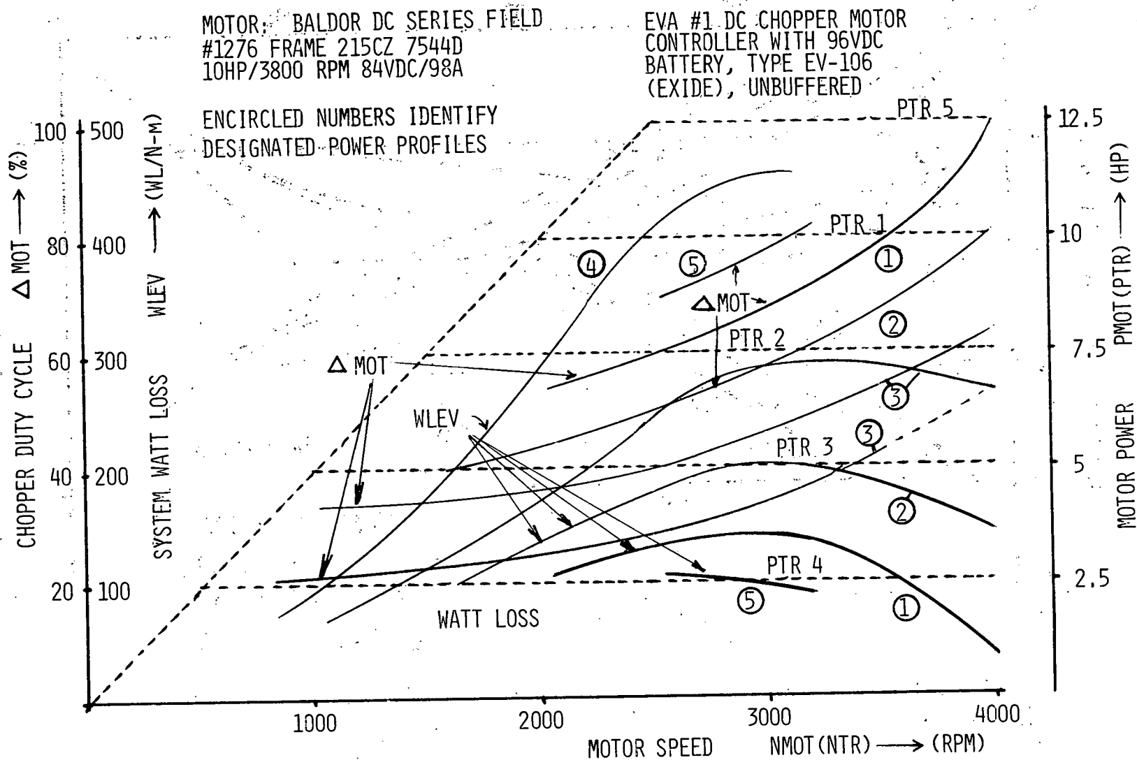
Figure 13.7. System propulsion profile, pulsed DC power.
