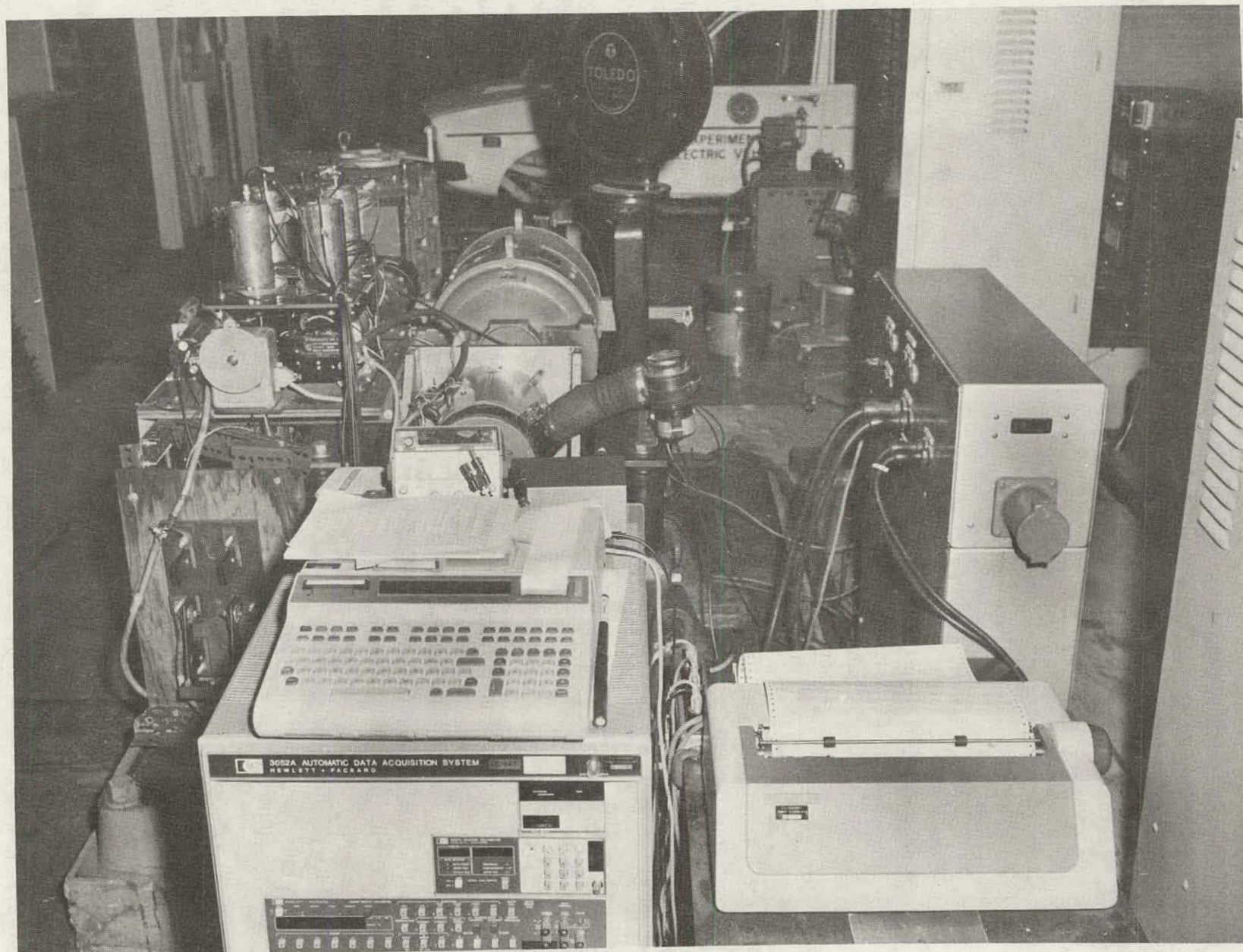
Figure 9.7. Dynamometer No. 3 test facility, overview.
