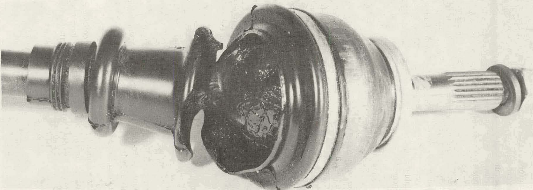
Figure 6.1. Broken seal of drive shaft.
