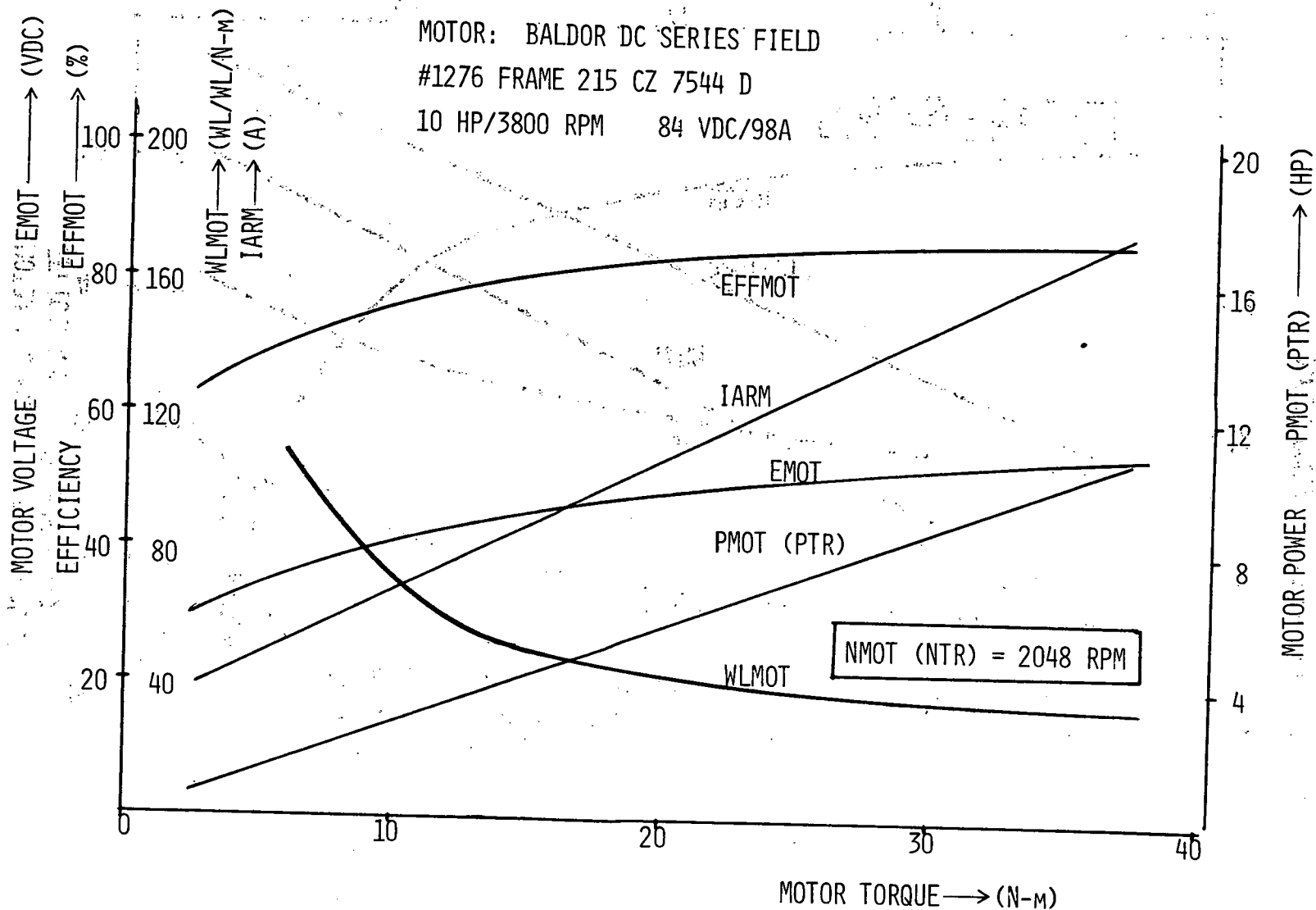
Figure 12.13F. Parametric test data @ NMOT = 2048 RPM.
