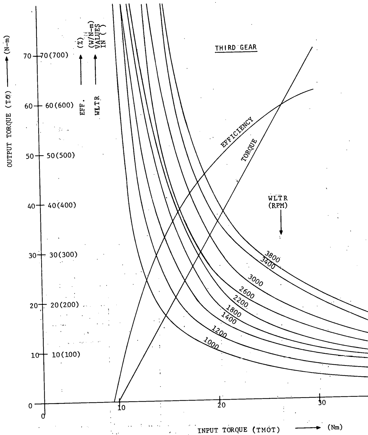
FIGURE 11.6: TRANSMISSION PERFORMANCE TEST IN THIRD GEAR (GR3)
