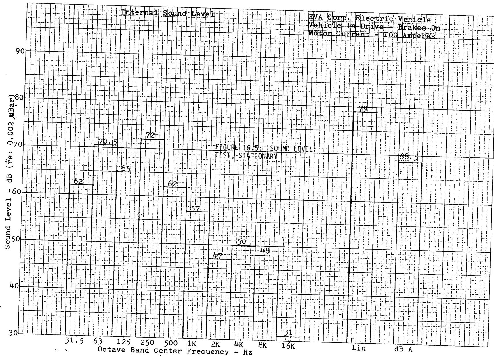
Figure 16.5. Sound level test, stationary.
