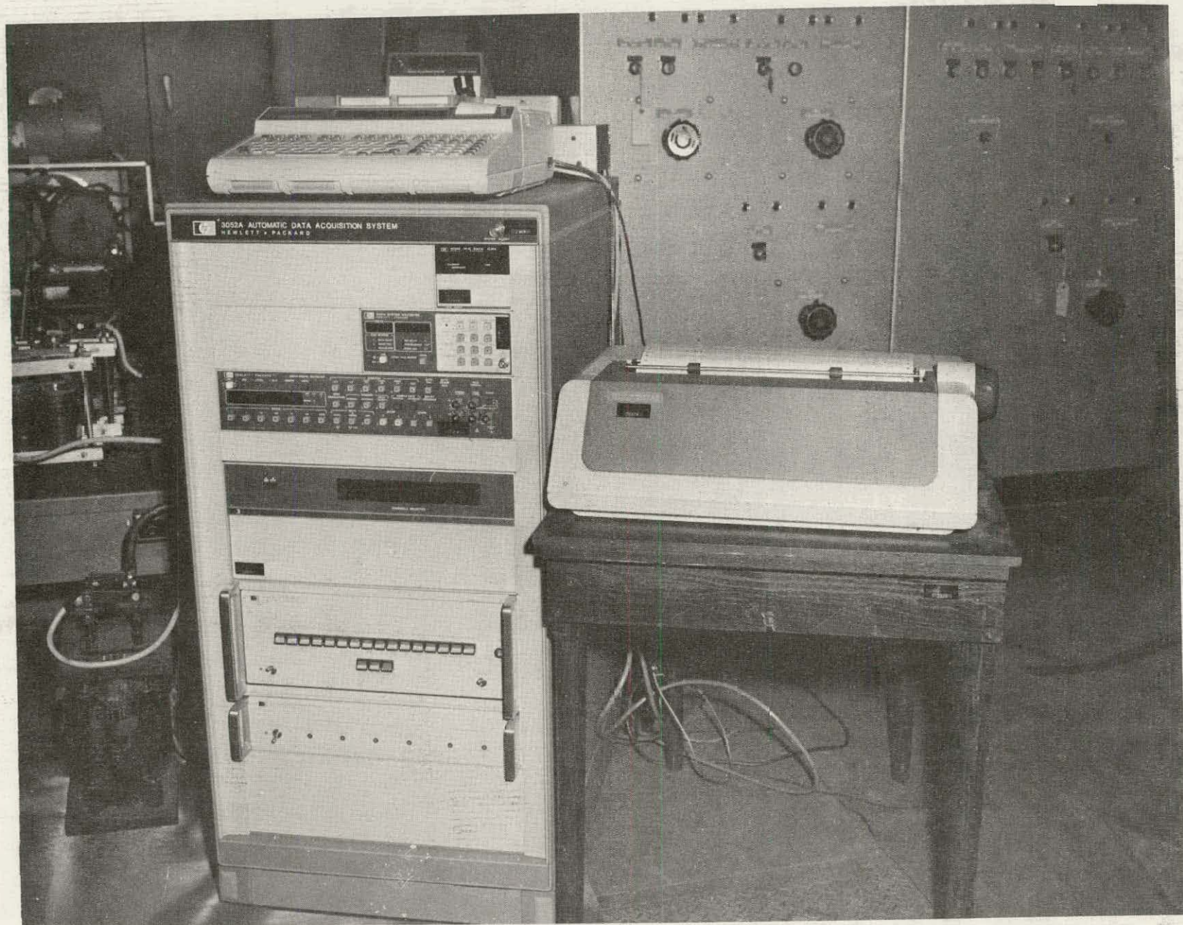
Figure 8.1. HP type 3052A data acquisition system.
