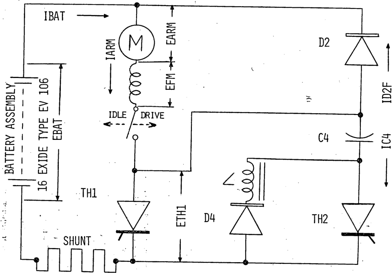
Figure 7.1. Simplified circuit schematic for CABLEFORM pulsomatic mark 10 controller.
