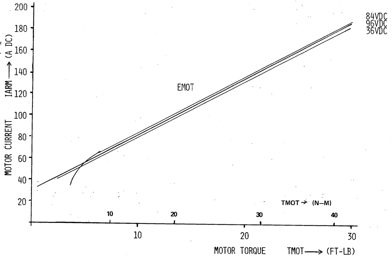
Figure 12.9. Motor current vs. motor shaft torque.
