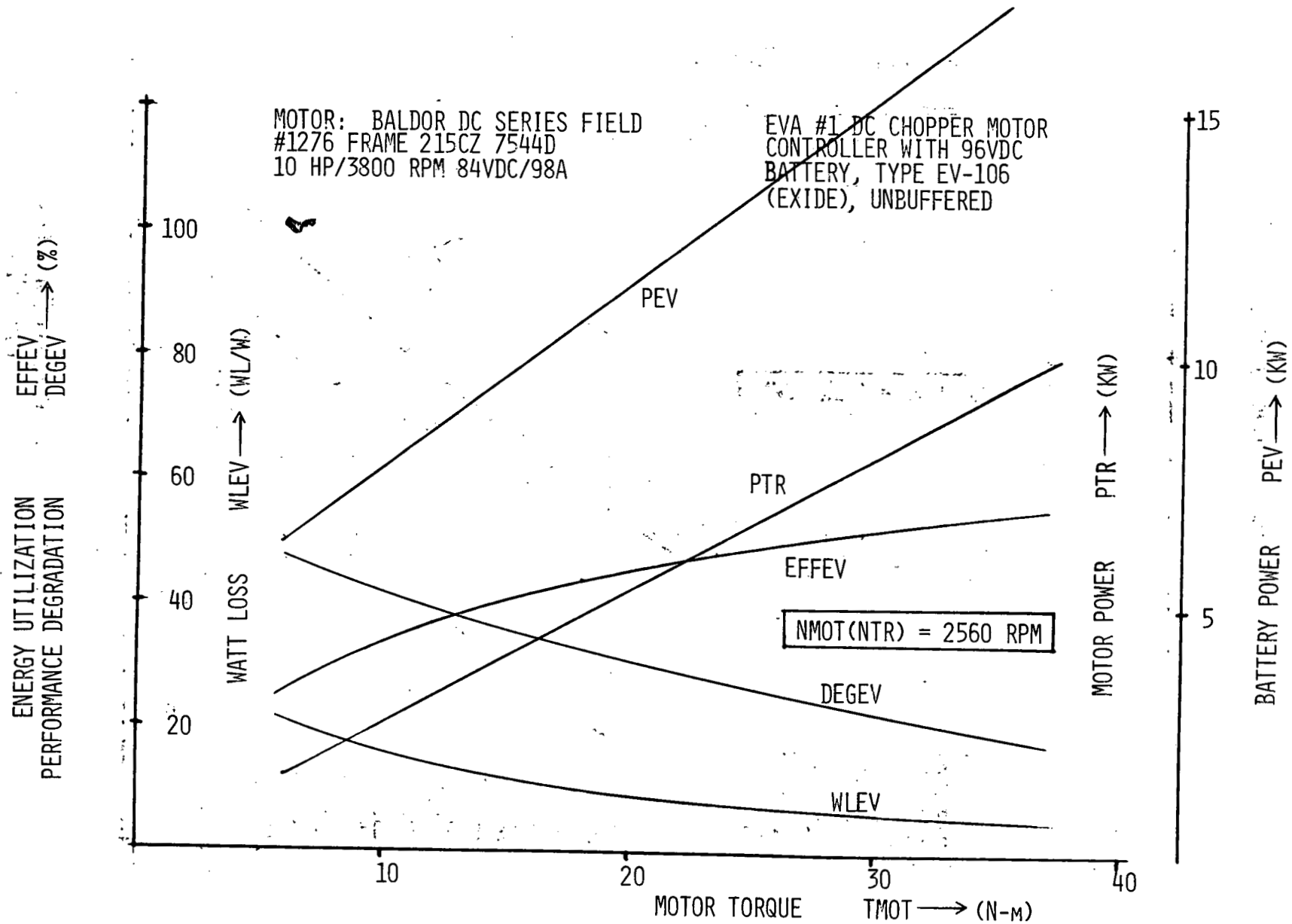
Figure 13.81. System propulsion profile @ 2560 RPM, pulsed DC power.
