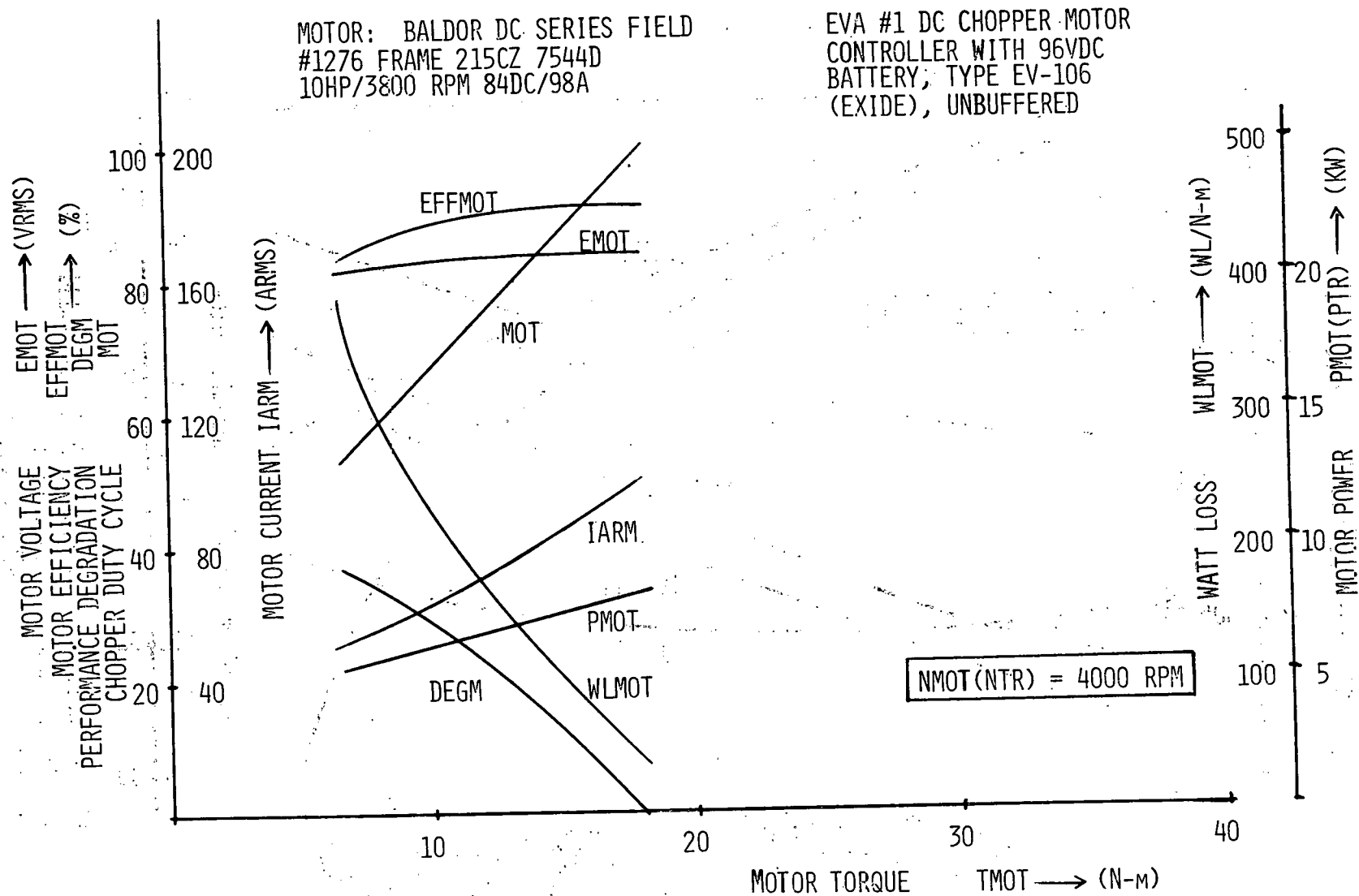
Figure 13.5L. Motor performance @ 4000 RPM, pulsed DC power.
