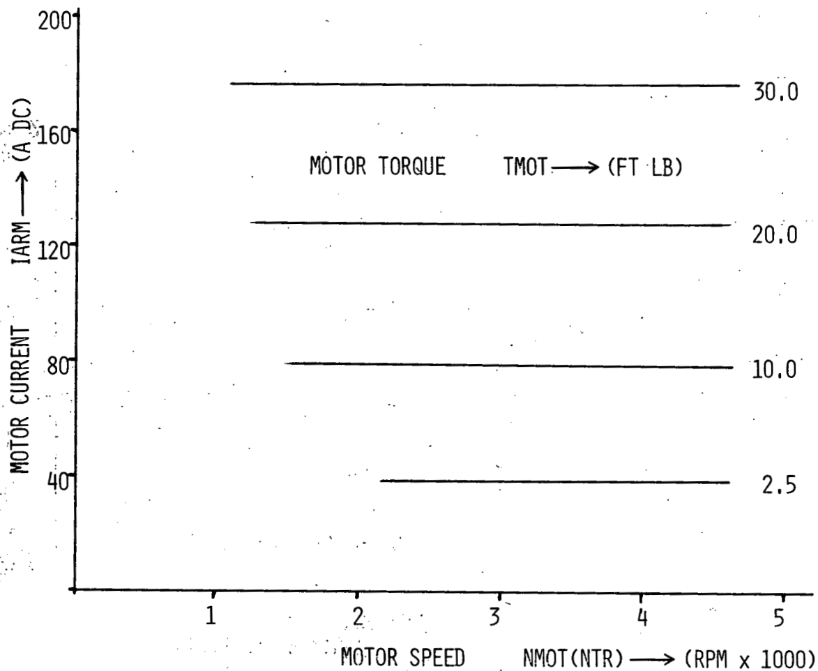
Figure 12.7. Motor current vs. speed.
