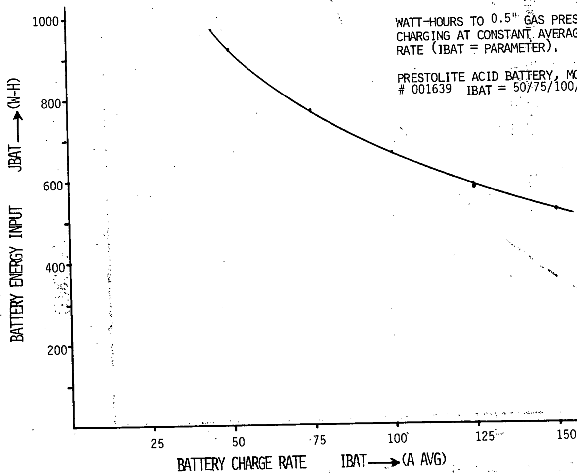
Figure 15.2. Battery energy input vs. charge rate.
