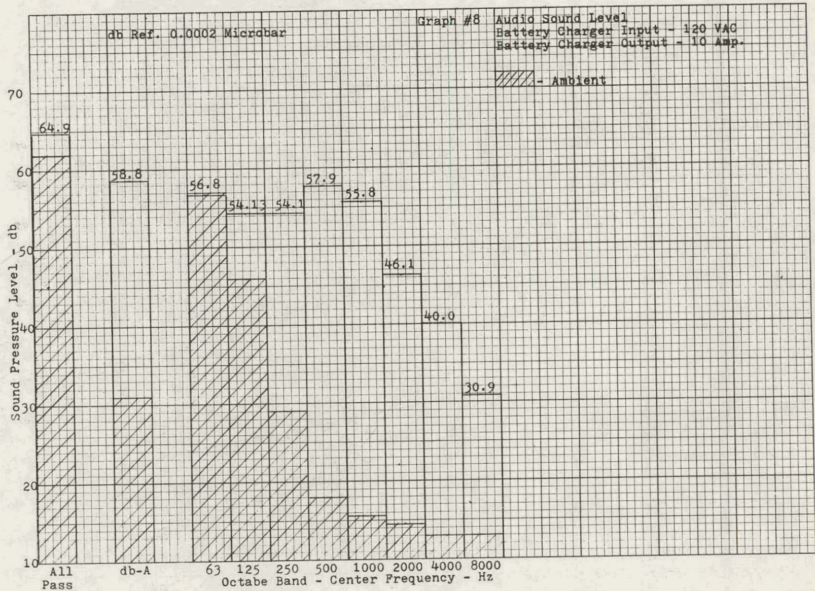
Figure E14. Audio Sound Level: Input - 120 V RMS; Output - 10A.
