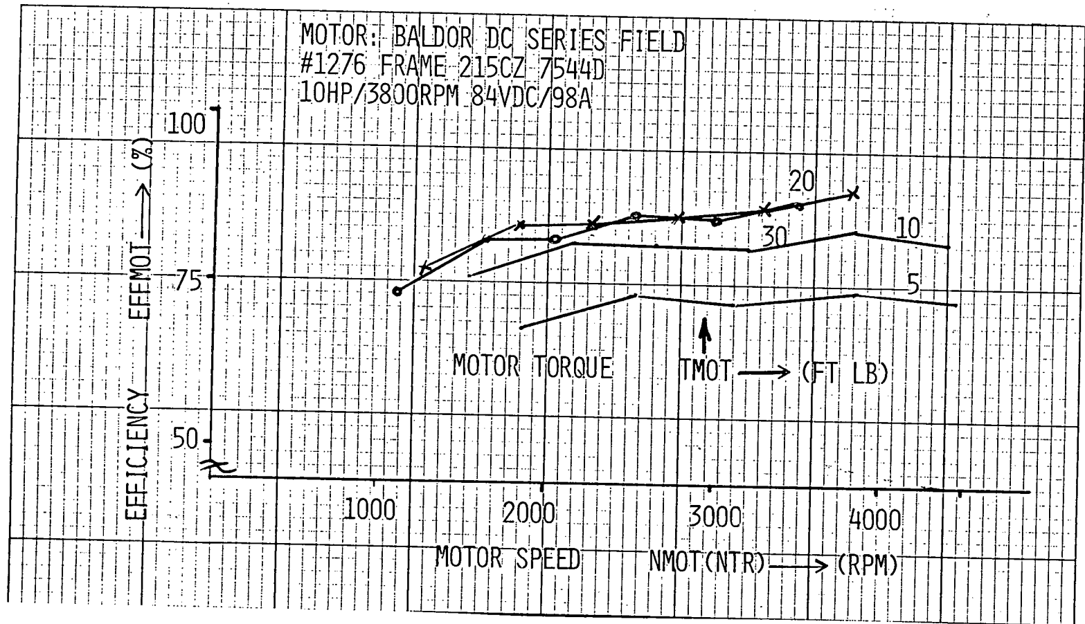
Figure 12.1. Motor efficiency, TMOT = parameter.
