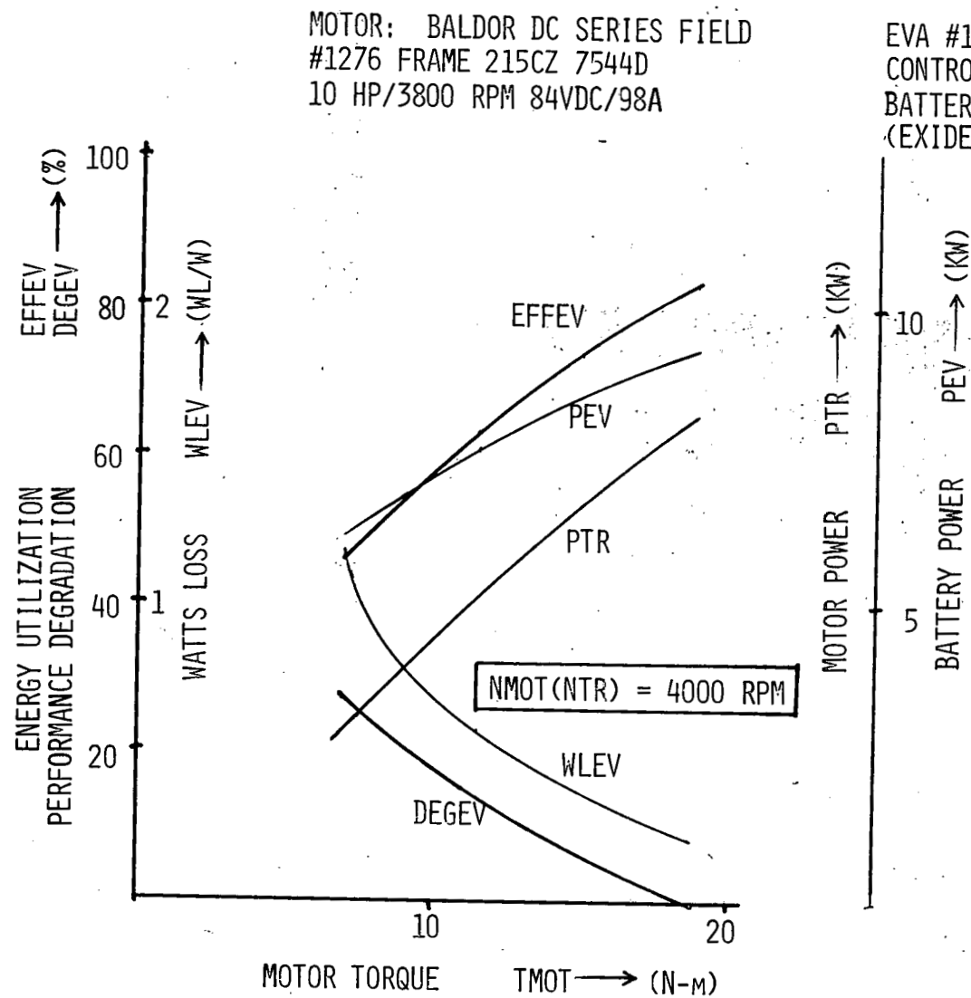
Figure 13.8L. System propulsion profile @ 4000 RPM, pulsed DC power.
