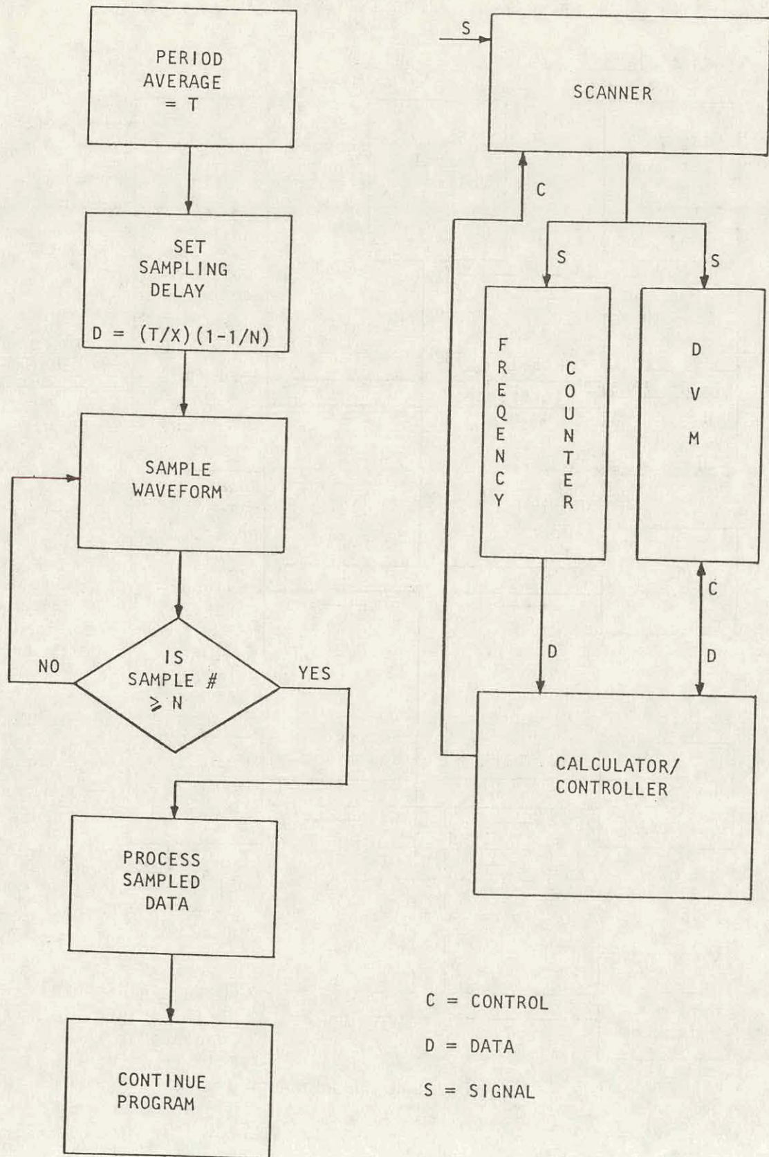
Figure 8.3. Flowchart and hardware implementation of variable frequency, arbitrary waveform voltage measurement.
