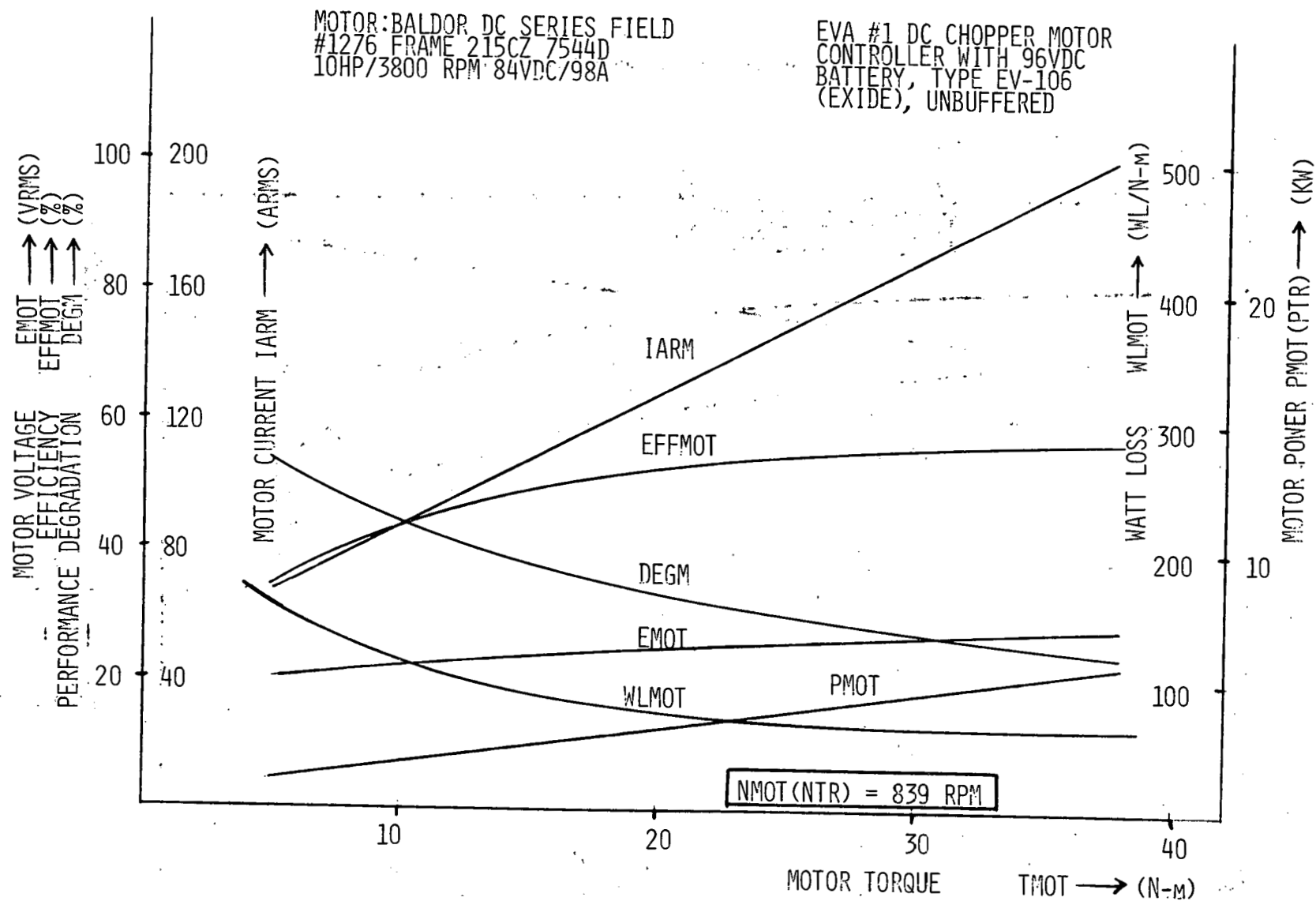
Figure 13.5D. Motor performance @ 839 RPM, pulsed DC power.
