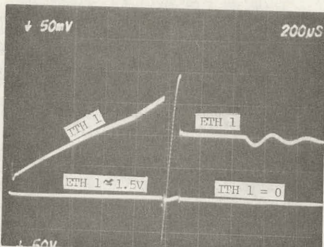
FIG. 14.2A: Superimposed ITH1 = 100A/cm and ETH1 = 50V/cm
