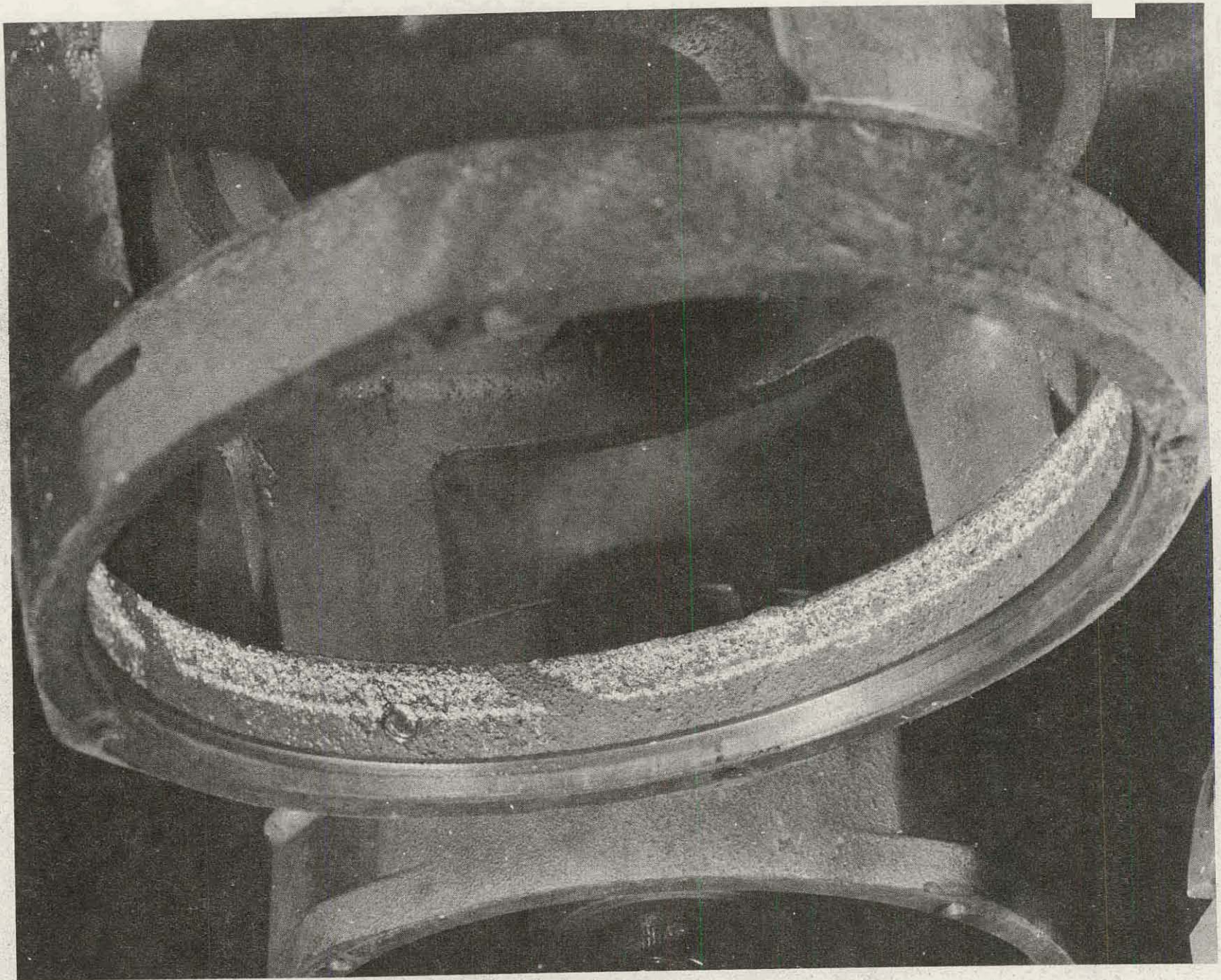
Figure 6.5. Motor damage to brush housing caused by disintegration of soft solder joints.
