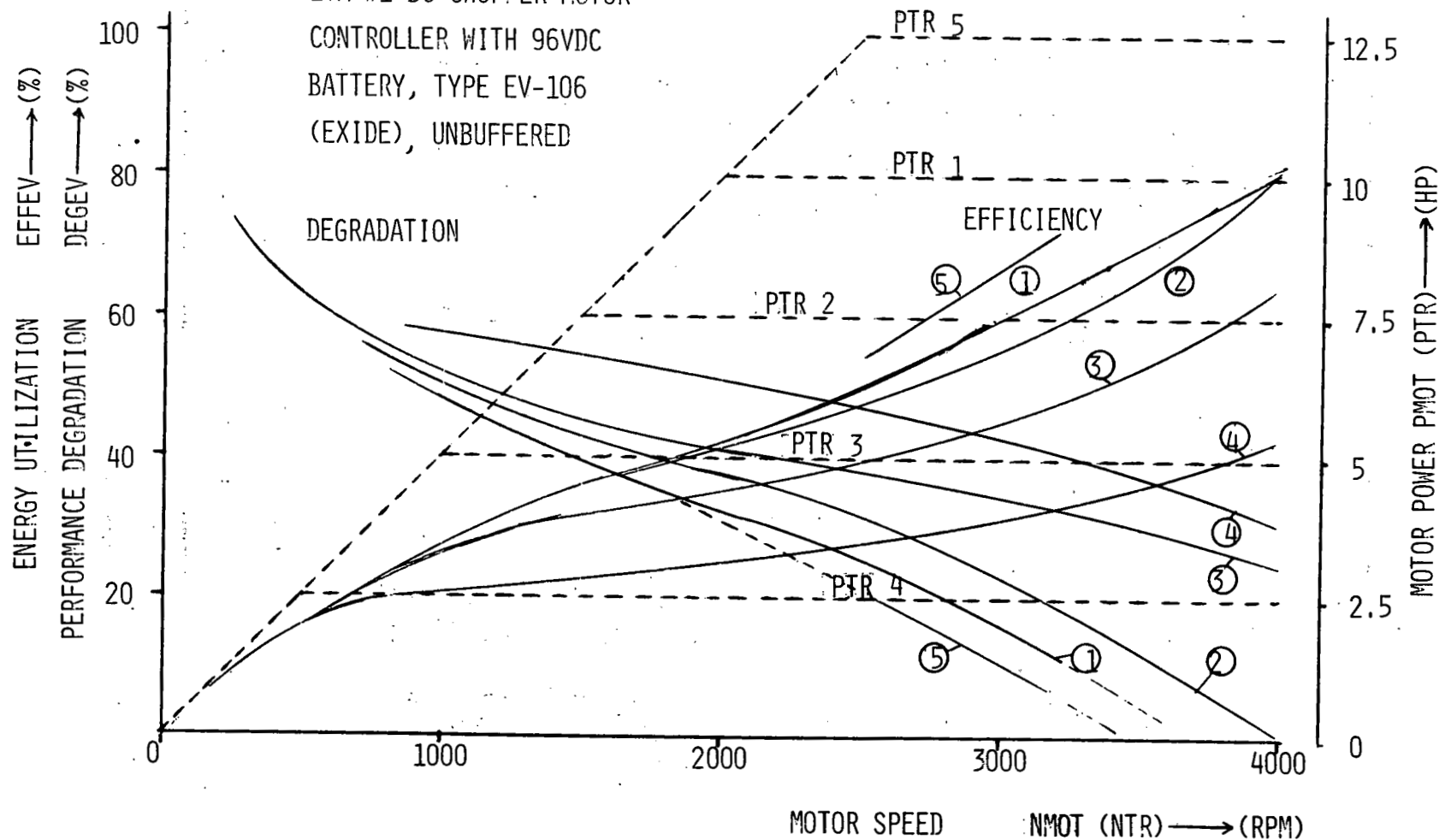
Figure 13.6. System propulsion profile, pulsed DC power.
