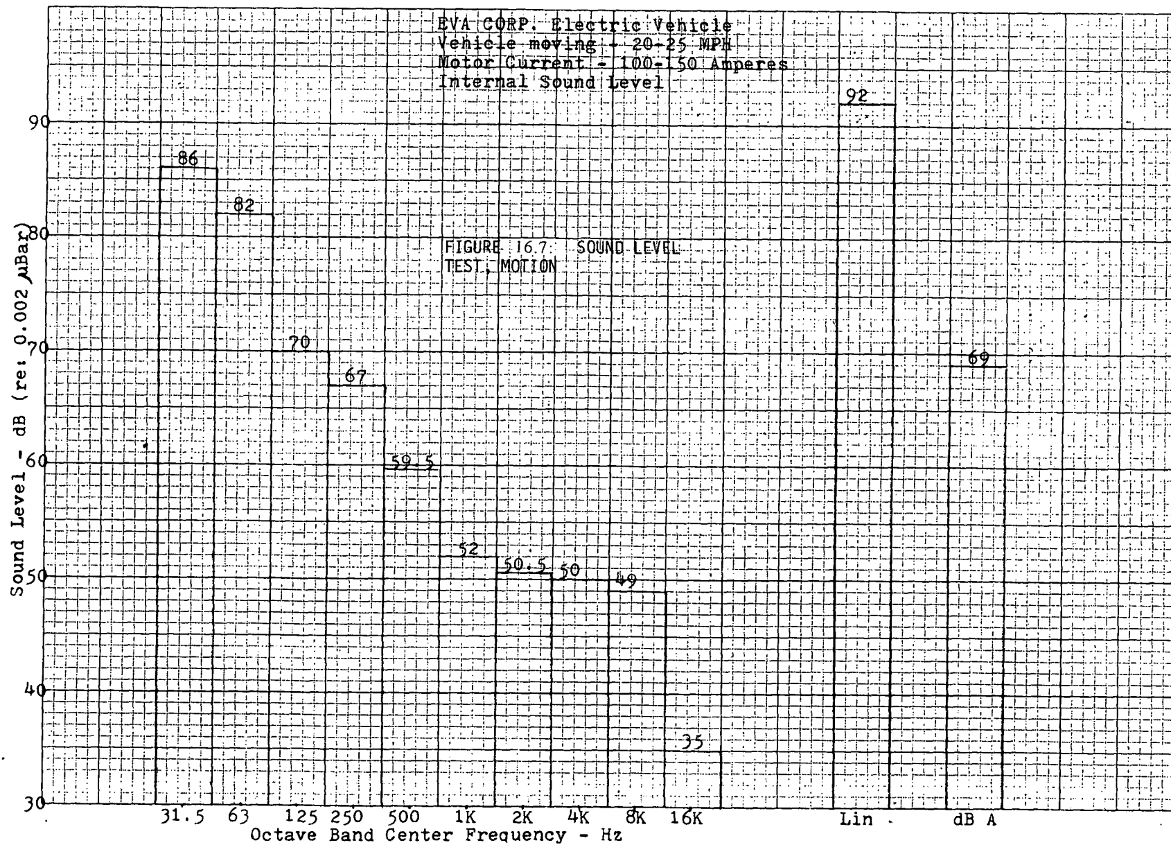
Figure 16.7. Sound level test, motion.
