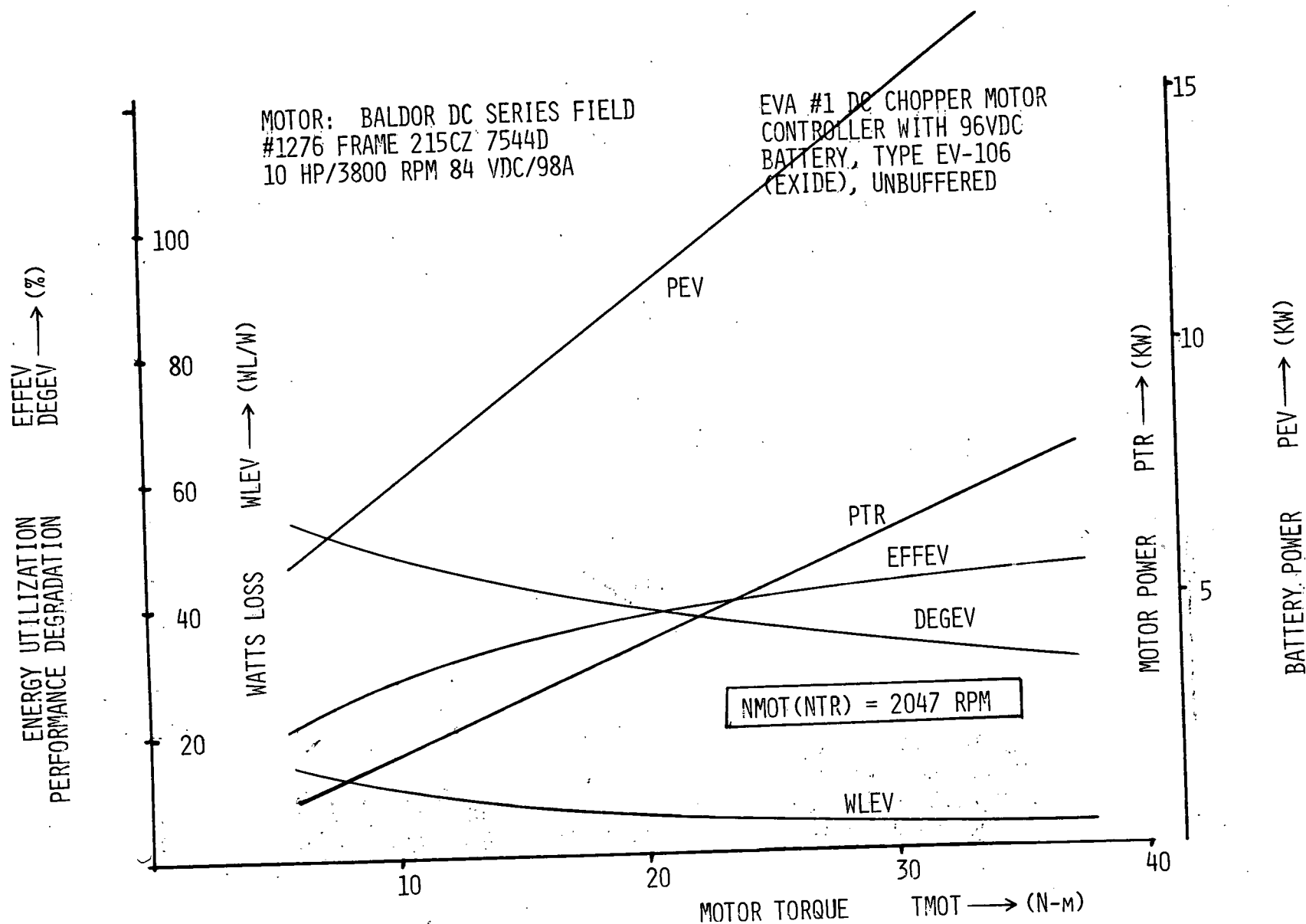
Figure 13.8H. System propulsion profile @ 2047 RPM, pulsed DC power.
