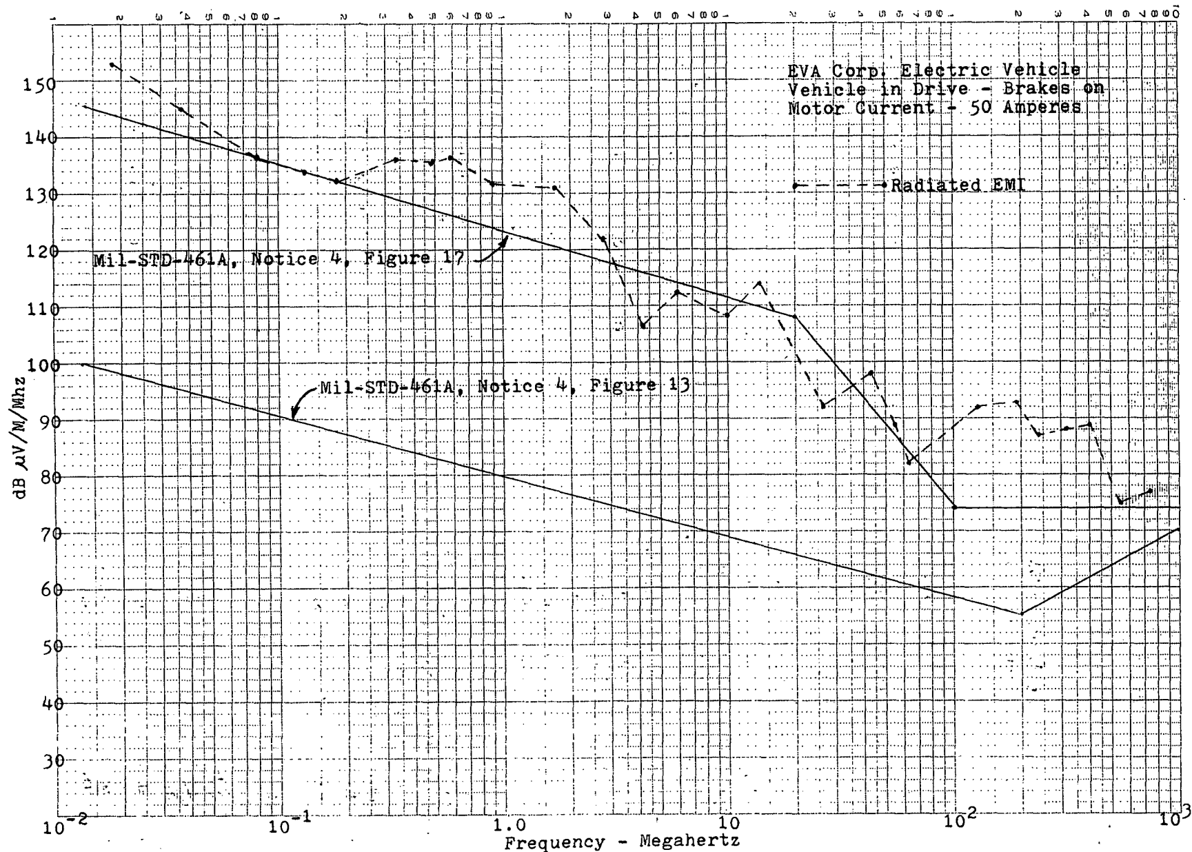
Figure 16.2. EMI test, 50A load.
