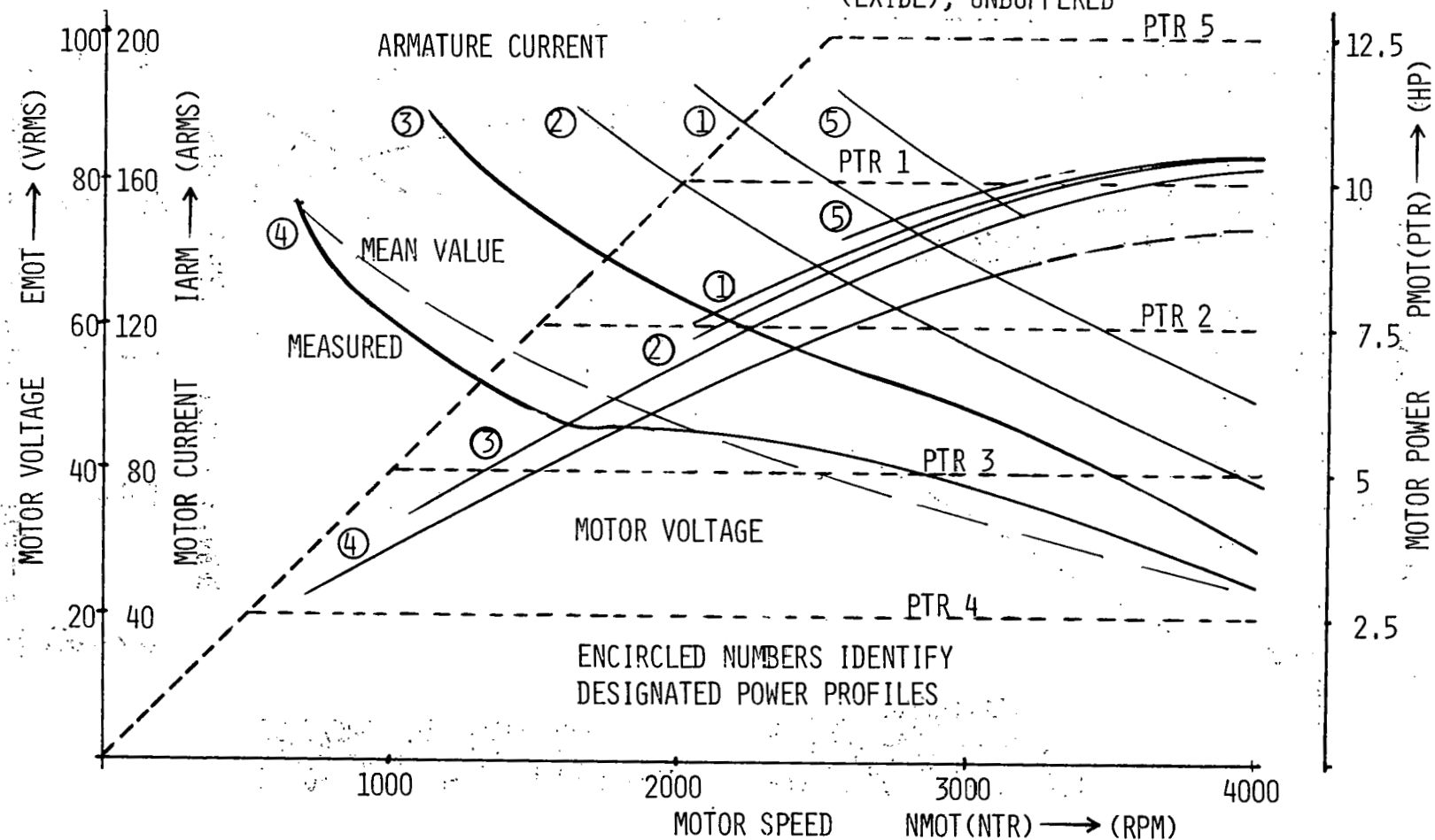
Figure 13.4. Motor propulsion profile, pulsed DC power.
