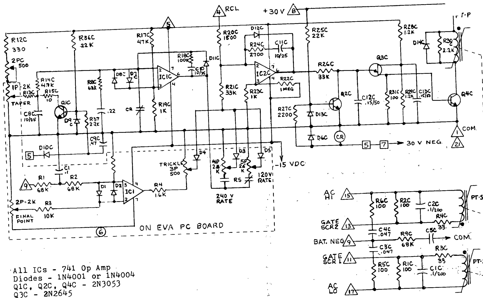
Figure E4. Battery Charger Control Circuit.
