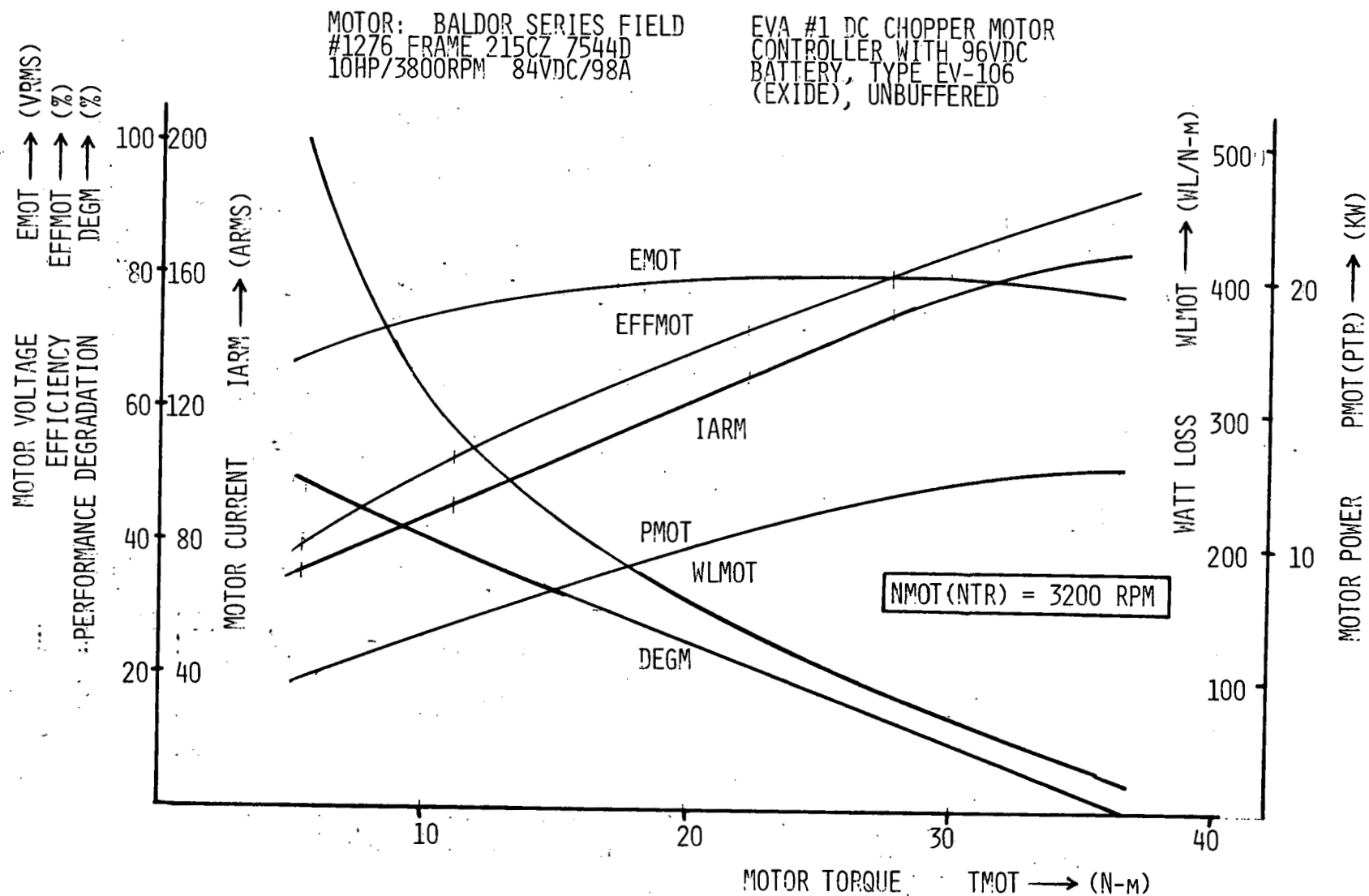
Figure 13.5K. Motor performance @ 3200 RPM, pulsed DC power.
