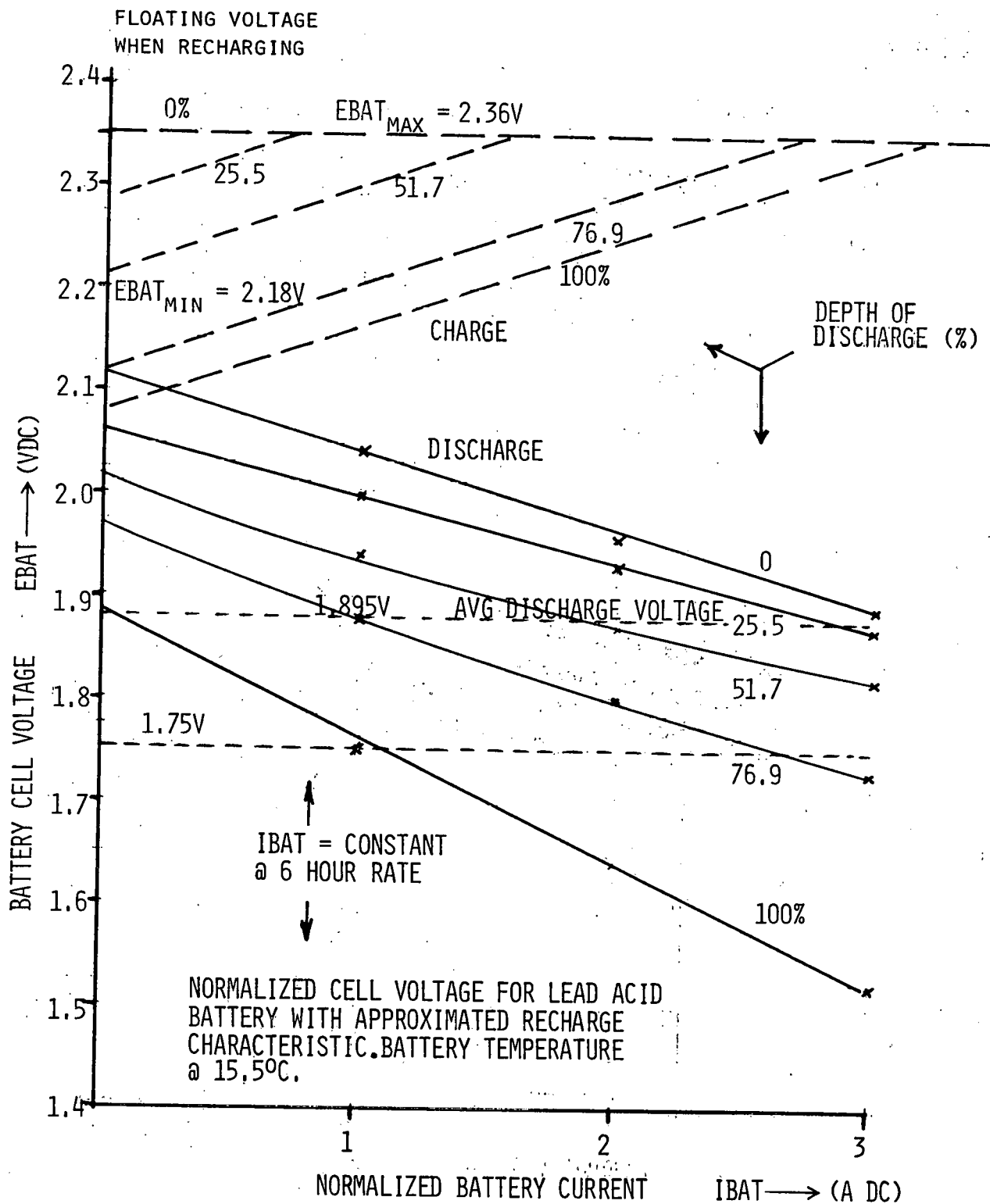
Figure 7.2. Battery cell voltage vs. charge level.
