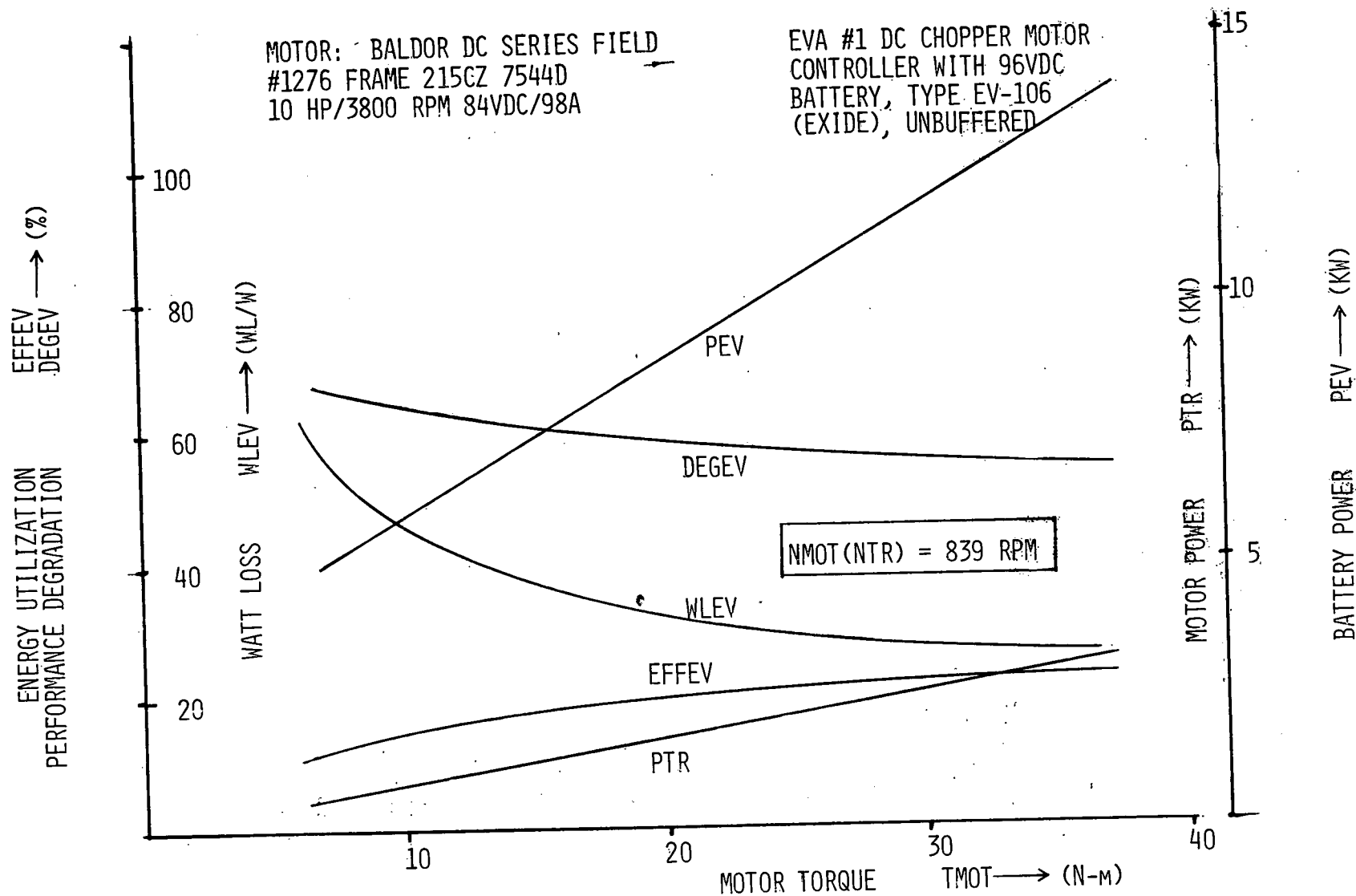
Figure 13.8D. System propulsion profile @ 839 RPM, pulsed DC power.
