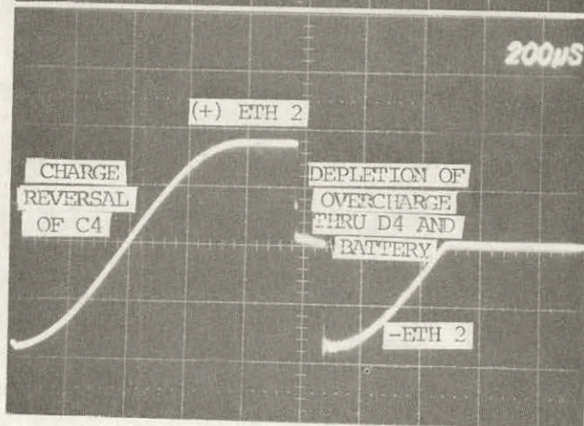
FIG 14.3B: Blocking volt- age of commutating thyristor (TH2) ETH2 = 50V/cm
