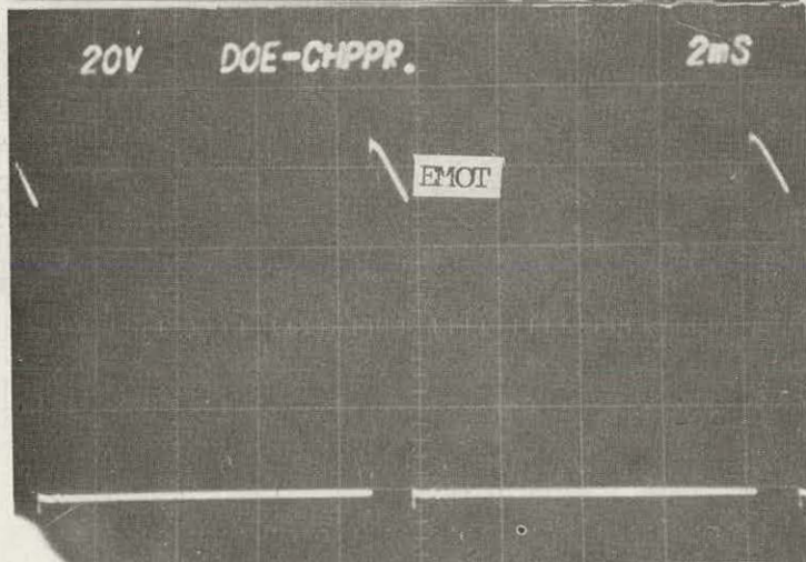
FIG. 14.6C: Motor voltage (EMOT). Common terminal of oscilloscope on anode of TH1. EMOT = 20V/cm
