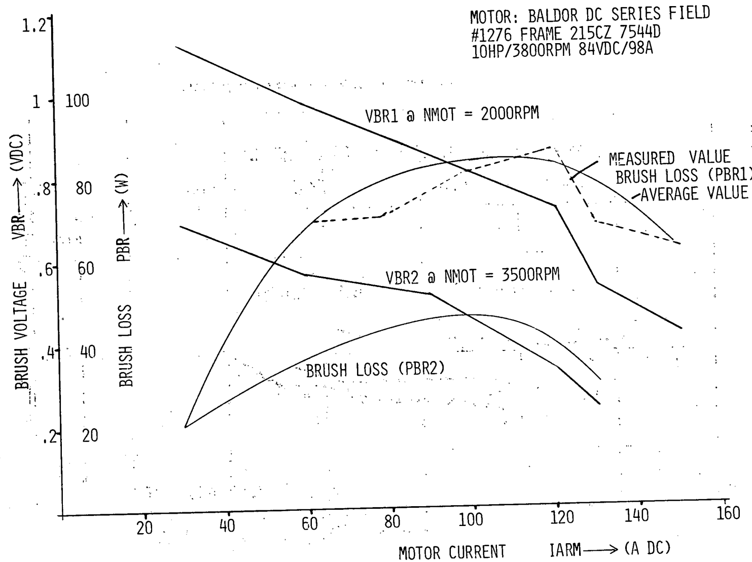
Figure 12.2. Brush losses vs. motor current.
