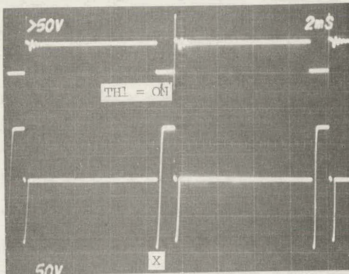
FIG. 14.8A: Upper trace: ETH1 100V/cm
