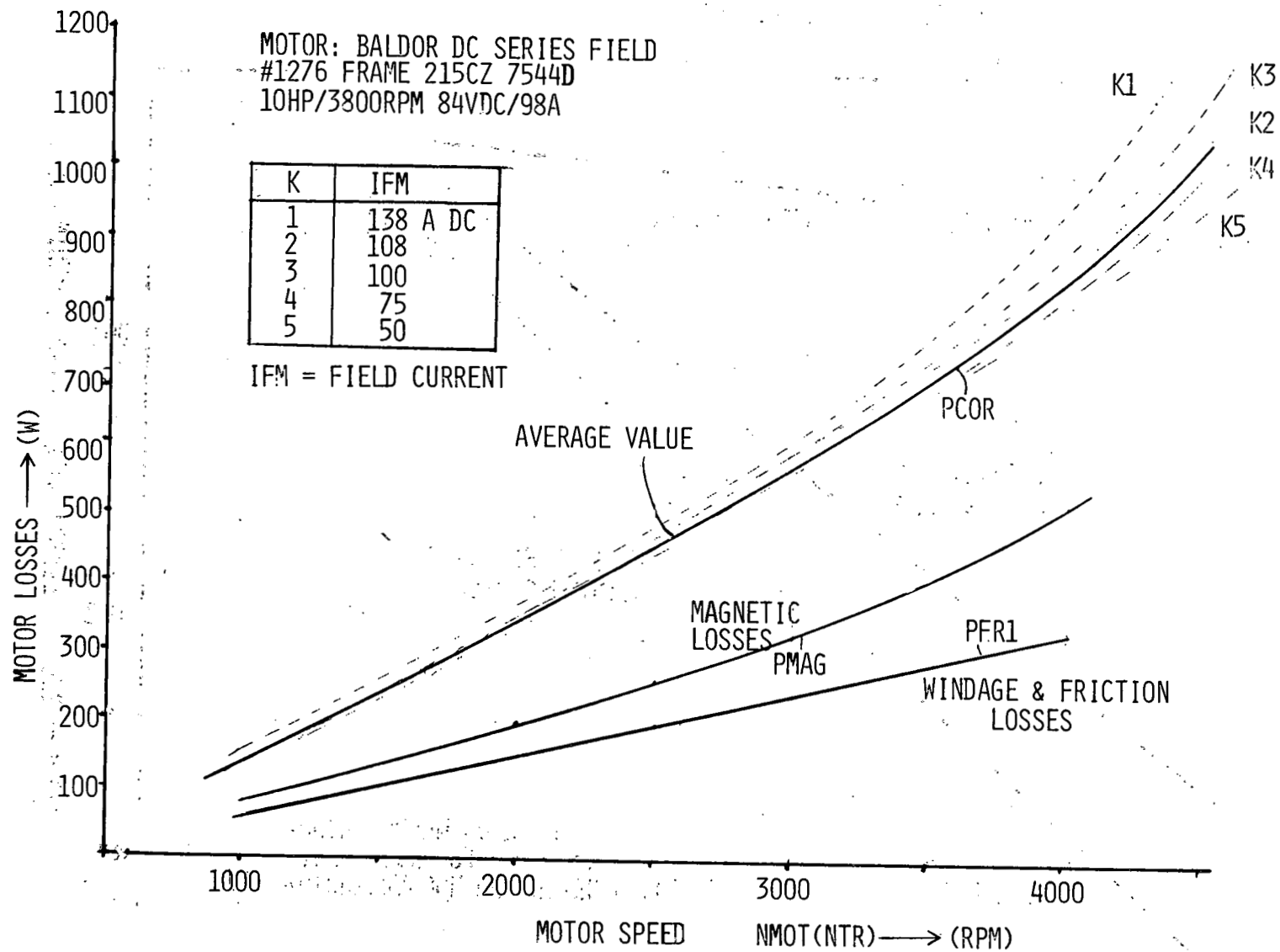
Figure 12.3. Windage, friction and magnetic loss.
