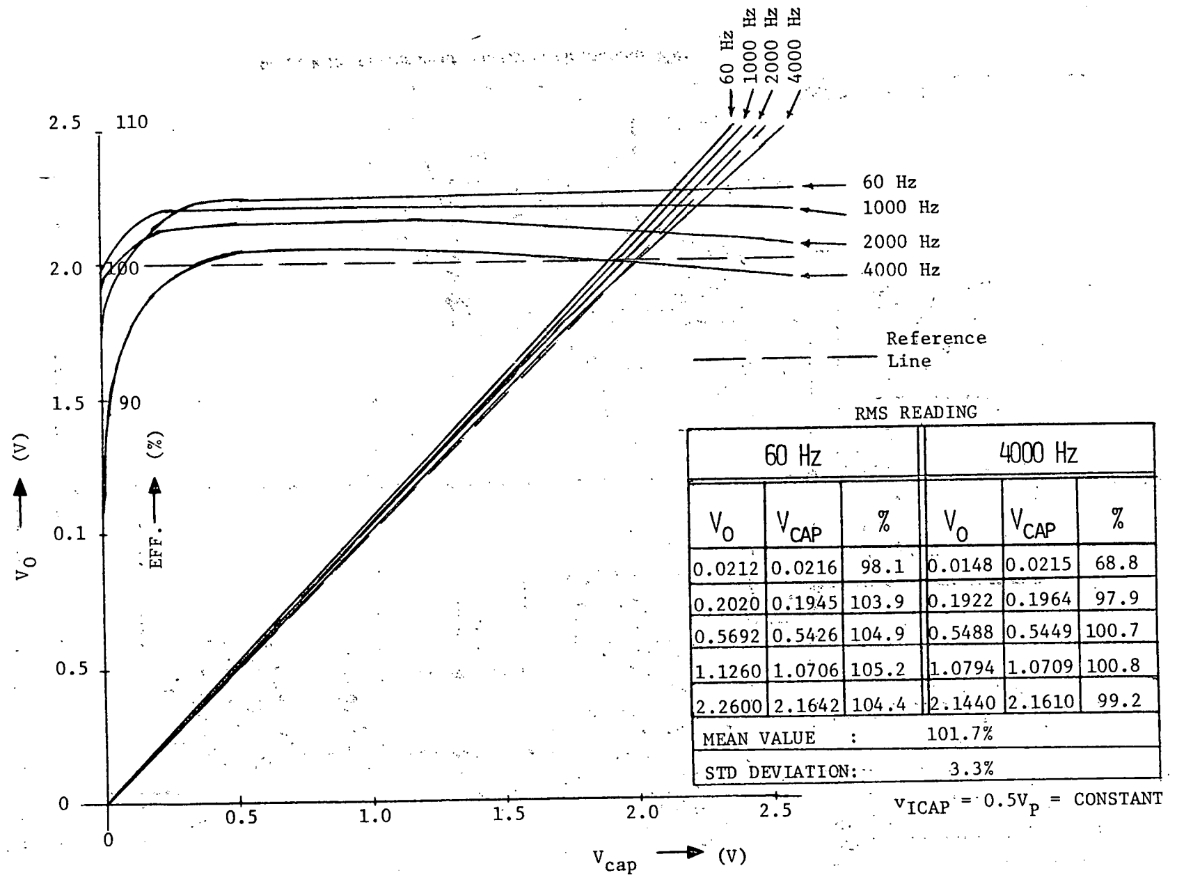
Figure 9.16. Typical calibration curve for wattmeter No. 2.
