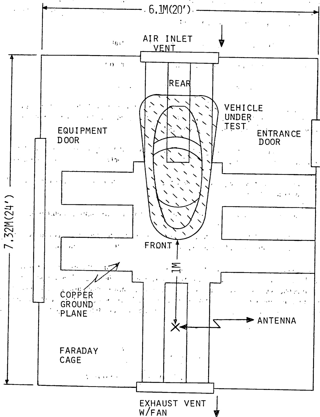
Figure 9.17. Shielded enclosure for EMI test.
