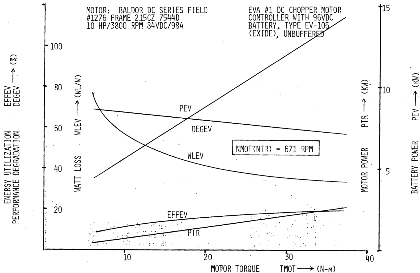
Figure 13.8C. System propulsion profile @ 671 RPM, pulsed DC power.
