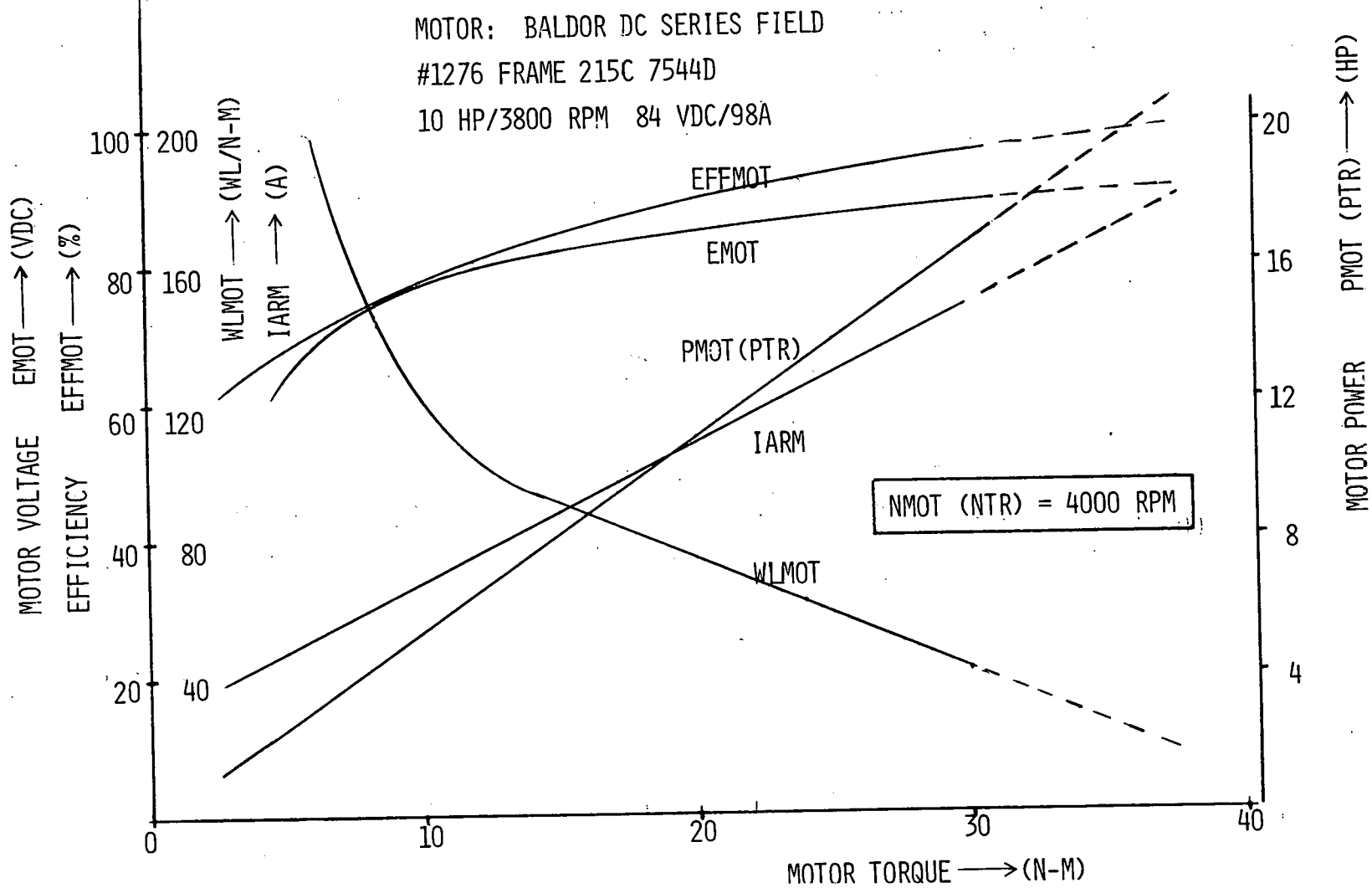
Figure 12.131. Parametric test data @ NMOT = 4000 RPM.
