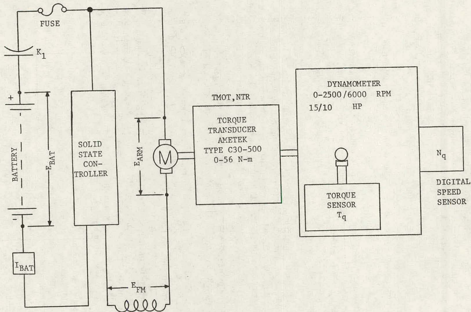
Figure 9.6. Schematic of dynamometer No. 3 DC motor test facility pulsating DC power mode.
