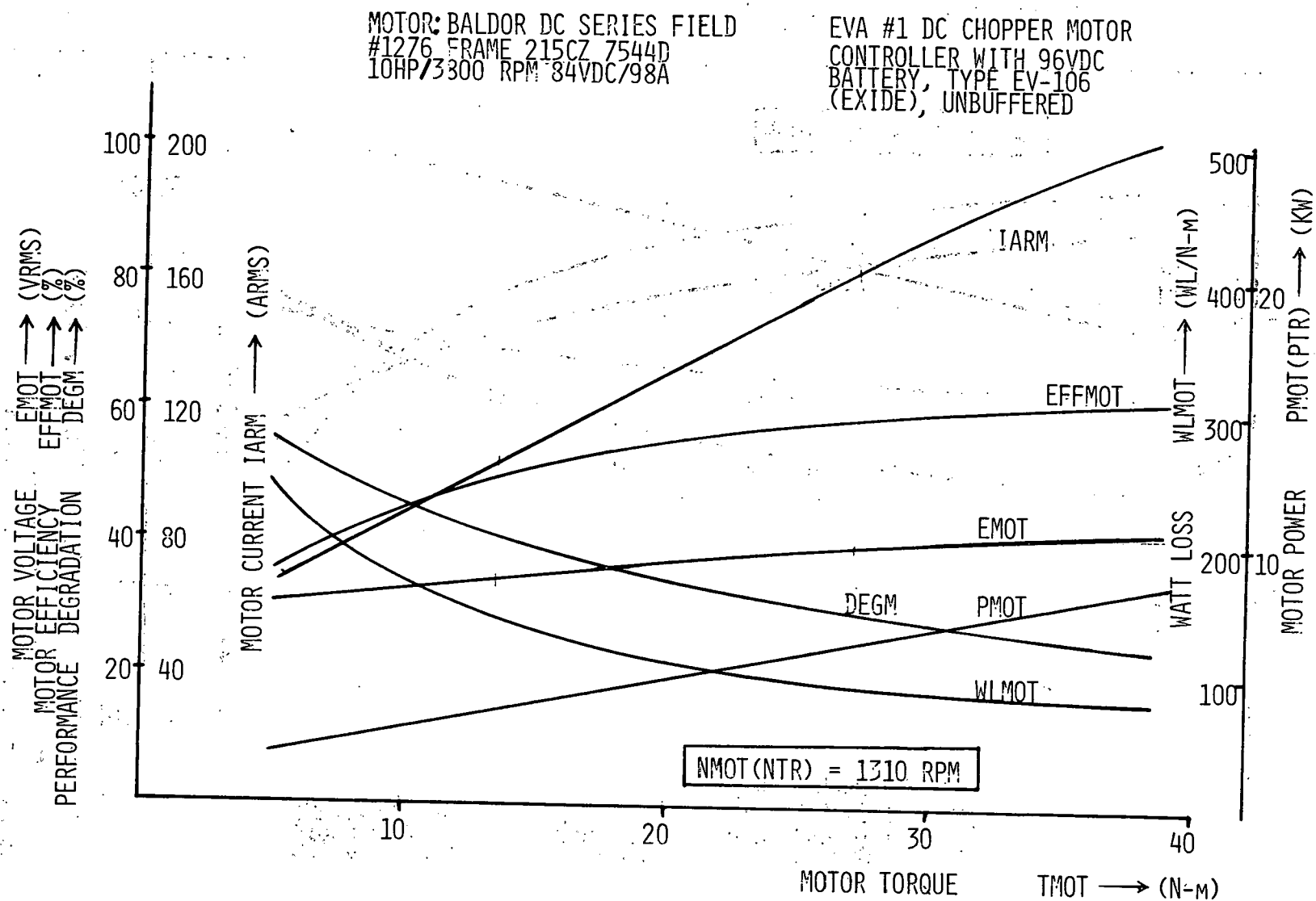
Figure 13.5F. Motor performance @ 1310 RPM, pulsed DC power.
