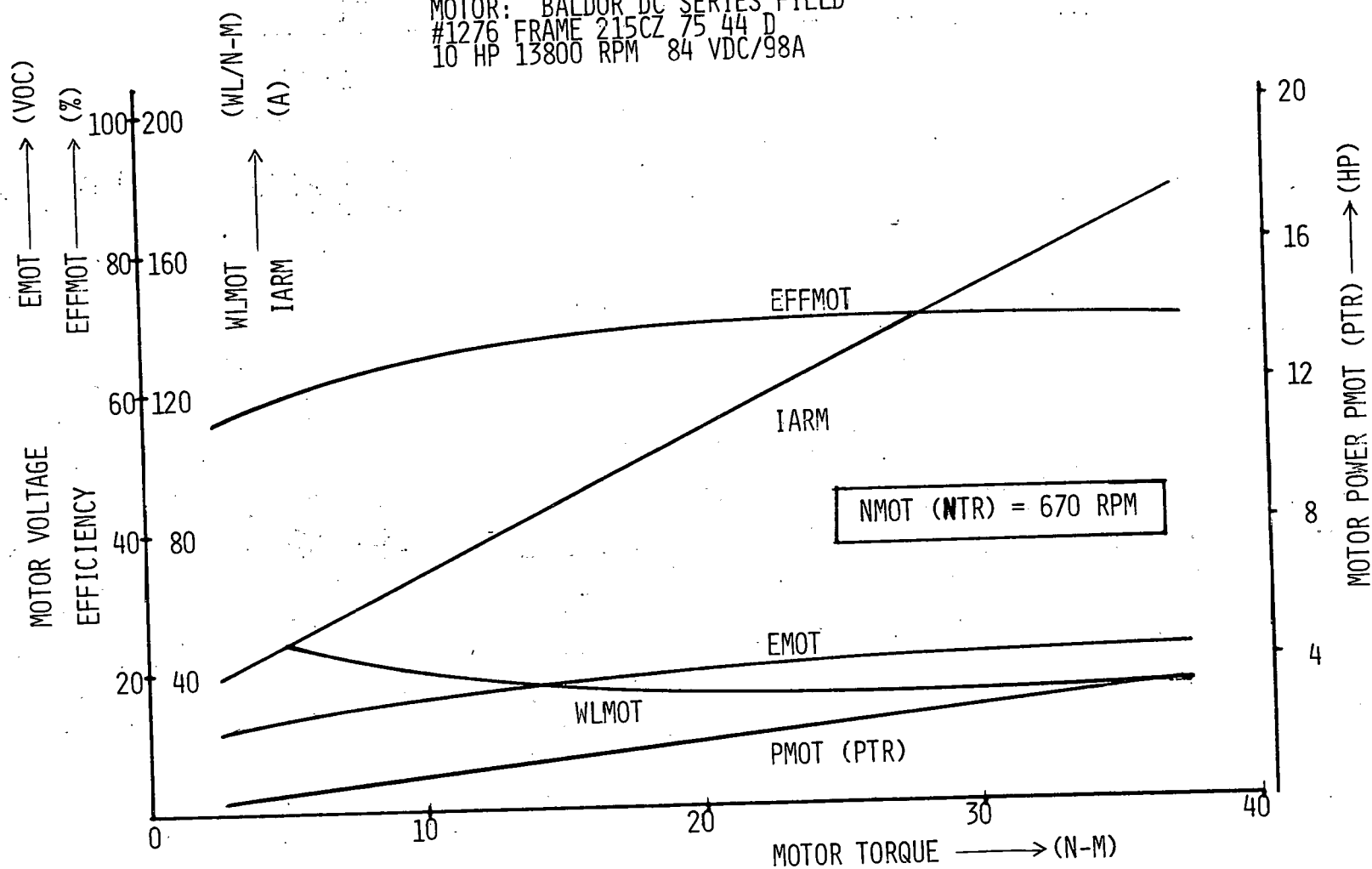
Figure 12.13A. Parametric test data @ NMOT = 670 RPM.
