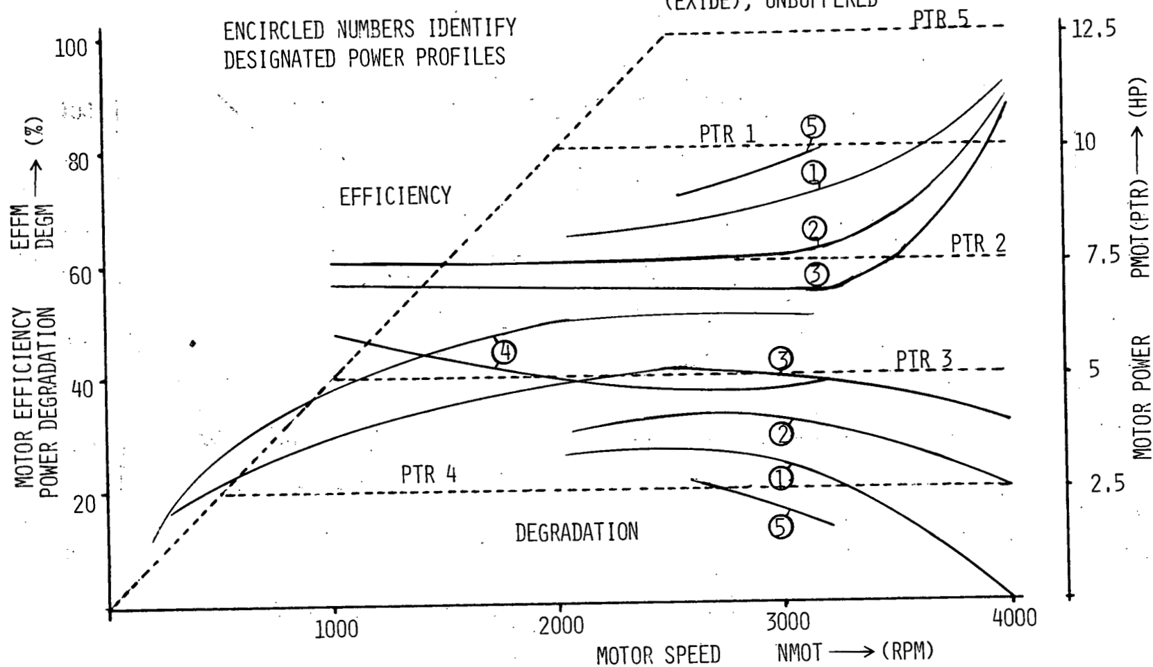
Figure 13.3. Motor propulsion profile, pulsed DC power.
