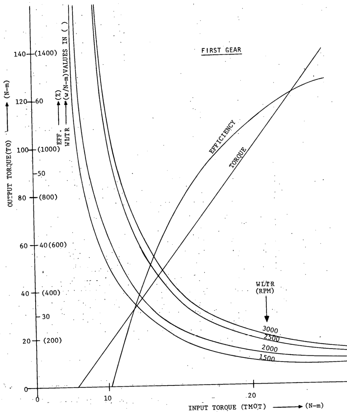
FIGURE 11.2: TRANSMISSION PERFORMANCE TEST IN FIRST GEAR (GR1)
