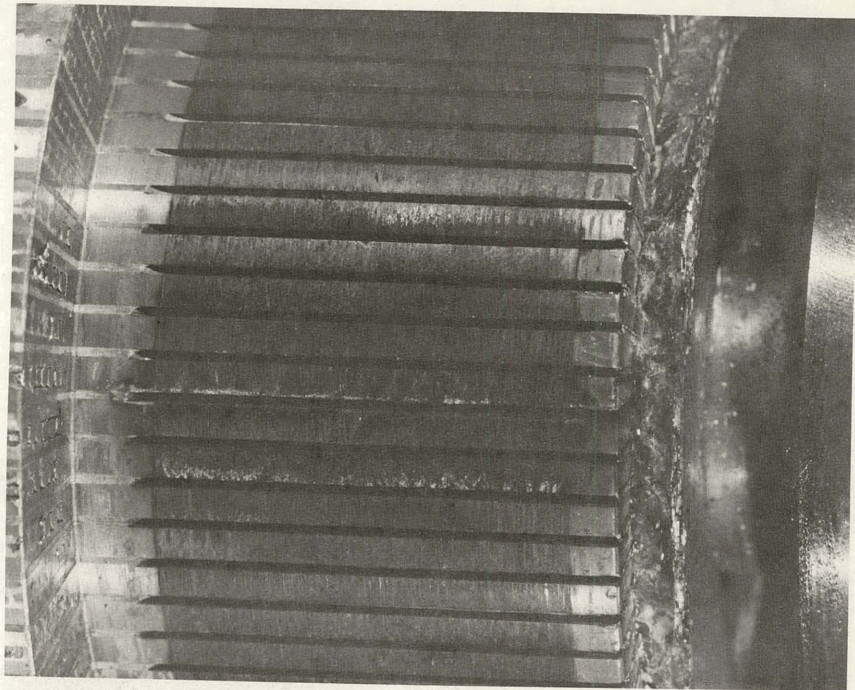
Figure 6.2. Motor damage to commutator caused by disintegration of soft solder joints.
