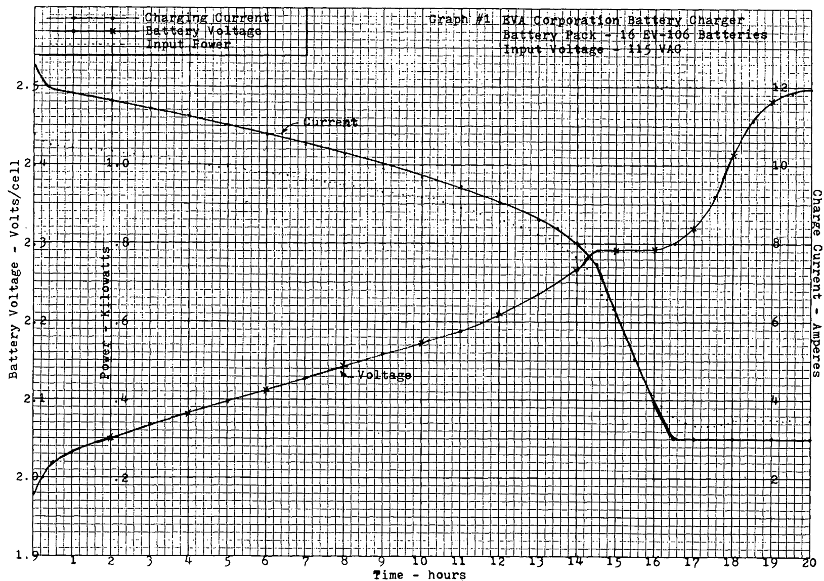
Figure E7. Battery Charger Current and Voltage Slopes.
