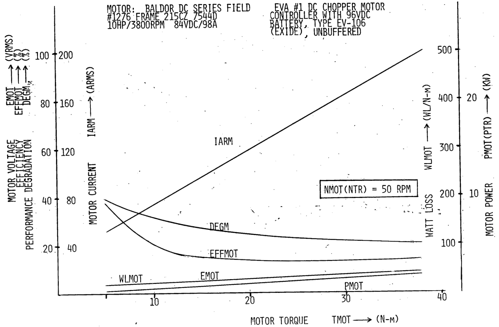
Figure 13.5A. Motor performance @ 50 RPM, pulsed power.
