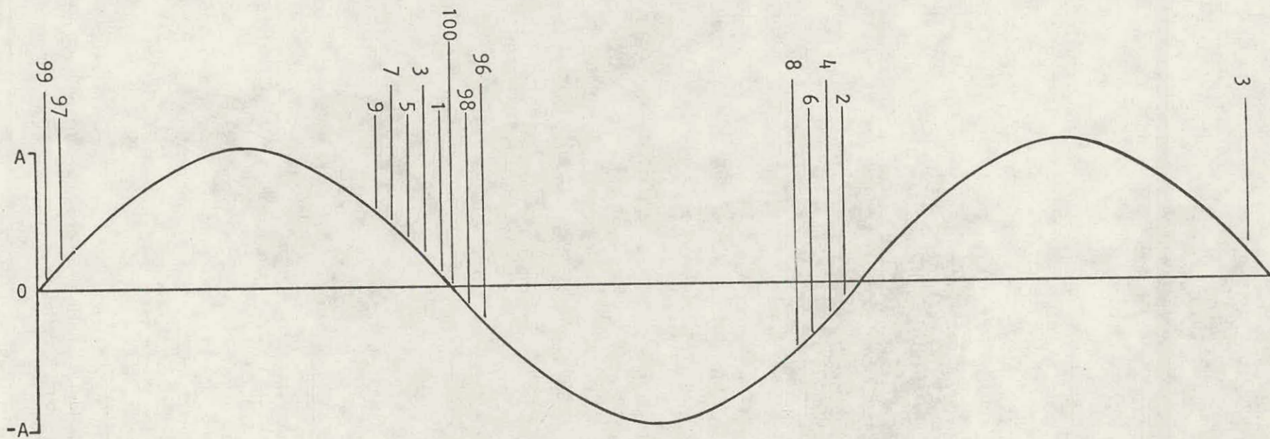
Figure 8.4. Consecutive sample positions for a 100 point sample, waveforms overlaid.
