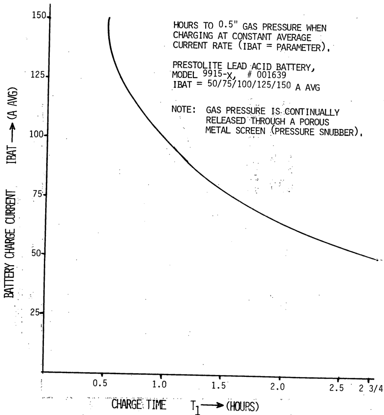
Figure 15.1. Battery maximum charge current vs. time prior to gasing.
