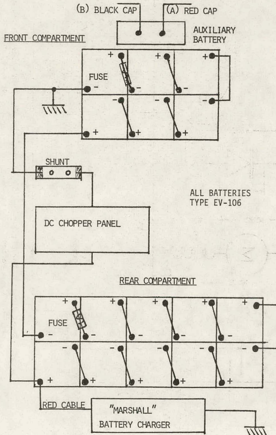
Figure 9.9B. Battery hook-up.
