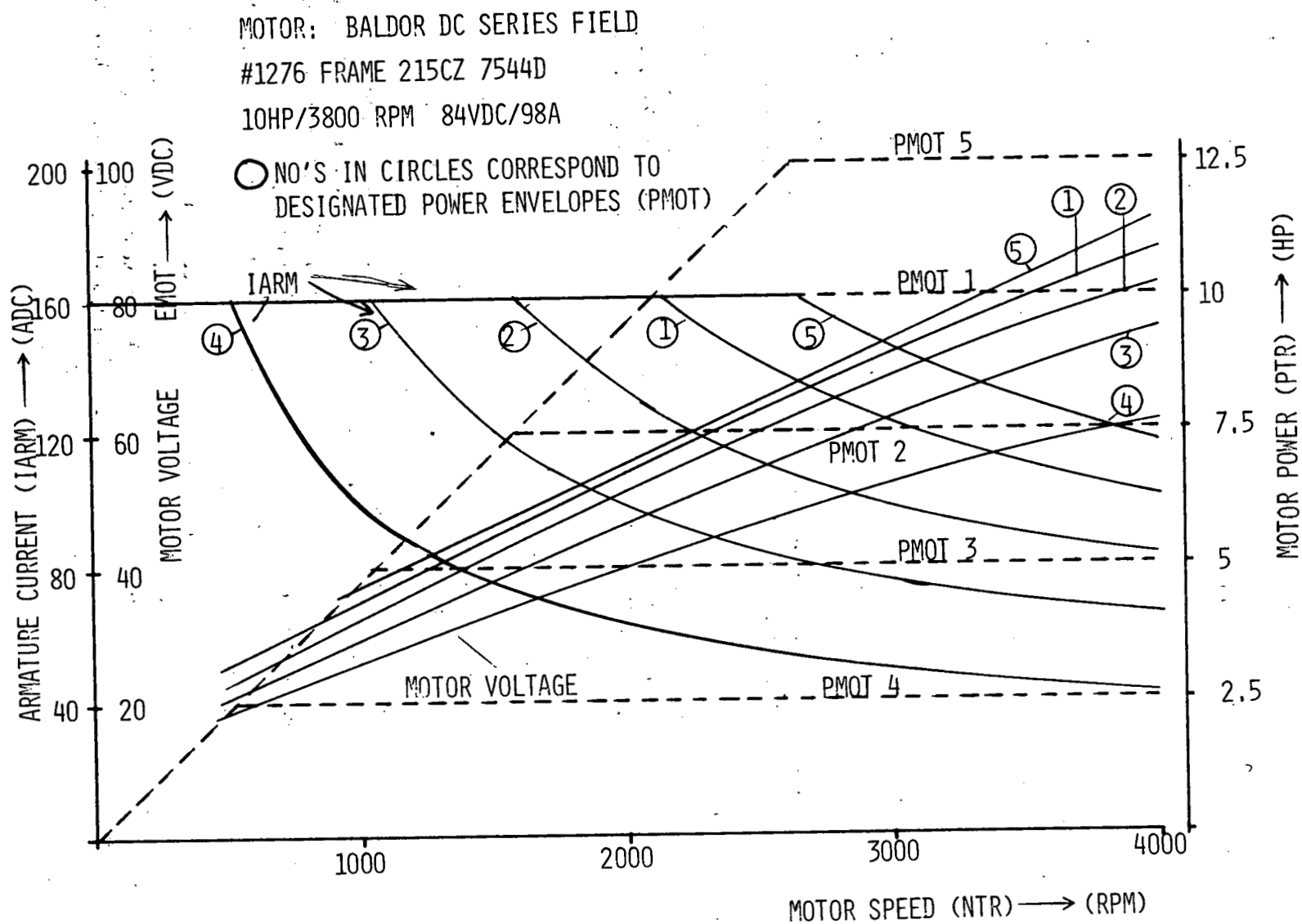
Figure 12.11. Parametric test data, motor current and voltage.
