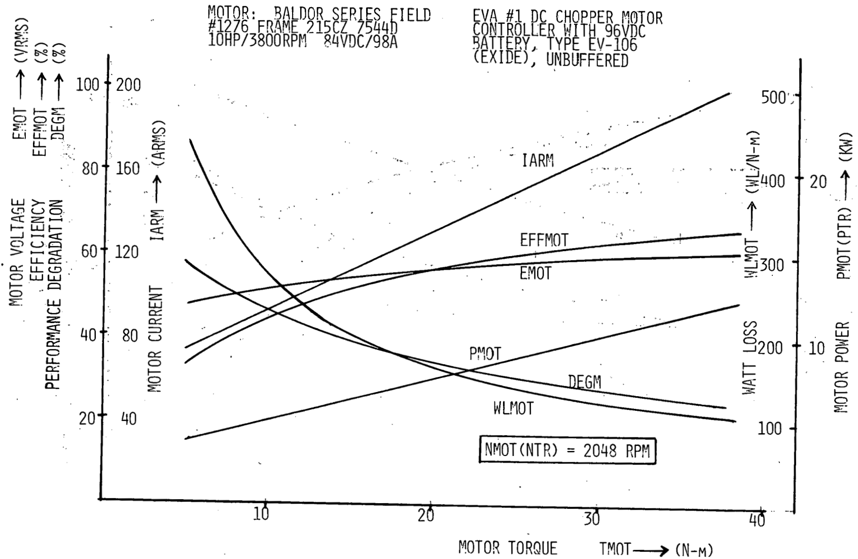
Figure 13.5H. Motor performance @ 2048 RPM, pulsed DC power.
