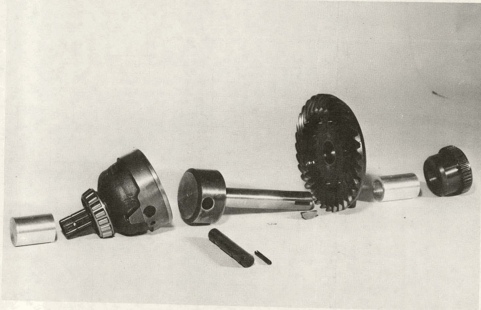
Figure 9.1. Adaptor to lock differential.
