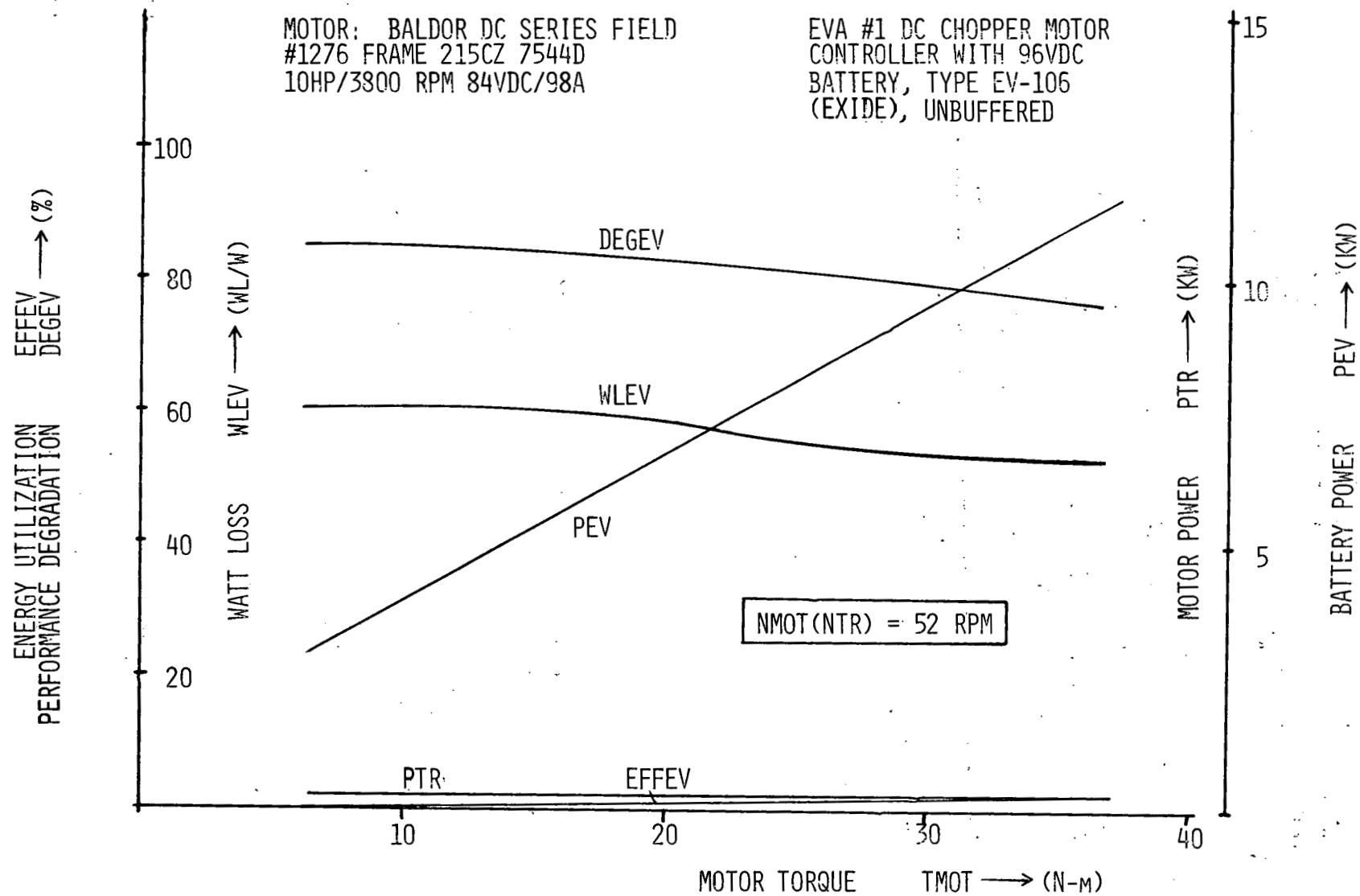
Figure 13.8A. System propulsion profile @ 52 RPM, pulsed DC power.
