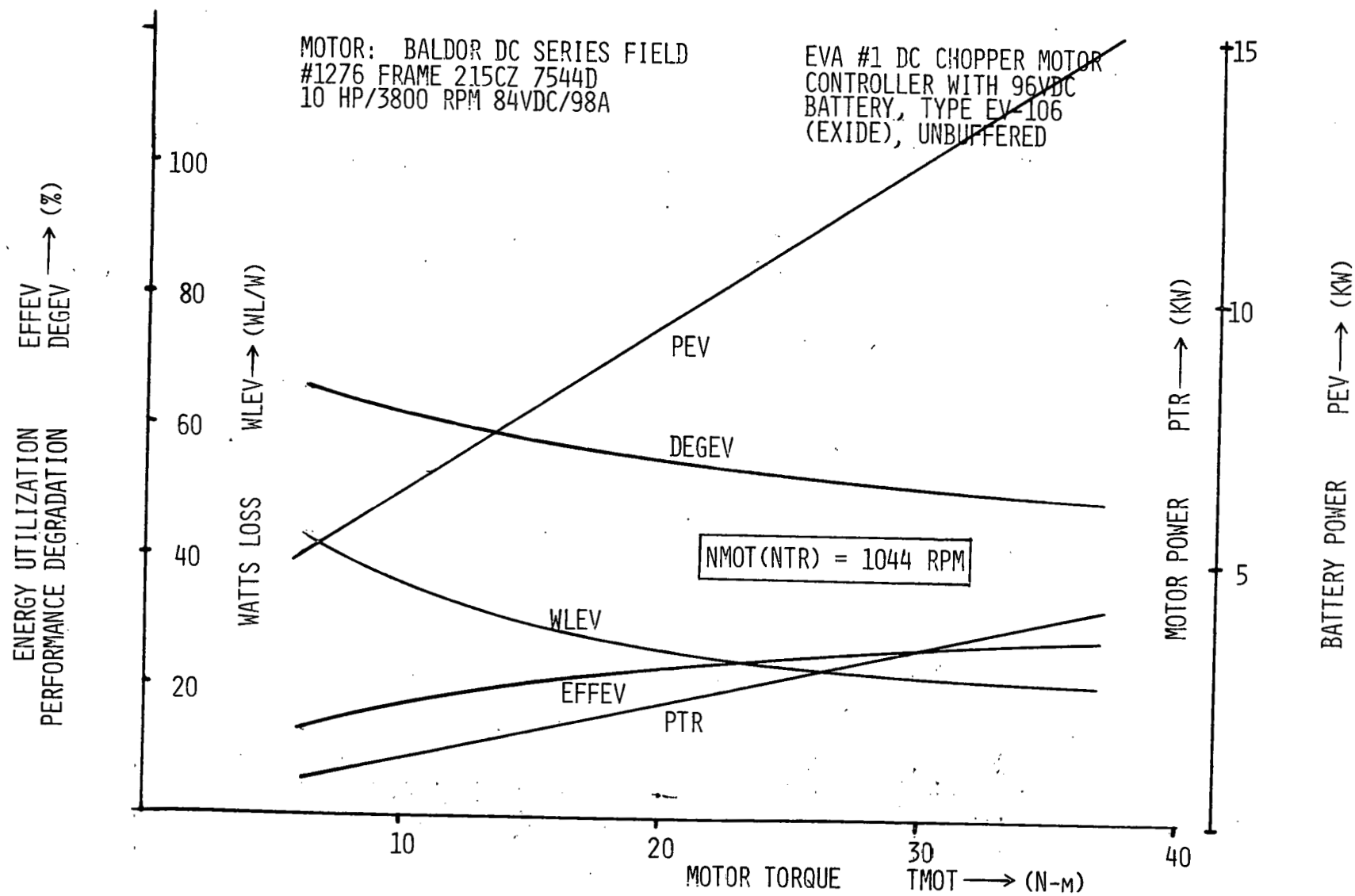
Figure 13.8E. System propulsion profile @ 1044 RPM, pulsed DC power.
