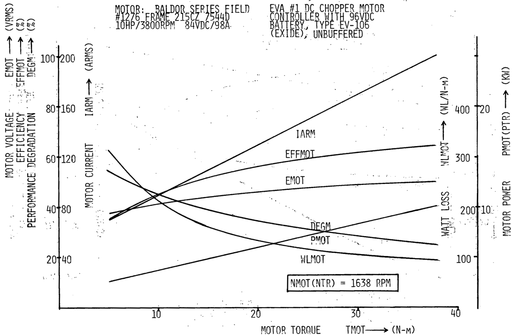
Figure 13.5G. Motor performance @ 1638 RPM, pulsed DC power.
