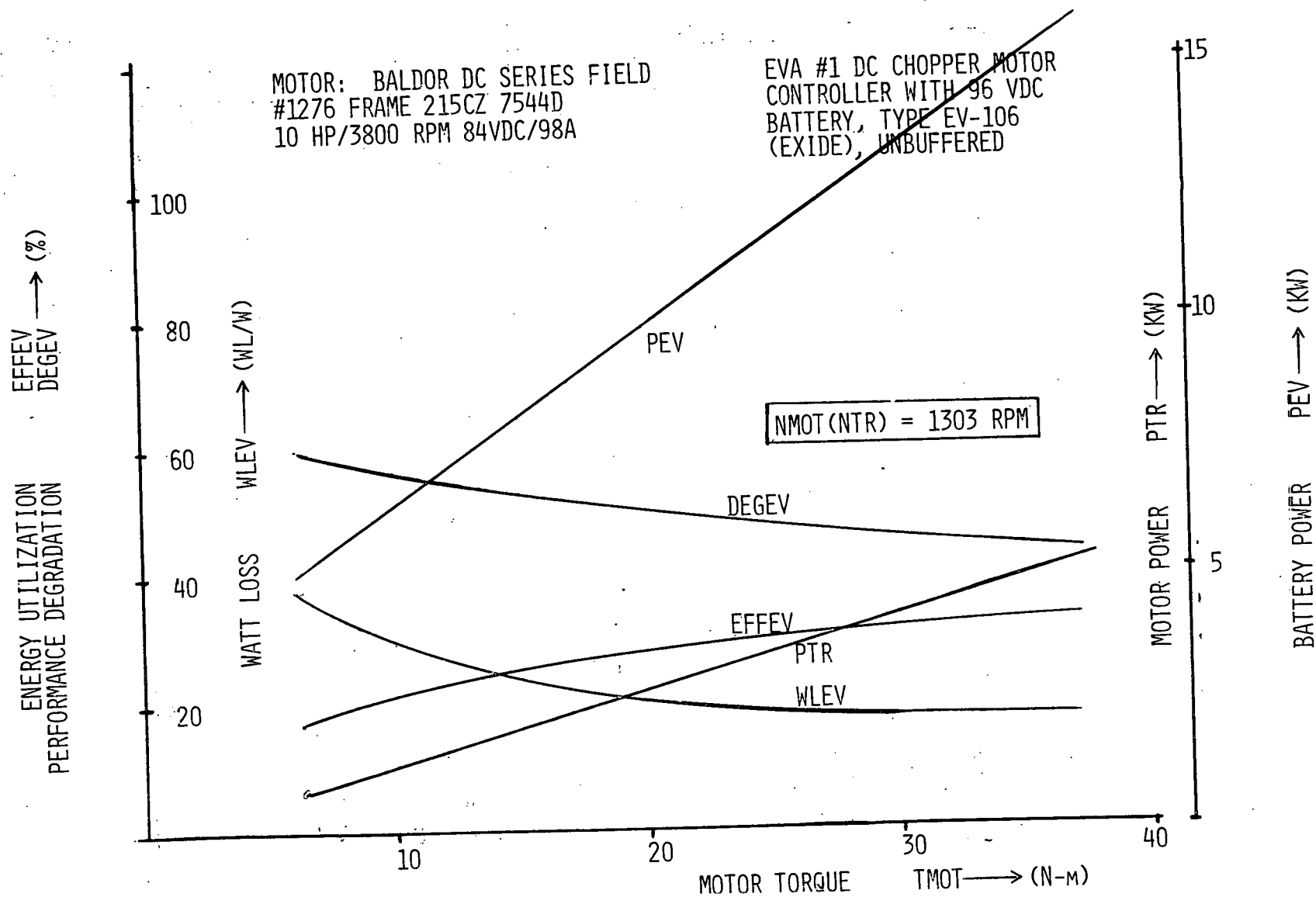
Figure 13.8F. System propulsion profile @ 1303 RPM, pulsed DC power.
