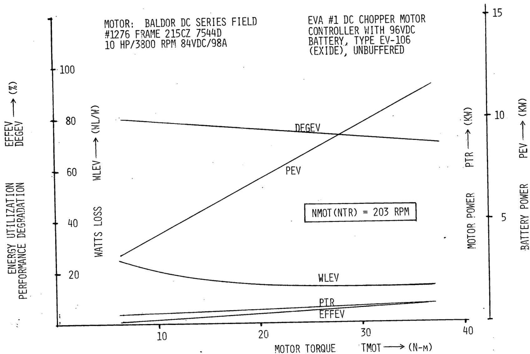
Figure 13.8B. System propulsion profile @ 203 RPM, pulsed DC power.
