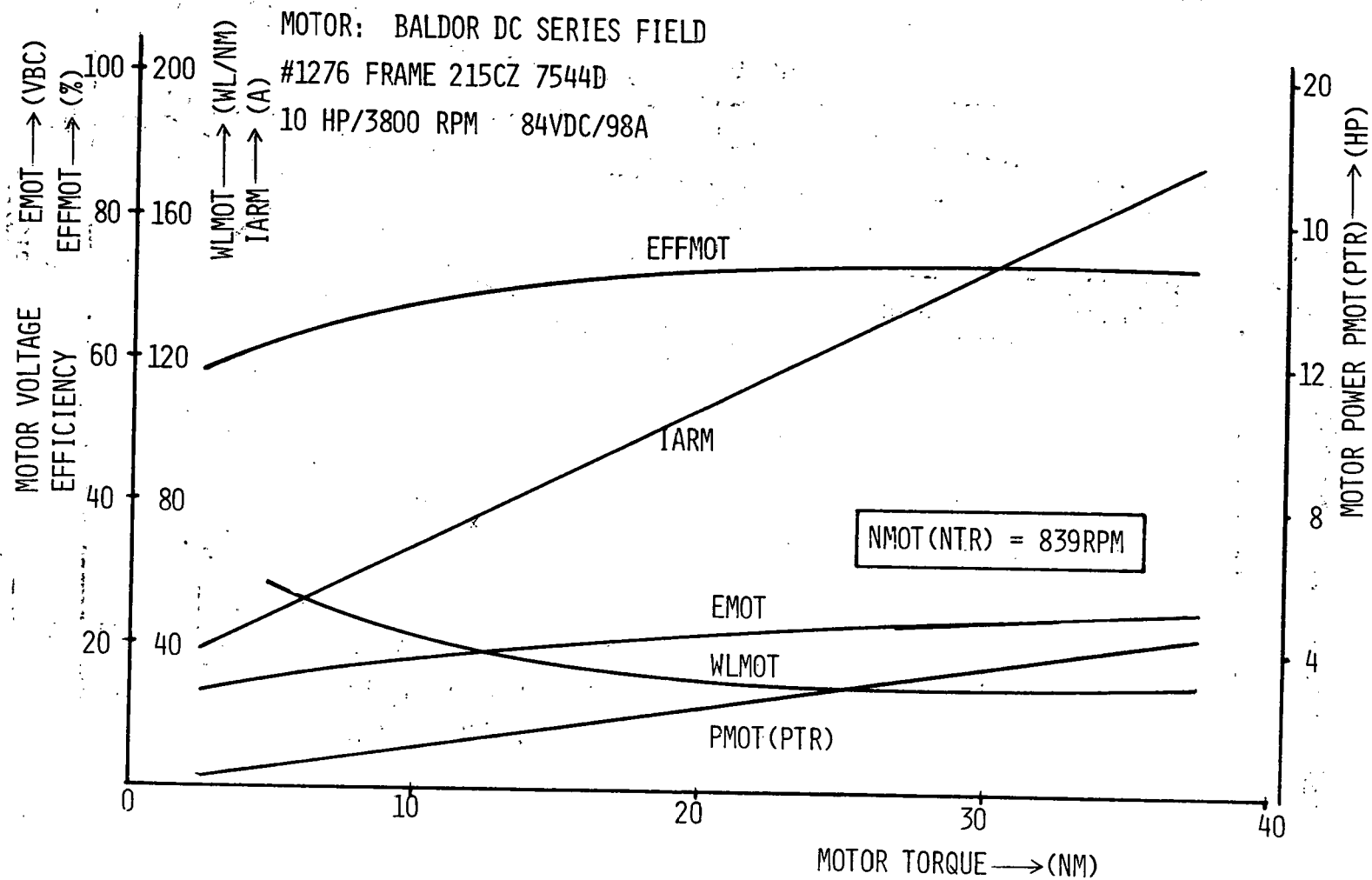
12.13B. Parametric test data @ NMOT = 839 RPM.
