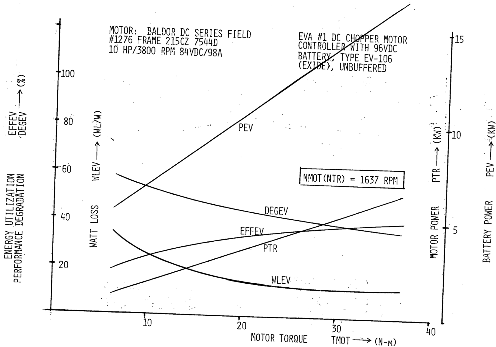
Figure 13.8G. System propulsion profile @ 1637 RPM pulsed DC power.
