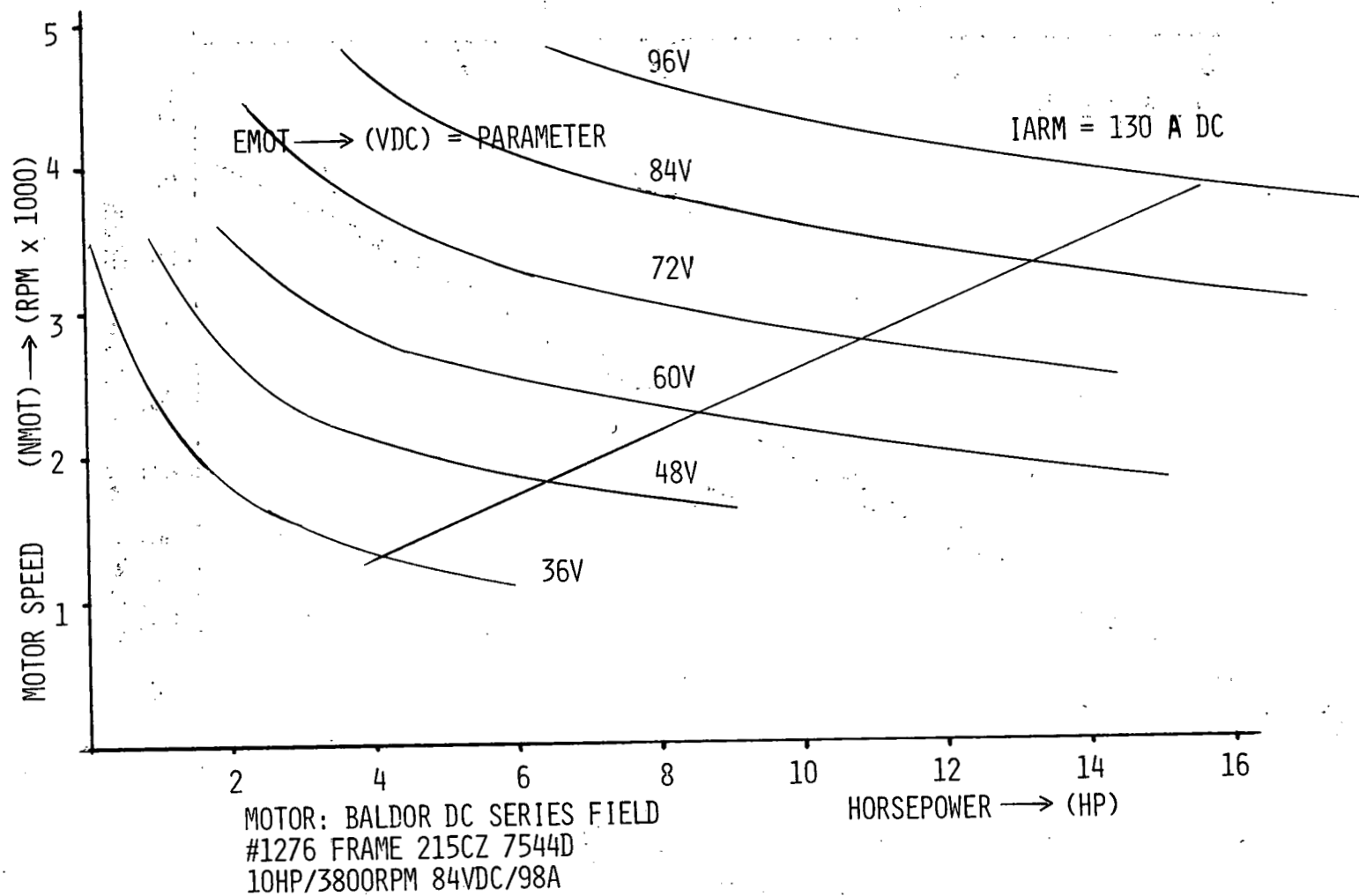
Figure 12.10. Motor speed vs. shaft power.
