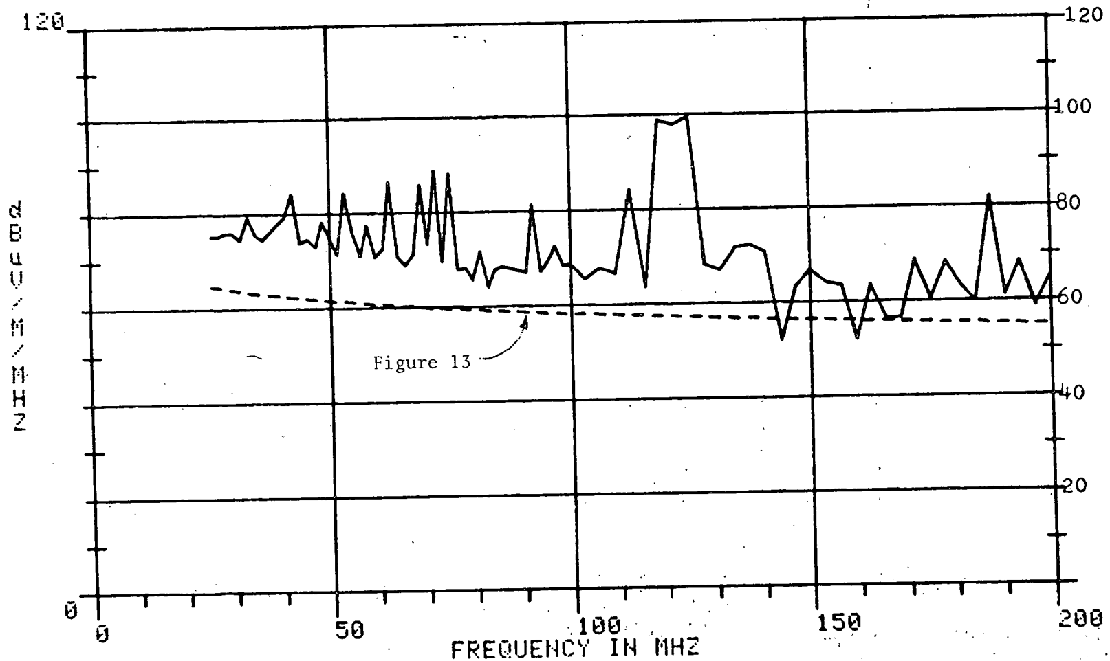
Figure 16.4. EMI test, 200A load.
