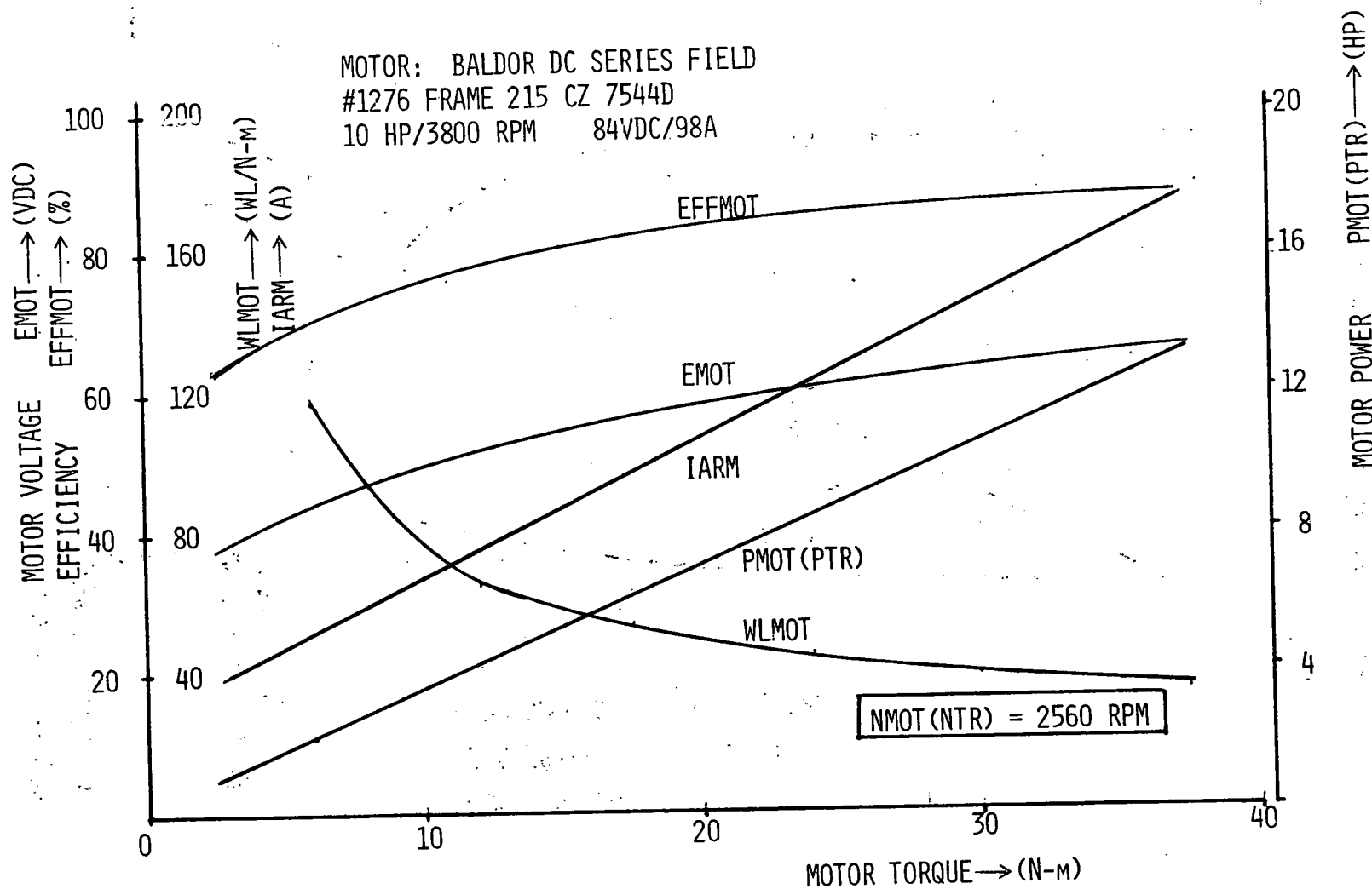
Figure 12.13G. Parametric test data @ NMOT = 2560 RPM.
