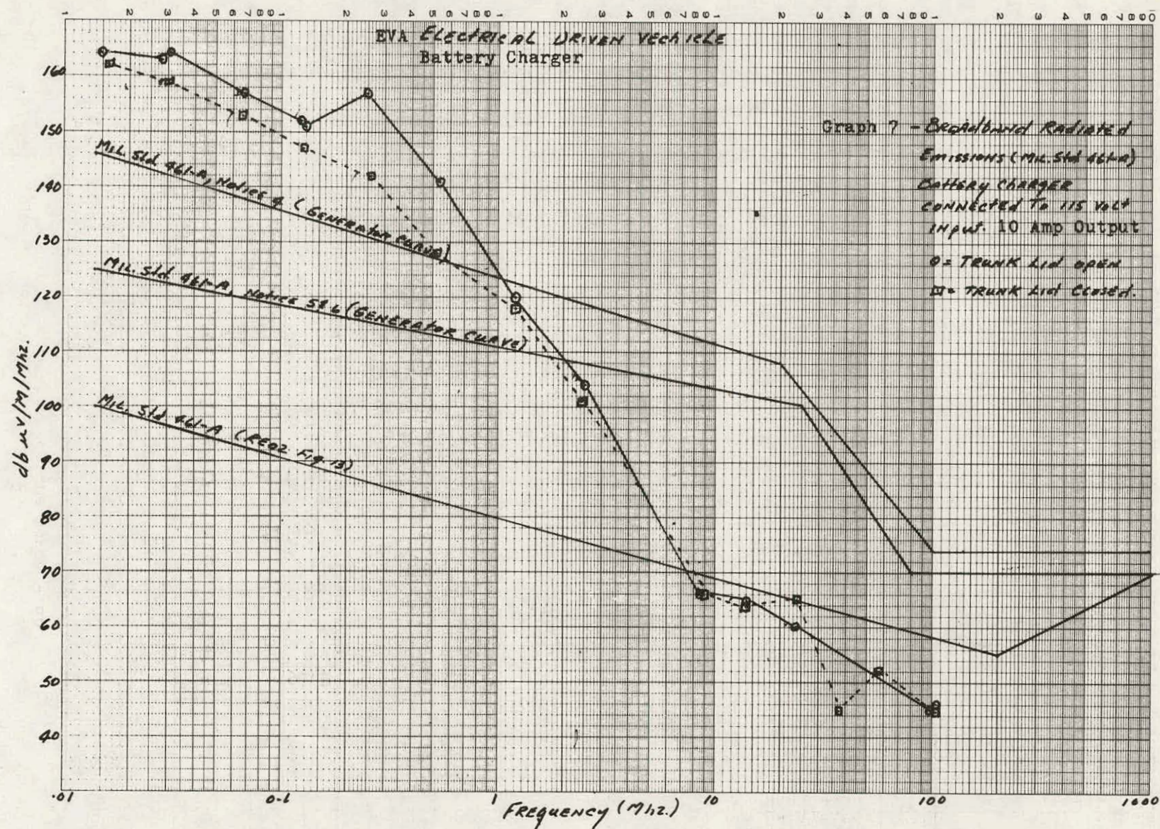
Figure E13. Broadband Radiated EMI.
