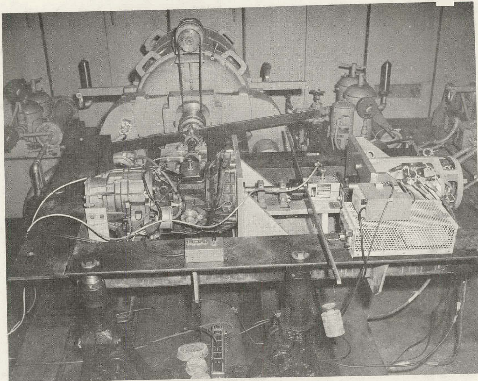
Figure 9.4 Calibration arm for torque sensor
