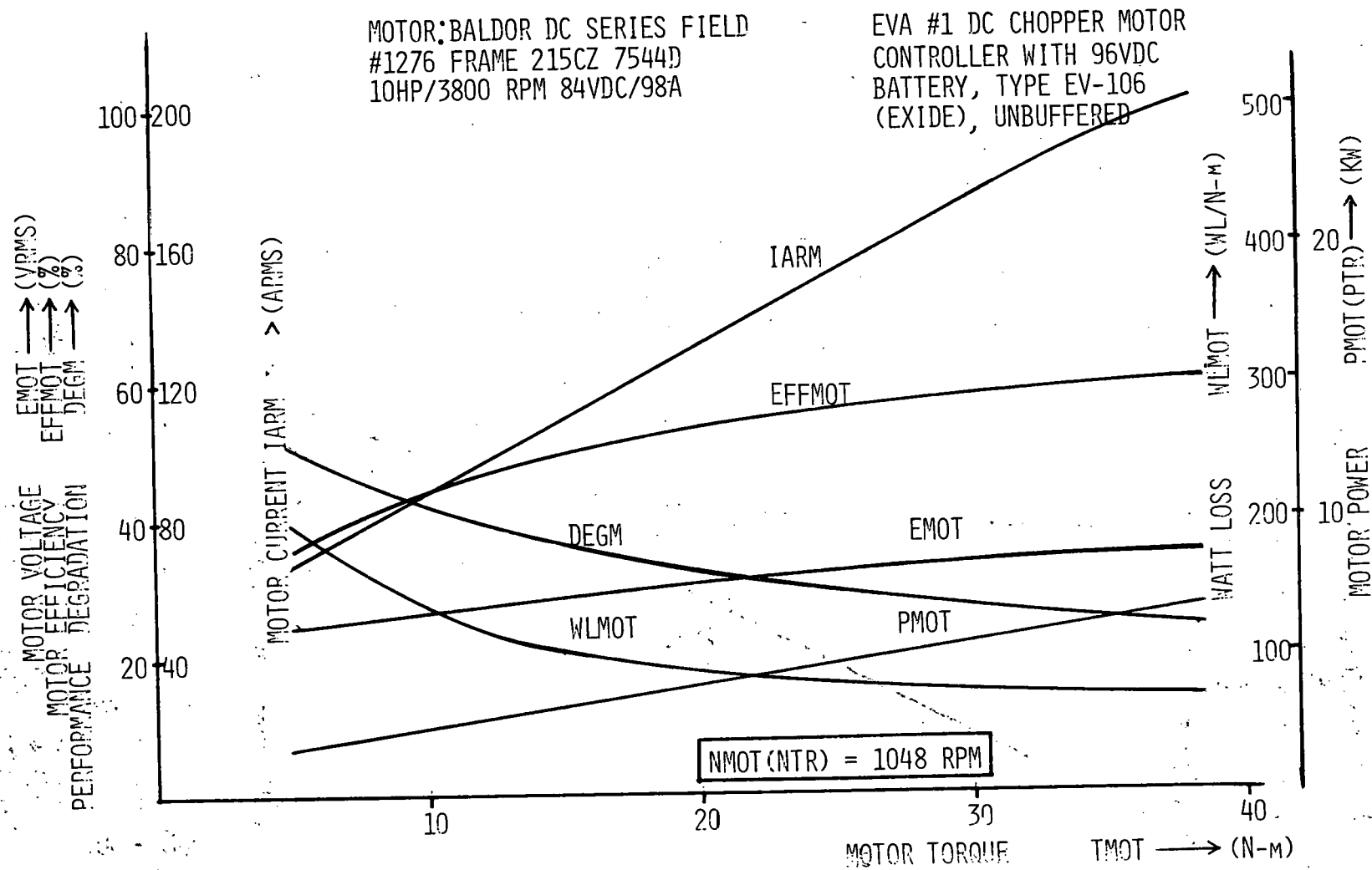
Figure 13.5E. Motor performance @ 1048 RPM, pulsed DC power.
