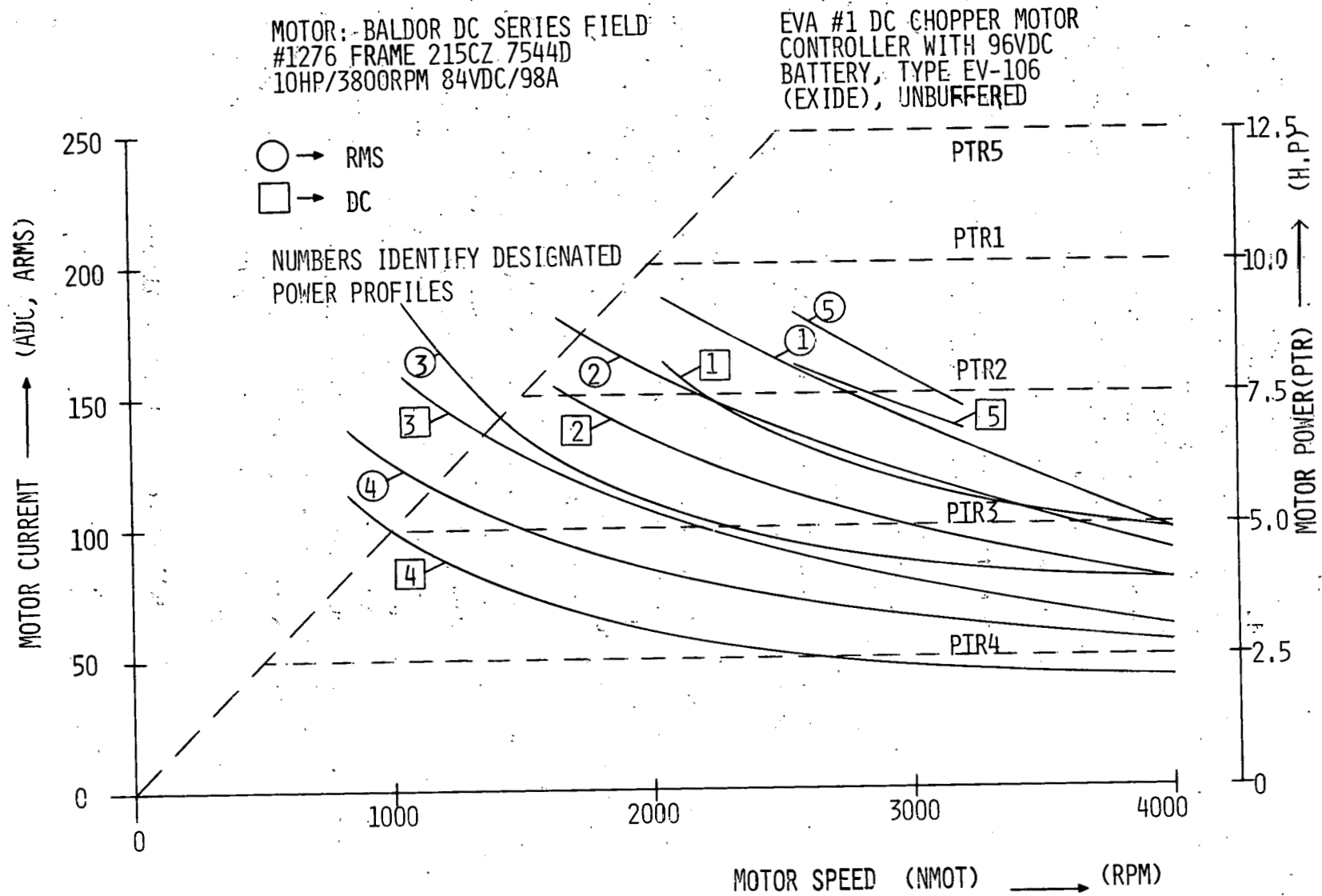
Figure 13.1. Motor propulsion profile, pulsed DC power.
