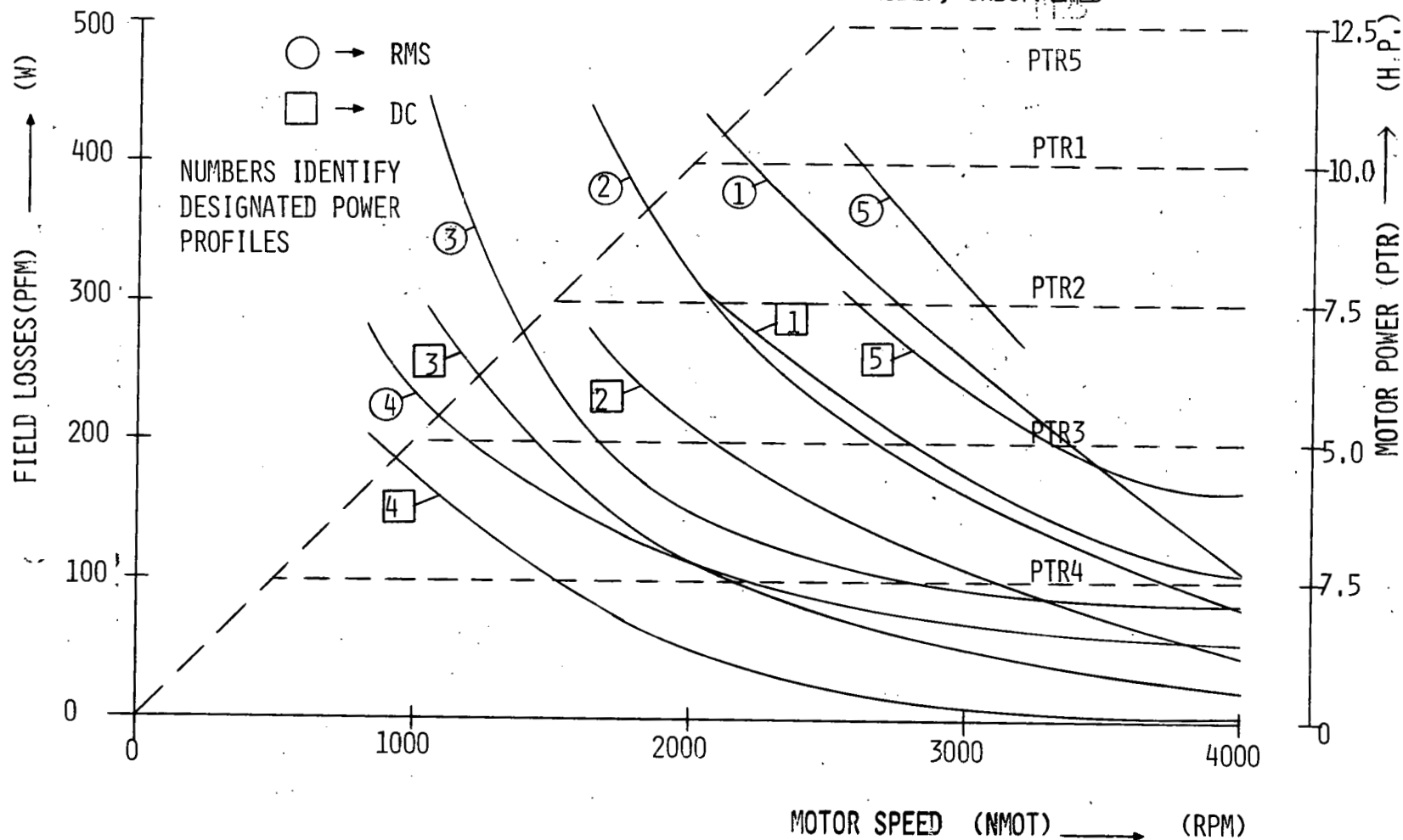
Figure 13.2. Motor propulsion profile, pulsed DC power.
