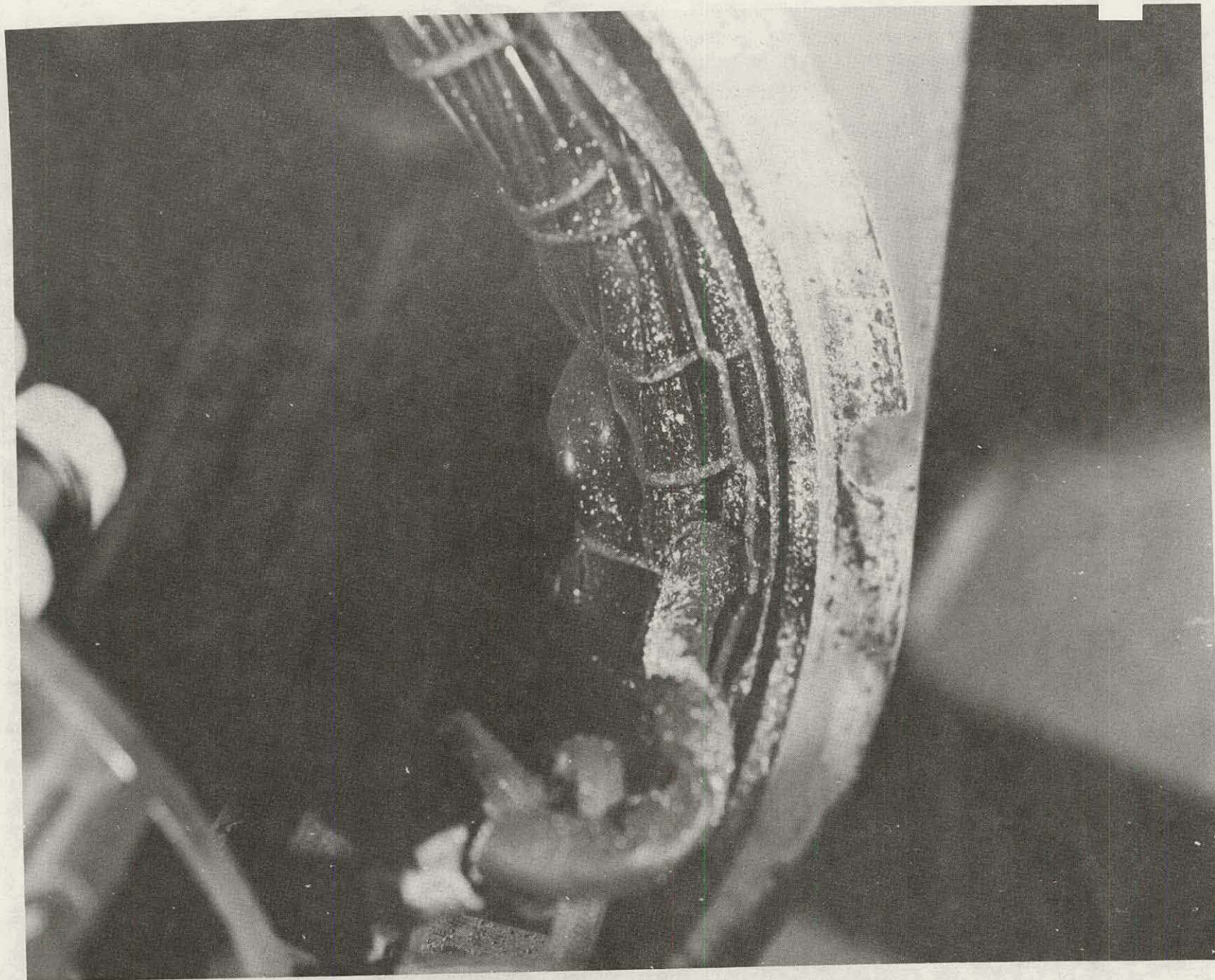
Figure 6.3. Motor damage to field winding caused by disintegration of soft solder joints.
