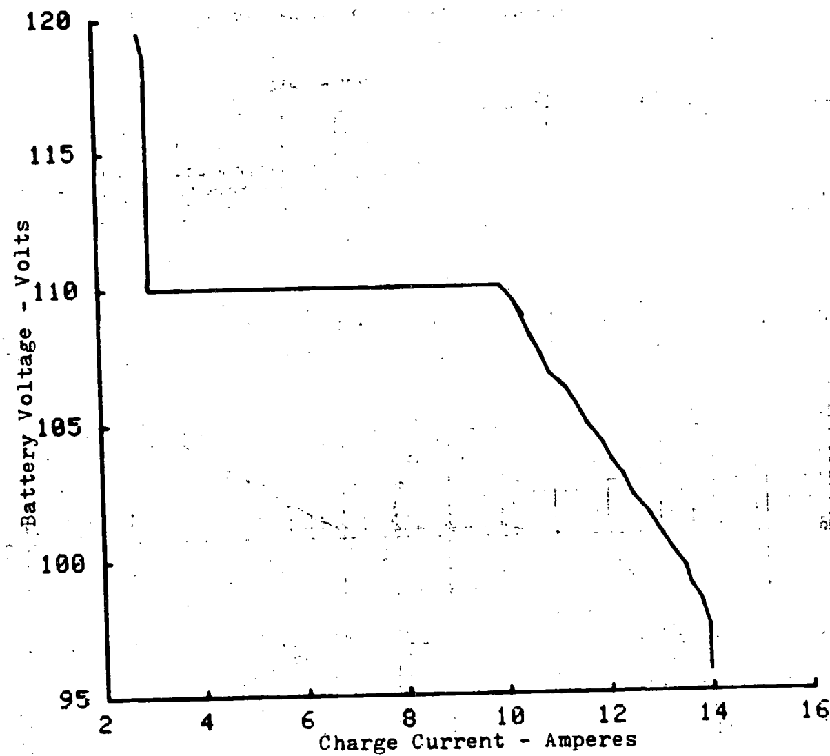
Figure E10. Battery Charger Voltage/Current Slope, Graph 4.
