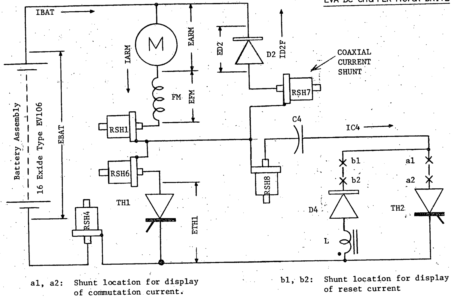
Figure 9.10. In-circuit location of coaxial current shunts during testing.
