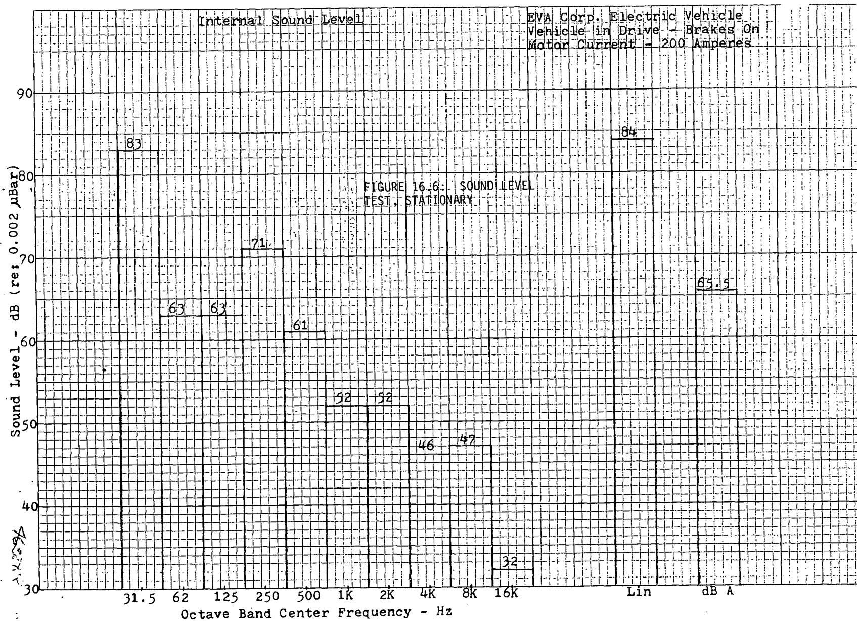
Figure 16.6. Sound level test, stationary.
