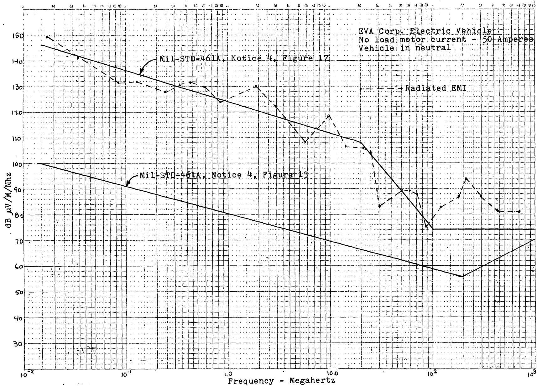
Figure 16.1. EMI test, no load.
