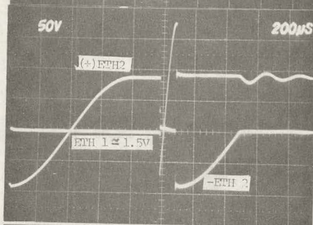
FIG. 14.3A: ETH1 vs. blocking voltage of commutating thyristor (TH2). ETH2 = 50V/cm ETH1 = 50V/cm
