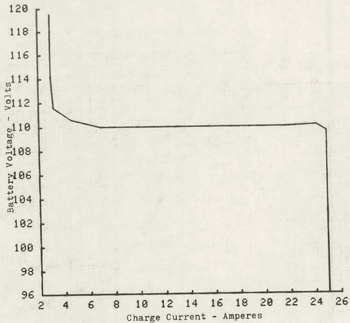
Figure E12. Battery Charger Voltage/Current Slope, 240 V RMS.
