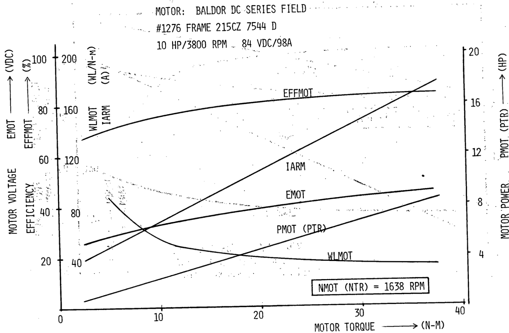
Figure 12.13E. Parametric test data @ NMOT = 1638 RPM.
