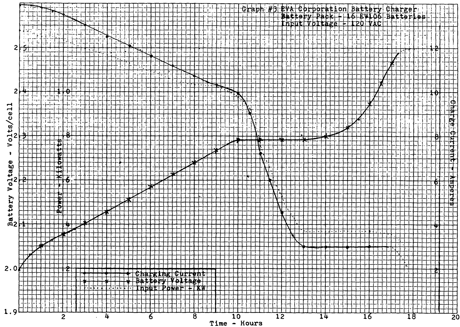
Figure E9. Battery Charger Power Consumption, 120 V RMS.
