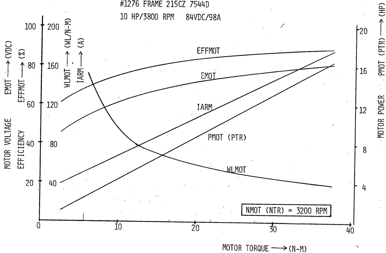
Figure 12.13H. Parametric test data @ NMOT = 3200 RPM.
