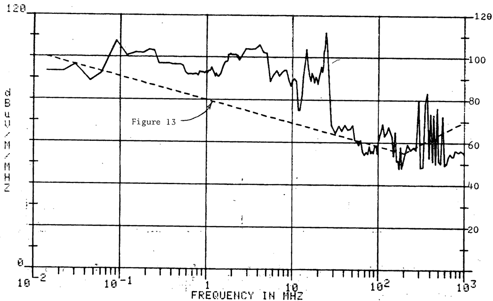
Figure 16.3. EMI test, 200A load.
