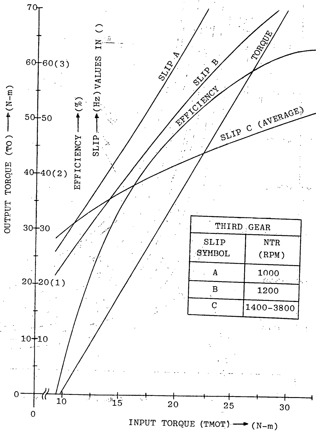
Figure 11.5. Transmission performance test in third gear (GR3).
