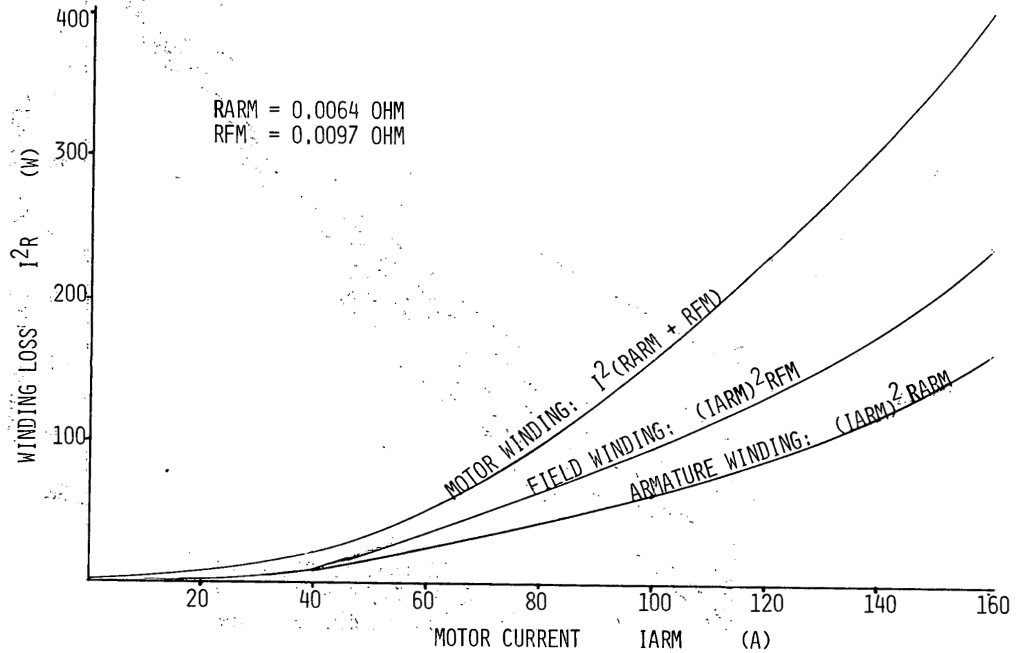
Figure 12.5. Motor winding dissipation.
