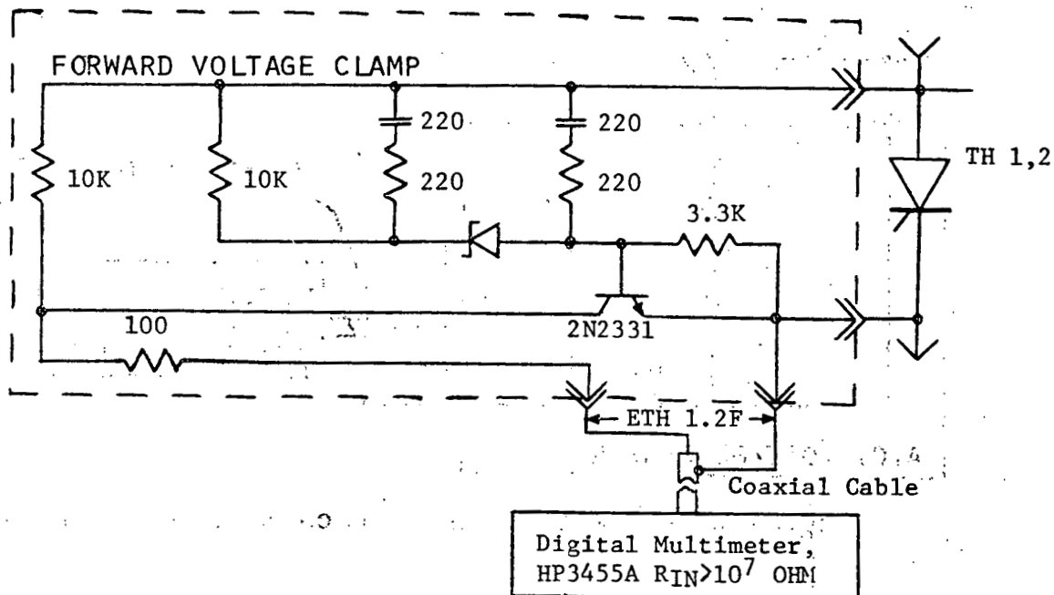
Figure 9.12. Adaptor circuit for measurement of thyristor forward voltage drop.
