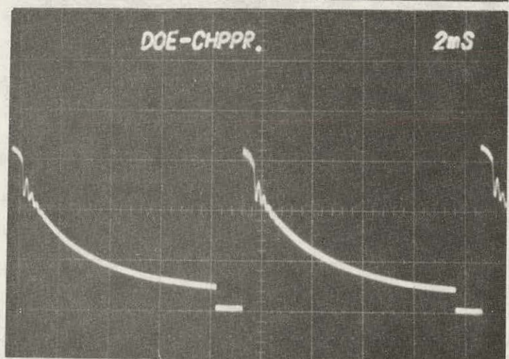
FIG. 14.5B: Freewheeling diode (D2) current (ID2F).
