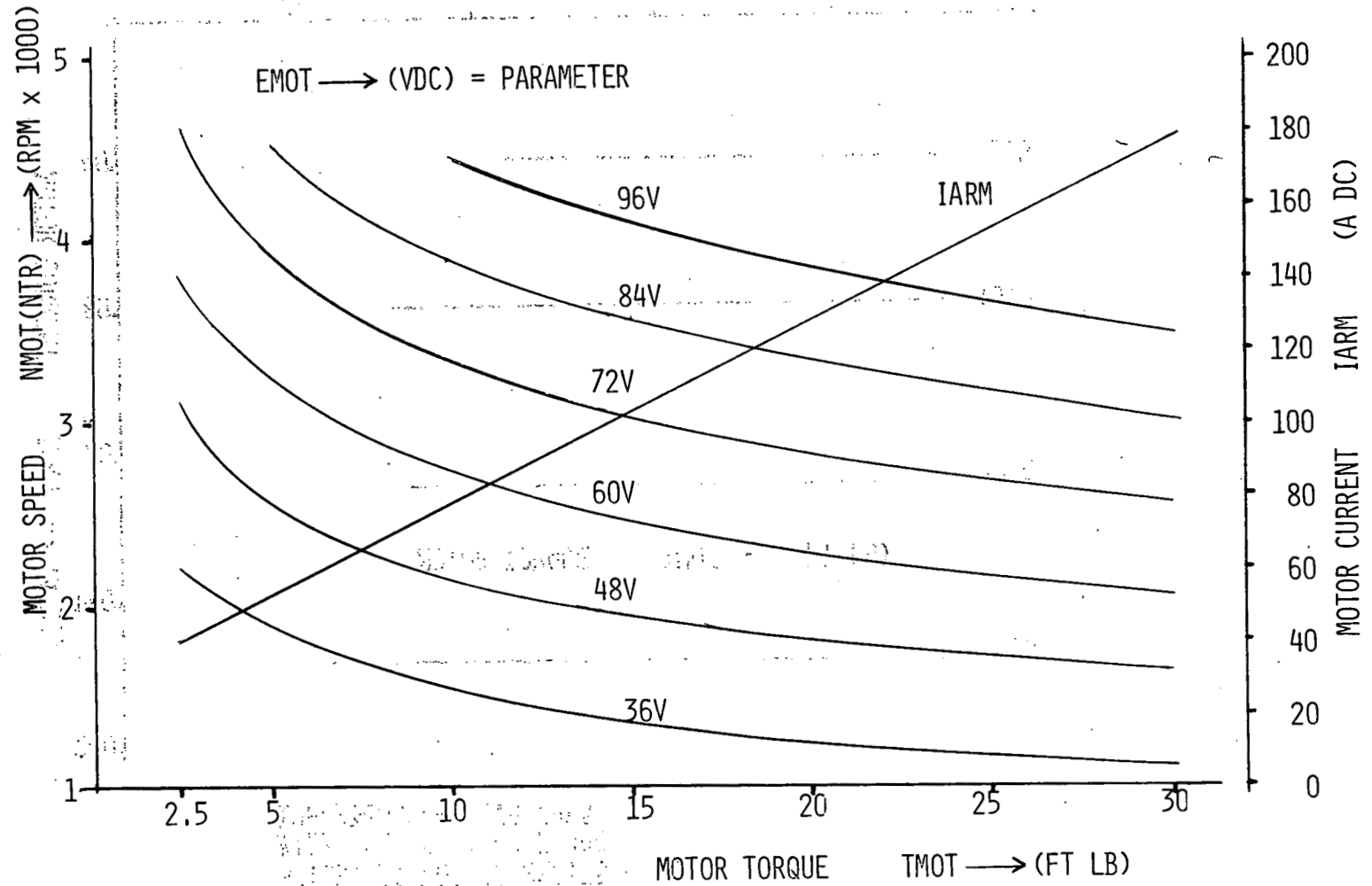
Figure 12.8. Motor torque vs. current and speed.
