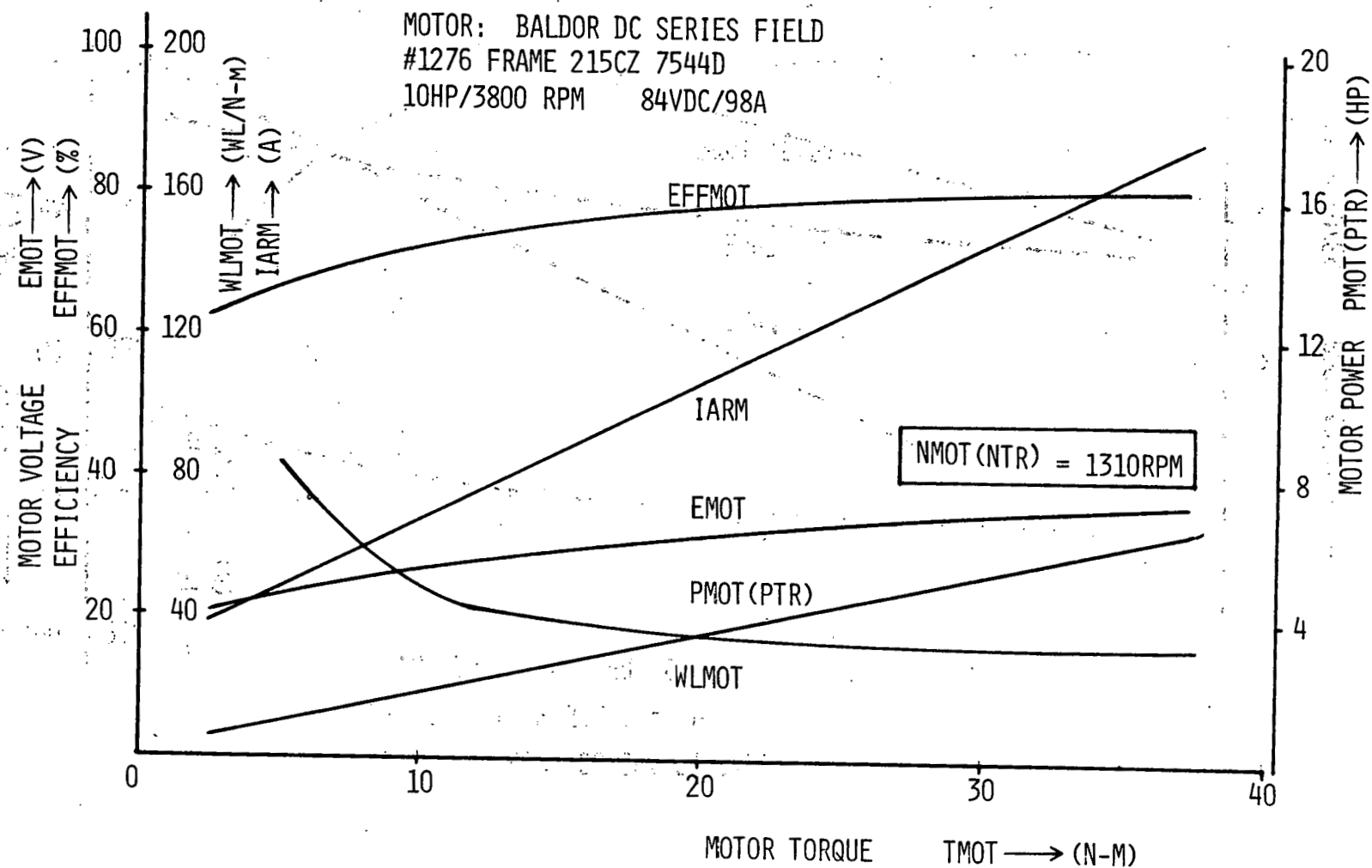
Figure 12.13D. Parametric test data @ NMOT = 1310 RPM.
