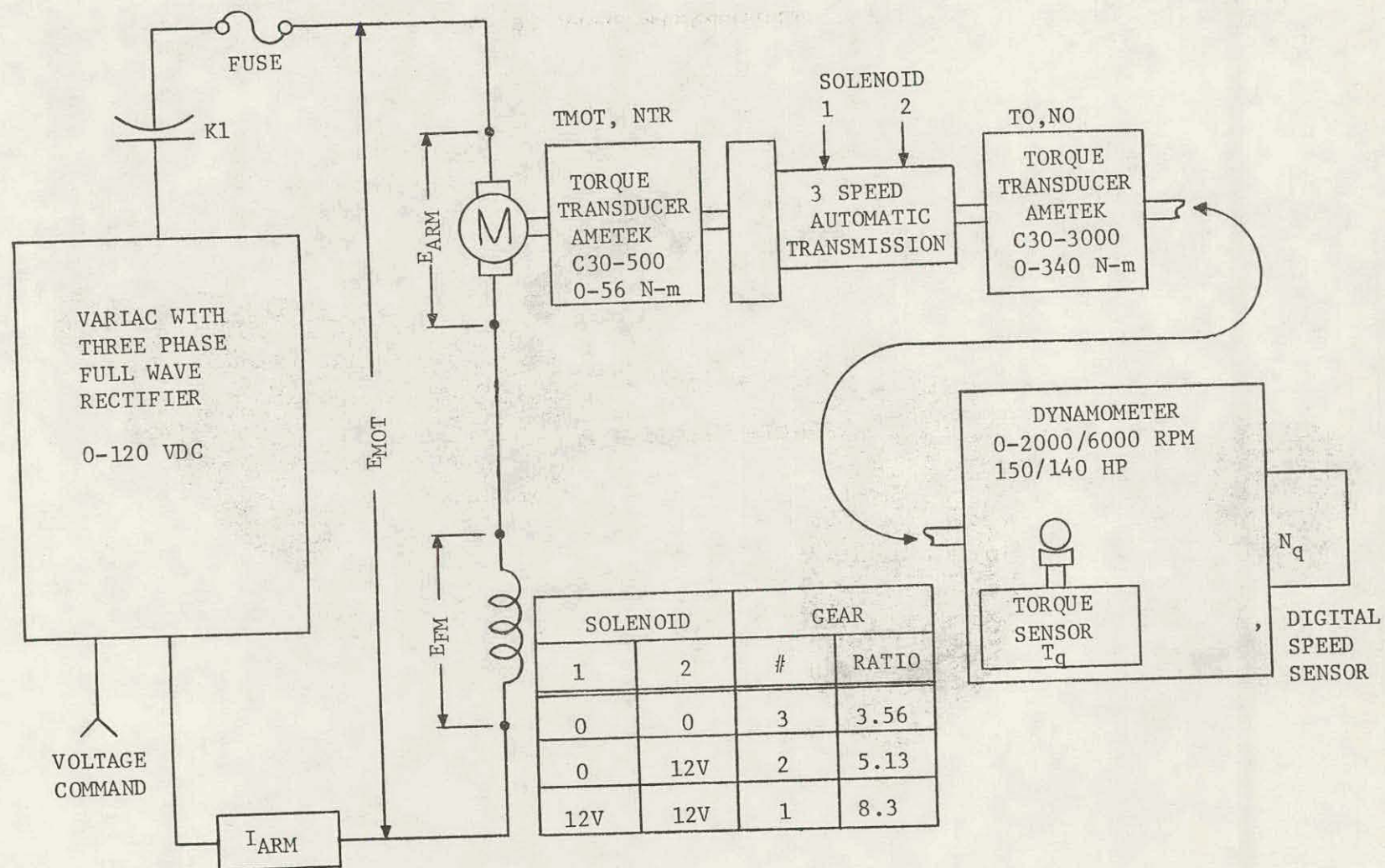
Figure 9.2. Schematic of dynamometer No. 1 transmission test facility.
