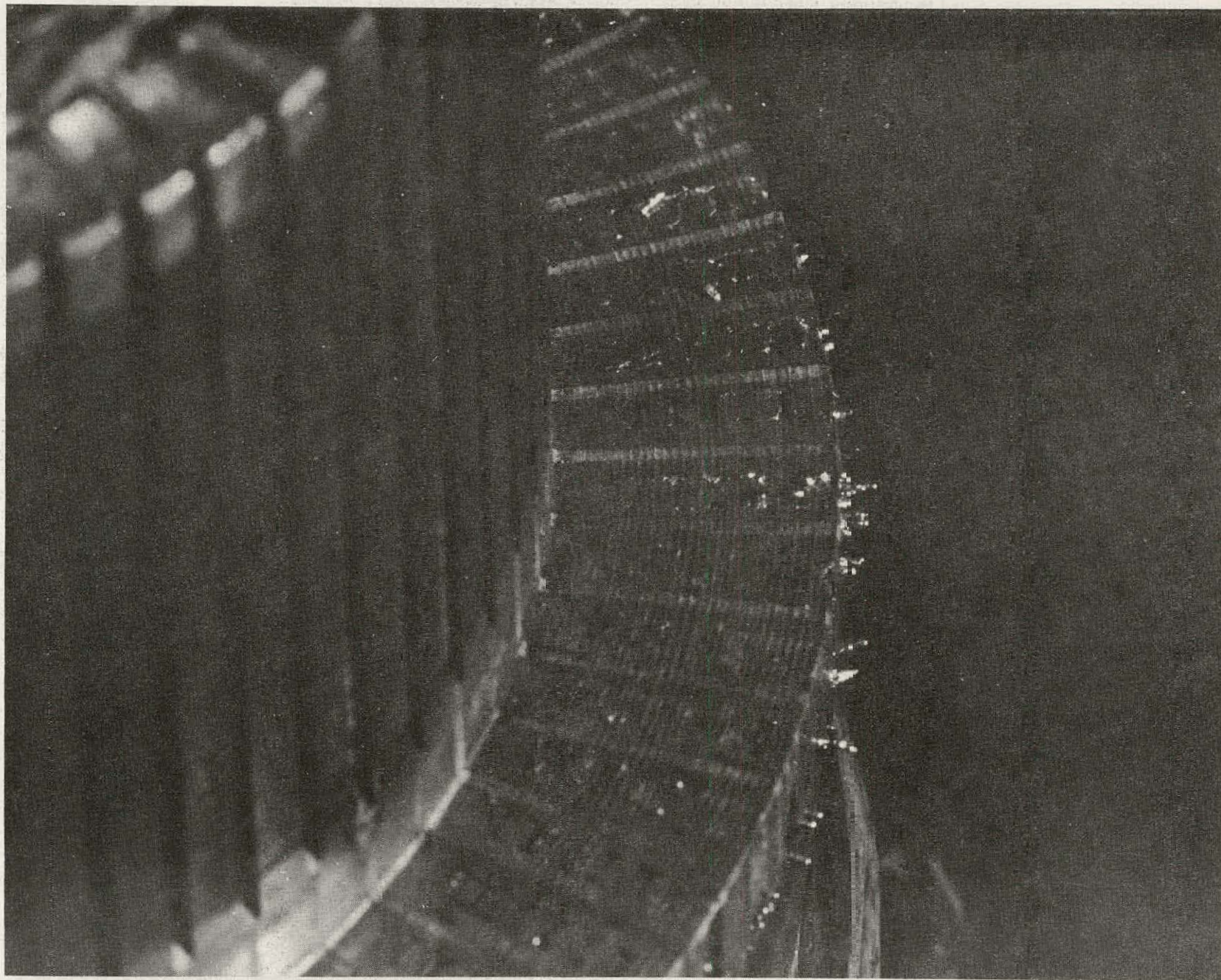
Figure 6.4. Motor damage to commutator risers caused by disintegration of soft solder joints.
