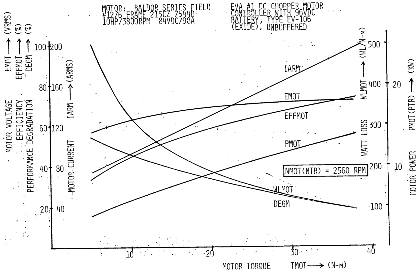
Figure 13.51. Motor performance @ 2560 RPM, pulsed DC power.
