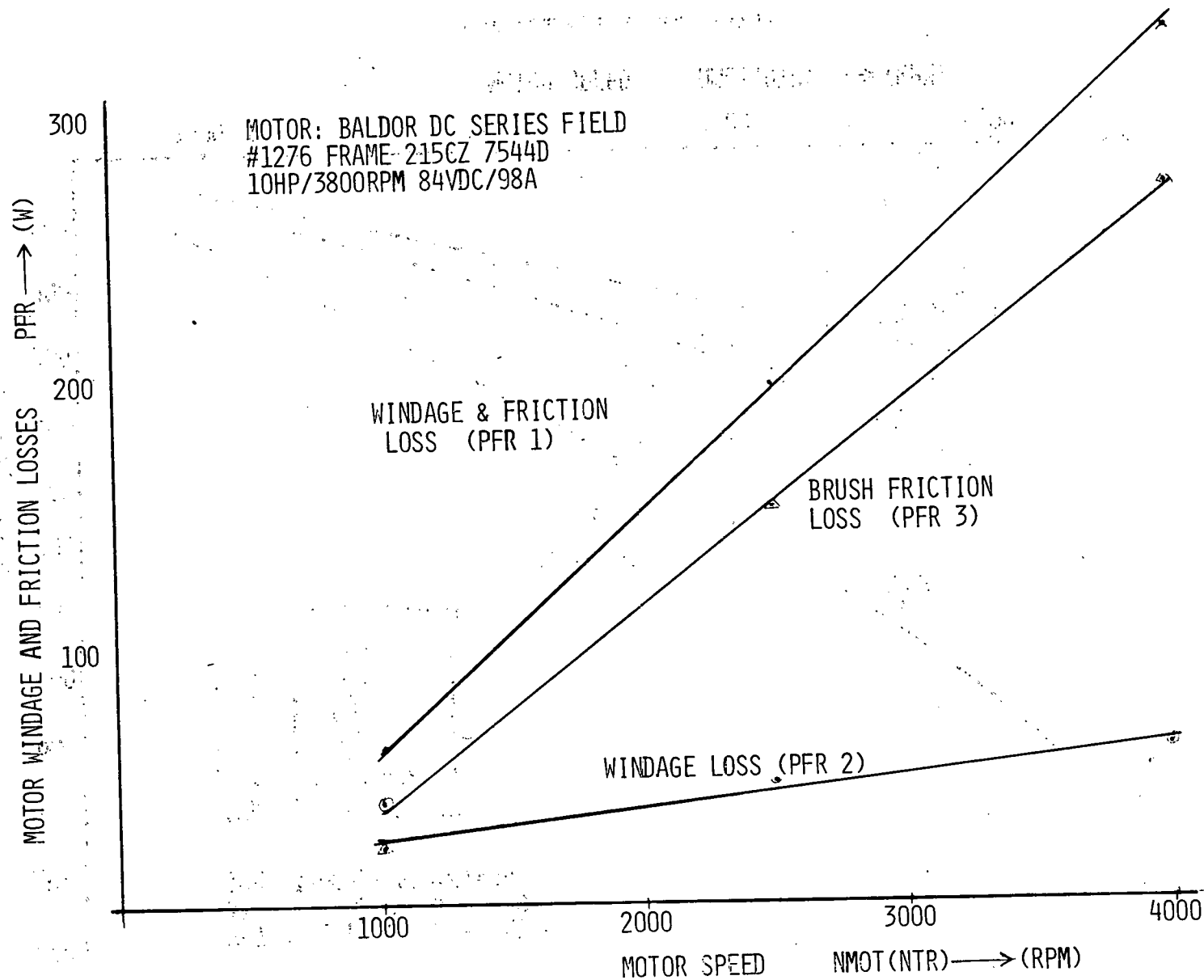
Figure 12.4. Windage and friction loss.
