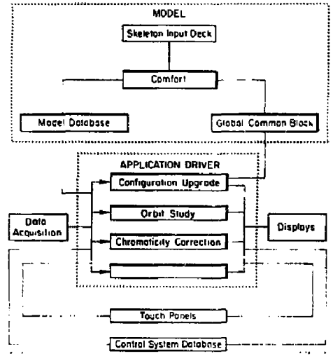
Fig. 1. Functional diagram of the model driven control system.
