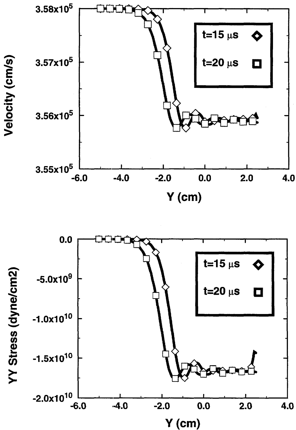
Figure 12. Profiles of the Y component of velocity and the YY component of stress along the axis of the rod from the ALEGRA calculation of case 5842 at times of 15 and 20 \mu s .
