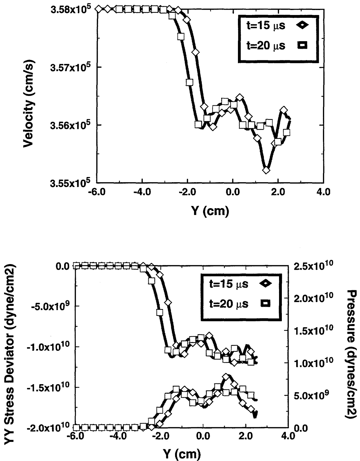
Figure 13. Profiles of the Y component of velocity and the YY stress deviator and pressure along the axis of the rod from the CTH calculation of case 5842 at times of 15 and 20 \mu s .
