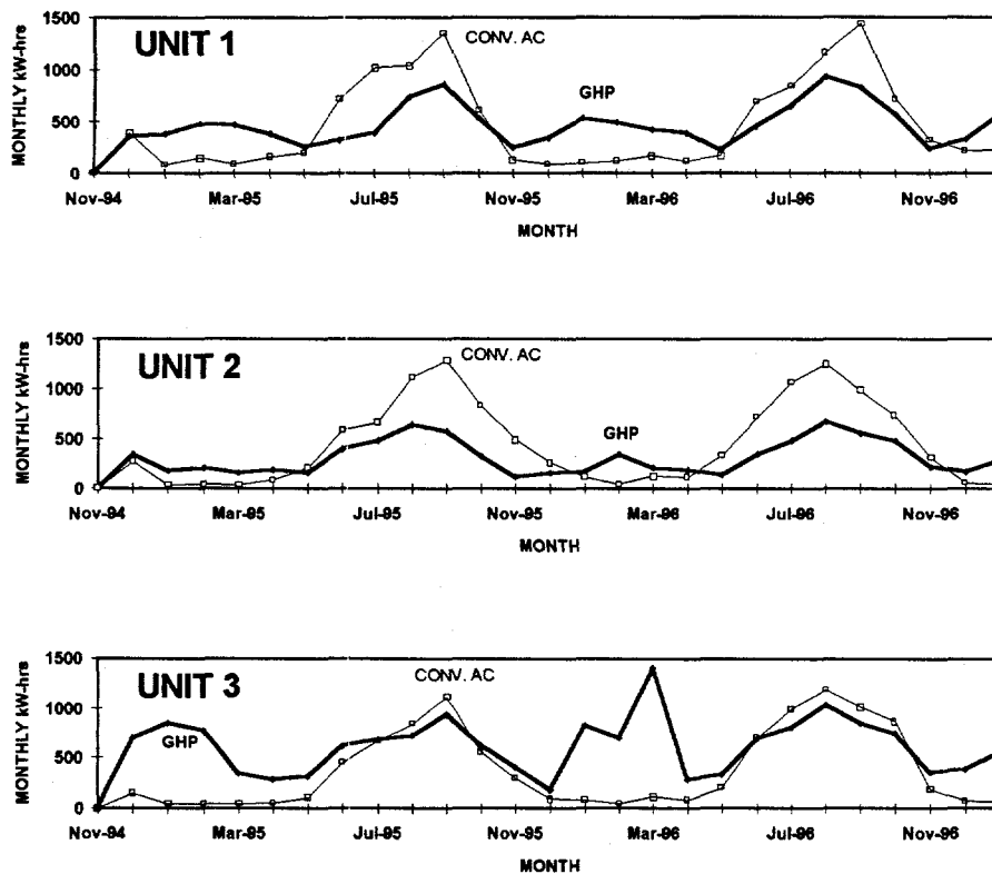
Figure 14. Monthly HVAC electrical energy use for GHP and conventional units at Ft. Hood. Conventional AC air handler energy not included in these figures.
