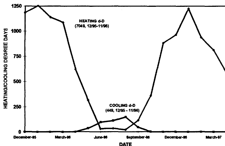
Figure 21. Measured 15 minute average heating (65 °F) and cooling (70 °F) degree days
