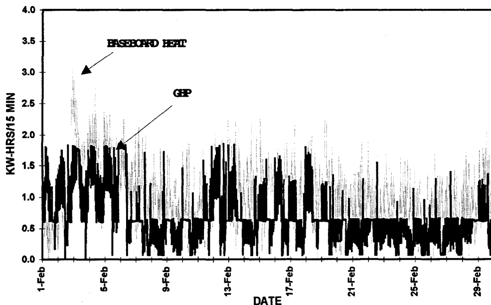
Figure 29. Peak HVAC demand for unit 1 GHP and resistance heat homes
