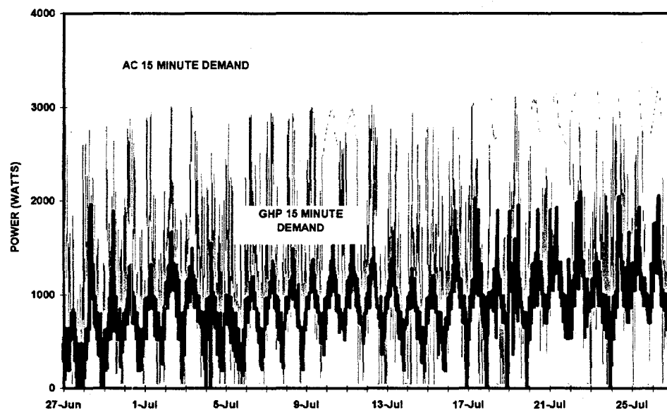
Figure 15. Demand reduction observed on unit 2, July 1995
