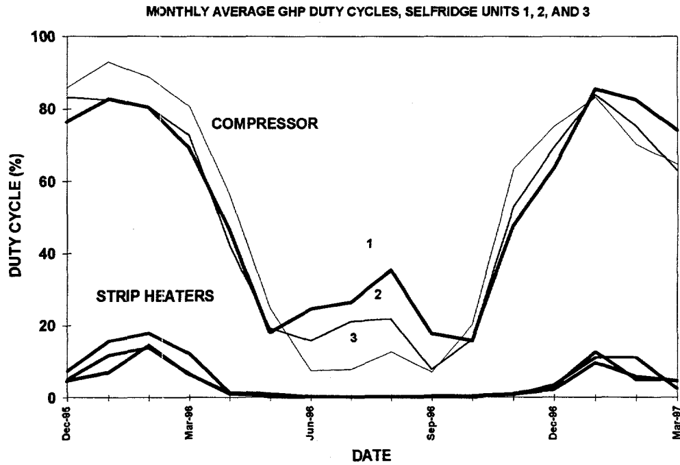
Figure 25. Monthly average duty cycles for the GHP compressors and resistance heaters.
