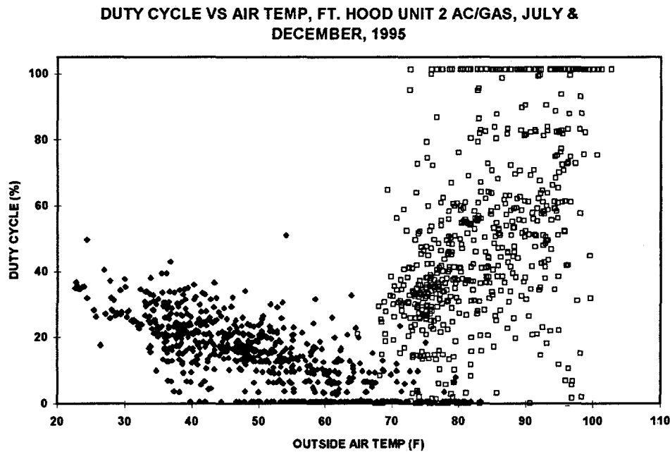
Figure 13. Hourly average duty cycle for unit 2 furnace and AC
