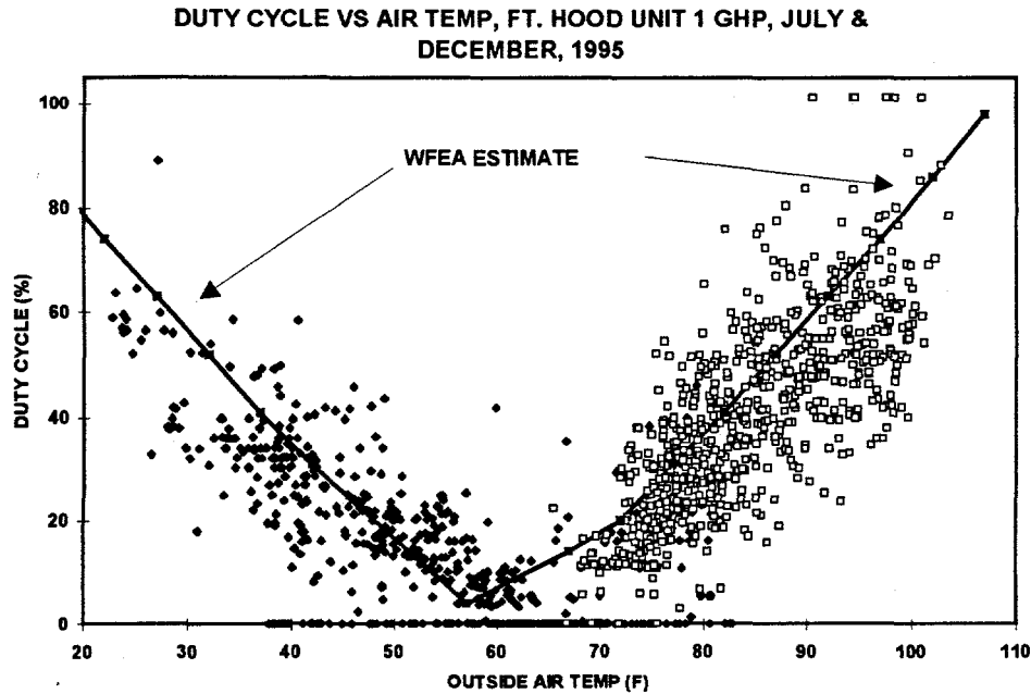
Figure 12. Hourly average duty cycle for unit 1 GHP. The solid points correspond to heating conditions, the open points for cooling.
