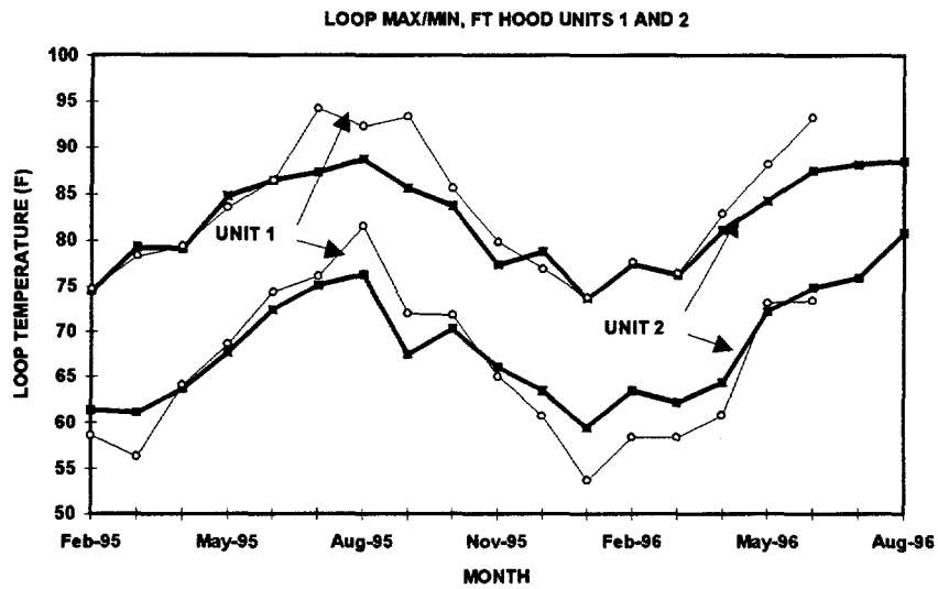
Figure 10. Loop temperature extremes (hourly averages)
