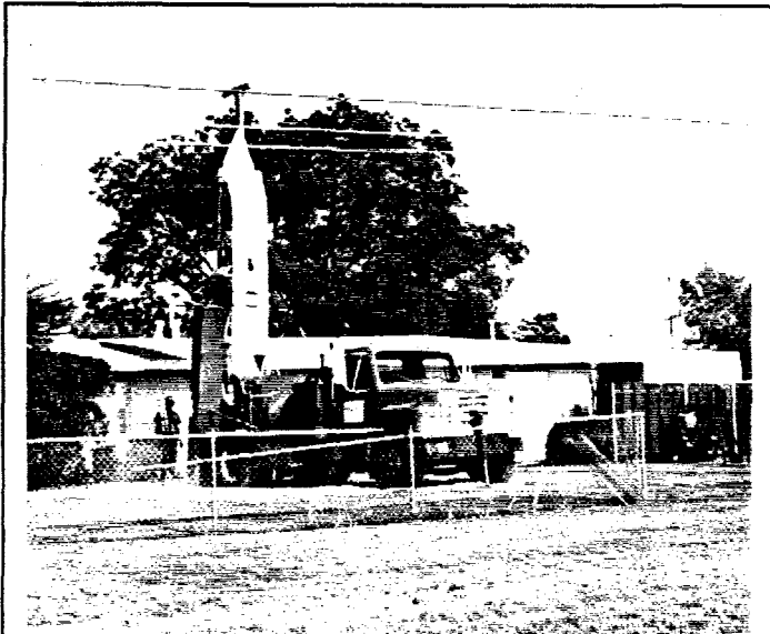
Figure 3. Drilling operation at Ft. Hood
