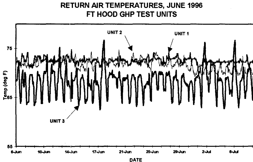
Figure 9. Summer return air temperature, GHP test units
