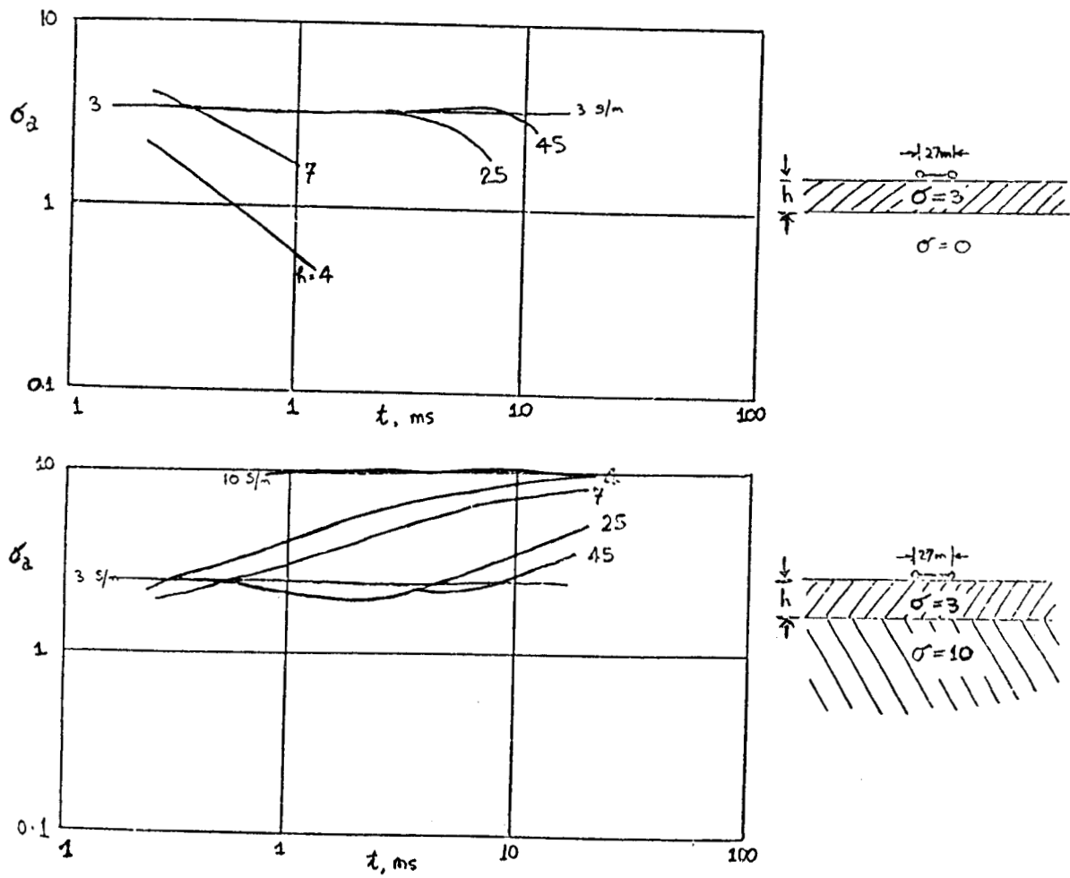
Fig. 2. One-loop response -- small loop
