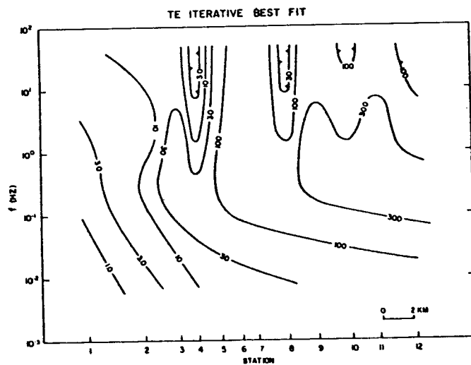
FIGURE 7: Calculated apparent resistivity pseudosection for previous trial-and-error best-fit model. Contours are in u-m.
