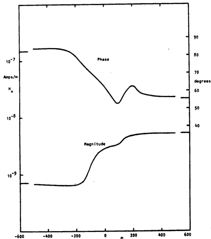
Figure 6. Contact response on H_x . Long tick marks on both axes indicate analytic solutions.
