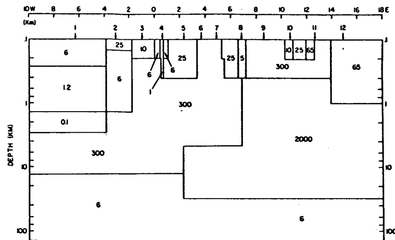
FIGURE 6: Trial-and-error best-fit model for observed transverse electric pseudosection of Figure 9. Resistivities are in u-m.
