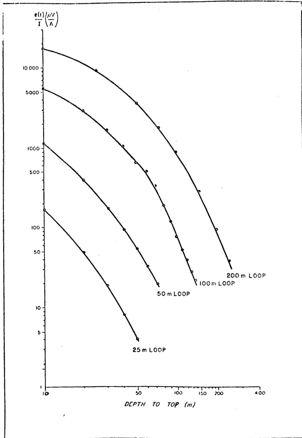
Fig. 5. Woodlawn model: response for different depths of orebody t = 1.1\text{ms}
