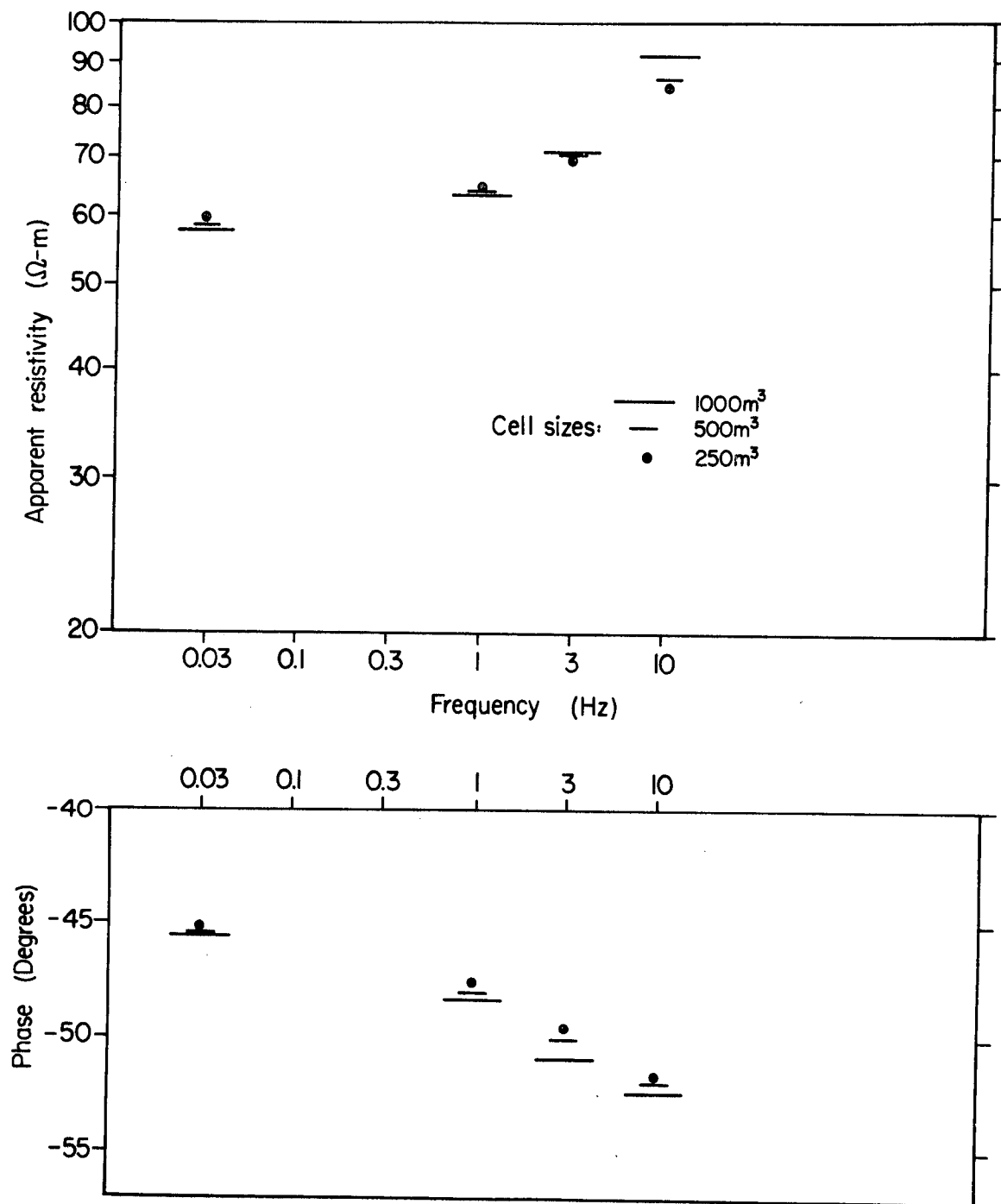
Figure 12 Convergence at Point A for E_1 Excitation.
