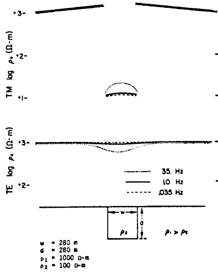
FIGURE 9: TM and TE multifrequency profiles for single, outcropping, shallow, 2-D conductor.
