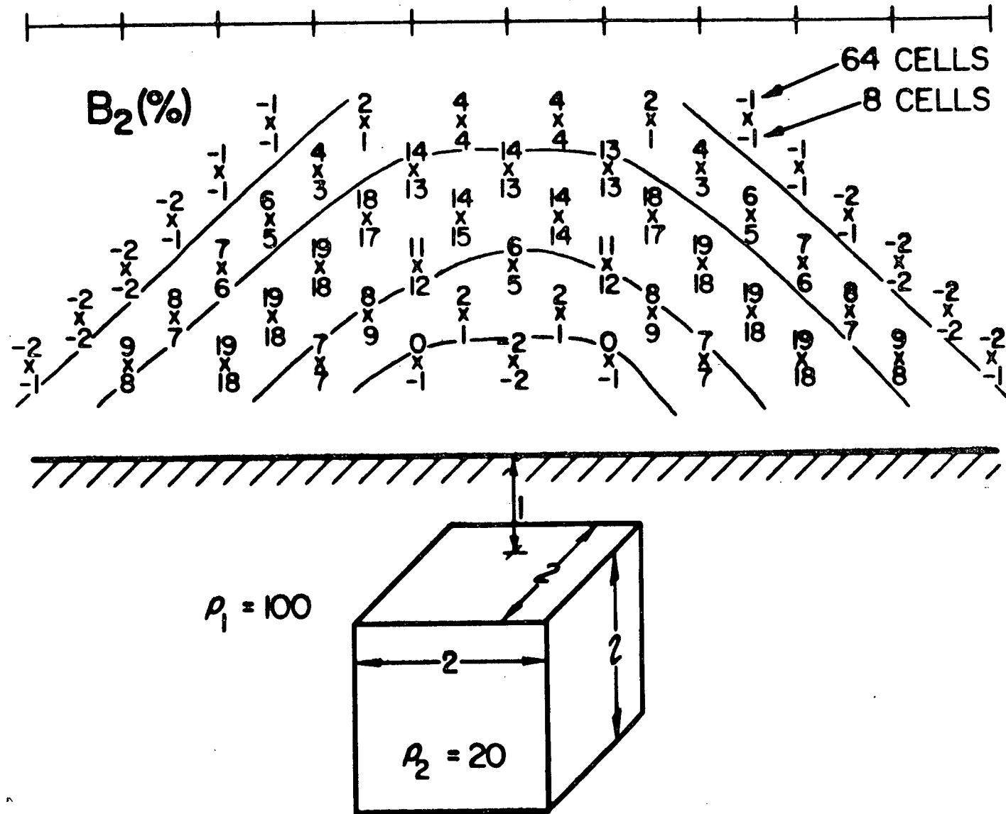
Figure 1 Check for Convergence and Reciprocity for Integral Equation Solution
