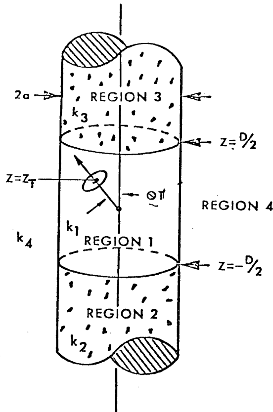
Figure 1 Model Geometry
