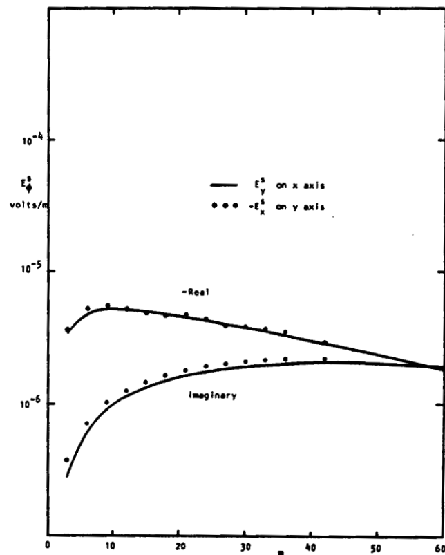
Figure 2. Symmetry of horizontal electric fields. Frequency = 25 kilocycles/sec Half space resistivity = 100 ohm-meters Source; A vertical magnetic dipole of unit moment located at 2 meters above the ground
